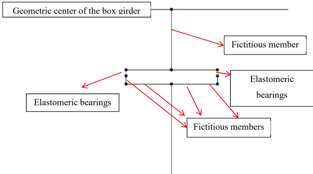
Figure 4.1. Modelling of superstructure – pier connection.
