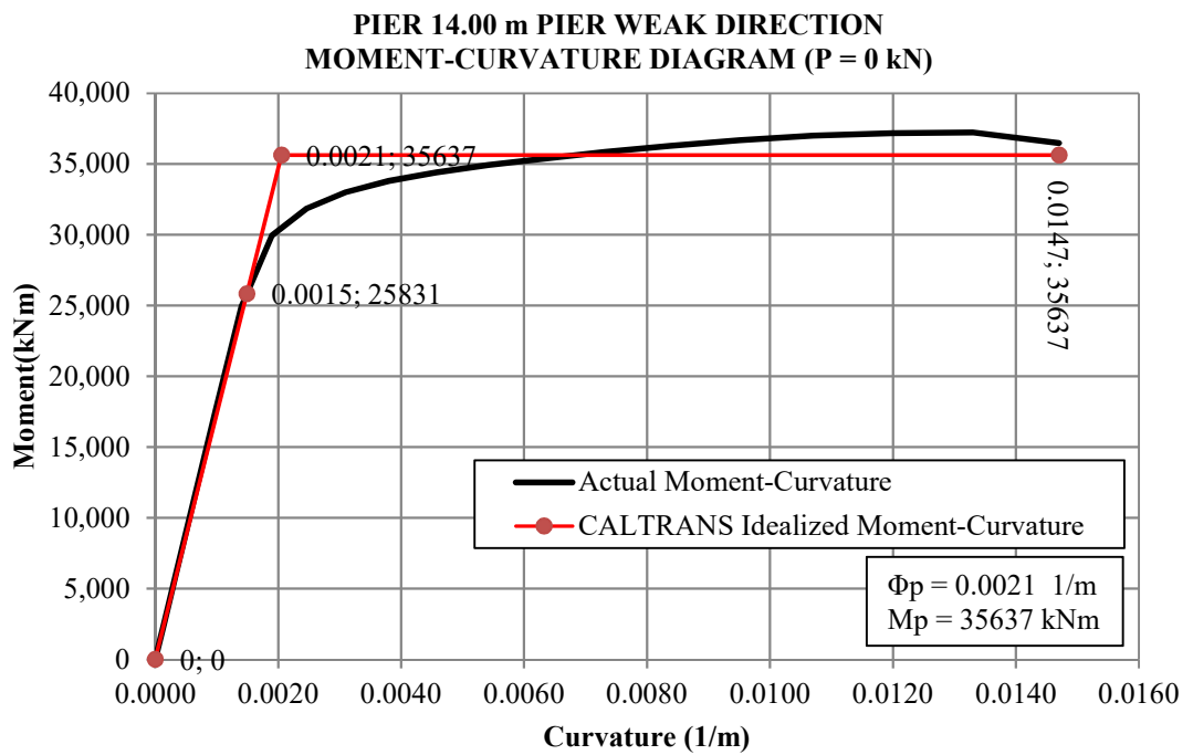
Figure 3.31. Pier 14.00 m pier weak direction moment-curvature diagram.
