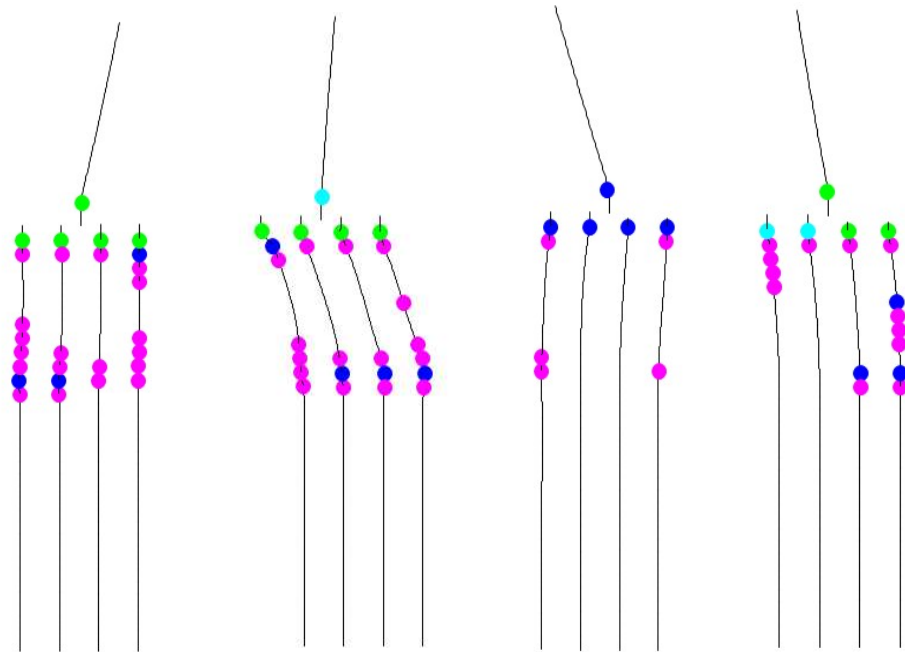
Figure 5.6. Bridge II record 68_090 / 174_11230 / 767_000 / 829_360 plastic hinge formation.
