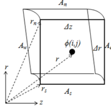
Figure 3.3. Control volume cell in cylindrical coordinates.
