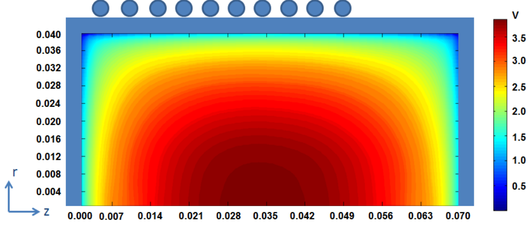
Figure 5.5. Electric potential distribution for the benchmark problem.
