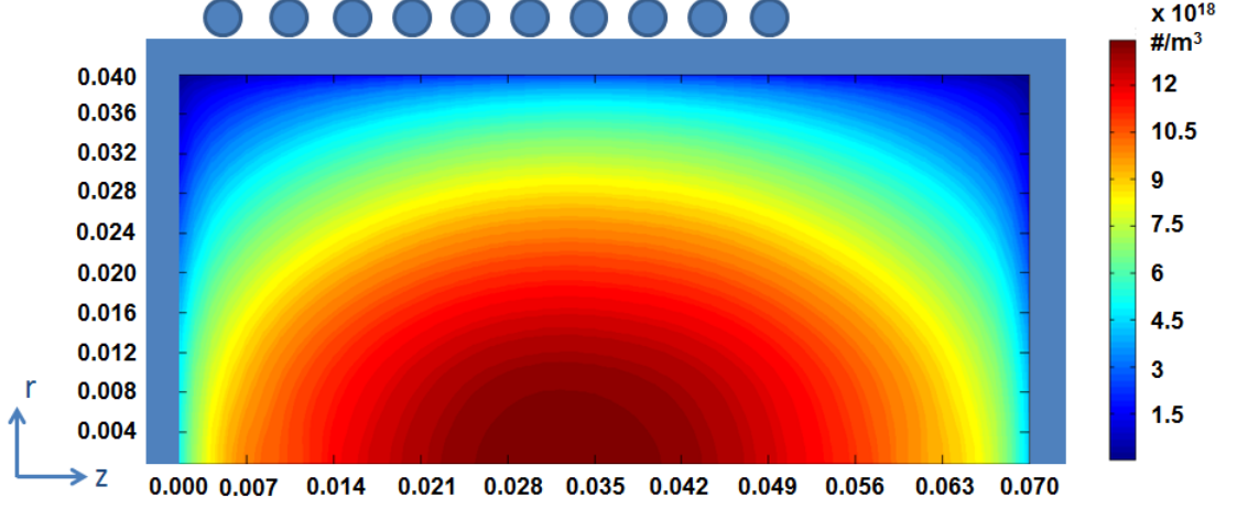
Figure 5.1. Plasma density at the end of 10 milliseconds. Due to the losses to the walls, plasma is confined in the center region of the domain.
