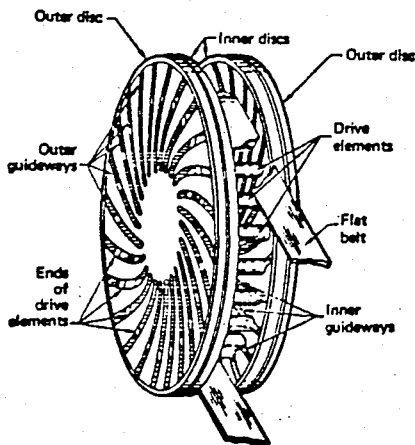
Fig. 8.5 Flat-belt CVT
