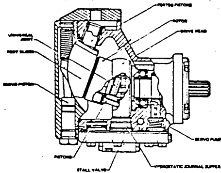
Fig 3.1 Ifield Pump/Motor for Hydrostatic CVT
