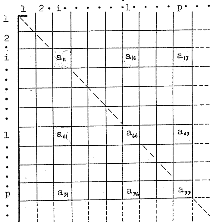
FIG.8- Assemblage of global matrices,
