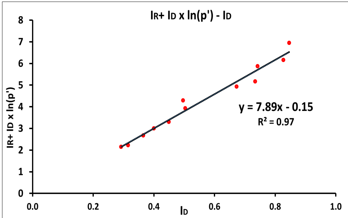
Figure 4.10. Determination of Q and R parameter from AC stress path of S1 sand.
