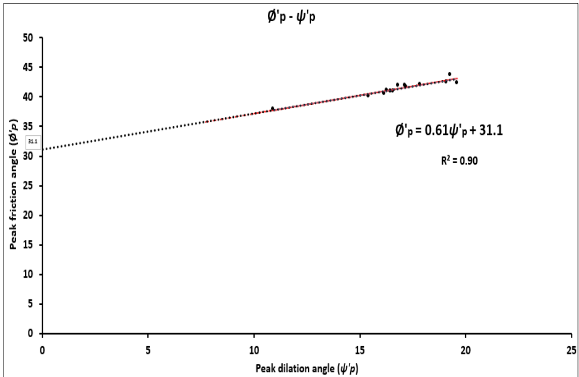
Figure 4.3. \psi'_p and \phi'_p relationship for AC stress path triaxial testing of S3 sand.
