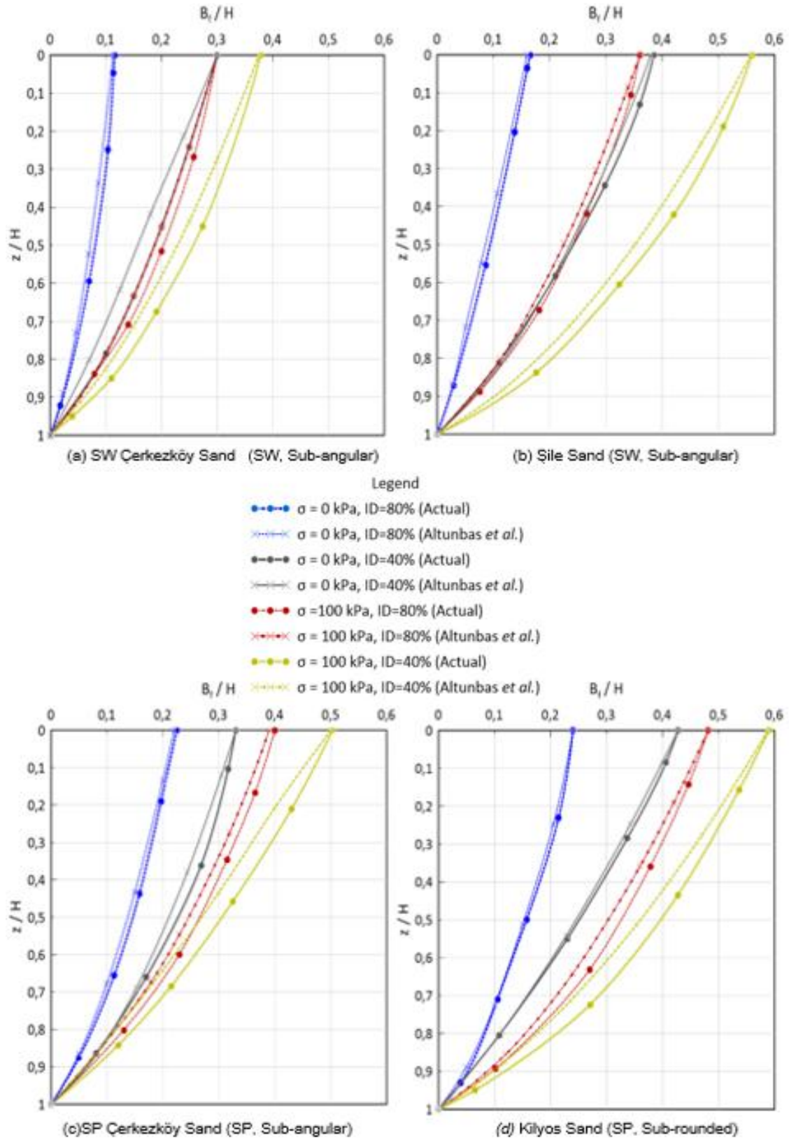
Figure 4.61. Actual - empirical failure surface geometry relationship of different sands at similar initial conditions.
