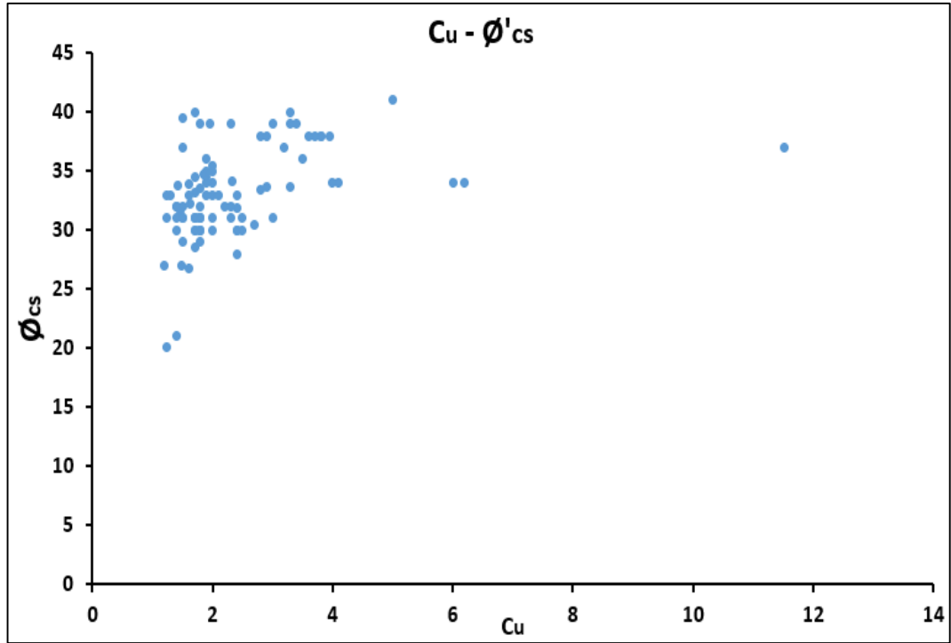
Figure 4.21. C_u - \phi_{cs} relationship.
