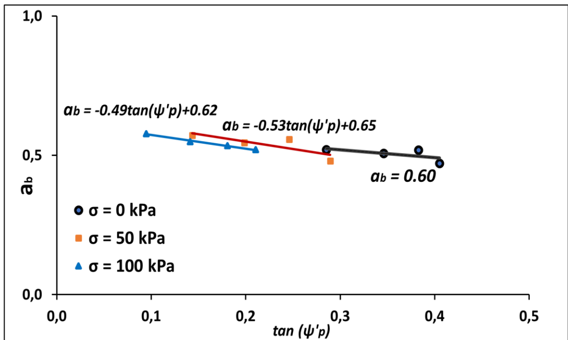
Figure 4.51. Influence of dilatancy on experimentally measured values of a_b for S3 Sand.
