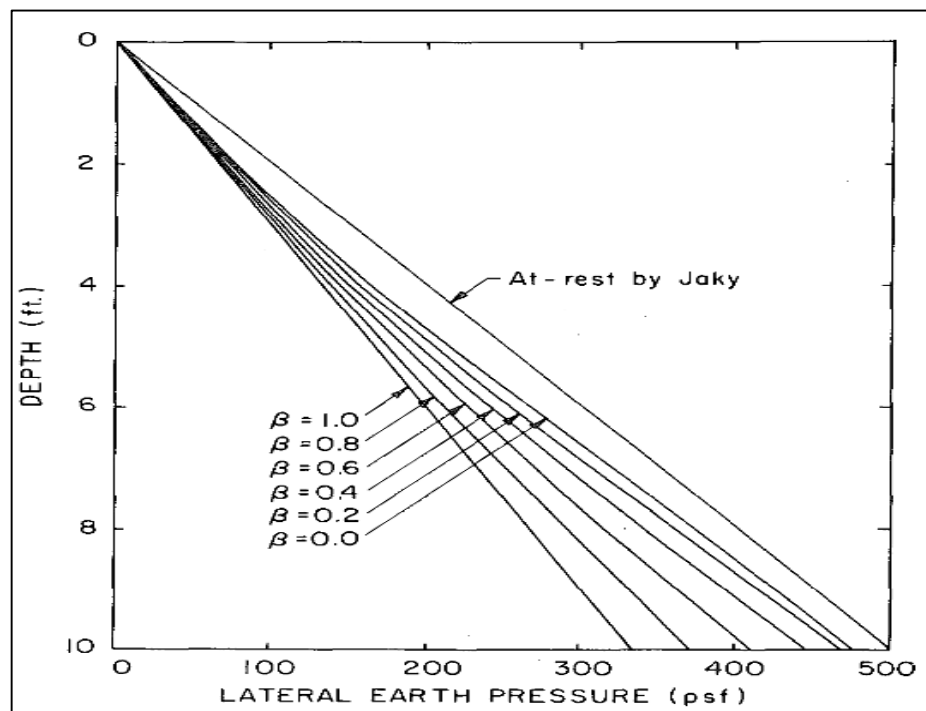
Figure 2.21. Variation in lateral earth pressures by retaining wall tilting (S. Bang, 1985).
