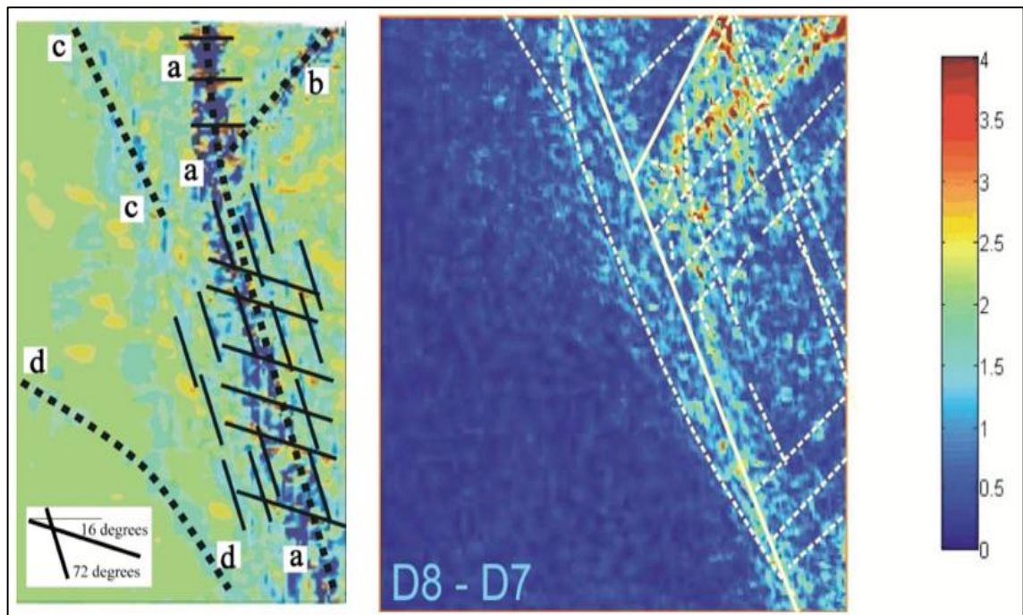
Figure 2.23. Imperfections and strain localization zones revealed by GeoPIV (Lesniewska and Wood, 2009).
