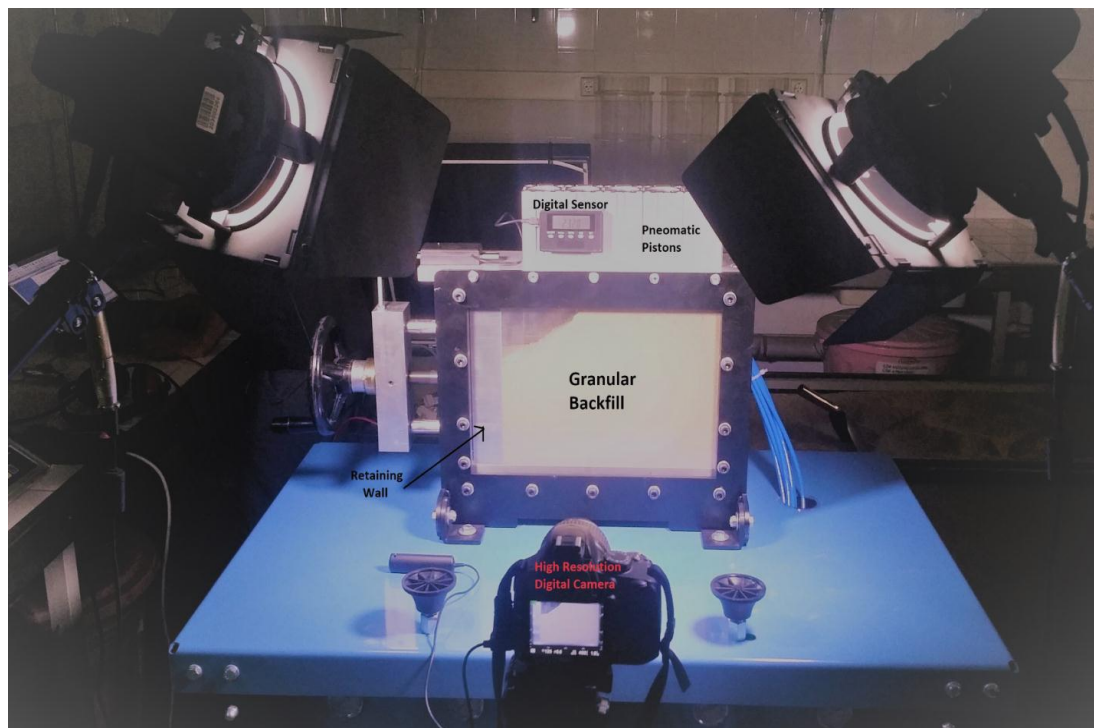
Figure 3.21. The physical test model used in retaining tests.
