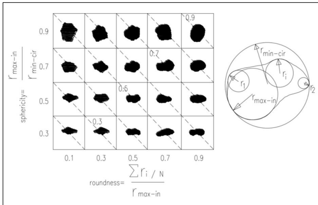
Figure 3.8. Sphericity – Roundness chart proposed by Krumbein and Sloss (1963).
