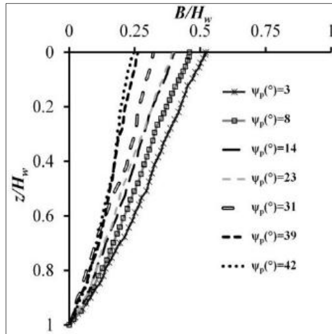
Figure 2.24. Dilatancy angle – failure surface relationship (Altunbas et al. , 2017).
