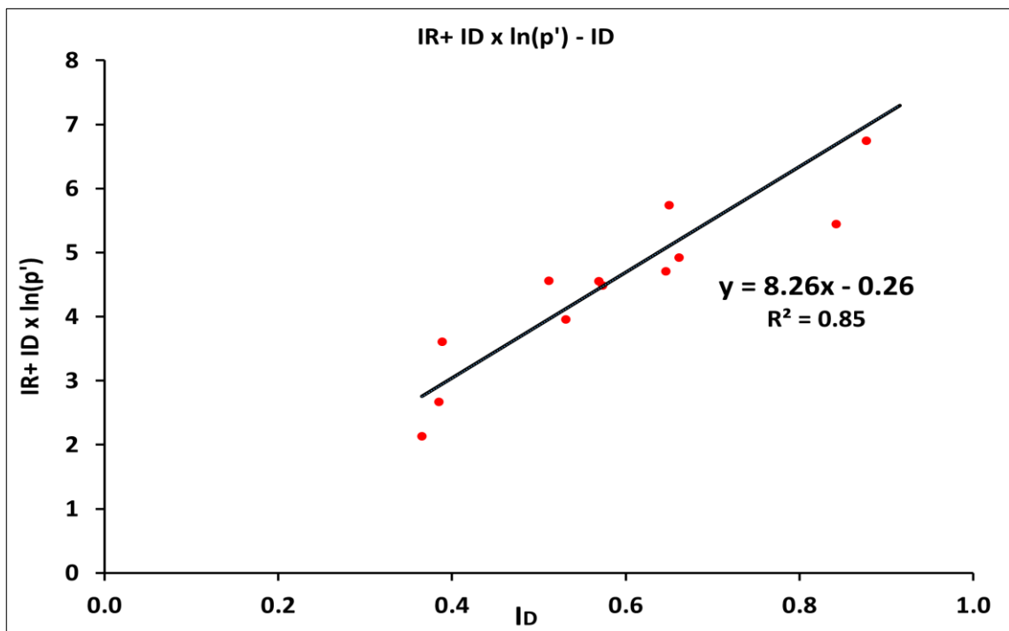
Figure 4.11. Determination of Q and R parameter from LE stress path of S1 sand.
