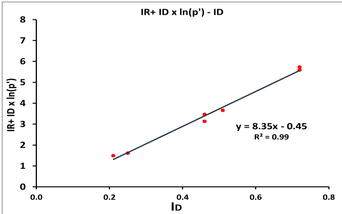
Figure 4.16. Determination of Q and R parameter from AC stress path of SW-S2.
