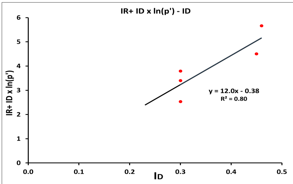
Figure 4.15. Determination of Q and R parameter from LE stress path of GB.
