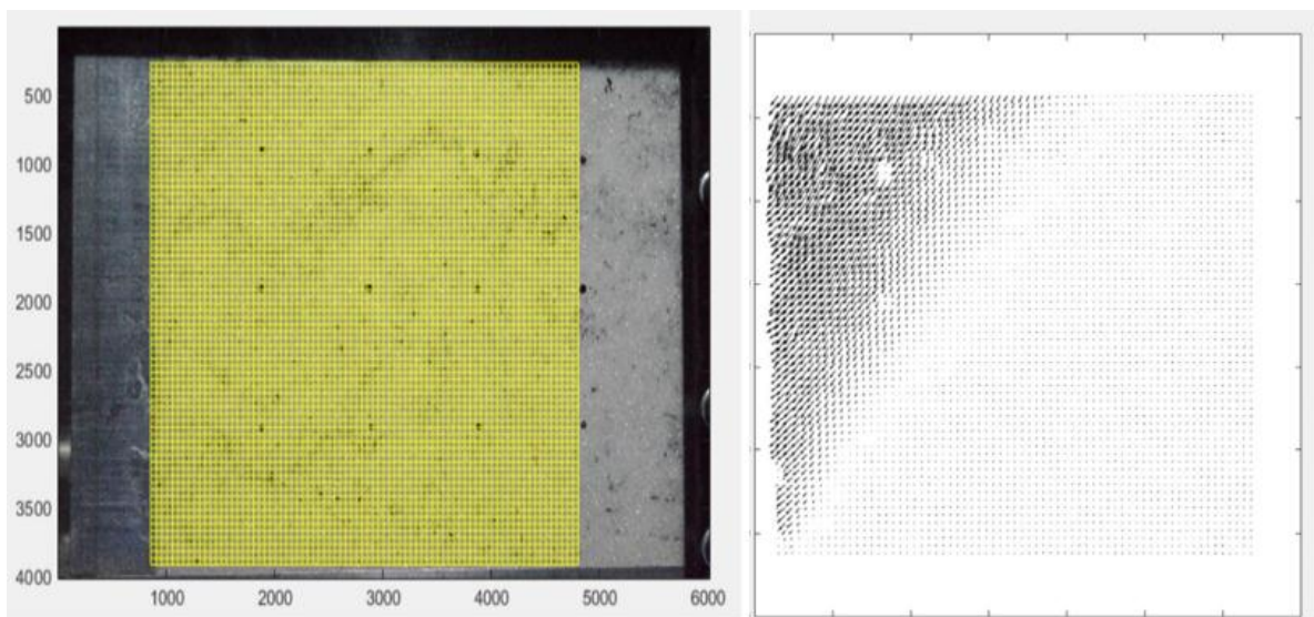
Figure 3.22. View of the generated mesh of square patches and the displacement vector field of the deformed mesh.
