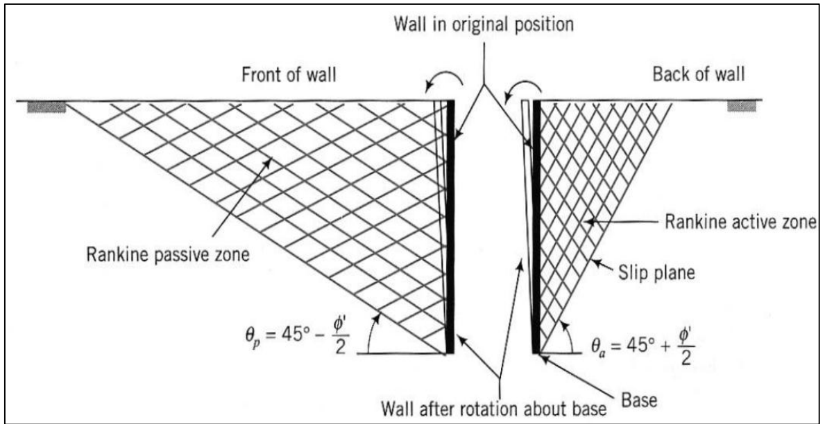
Figure 2.19. Slip planes within a soil mass near a retaining wall.
