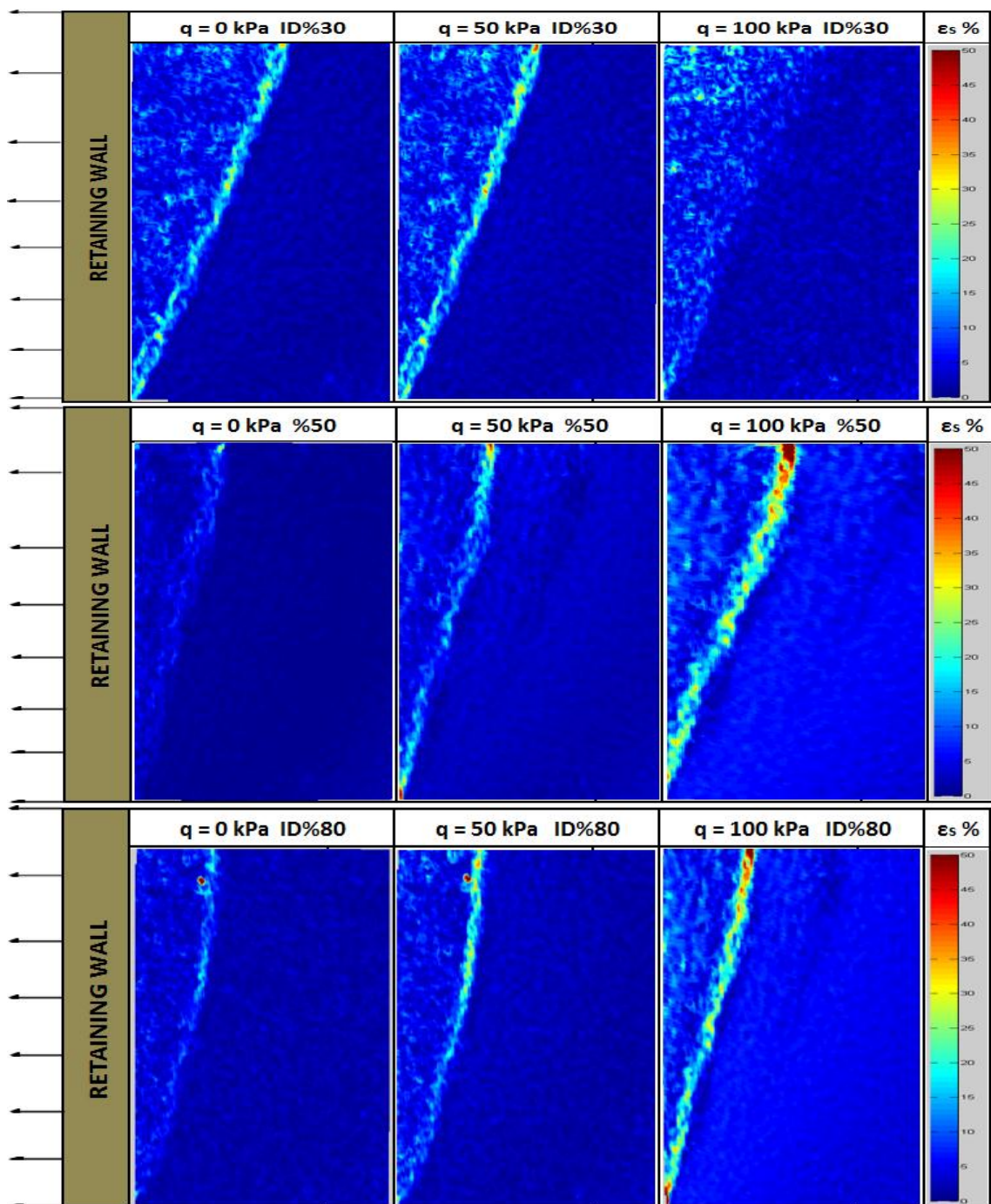
Figure 4.32. PIV analysis results for S1 sand.
