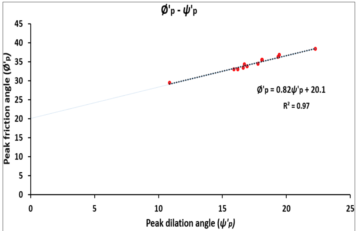
Figure 4.5. \psi'_p and \phi'_p relationship for AC stress path triaxial testing of GB.
