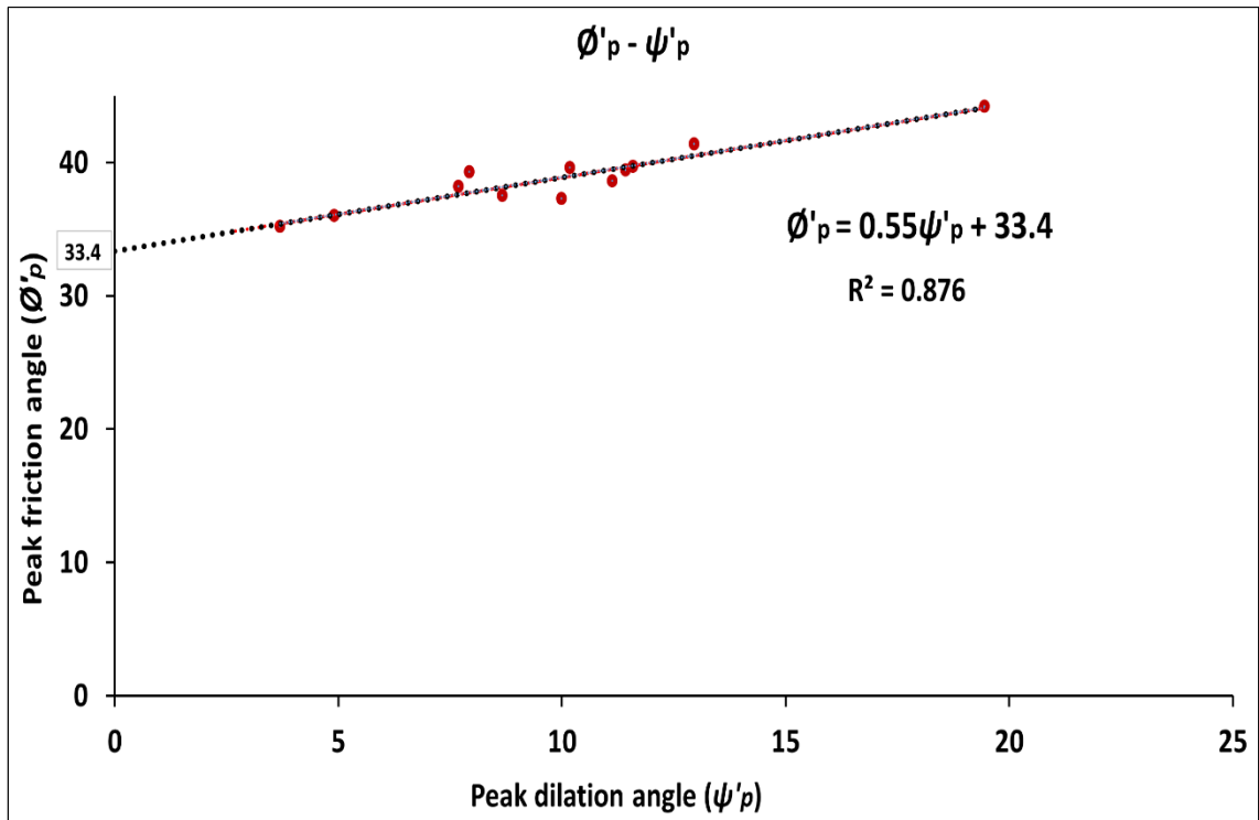
Figure 4.1. \psi'_p and \phi'_p relationship for AC stress path triaxial testing of S1 sand.
