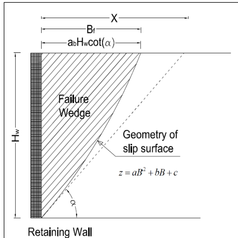
Figure 2.25. Geometrical parameters of the shear band (Altunbas et al. , 2017).
