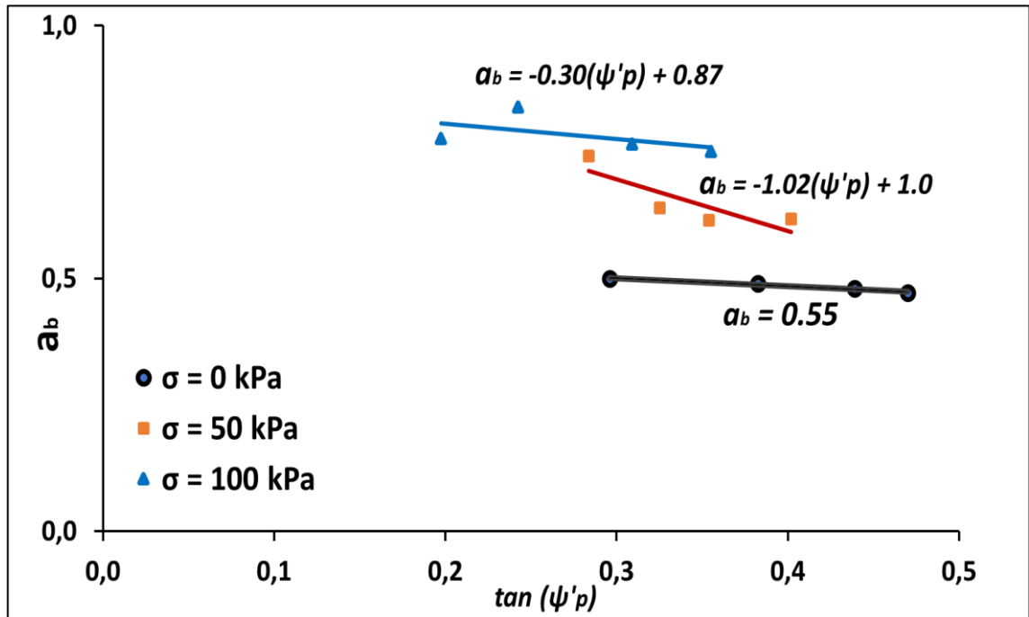
Figure 4.50. Influence of dilatancy on experimentally measured values of a_b for S1 Sand.
