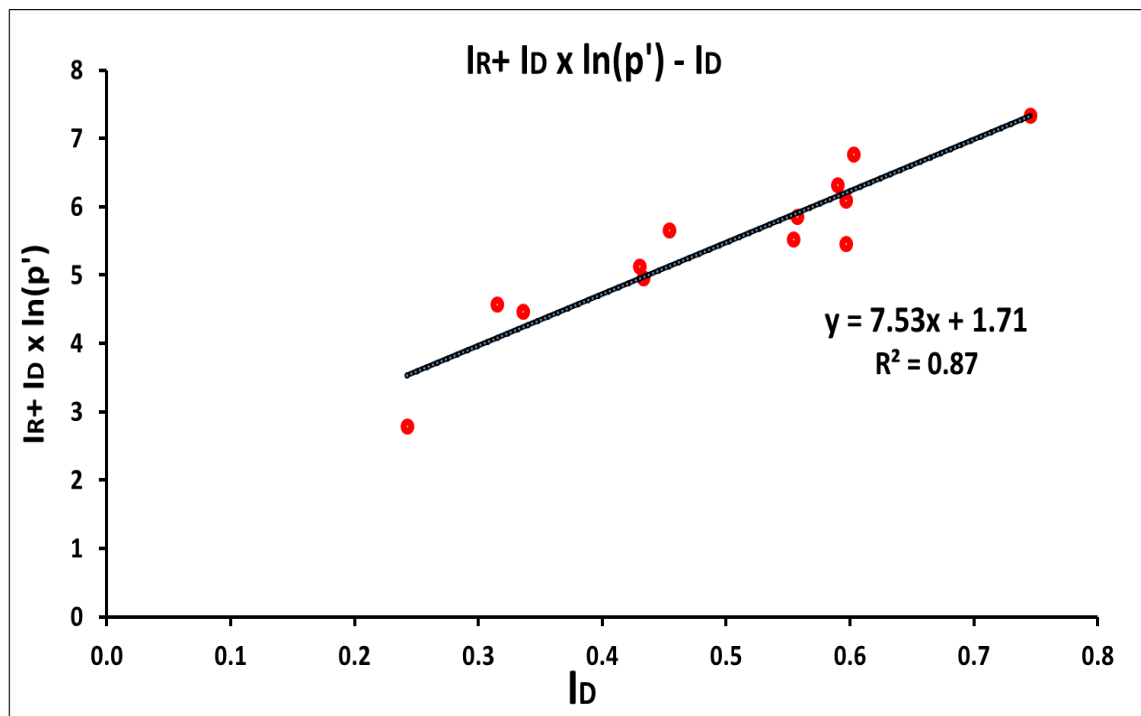
Figure 4.12. Determination of Q and R parameter from AC stress path of S3 sand.
