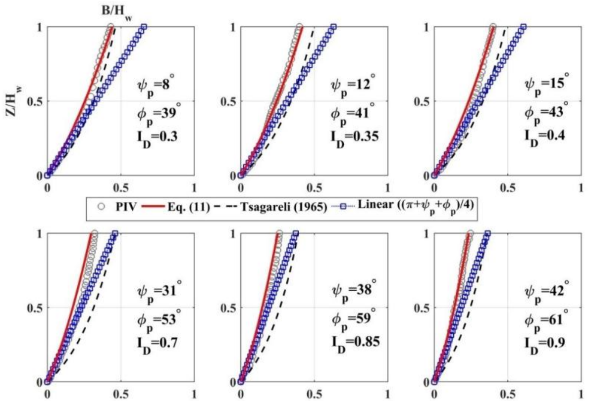
Figure 2.27. Comparison of estimated and experimentally visualized failure surfaces (Altunbas et al. , 2017).
