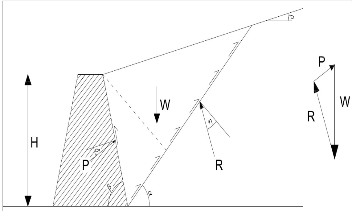
Figure 2.18. Coulomb failure wedge.
