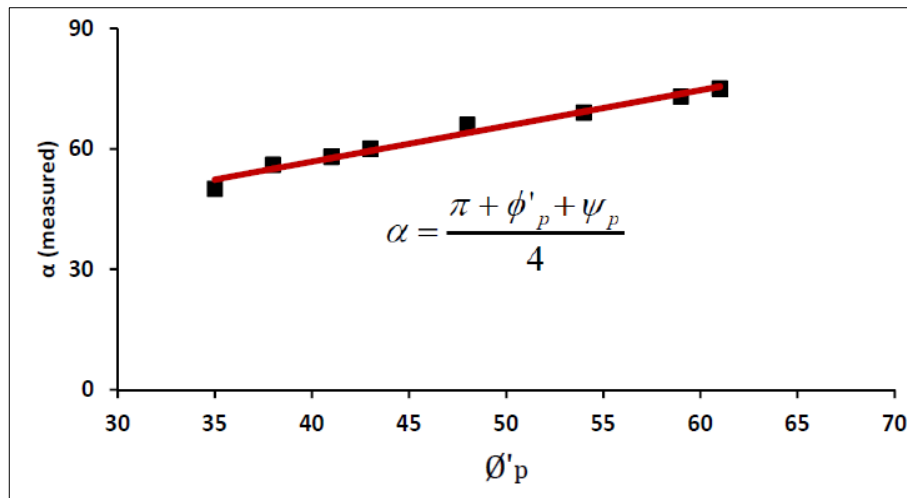
Figure 2.26. Variation of \alpha with \phi'_p as obtained from model test results (Vardoulakis, 1980).
