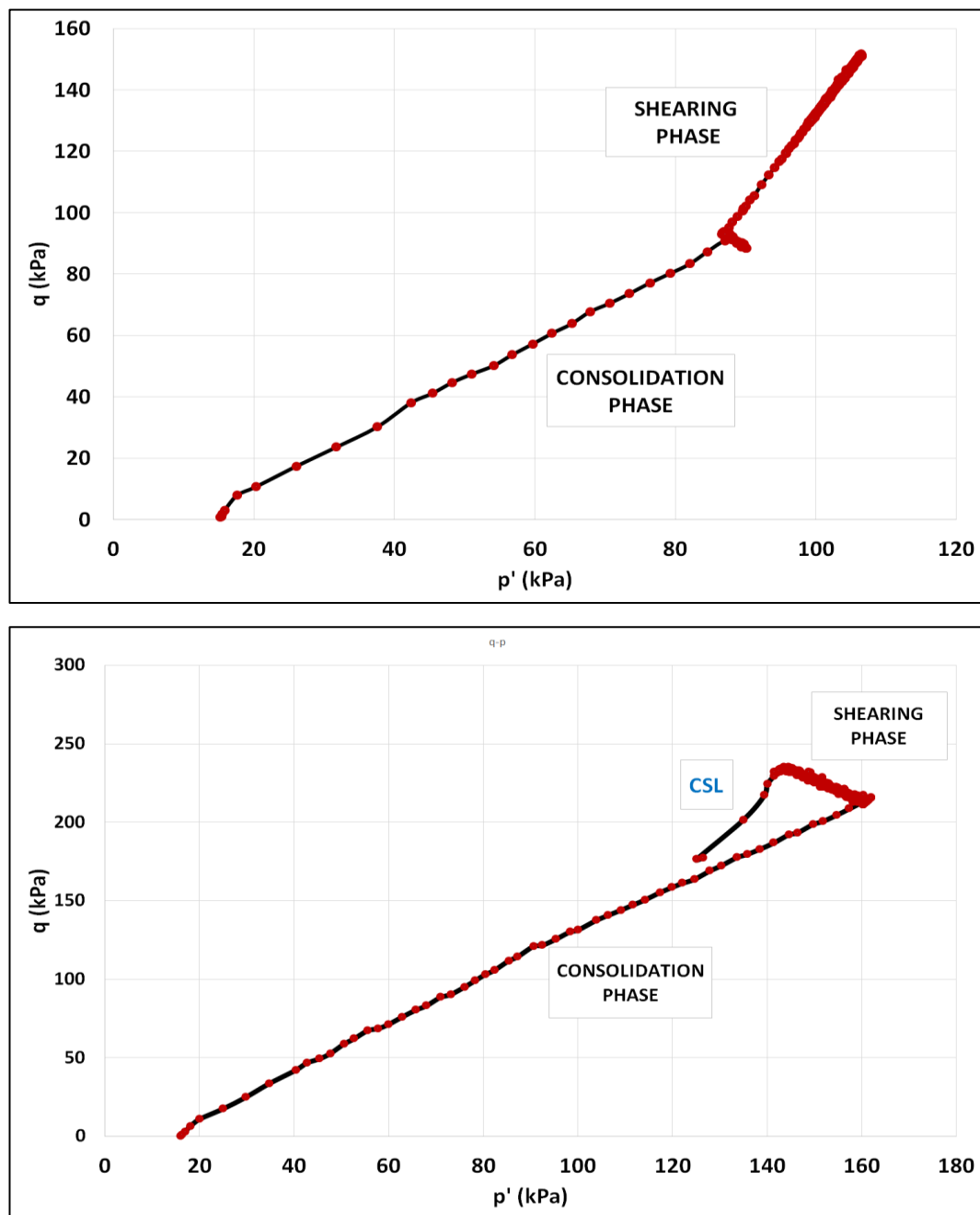
Figure 3.14. q - p relationship for AC and LE stress path.
