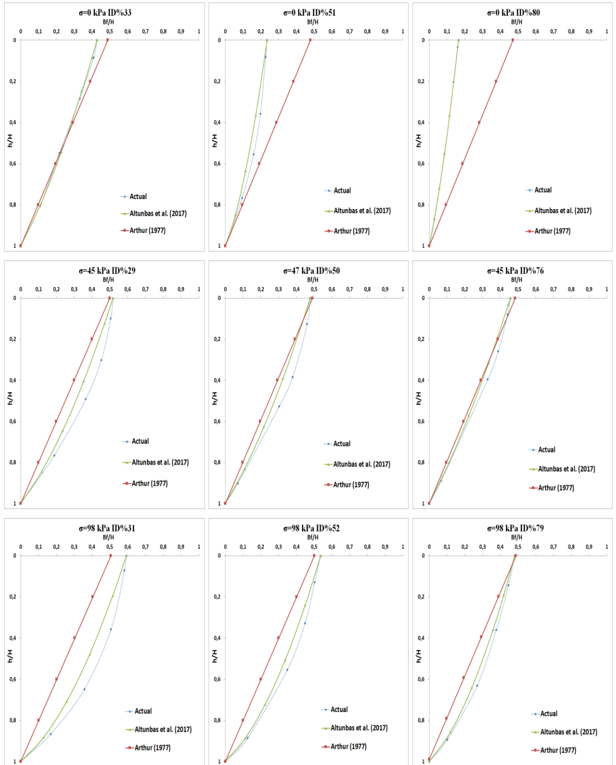
Figure 4.55. Comparison between plots of estimated and actual failure surfaces on normalized coordinate system for varying dilatancy values of physical model experiment data of SW-S2.
