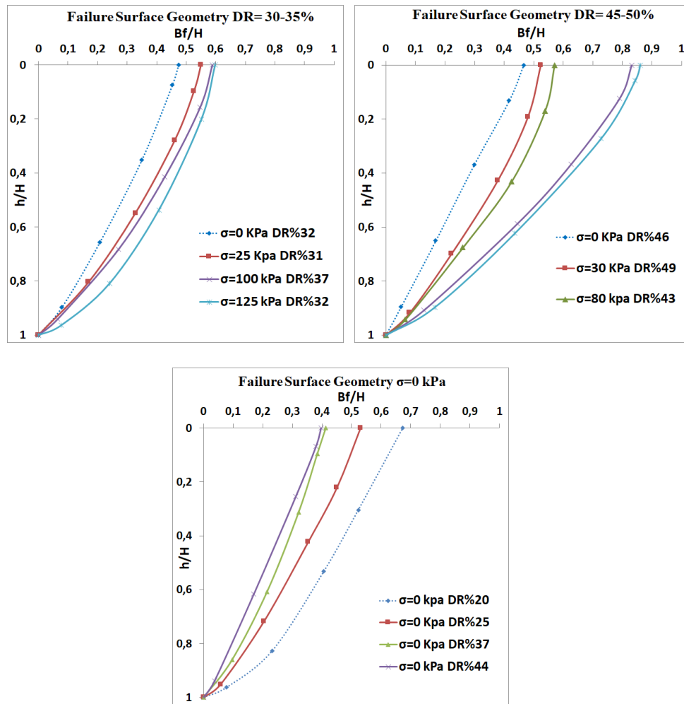
Figure 4.44. Active failure surface geometries of GB at varying surcharge and densities.
