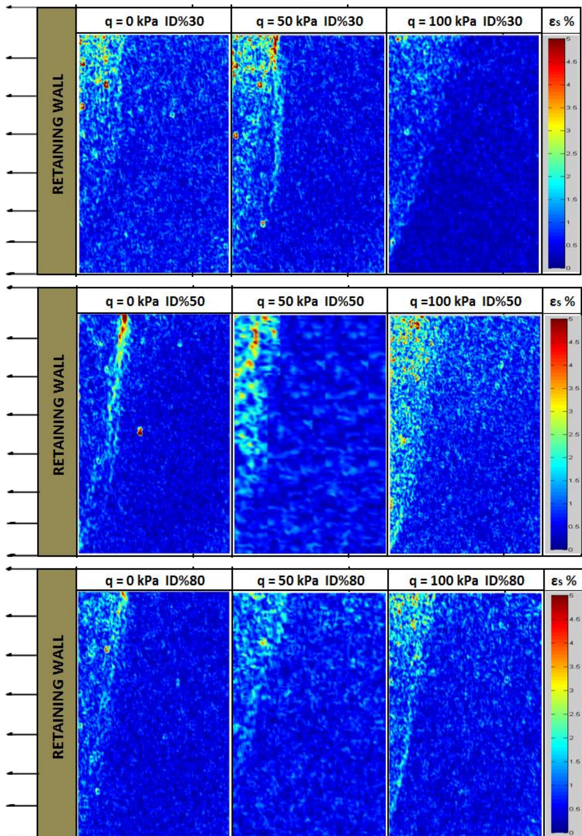
Figure 4.33. PIV analysis results for S3 sand.
