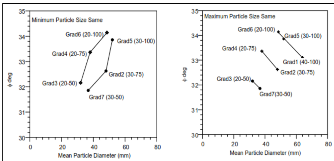
Figure 2.14. Influence of grain distribution on friction (Latha and Sitharam, 2008).
