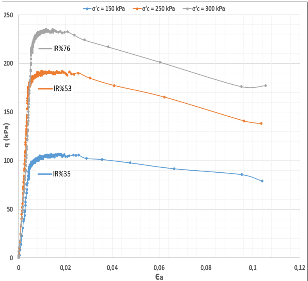
Figure 2.1. Stress-strain relationship of a granular soil at varying confining pressure and relative density ranges.
