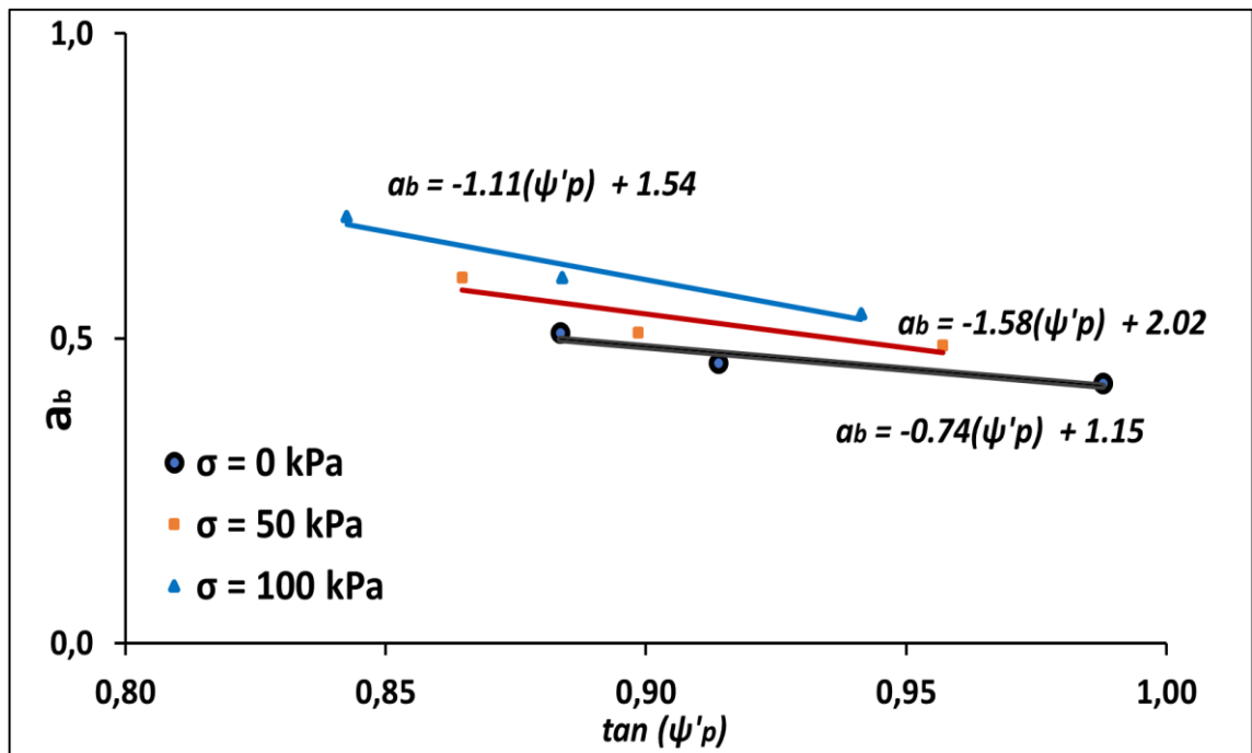
Figure 4.53. Influence of dilatancy on experimentally measured values of a_b for S2-SP.
