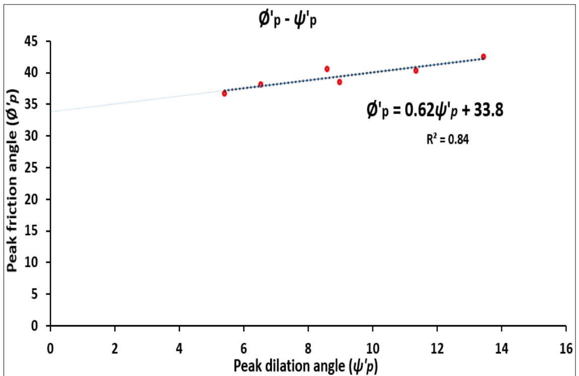
Figure 4.8. \psi'_p and \phi'_p relationship for AC stress path triaxial tests of SP-S2.
