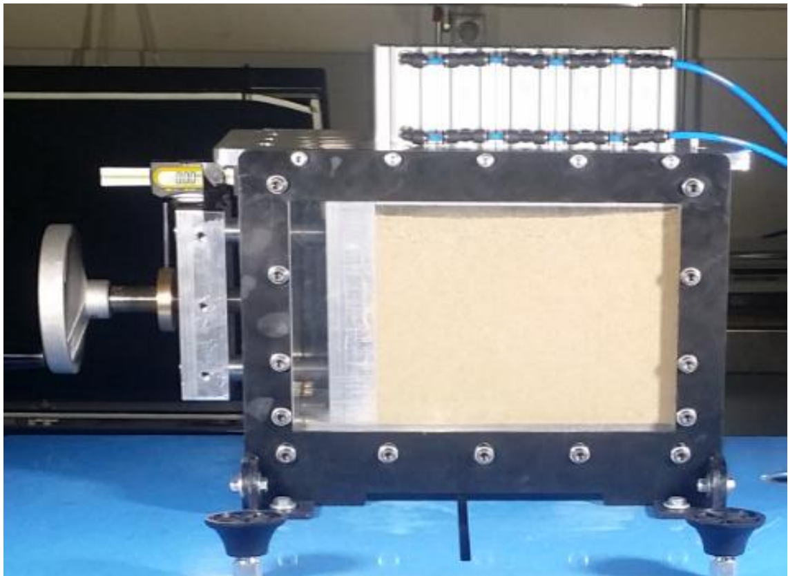
Figure 3.15. Front view of the physical retaining wall model.
