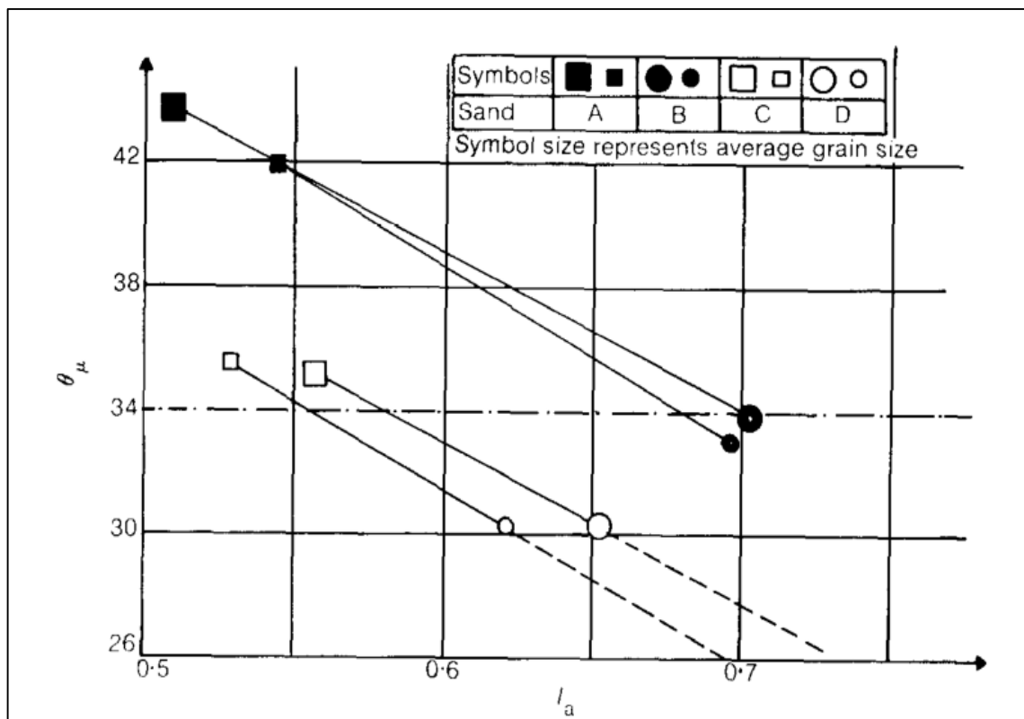
Figure 2.10. Asperity index – interparticle friction angle relationship (E. Frossard, 1979).
