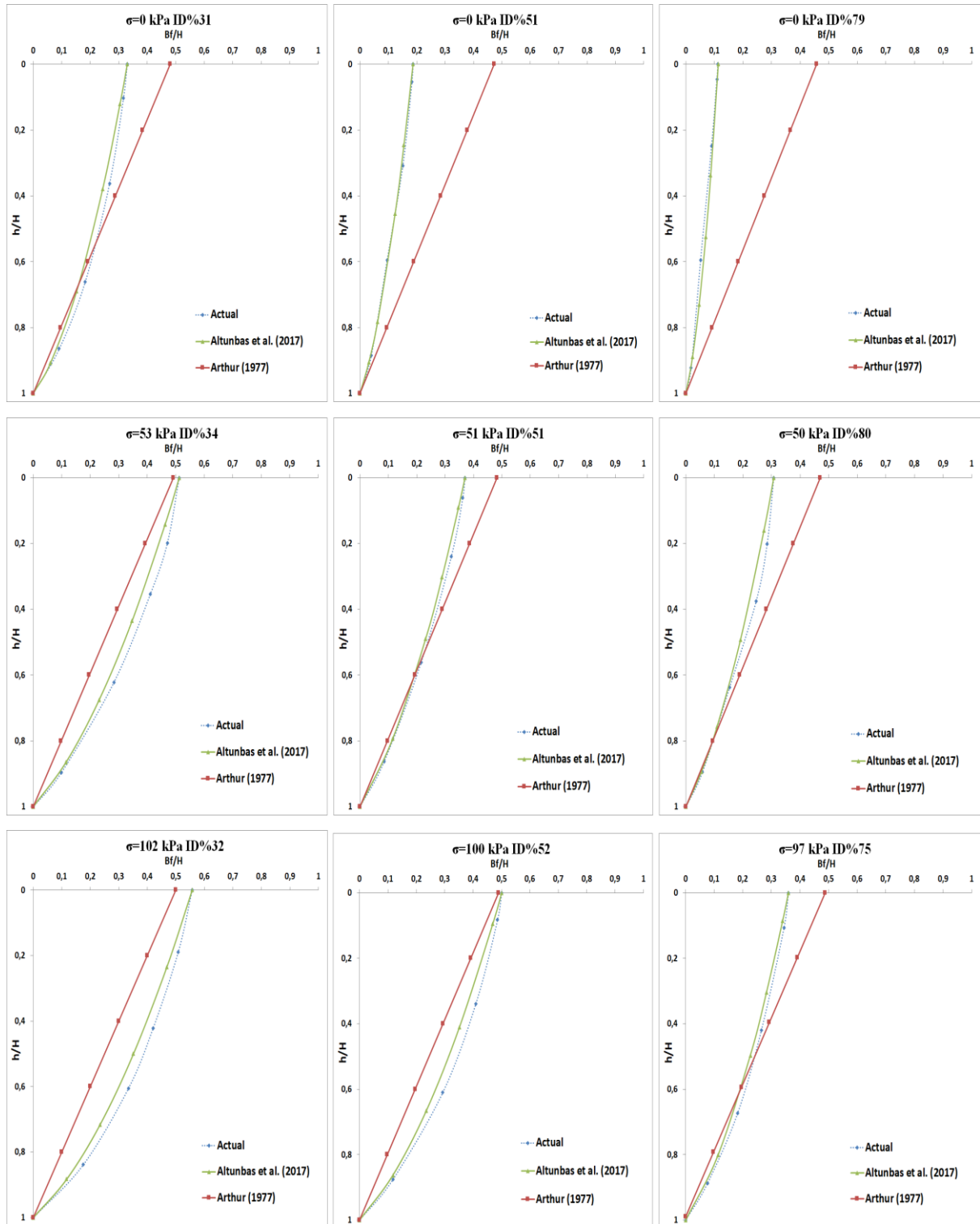
Figure 4.57. Comparison between plots of estimated and actual failure surfaces on normalized coordinate system for varying dilatancy values of physical model experiment data of SP-S2.
