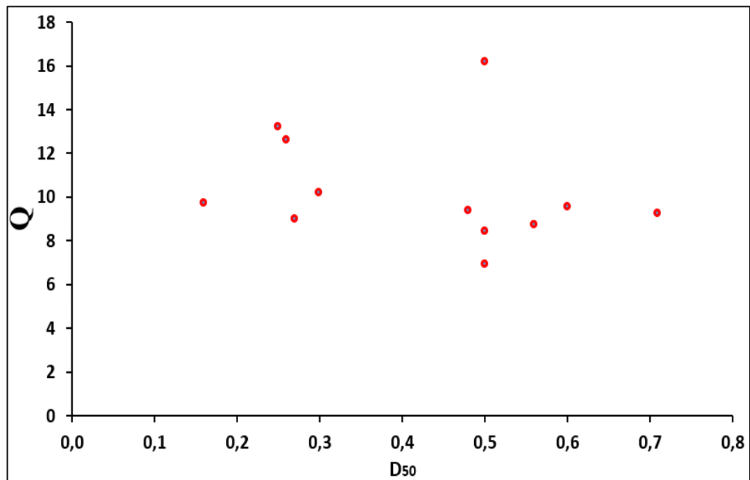
Figure 4.25. D_{50} - Q relationship.
