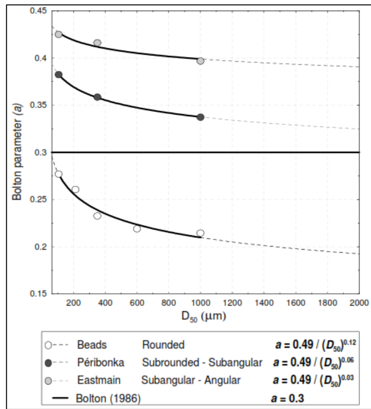
Figure 2.16. Variance of Bolton’s ‘ a ’ parameter with median grain size ( D_{50} ) and angularity (Amirpour et al. , 2017).
