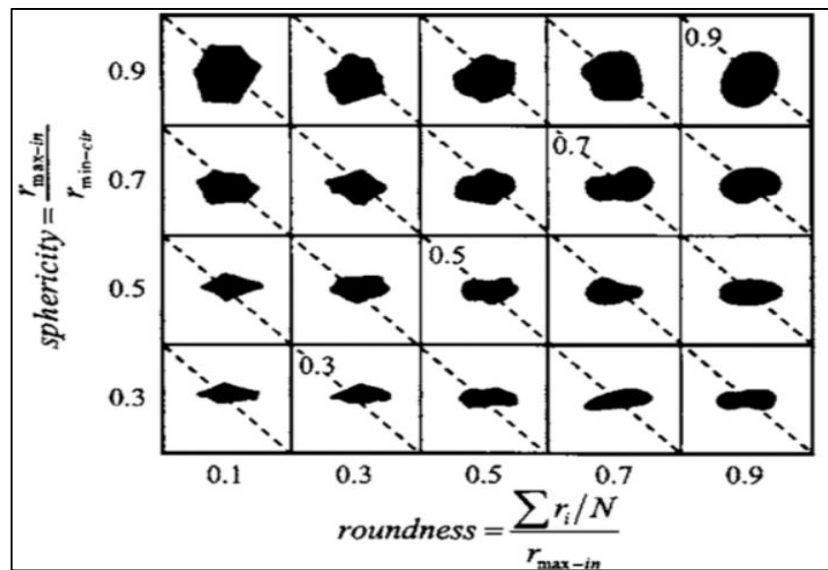
Figure 2.8. Sphericity and Roundness chart presented by Krumbein and Sloss (1963).
