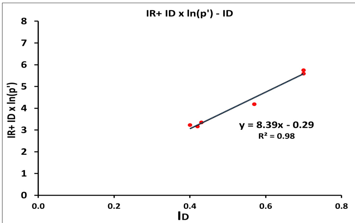
Figure 4.17. Determination of Q and R parameter from AC stress path of SP-S2.
