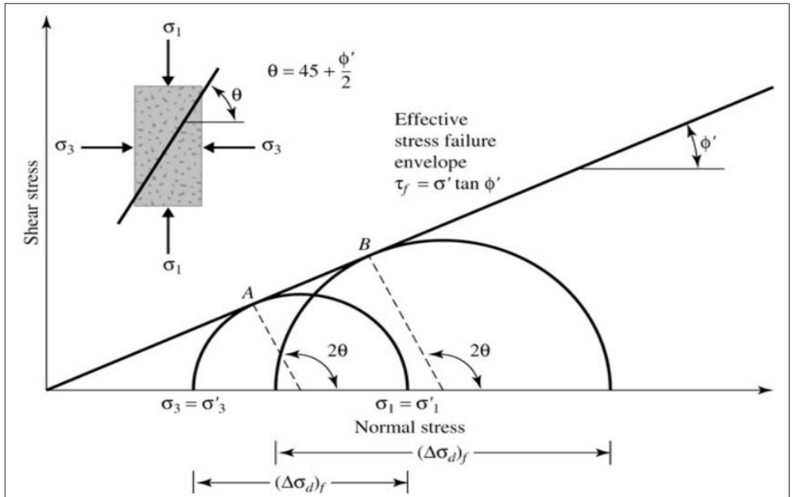
Figure 2.4. Mohr Circle at failure state.
