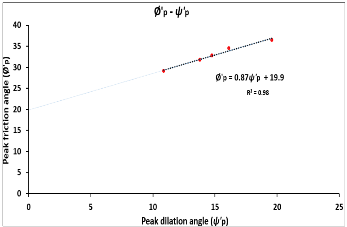
Figure 4.6. \psi'_p and \phi'_p relationship for LE stress path triaxial testing of GB.
