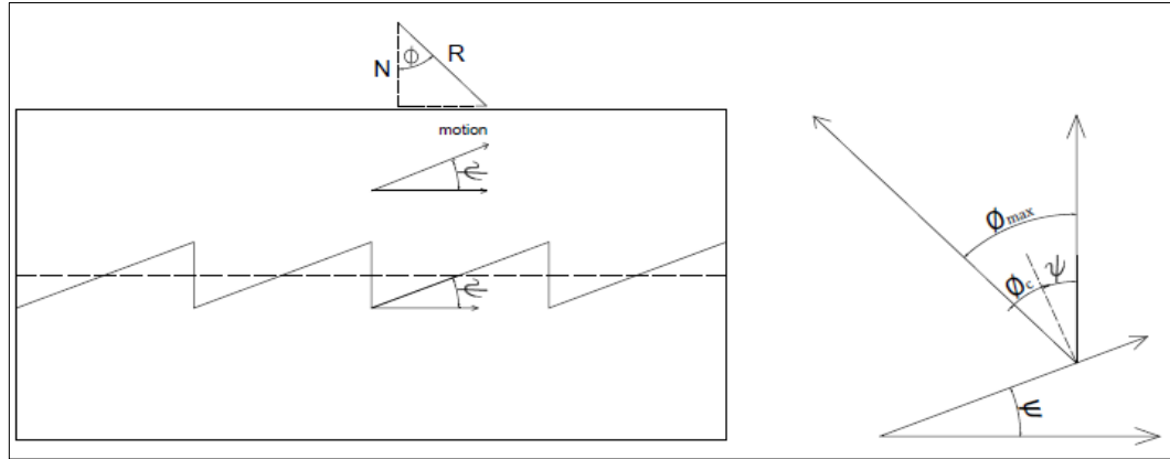
Figure 2.2. The saw blades model of dilatancy.
