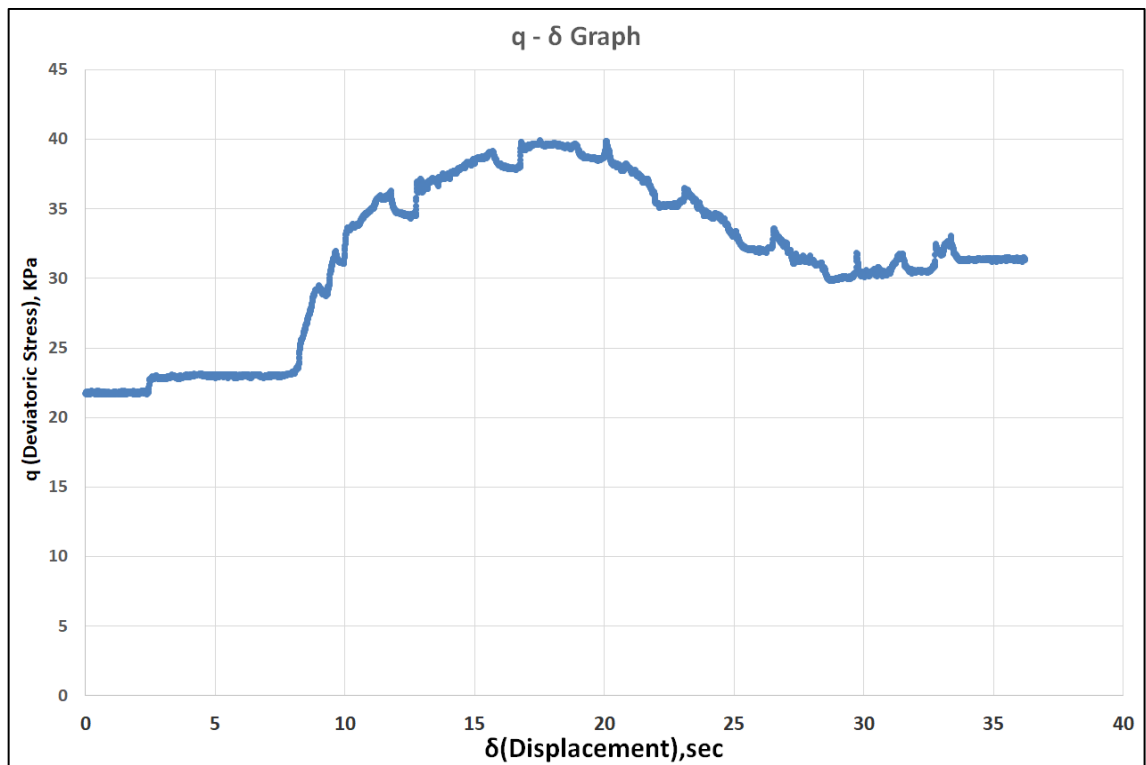
Figure 3.19. Plot of deviatoric stress – displacement graph during wall transition.
