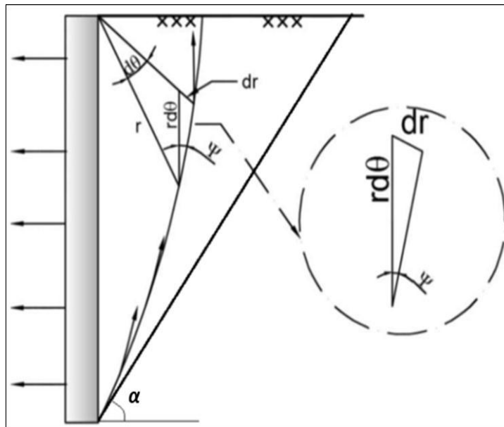
Figure 4.47. Influence of dilatancy on slip surface geometry.
