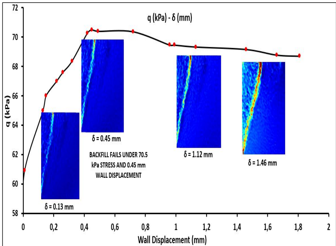
Figure 4.37. Deviatoric stress – wall displacement graph for a particular physical model experiment.
