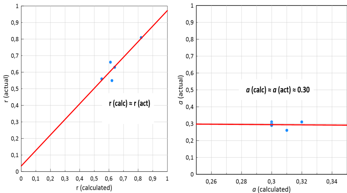
Figure 4.39. Comparison of calculated ' r ' and ' a ' stress-dilatancy coefficients from triaxial tests and actual ' r ' and ' a ' from physical model tests.
