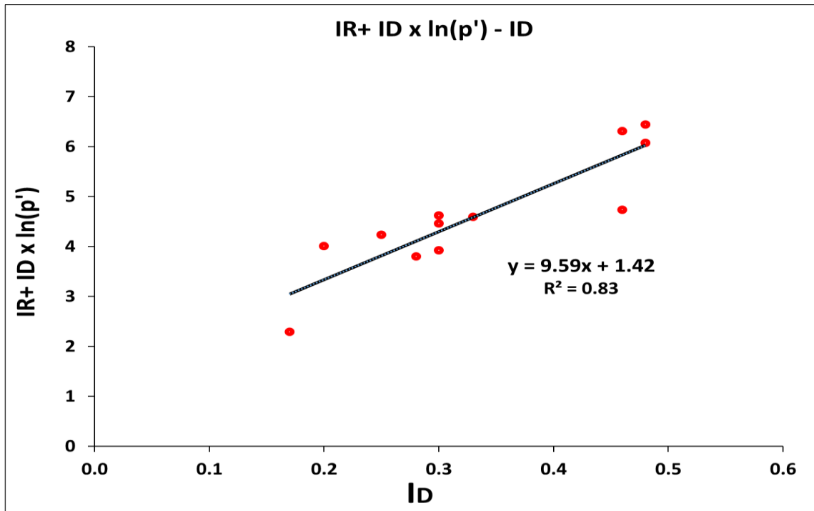
Figure 4.14. Determination of Q and R parameter from AC stress path of GB.
