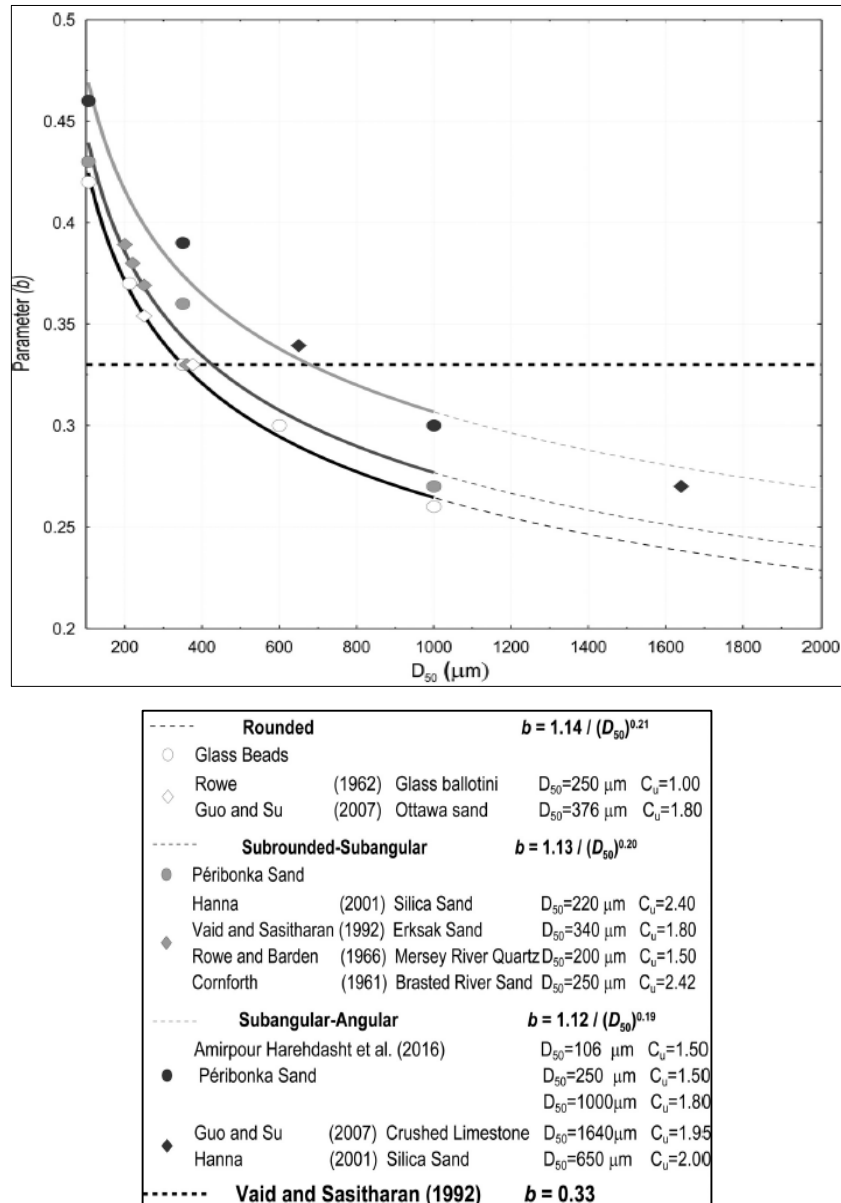
Figure 2.17. Variance of 'r' with median grain size and angularity (Amirpour et al. , 2017).
