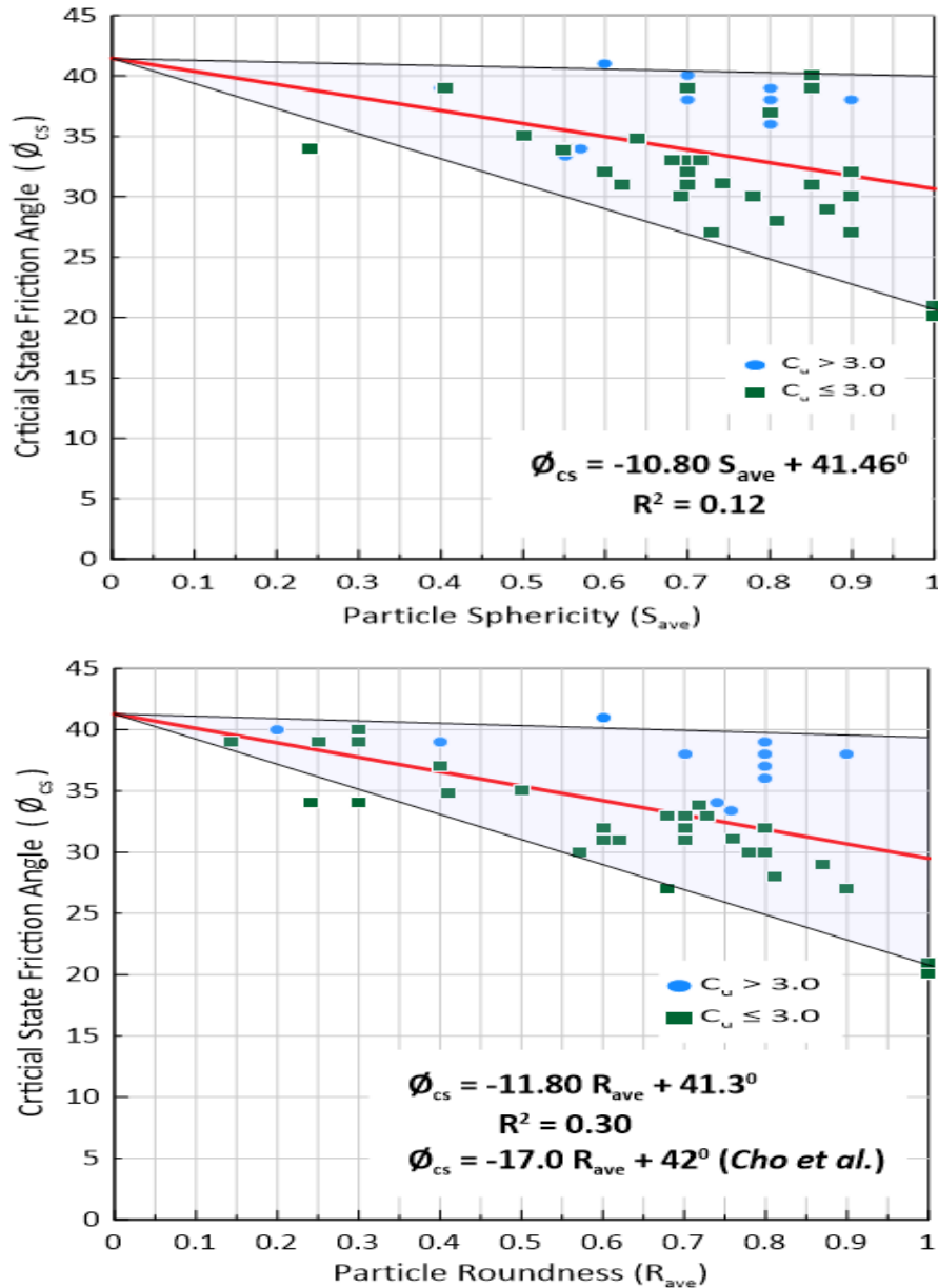
Figure 4.29. S_{ave} - \phi'_{cs} and R_{ave} - \phi'_{cs} relationship.
