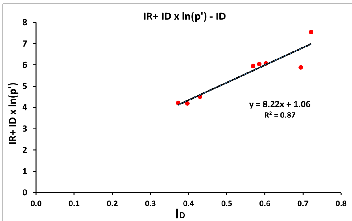
Figure 4.13. Determination of Q and R parameter from LE stress path of S3 sand.
