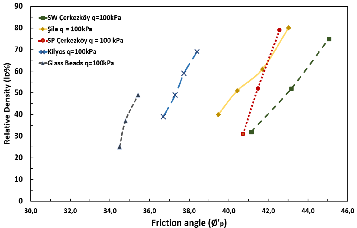
Figure 4.40. Relative density – Friction angle relationship at 100 kPa surcharge pressure for tested soils.
