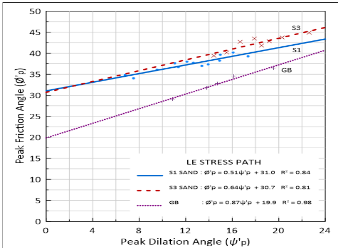
Figure 4.9. Summary of \psi'_p and \phi'_p relationships for AC - LE conditions.
