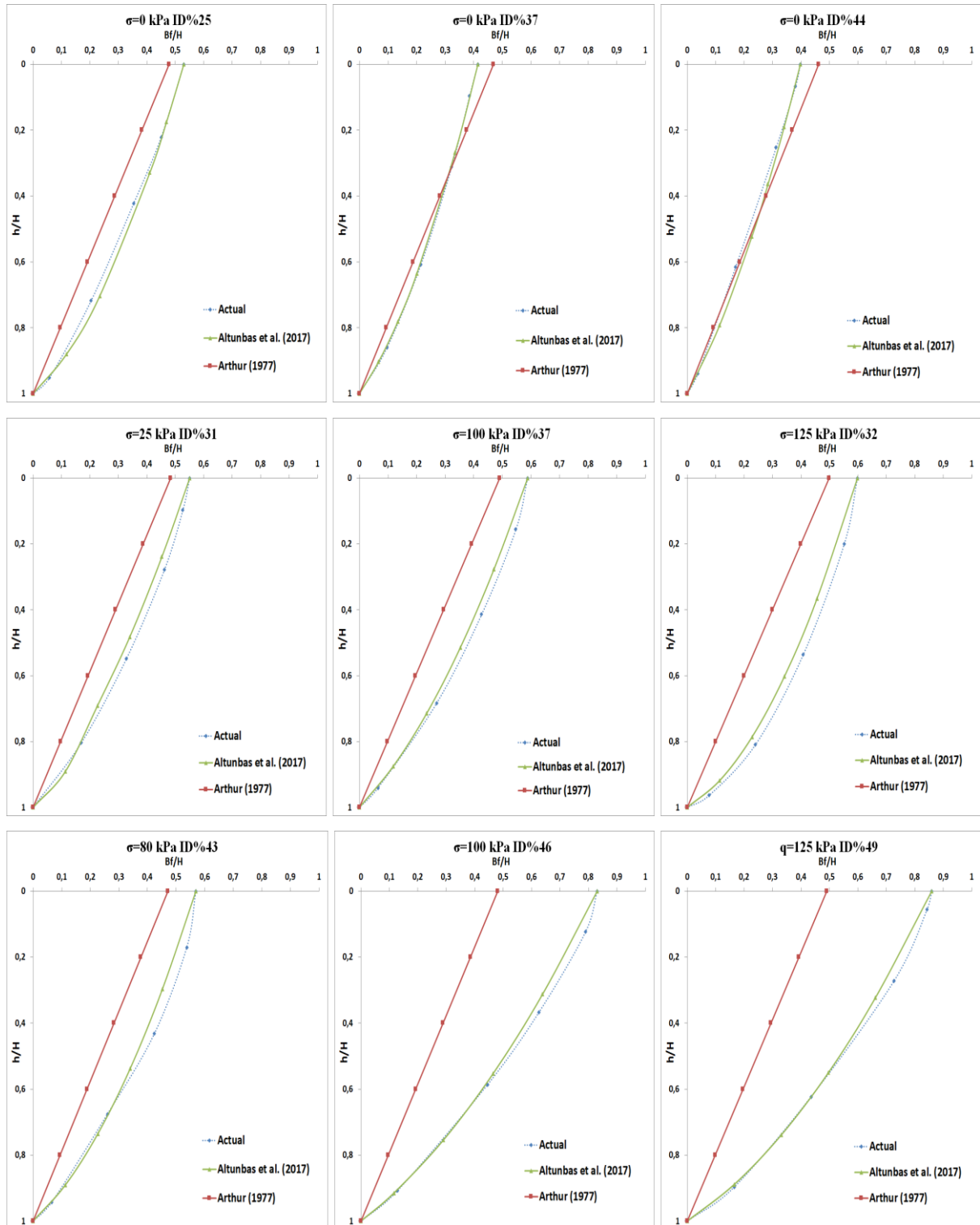
Figure 4.59. Comparison between plots of estimated and actual failure surfaces on normalized coordinate system for varying dilatancy values of physical model experiment data of GB.
