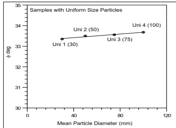
Figure 2.13. Influence of particle size on friction angle (Latha and Sitharam, 2008)
