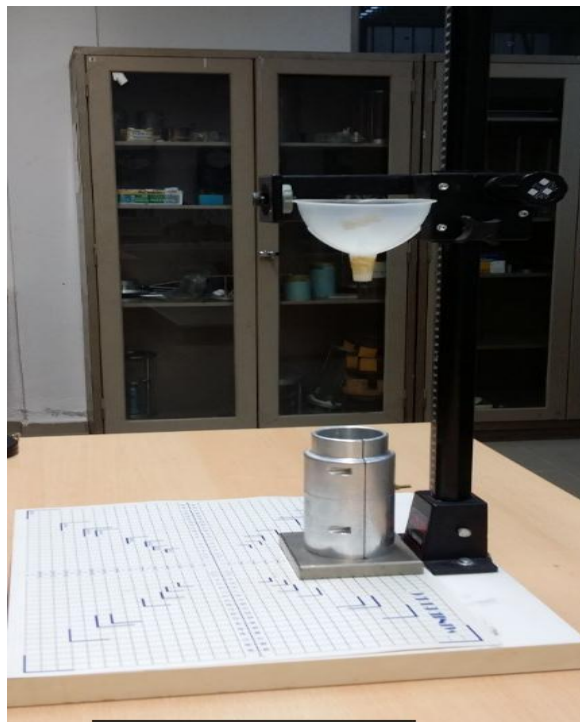
Figure 3.10. Equipment used in dry pluvation technique.
