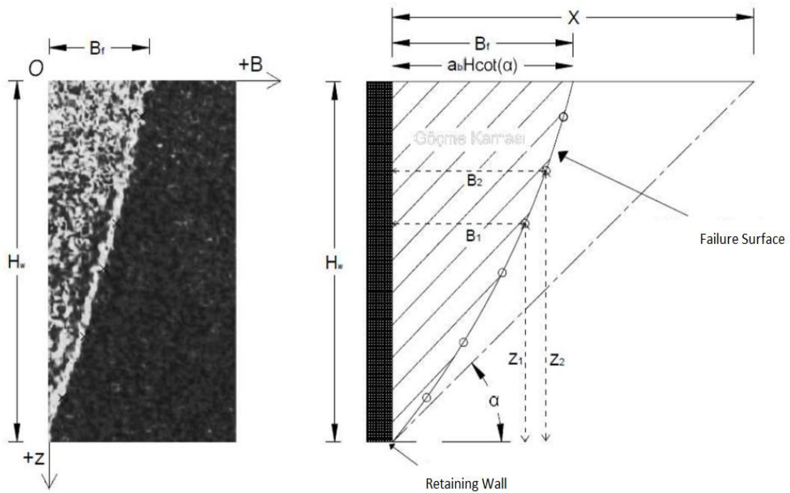
Figure 4.54. Geometric properties of failure surface geometry.
