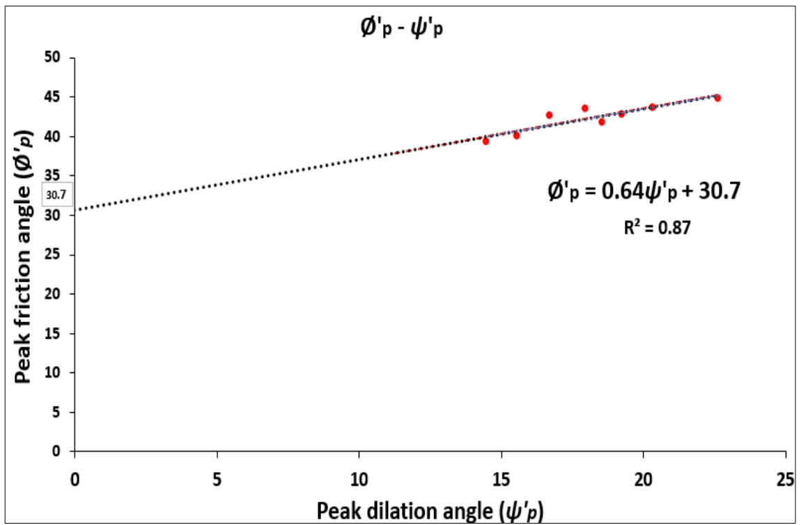
Figure 4.4. \psi'_p and \phi'_p relationship for LE stress path triaxial testing of S3 sand.
