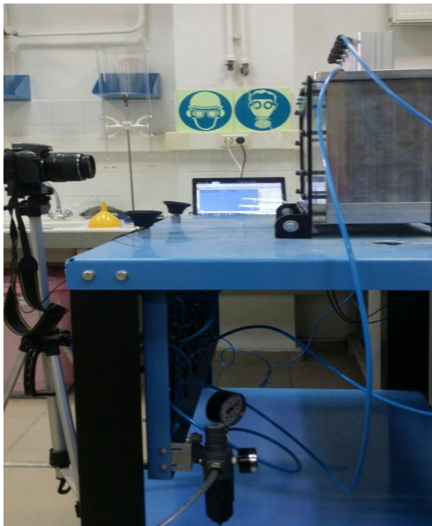
Figure 3.16. View of measure gauge and air hose connecting to pneumatic pistons.
