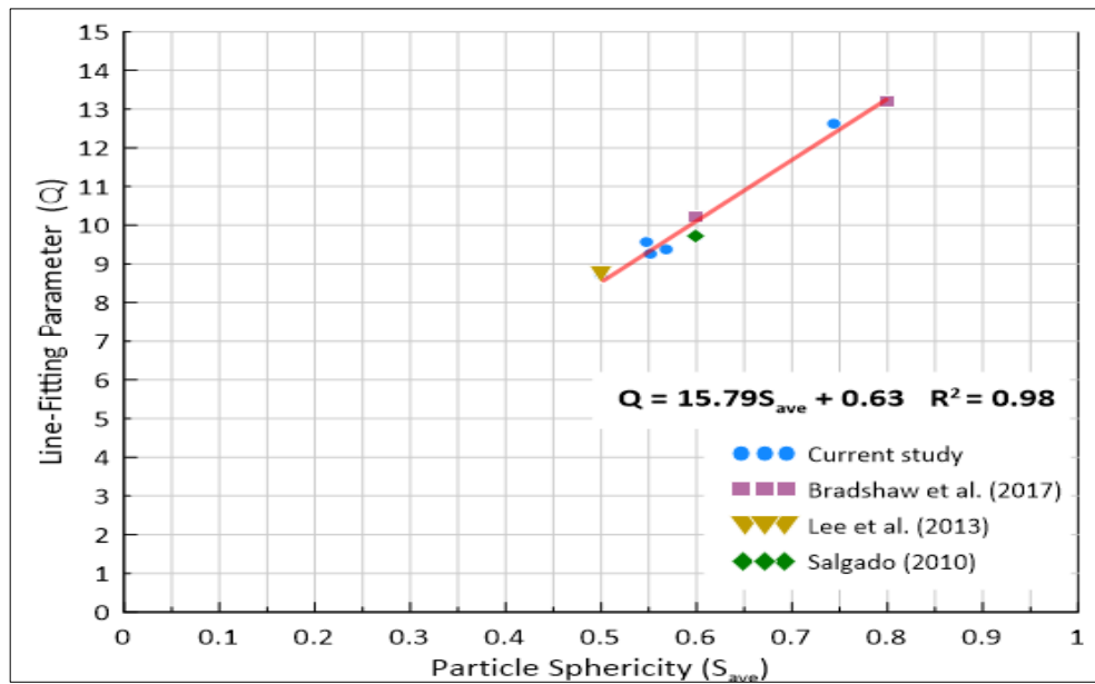
Figure 4.28. S_{ave} – Q relationship provided that R = 1 .
