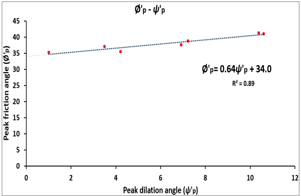
Figure 4.7. \psi'_p and \phi'_p relationship for AC stress path triaxial tests of SW-S2.
