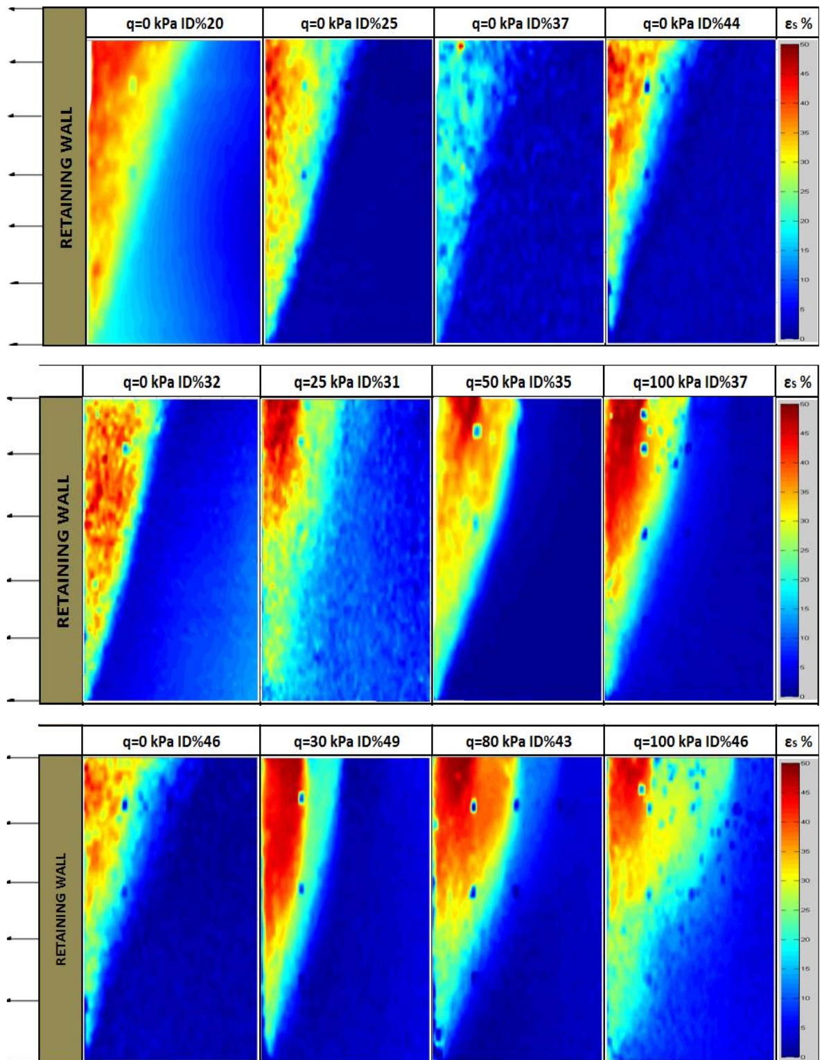
Figure 4.35. PIV analysis results for SP-S2.
