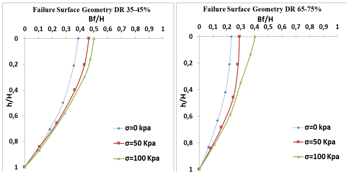
Figure 4.45. Active failure surface geometries of S1 at varying surcharge and densities.
