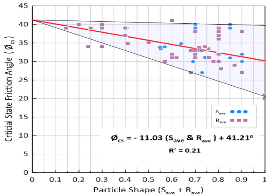
Figure 4.30. Grain shape – \phi_{cs} relationship.
