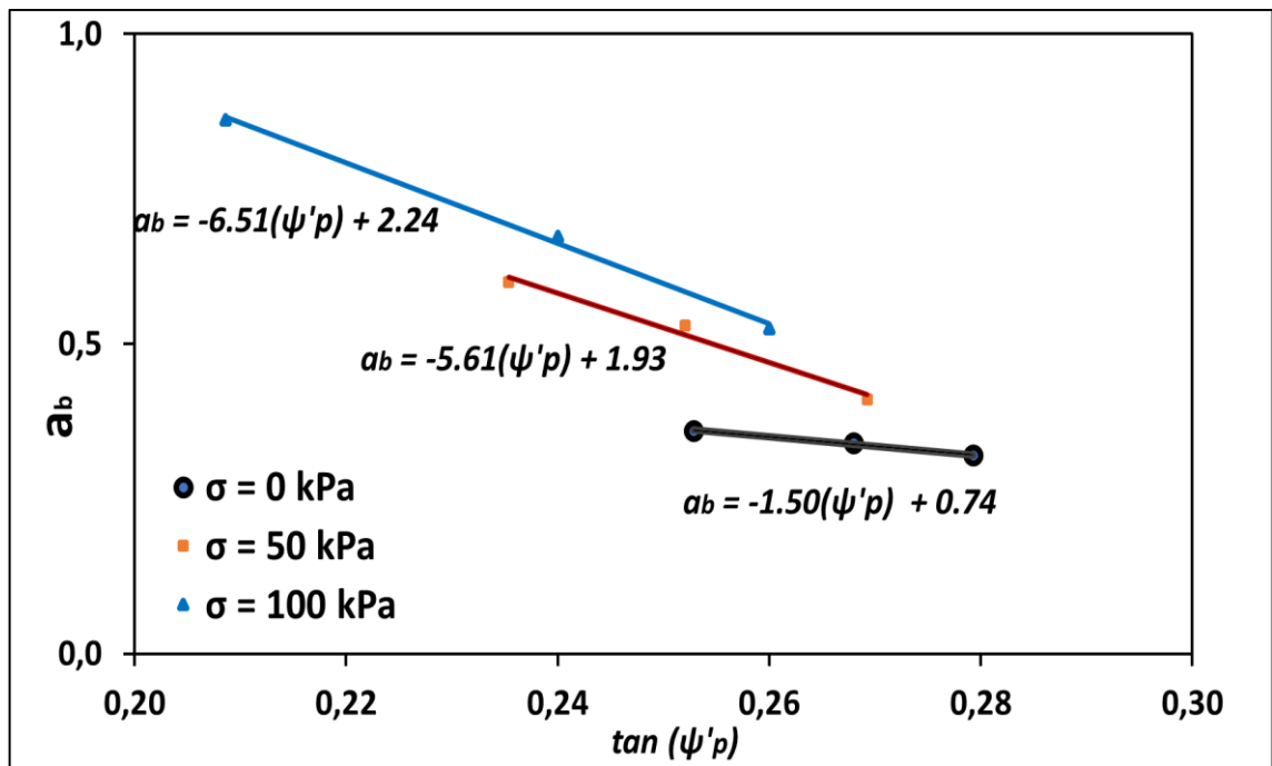
Figure 4.52. Influence of dilatancy on experimentally measured values of a_b for S2-SW.
