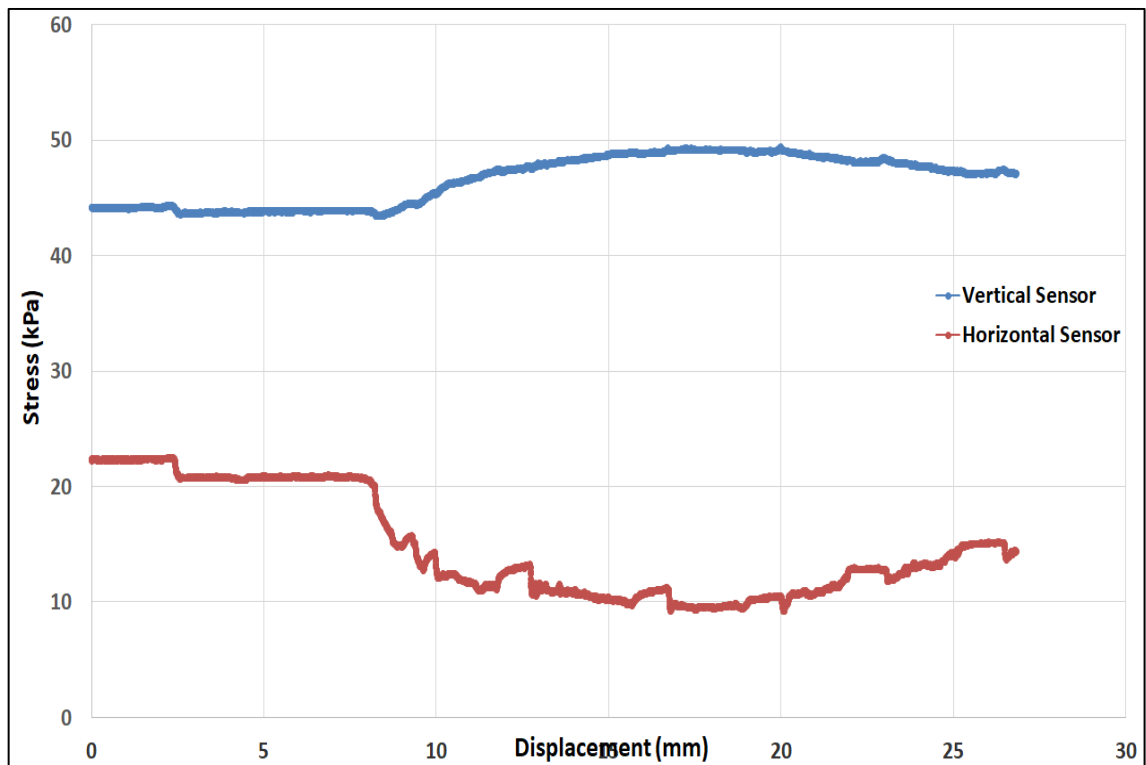
Figure 3.18. Plot of vertical and horizontal sensor readings through wall transition.
