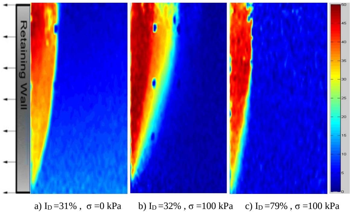
Figure 3.23. Shear strain distribution generated by PIV behind retaining of S2 sand.
