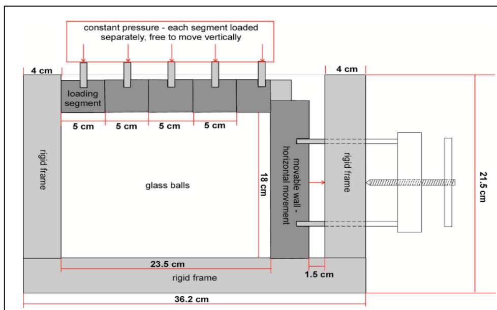
Figure 2.22. Physical model apparatus designed by Lesniewska and Wood (2009).
