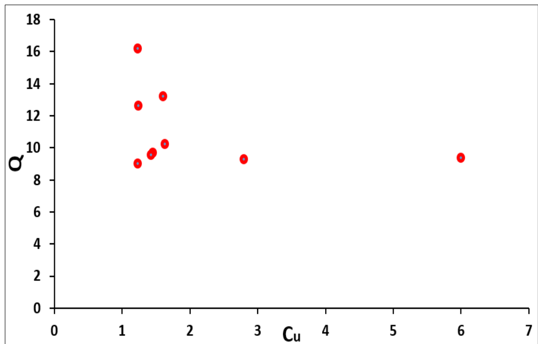
Figure 4.20. C_u - Q relationship of tested soils together with literature data.
