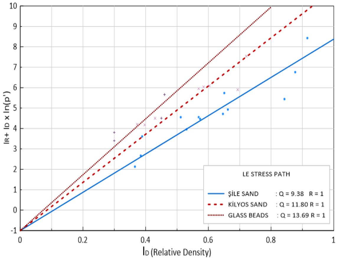
Figure 4.18. Evaluation of line fitting Q parameter when R = 1 for AC-LE conditions.
