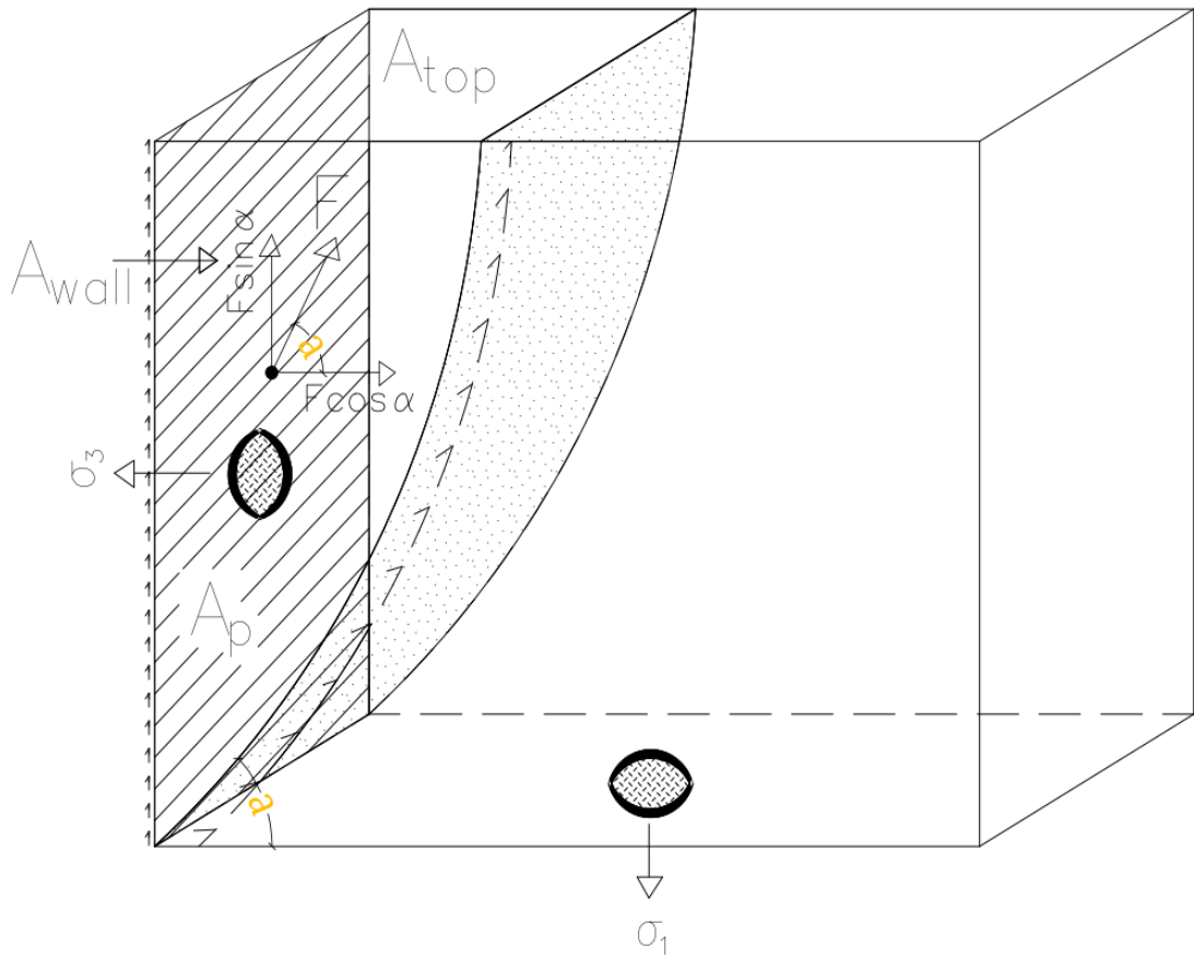
Figure 4.38. Visualization of friction forces between shear wedge and model frame.
