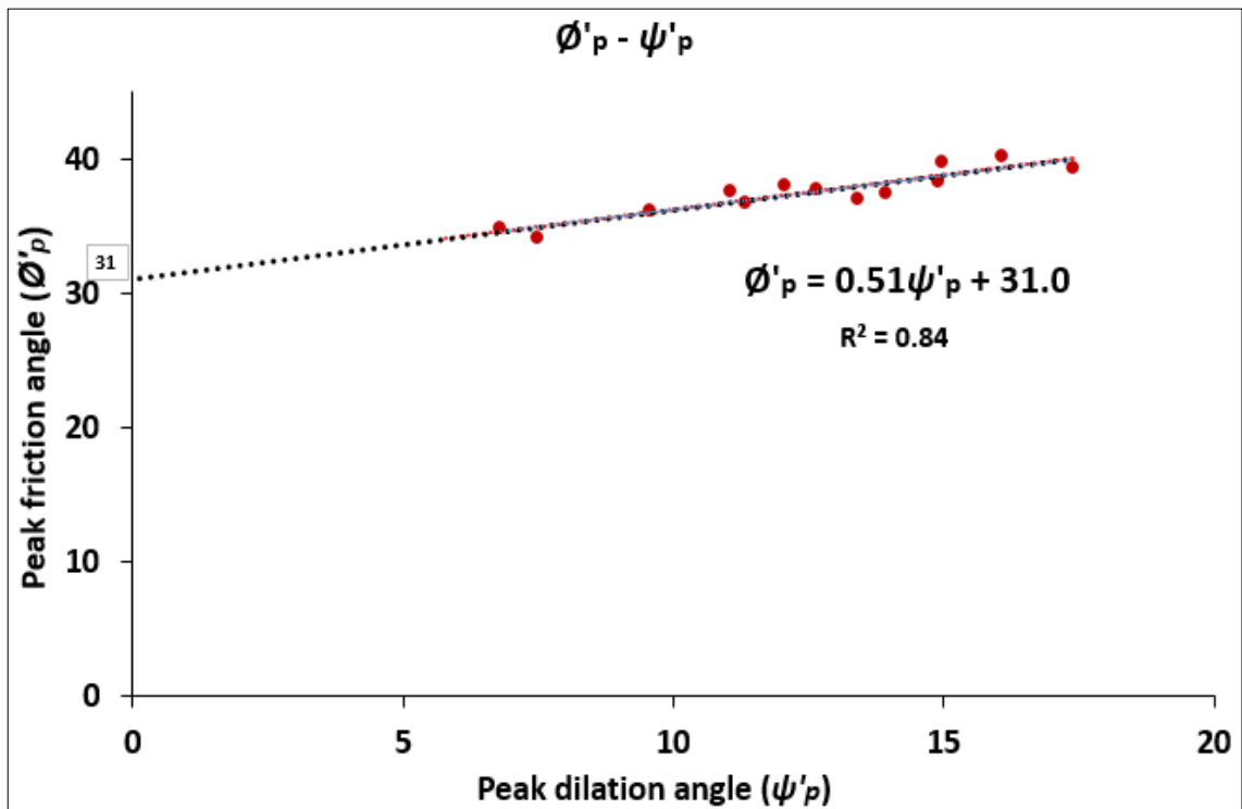
Figure 4.2. \psi'_p and \phi'_p relationship for LE stress path triaxial testing of S1 sand.
