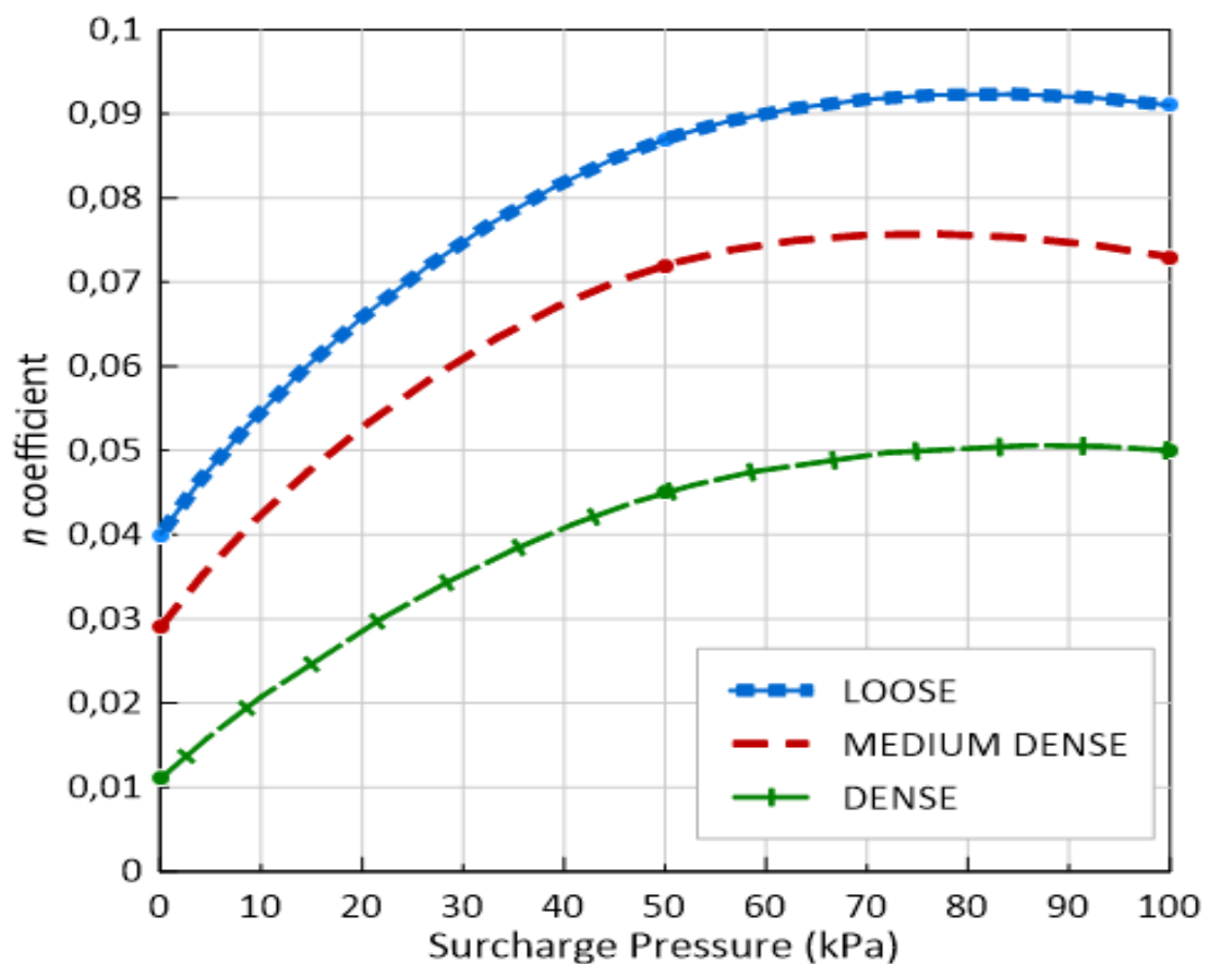
Figure 4.62. Change of “ n ” coefficient with respect to surcharge pressure.
