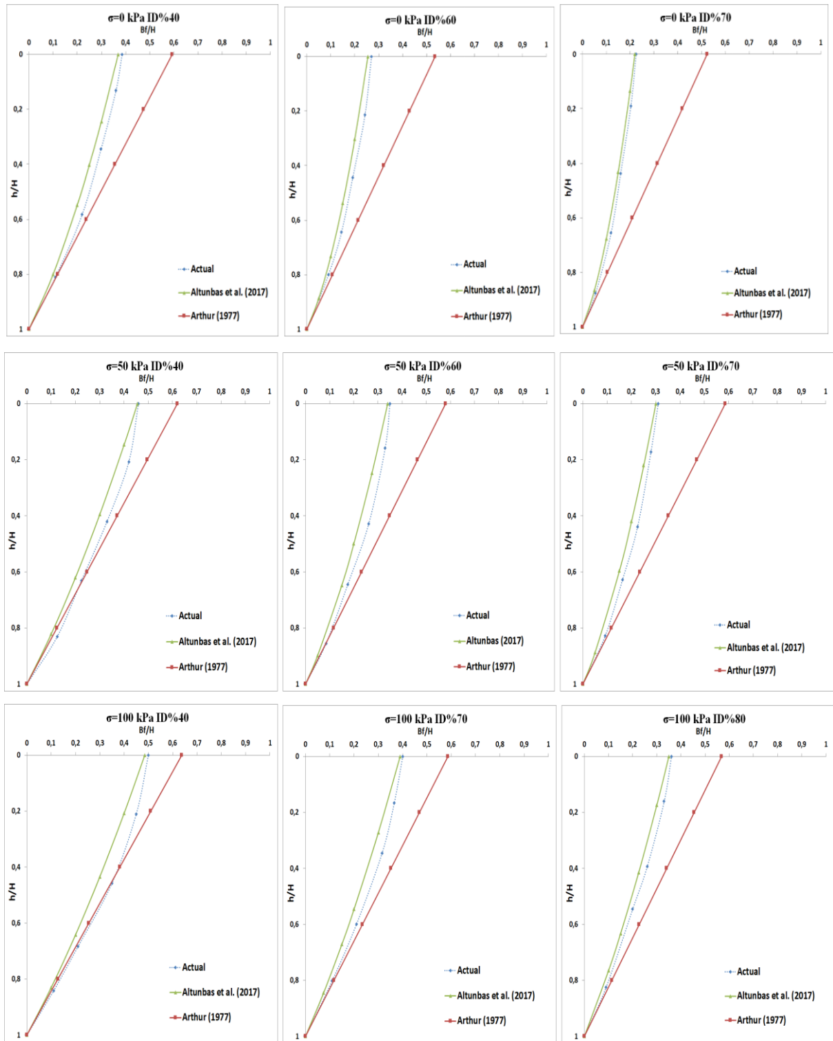
Figure 4.56. Comparison between plots of estimated and actual failure surfaces on normalized coordinate system for varying dilatancy values of physical model experiment data of S1 Sand.
