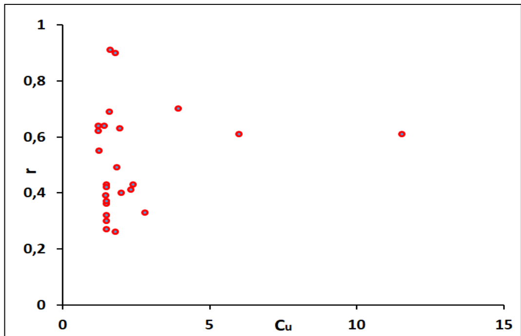
Figure 4.19. C_u - r relationship of tested soils together with literature data.
