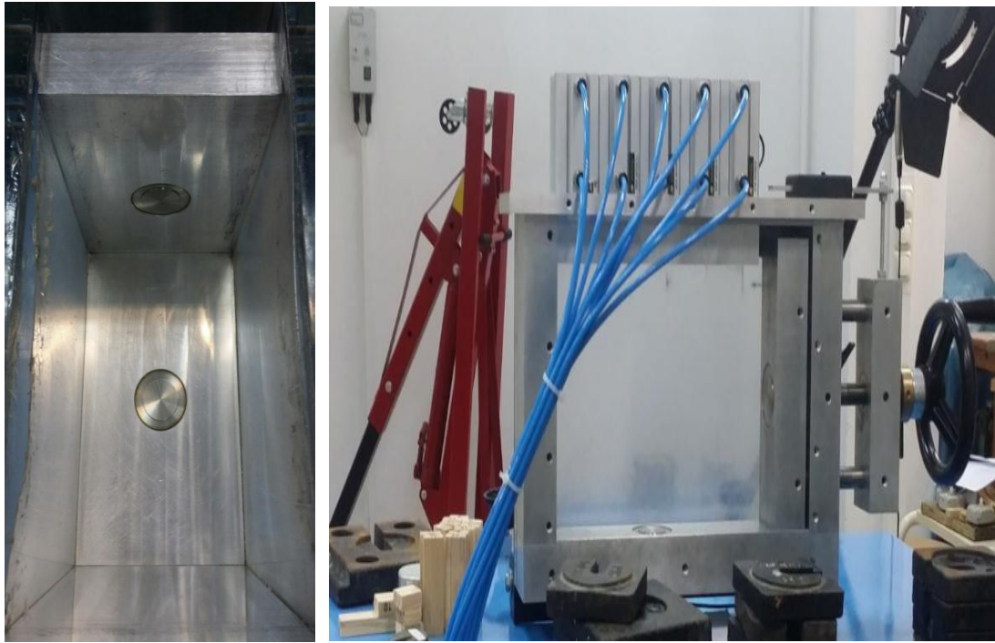
Figure 3.17. View of vertical and horizontal sensors in the model box.
