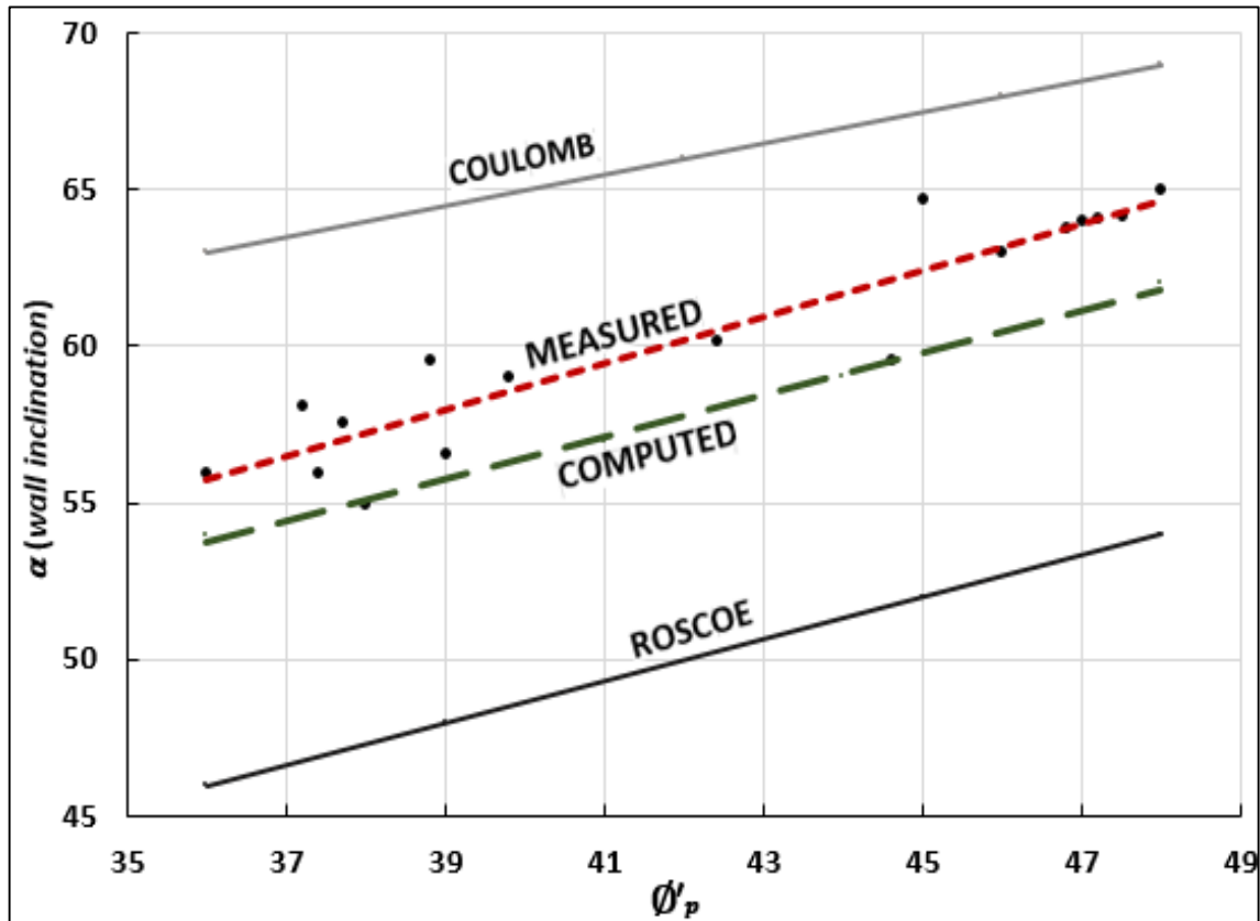
Figure 2.20. Measured vs. computed shear band inclination (Vardoulakis, 1980).
