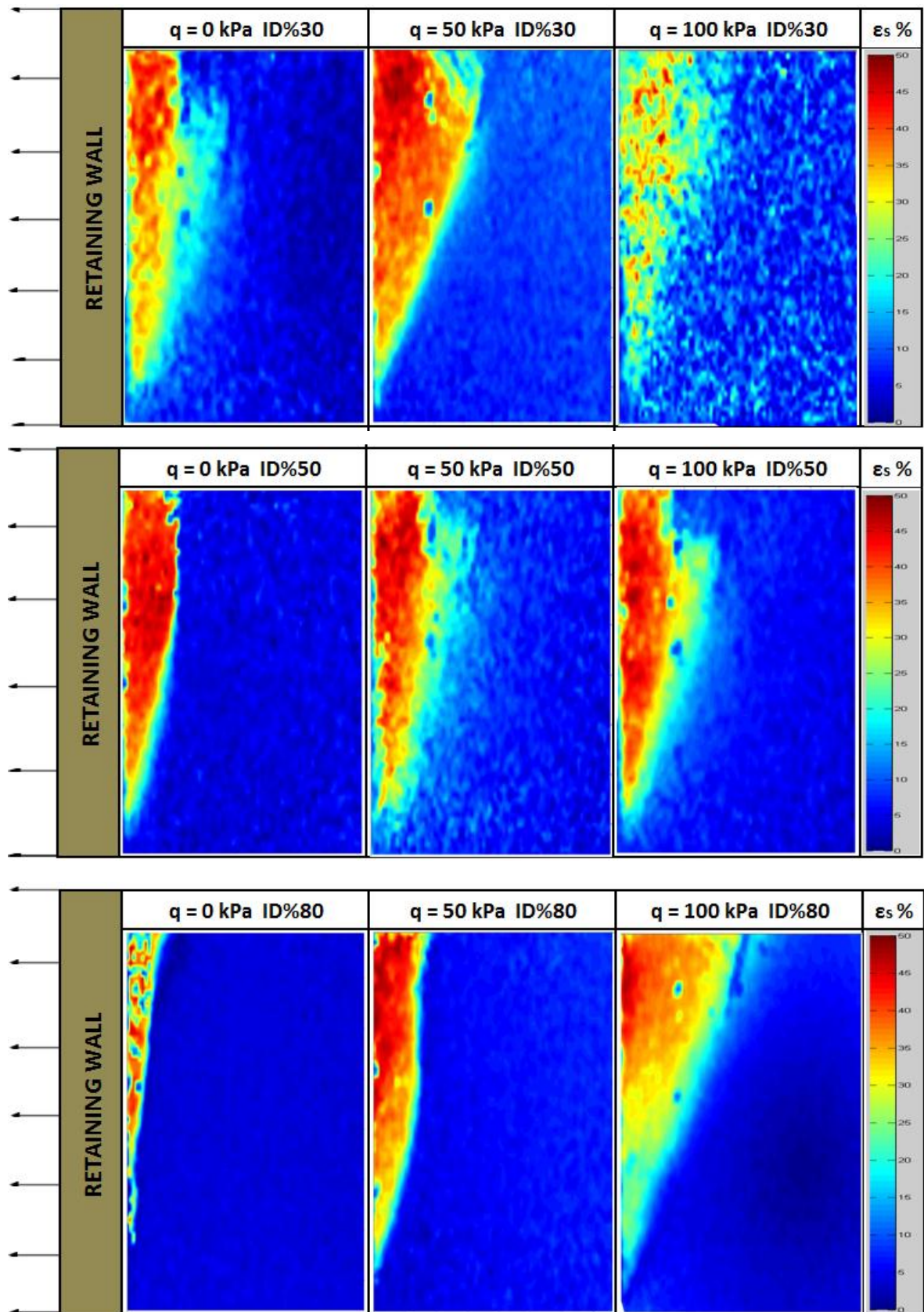
Figure 4.34. PIV analysis results for SW-S2.
