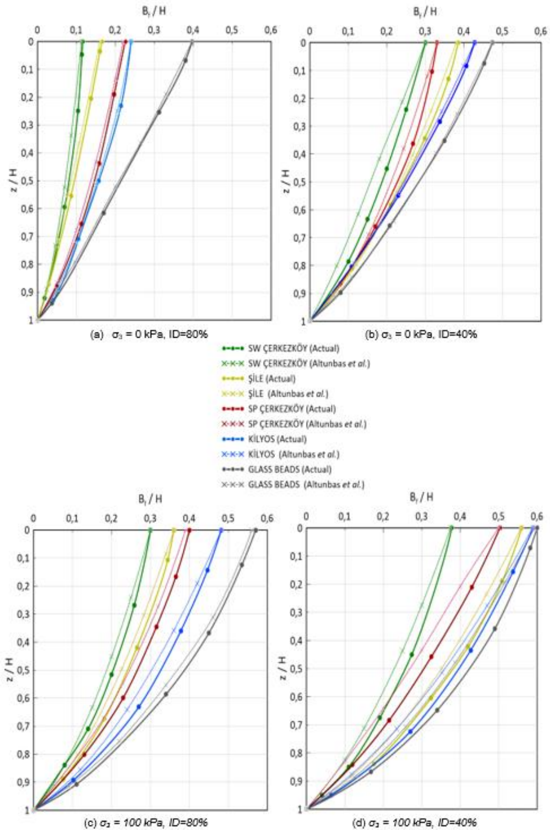
Figure 4.60. Comparison of actual failure surface geometries with empirical method (Altunbas et al. , 2017) of tested soils.
