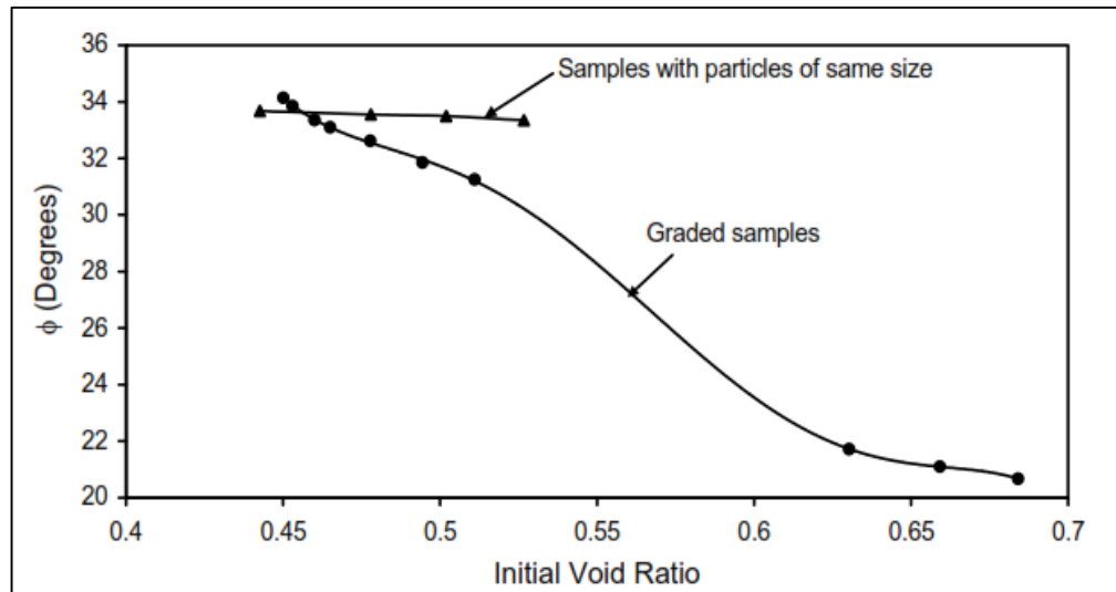
Figure 2.15. Variation of friction angle with void ratio (Latha and Sitharam, 2008).
