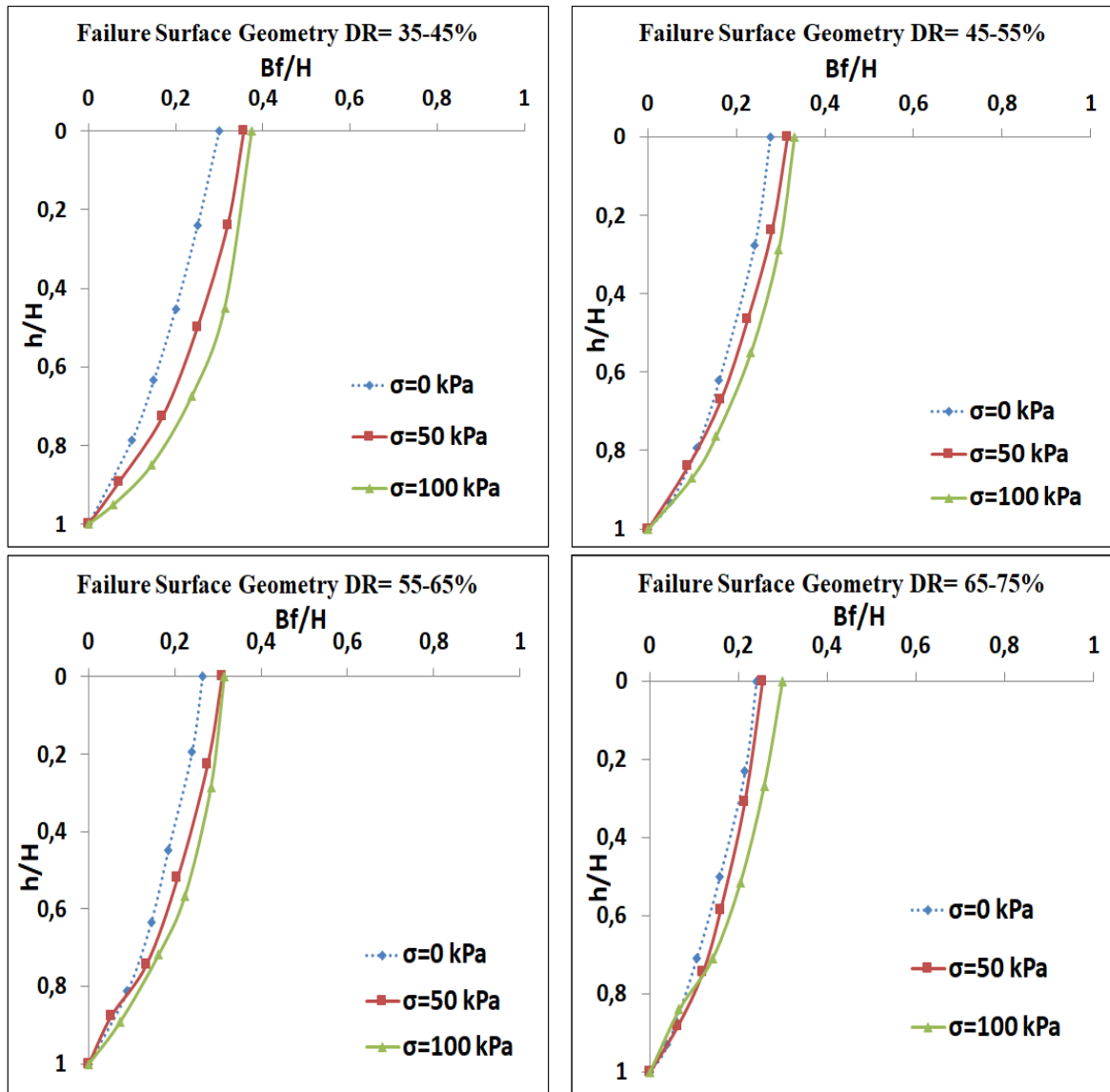
Figure 4.46. Active failure surface geometries of S3 at varying surcharge and densities.
