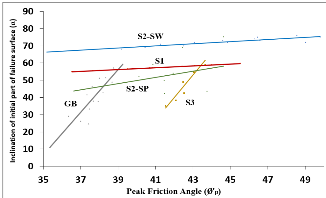
Figure 4.49. Relationship between inclination of initial part of the failure surface and peak friction angle for tested granular backfills.
