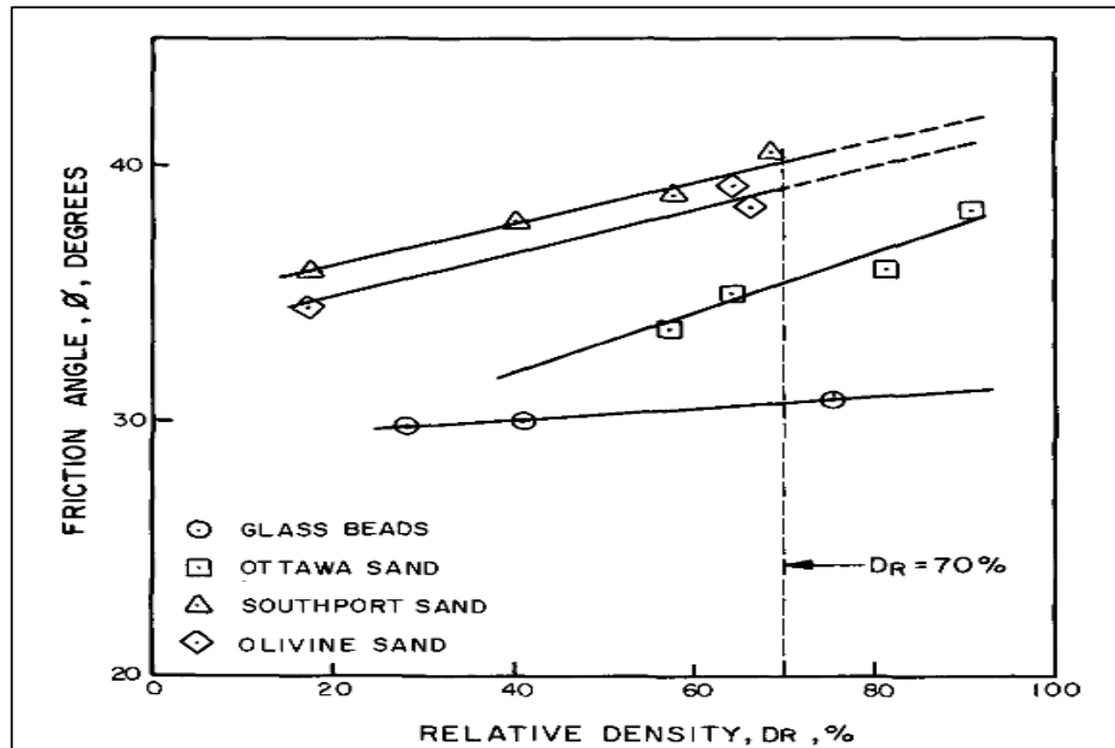
Figure 2.9. Effect of particle shape on angle of internal friction (Holubec and Appolonia, 1973).
