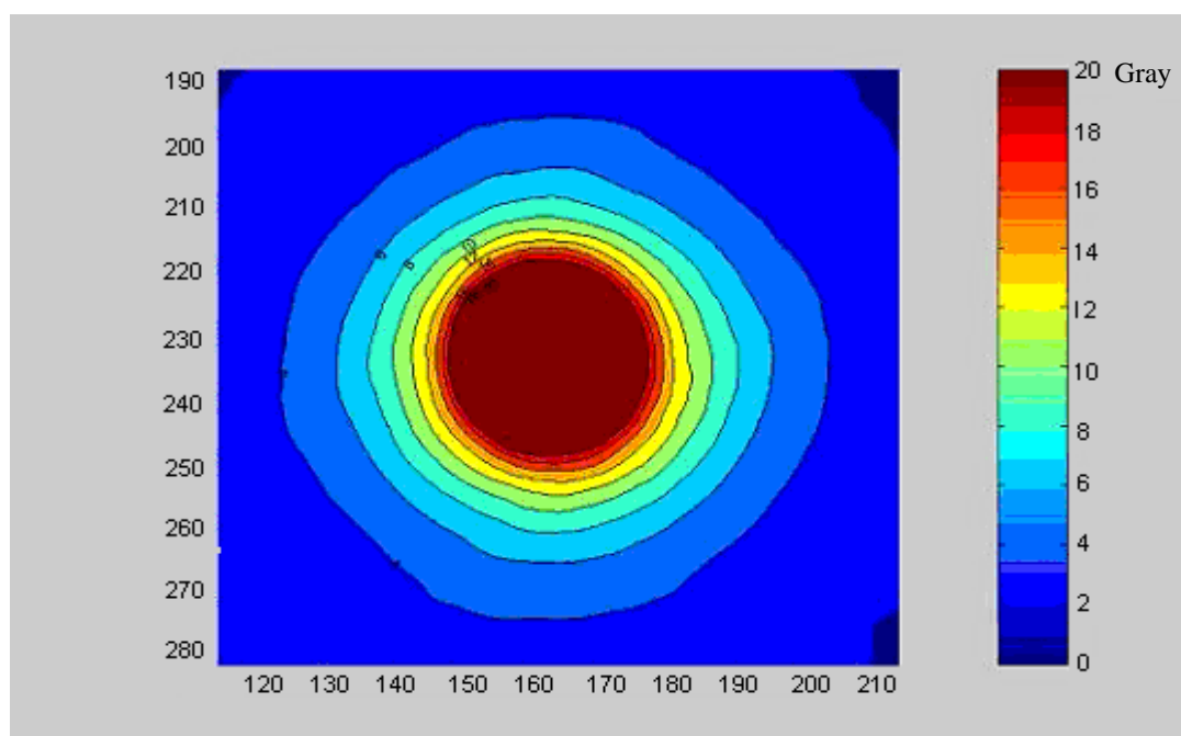
Figure 6.5: Homogeneous phantom dose distribution (Gy) in the axial plane, for slice Z=105 in stereotactic frame coordinates.
