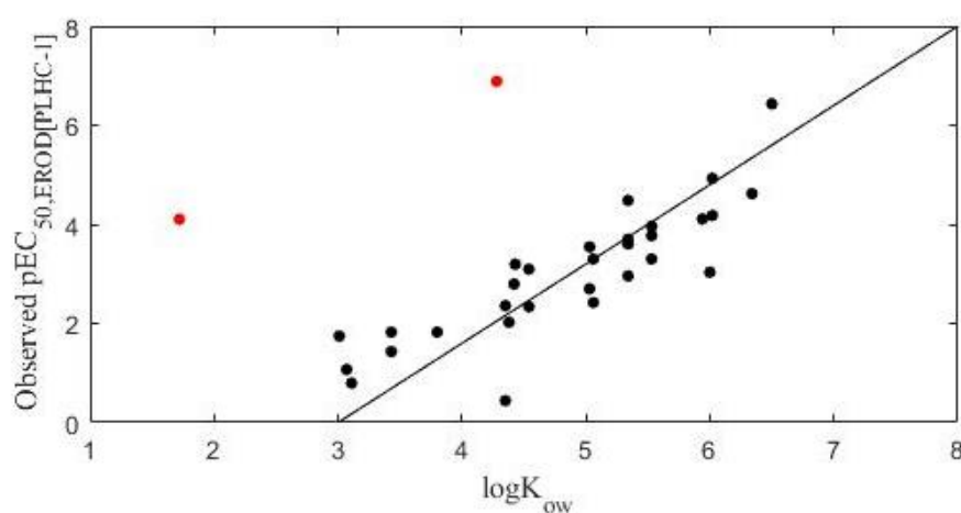
Figure 4.4. Plot of observed \text{pEC}_{50,\text{EROD}[\text{PLHC-1}]} values versus \log K_{\text{ow}} values.
