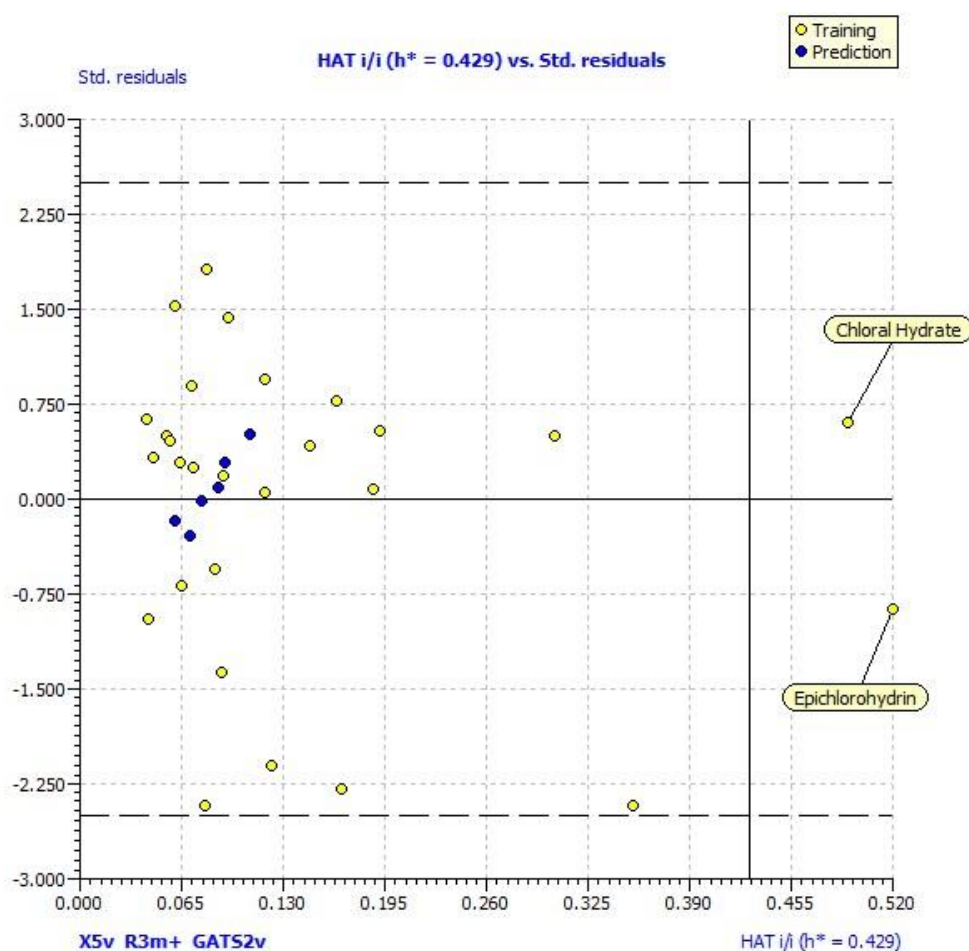
Figure 4.18. Williams plot of pEC_{50,NR[FHM]} model.
