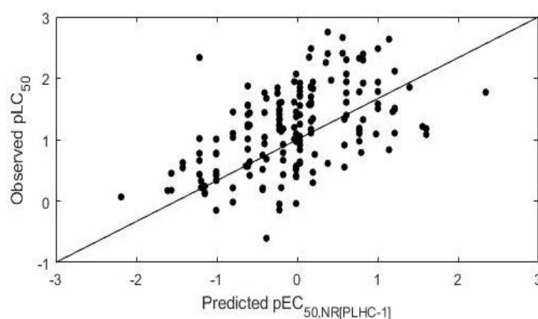
Figure 4.11. Plot of observed pLC_{50} versus predicted pEC_{50,NR[PLHC-1]} values by Eq. 4.3.
