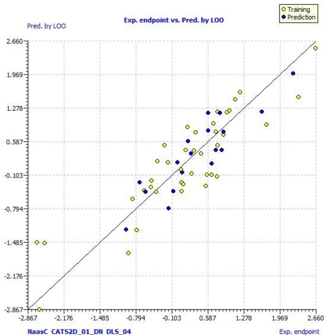
Figure 4.7. Plot of predicted \text{pEC}_{50,\text{NR}[\text{PLHC-1}]} values from Eq. 4.3 versus experimental \text{pEC}_{50,\text{NR}[\text{PLHC-1}]} values.
