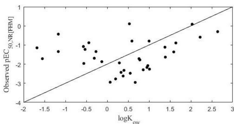
Figure 4.20. Plot of observed \text{pEC}_{50,\text{NR[FHM]}} values versus \log K_{\text{ow}} values.
