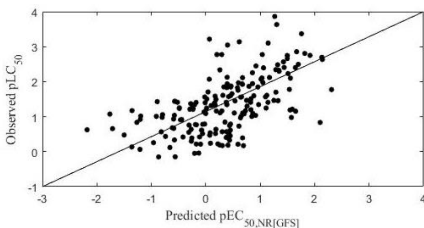
Figure 4.16. Plot of observed pLC_{50} versus predicted pEC_{50,NR[GFS]} values by Eq. 4.7.
