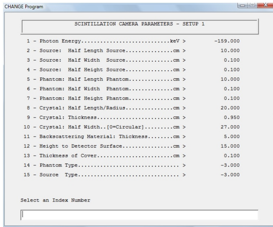
Figure A.1 Interface of the CHANGE program [47].
