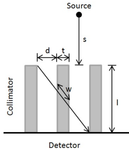
Figure 2.4 Cross-section of a parallel-hole collimator.
