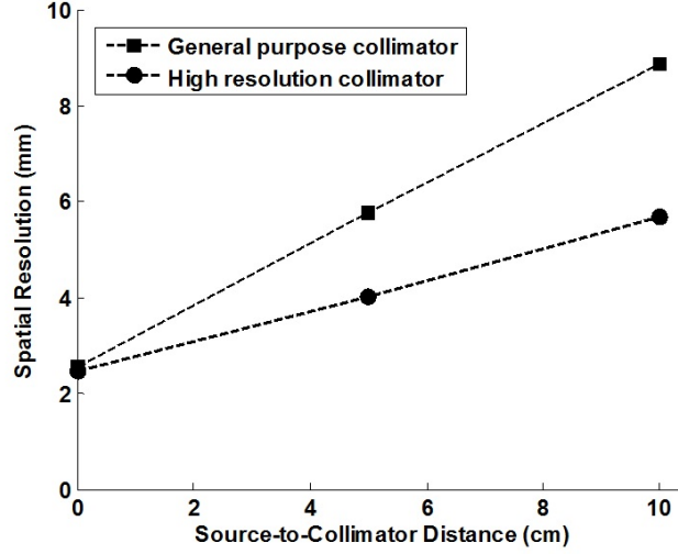
Figure 2.5 Spatial resolution vs. source-to-collimator distance for the camera.
