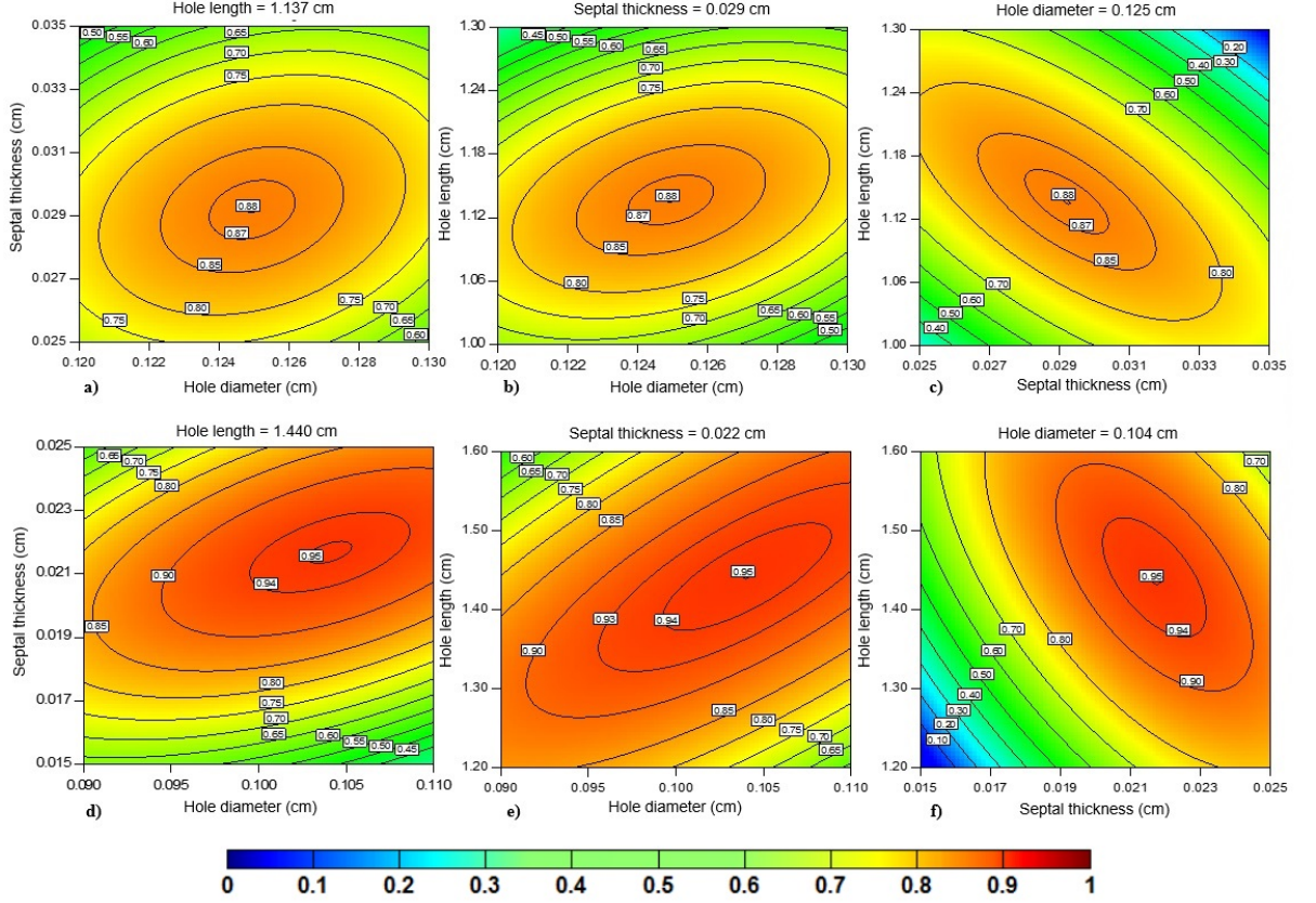
Figure 2.7 Iso-desirability contours. a) , d) Hole diameter vs. septal thickness, b) , e) hole diameter vs. hole length, and c) , f) septal thickness vs. hole length, for CNR models developed for lesions lying at a depth of 3 cm and 5 cm, respectively. The third parameter was kept at its optimal level for each plot ( a ) hole length=1.137 cm, b) septal thickness=0.029 cm, c) hole diameter=0.125 cm), d) hole length=1.440 cm, e) septal thickness=0.022 cm, f) hole diameter=0.104 cm).
