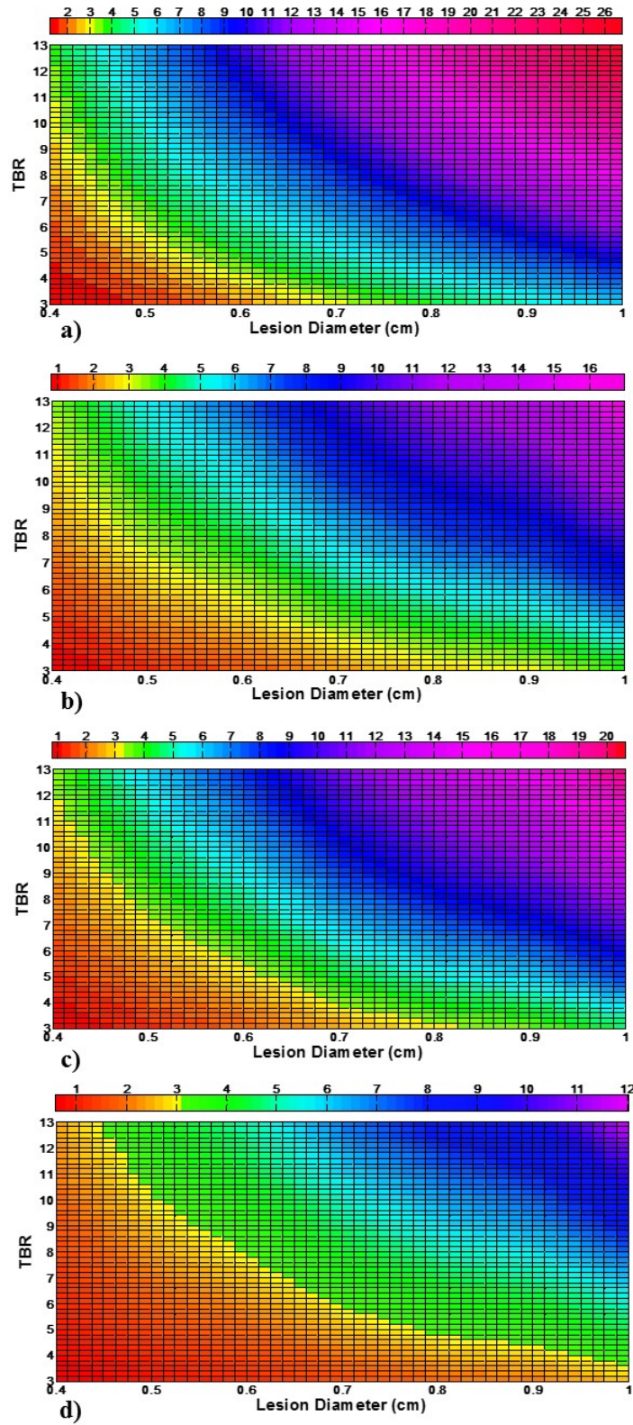
Figure 2.8 Iso-CNR plots with respect to TBR and lesion diameter for a lesion depth of 3 cm obtained with a) the optimum (optimized for 3 cm SCD) collimator, b) collimator D, c) collimator GP and d) collimator HR.
