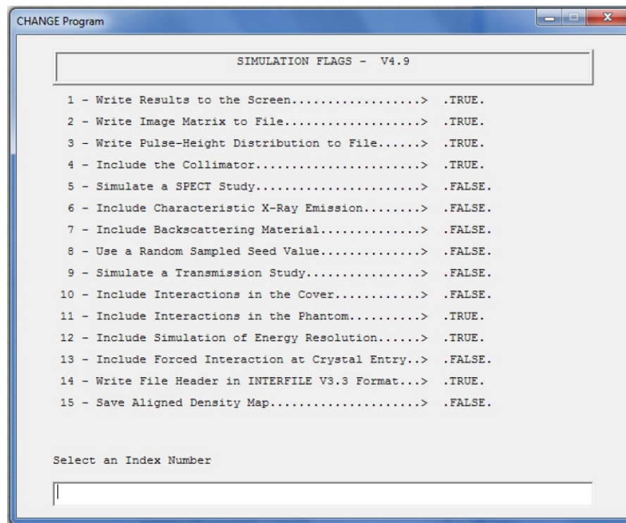
Figure A.2 Simulation flags within the CHANGE program [47].
