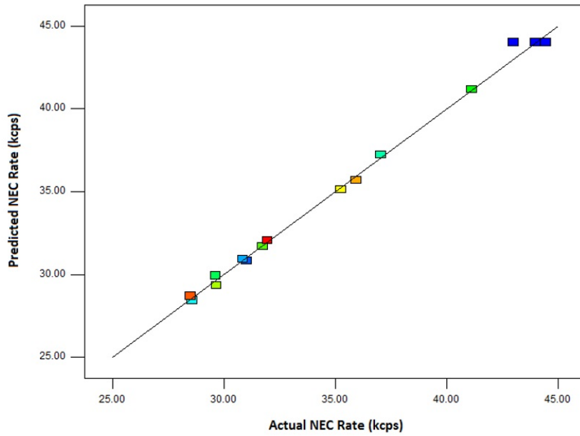
Figure 3.6 Predicted vs. simulated NECR.
