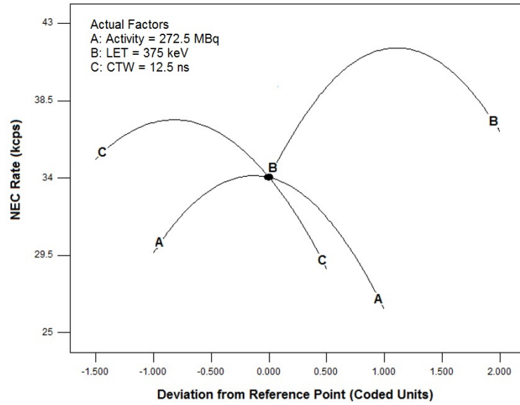
Figure 3.7 Perturbation plot of scanning parameters for NECR. At the point of intersection, the scanner parameters are kept at their default values (375 keV and 12.5 ns) and the activity is taken as 272.5 MBq. Individual effect and combined effects of parameters can be seen moving along the curves.
