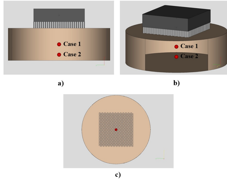
Figure 2.3 a) Side view, b) Oblique view and c) Bottom view of the camera and the breast phantom for a craniocaudal projection of the breast. Red dots in a) and b) represent the lesions and their locations. Case 1 and Case 2 stands for 3 cm depth optimization case and 5 cm depth optimization case, respectively.
