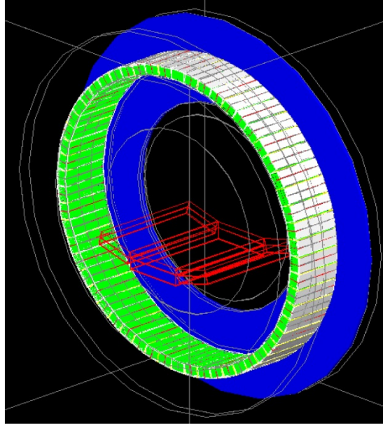
Figure 3.3 Geometry of GE Discovery LS PET module modeled using GATE simulation platform.
