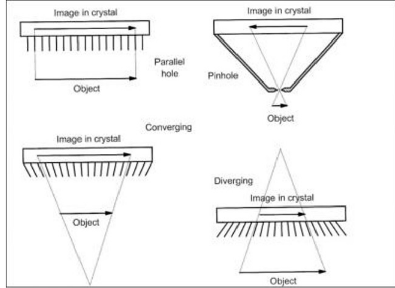
Figure 2.1 Collimator types according to their geometries [14].
