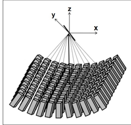
Figure 2.2 Geometry of a fan-beam collimator [15].
