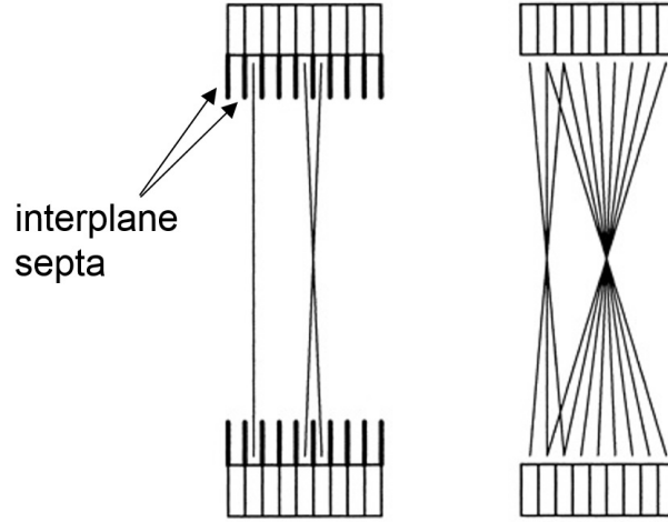
Figure 3.2 a) 2D and b) 3D data acquisition in PET [84].
