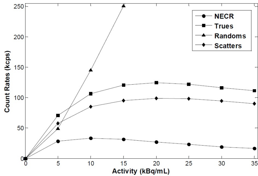
Figure 3.4 Simulated 3D count rate response of GE Discovery LS PET module.
