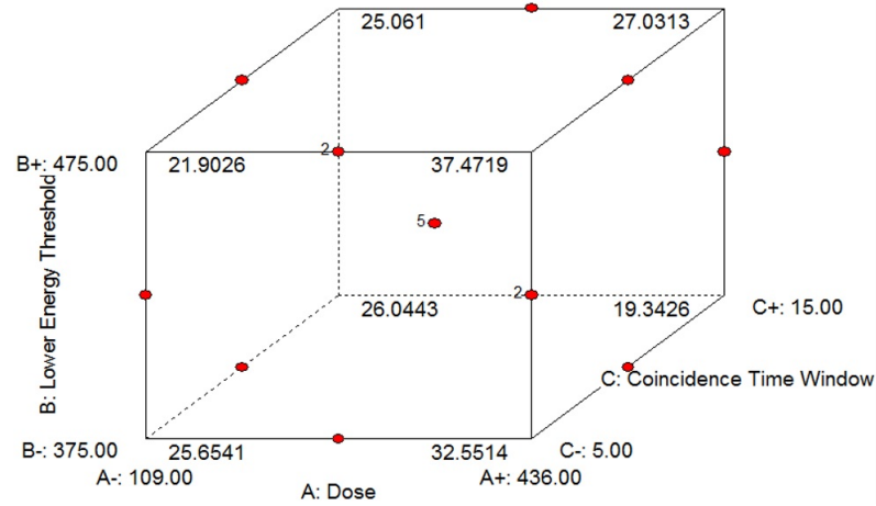
Figure 3.5 Box-Behnken design points shown in the 3D design space.
