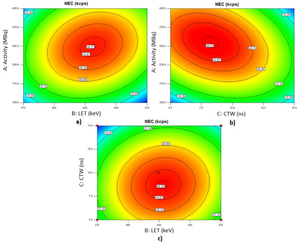
Figure 3.8 Response surface plot of NECR with respect to scanning parameters. a) Activity and lower energy threshold, b) activity and coincidence time window and c) lower energy threshold vs. coincidence time window.
