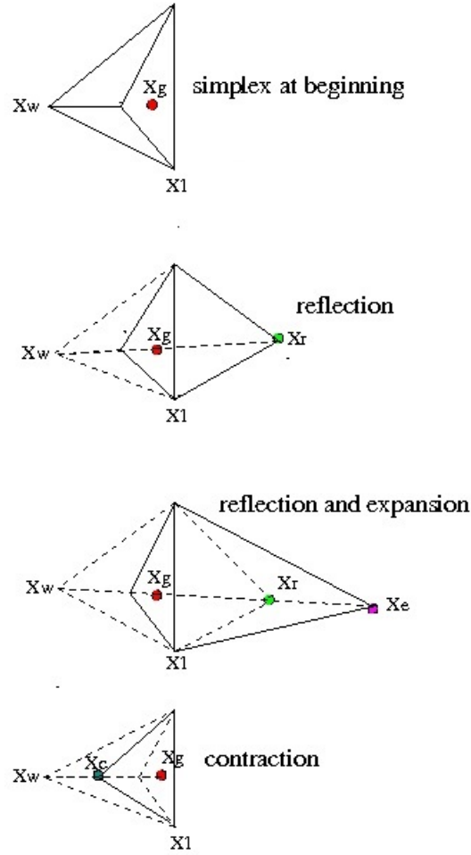
Figure B.4 Update of the simplex (tetrahedron) in 3-parameter optimization case [138].
