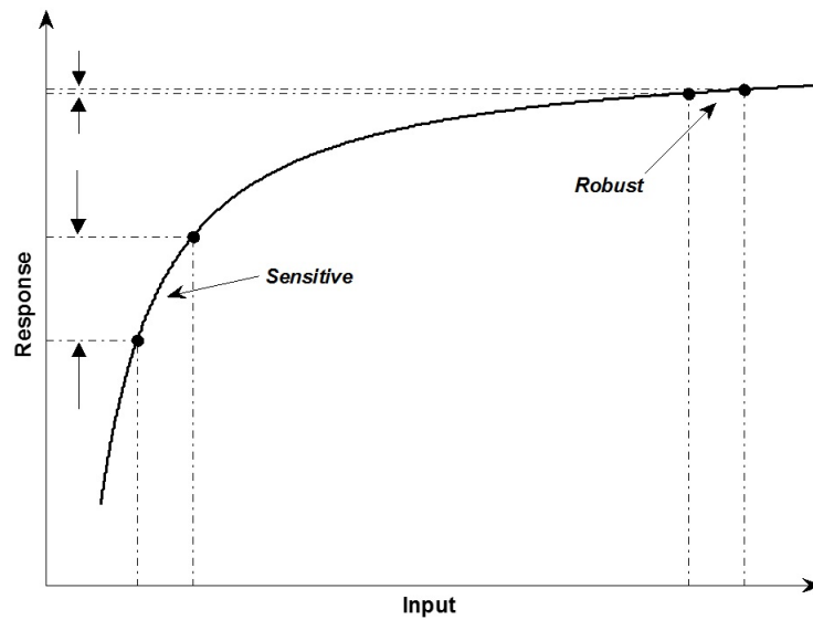
Figure B.6 The transmitted variation in the response vs. the choice of level of a control factor. The objective of the robust optimization is to minimize the transmitted variation to the response.
