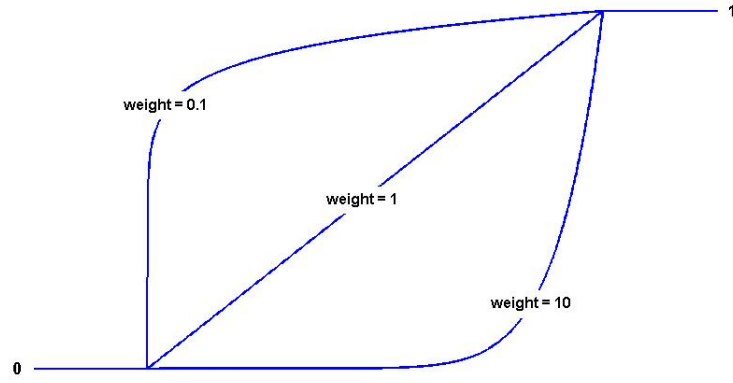
Figure B.5 Desirability functions according to weights for the maximization case.
