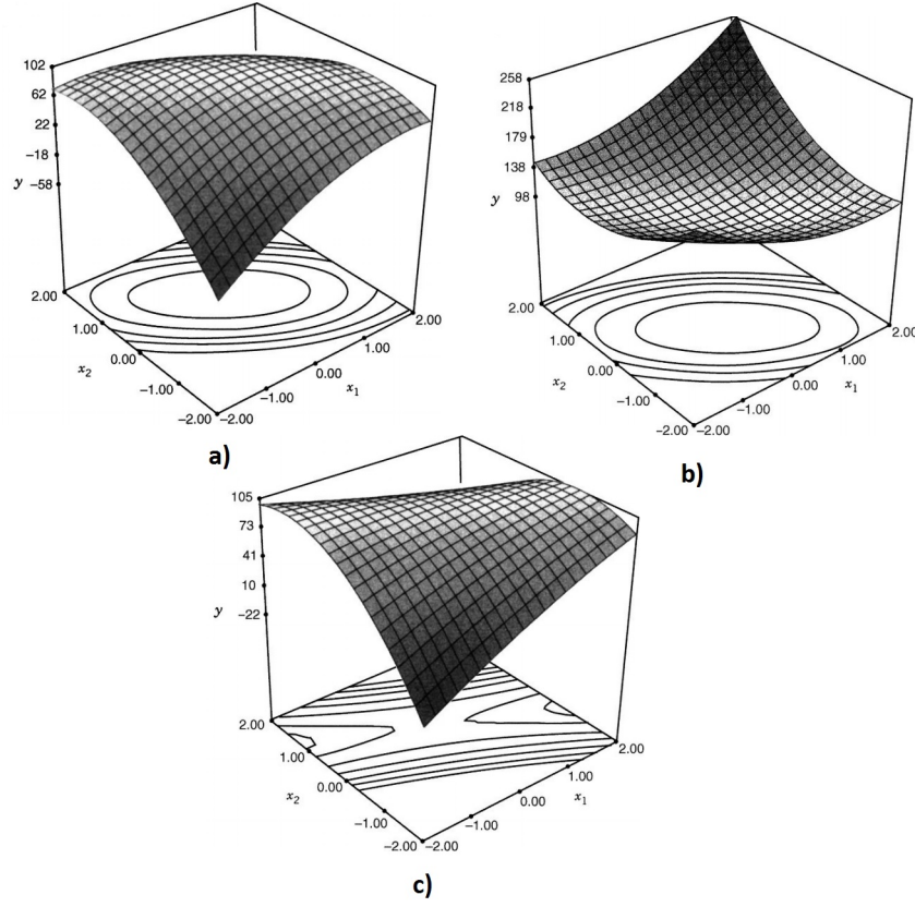
Figure B.2 Response surface of a second-order system displaying a) a maximum, b) a minimum, and c) a saddle point [38].
