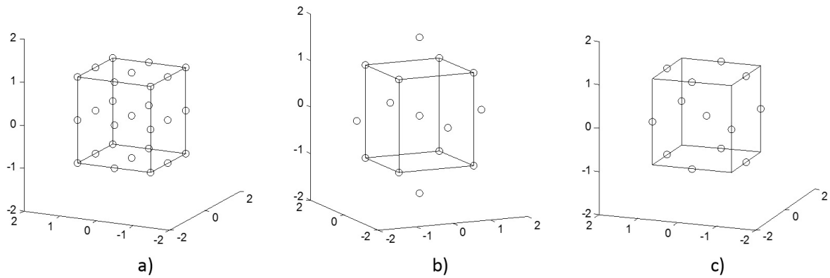
Figure B.1 Second-order experiment designs. a) 3^k factorial, b) CCD, and c) BBD.
