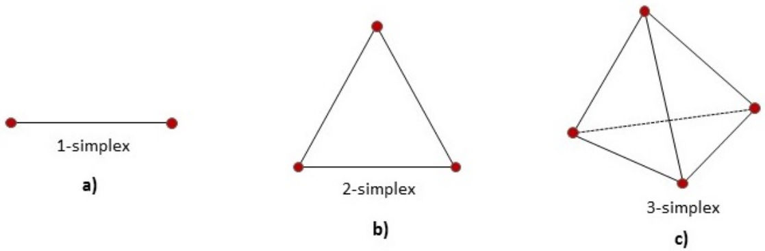
Figure B.3 Simplex types. a) A 1-simplex is a line, b) a 2-simplex is a triangle, and c) a 3-simplex is a tetrahedron.
