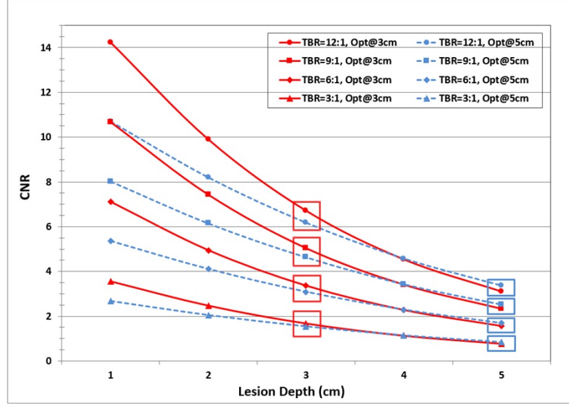
Figure 2.9 Collimators' performances at various lesion depths ranging from 1 cm to 5 cm for TBR values from 3:1 to 12:1.
