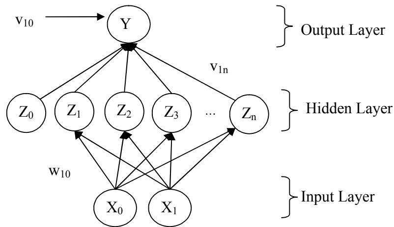
Figure 5.1. Multi-layer Perceptron
