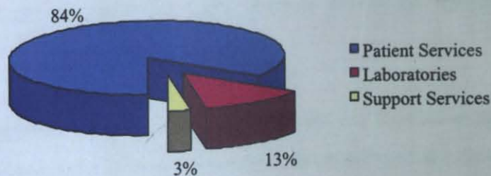
Figure 4.36. Percentage distribution of the of the health-care waste generation with respect to generation sources.
