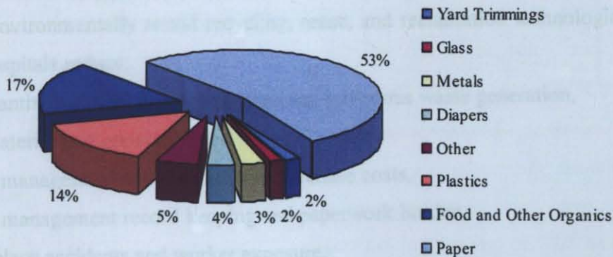
Figure 2.2. Percent solid waste composition in hospitals
