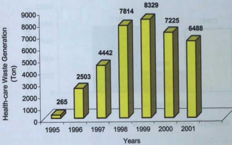
Figure 4.30. The quantity of collected health-care wastes in İstanbul between 1995-2001 (Öztürk and İskenderoğlu, 2002).
