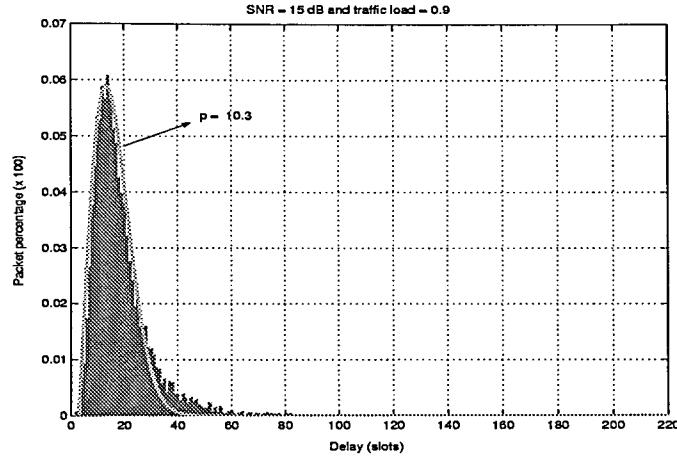
Figure 5.14. Delay distribution for the ICA-based method when \text{SNR} = 15 dB and traffic load (\lambda J) = 0.9 packet/slot (single antenna)
