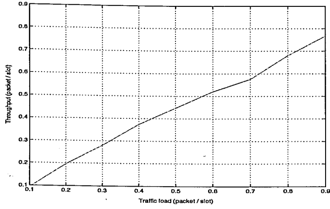
Figure 5.2. Throughput ( \lambda_T ) versus traffic load ( \lambda J ) for the ICA-based method when SNR = \infty (single antenna)
