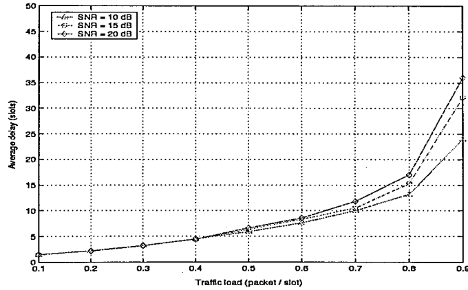
Figure 5.3. Average delay ( \bar{D} ) versus traffic load ( \lambda J ) for the ICA-based method (single antenna)
