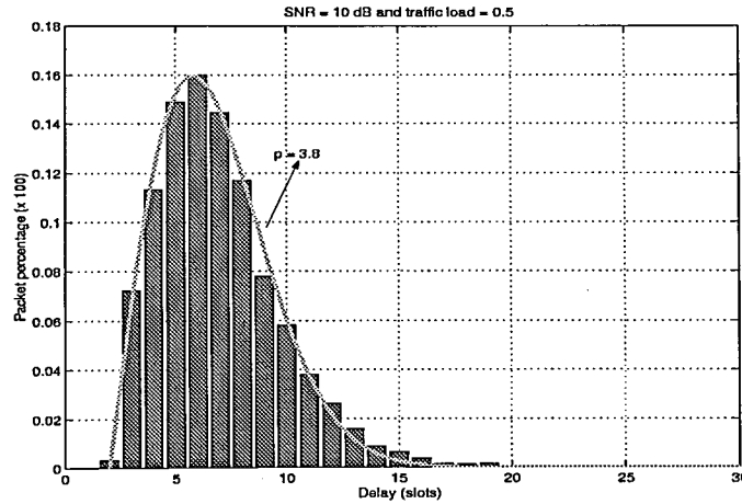
Figure 5.10. Delay distribution for the ICA-based method when SNR = 10 dB and traffic load (\lambda J) = 0.5 packet/slot (single antenna)
