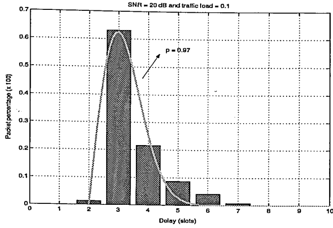
Figure 5.15. Delay distribution for the ICA-based method when SNR = 20 dB and traffic load ( \lambda J ) = 0.1 packet/slot (single antenna)
