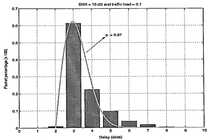
Figure 5.12. Delay distribution for the ICA-based method when \text{SNR} = 15 dB and traffic load (\lambda J) = 0.1 packet/slot (single antenna)
