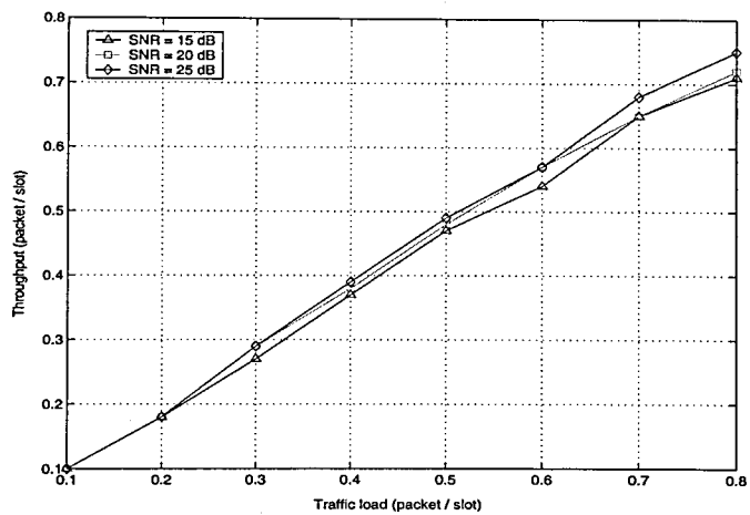
Figure 5.21. Throughput ( \lambda_T ) versus traffic load ( \lambda J ) for BNDMA (two antennas)
