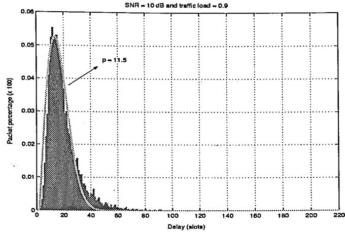
Figure 5.11. Delay distribution for the ICA-based method when \text{SNR} = 10 dB and traffic load (\lambda J) = 0.9 packet/slot (single antenna)
