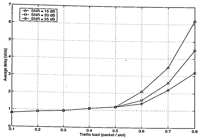
Figure 5.20. Average delay ( \bar{D} ) versus traffic load ( \lambda J ) for BNDMA (two antennas)
