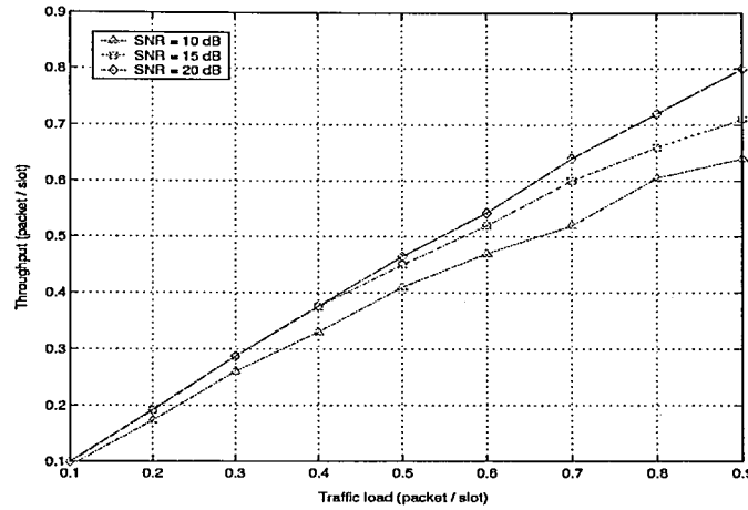
Figure 5.5. Throughput ( \lambda_T ) versus traffic load ( \lambda_J ) for the ICA-based method with error correction (single antenna)
