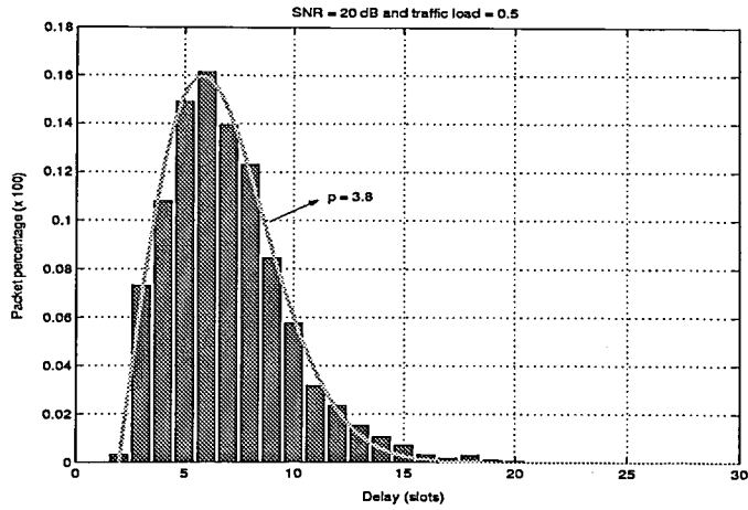
Figure 5.16. Delay distribution for the ICA-based method when SNR = 20 dB and traffic load ( \lambda J ) = 0.5 packet/slot (single antenna)
