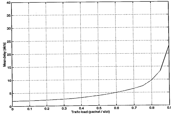
Figure 4.3. Mean delay ( D ) versus traffic load ( \lambda J ) depending on the mathematical results
