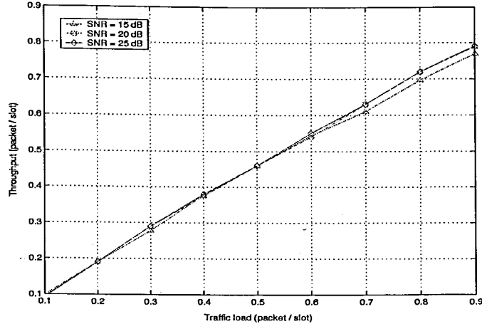
Figure 5.7. Throughput ( \lambda_T ) versus traffic load ( \lambda_J ) for the ICA-based method with no error correction (two antennas)
