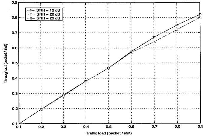
Figure 5.8. Throughput ( \lambda_T ) versus traffic load ( \lambda_J ) for the ICA-based method with error correction (two antennas)
