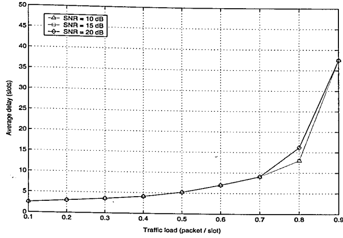
Figure 5.18. Average delay ( \bar{D} ) versus traffic load ( \lambda J ) for BNDMA (single antenna)
