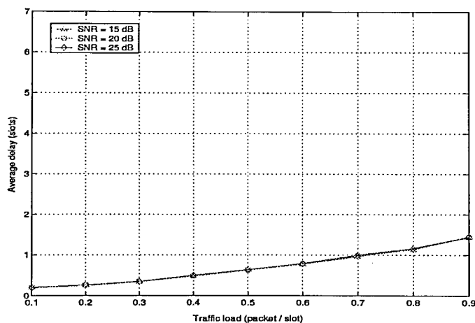
Figure 5.6. Average delay ( \bar{D} ) versus traffic load ( \lambda J ) for the ICA-based method (two antennas)
