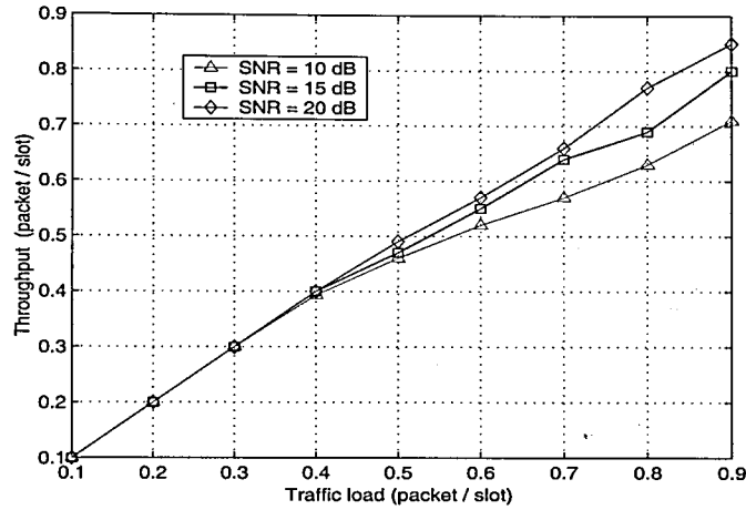
Figure 5.19. Throughput ( \lambda_T ) versus traffic load ( \lambda J ) for BNDMA (single antenna)
