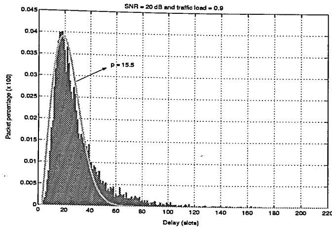
Figure 5.17. Delay distribution for the ICA-based method when SNR = 20 dB and traffic load (\lambda J) = 0.9 packet/slot (single antenna)
