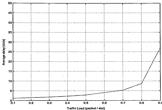
Figure 5.1. Average delay ( \bar{D} ) versus traffic load ( \lambda J ) for the ICA-based method when SNR = \infty (single antenna)
