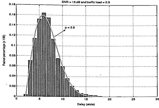
Figure 5.13. Delay distribution for the ICA-based method when \text{SNR} = 15 dB and traffic load (\lambda J) = 0.5 packet/slot (single antenna)
