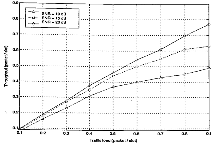
Figure 5.4. Throughput ( \lambda_T ) versus traffic load ( \lambda_J ) for the ICA-based method with no error correction (single antenna)
