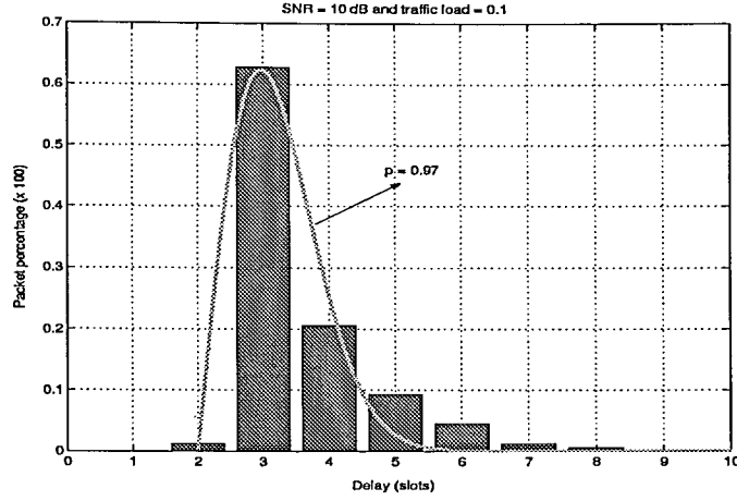
Figure 5.9. Delay distribution for the ICA-based method when SNR = 10 dB and traffic load (\lambda J) = 0.1 packet/slot (single antenna)
