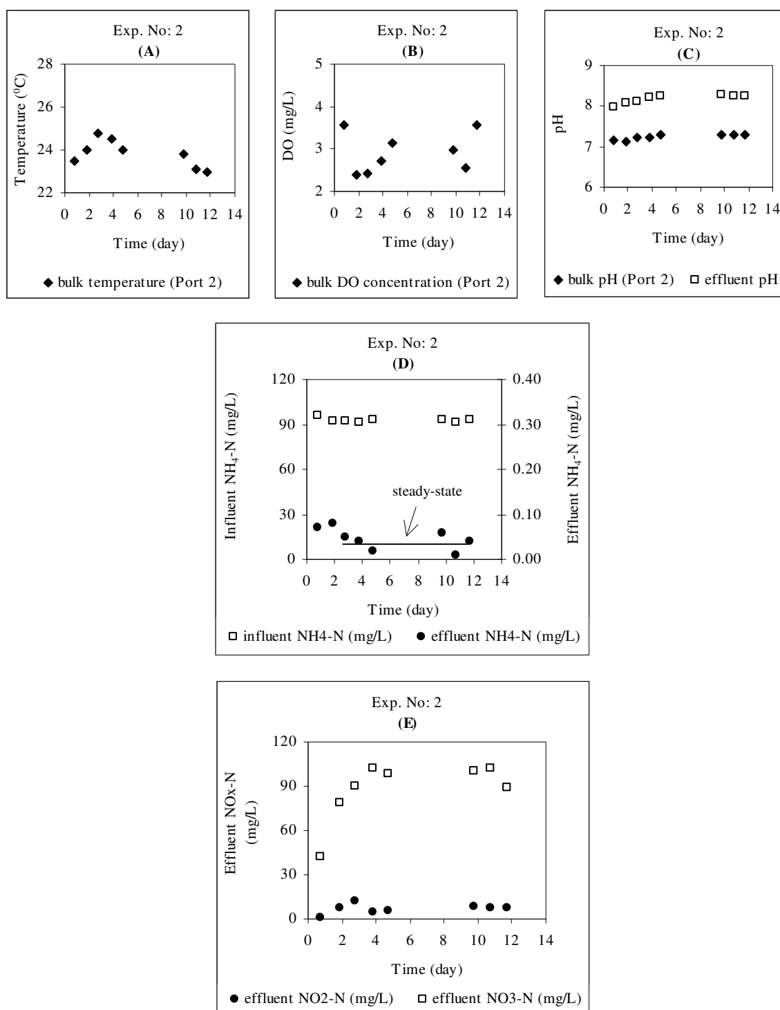
Figure R.2. Preliminary continuous-flow experiment No:2 measurements for (a) T, (b) DO, (c) pH, (d) \text{NH}_4\text{-N} and (e) \text{NO}_x\text{-N}
