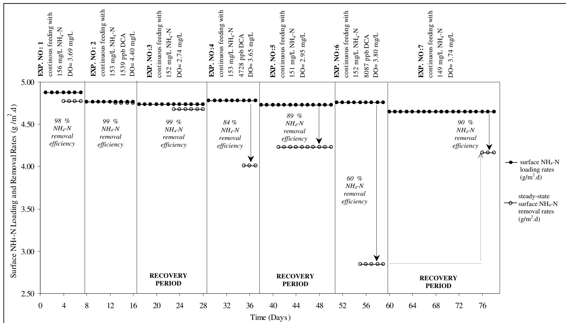
Figure 6.56. Chronological illustration of \text{NH}_4\text{-N} loading and removal rates in the 1 st set of experiments [influent \text{NH}_4\text{-N} = 149-156 mg/L, influent 1,2-DCA=1539-8087 \mu\text{g/L} ]
