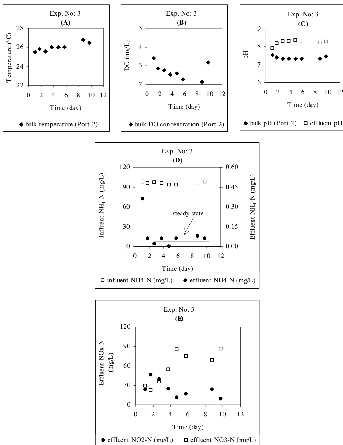
Figure R.3. Preliminary continuous-flow experiment No:3 measurements for (a) T, (b) DO, (c) pH, (d) \text{NH}_4\text{-N} and (e) \text{NO}_x\text{-N}
