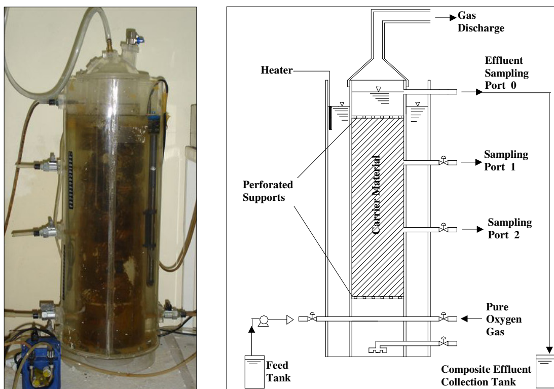
Figure 5.5. Experimental set-up of the nitrifying biofilm reactor
