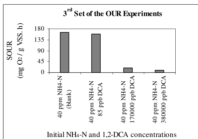
Figure 6.30. SOUR values observed in the 3 rd set OUR experiments with 1,2-DCA [Initial NH 4 -N = 40 mg/L, Initial 1,2-DCA = 85-380000 µg/L]
