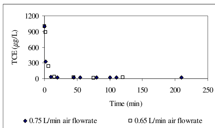
Figure 6.5. TCE stripping under fine- bubble diffused aeration
