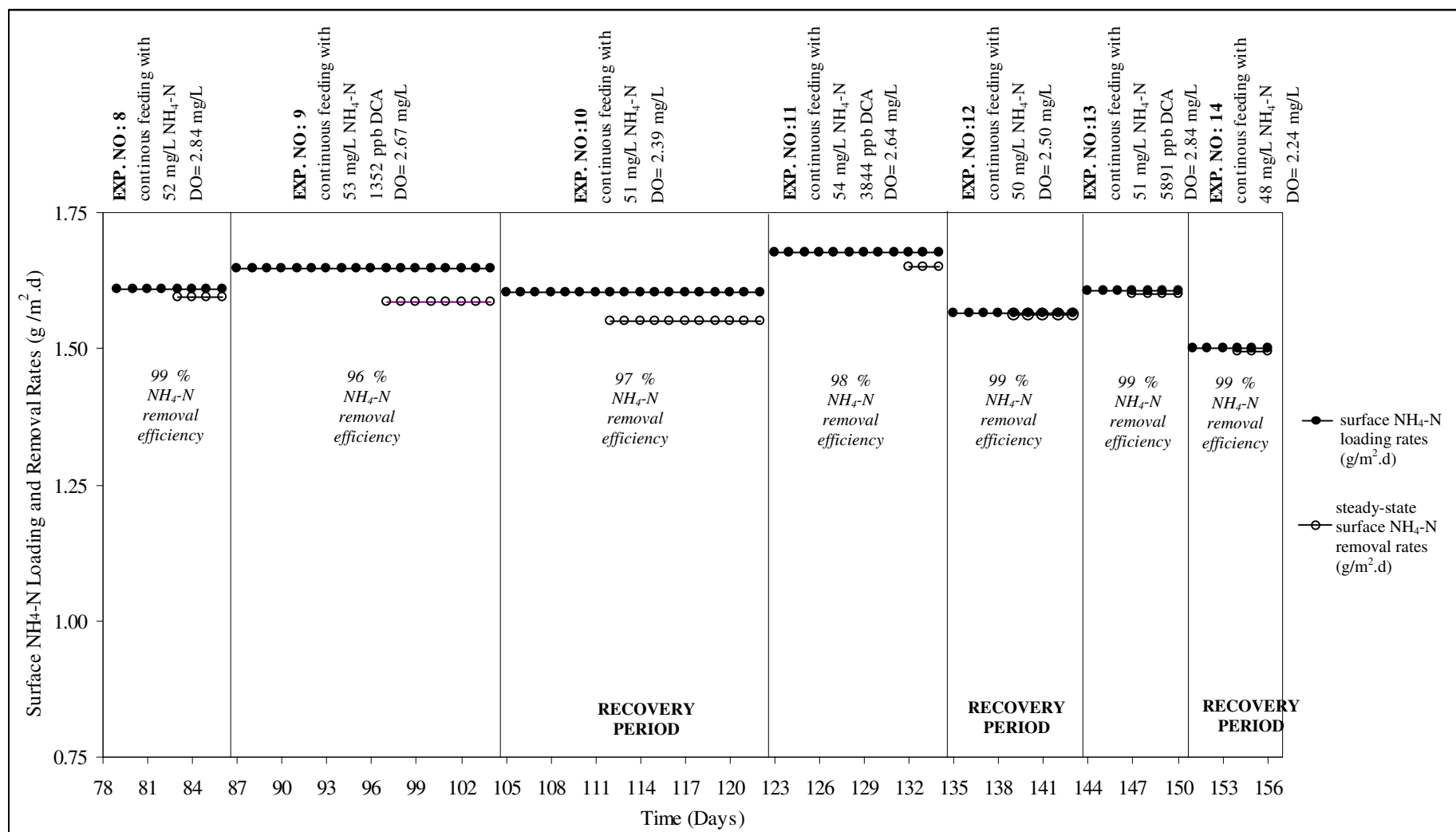
Figure 6.57. Chronological illustration of \text{NH}_4\text{-N} loading and removal rates in the 2 nd set of experiments [influent \text{NH}_4\text{-N} = 48-54 mg/L , influent 1,2-DCA=1352-5891 \mu\text{g}/\text{L} ]
