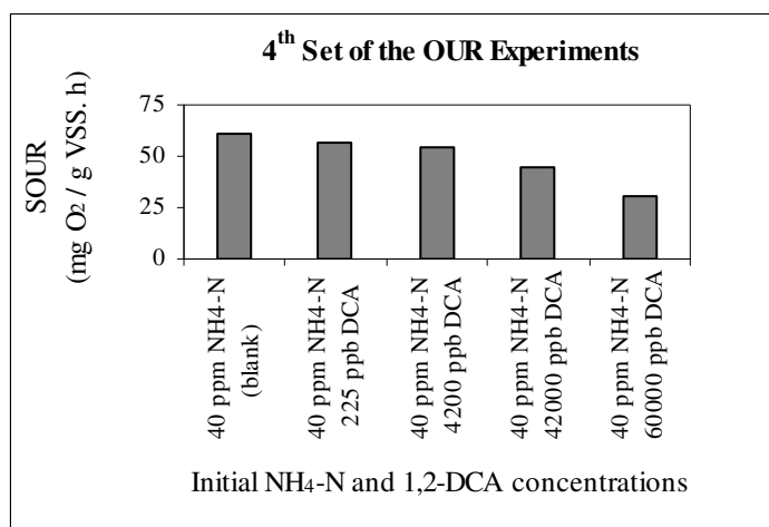
Figure 6.31. SOUR values observed in the 4 th set OUR experiments with 1,2-DCA [Initial NH 4 -N = 40 mg/L, Initial 1,2-DCA = 225-60000 µg/L]
