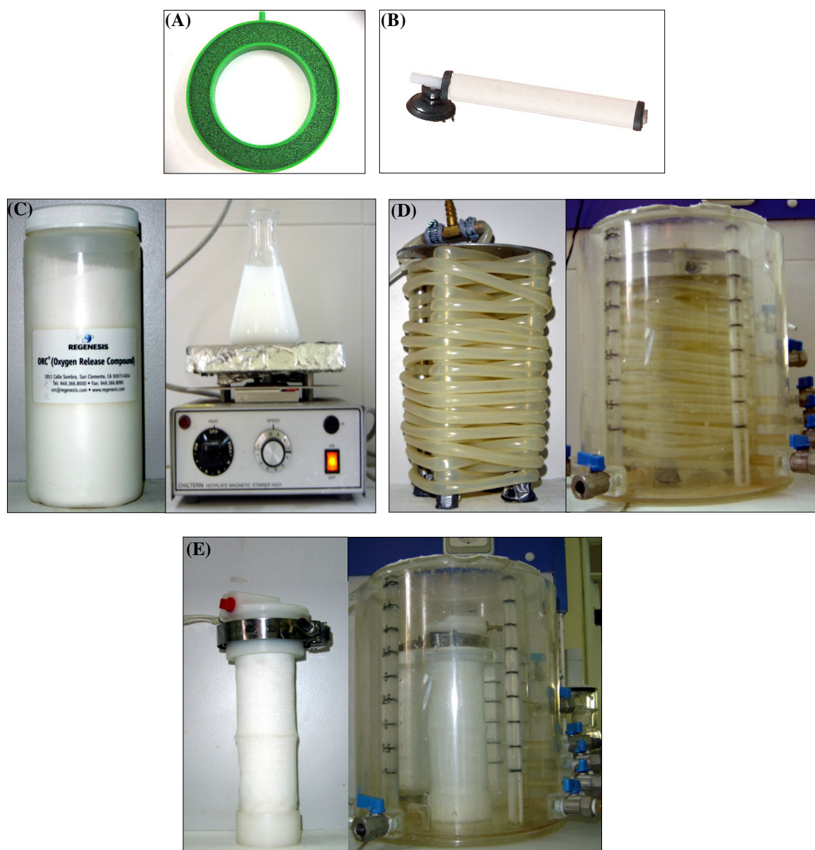
Figure 5.2. Oxygenation systems (a) fine-bubble airstone diffuser (Has Tropical Ltd.), (b) micro bubble ceramic diffuser (Foster&Smith Inc., U.S.), (c) oxygen releasing compound (ORC) (Regenesis Inc., U.S.), (d) gas permeable silicon-tubing (McMaster-Carr, Inc., U.S.) and (e) gas permeable hollow fiber membrane module (Celgard Inc., U.S.)
