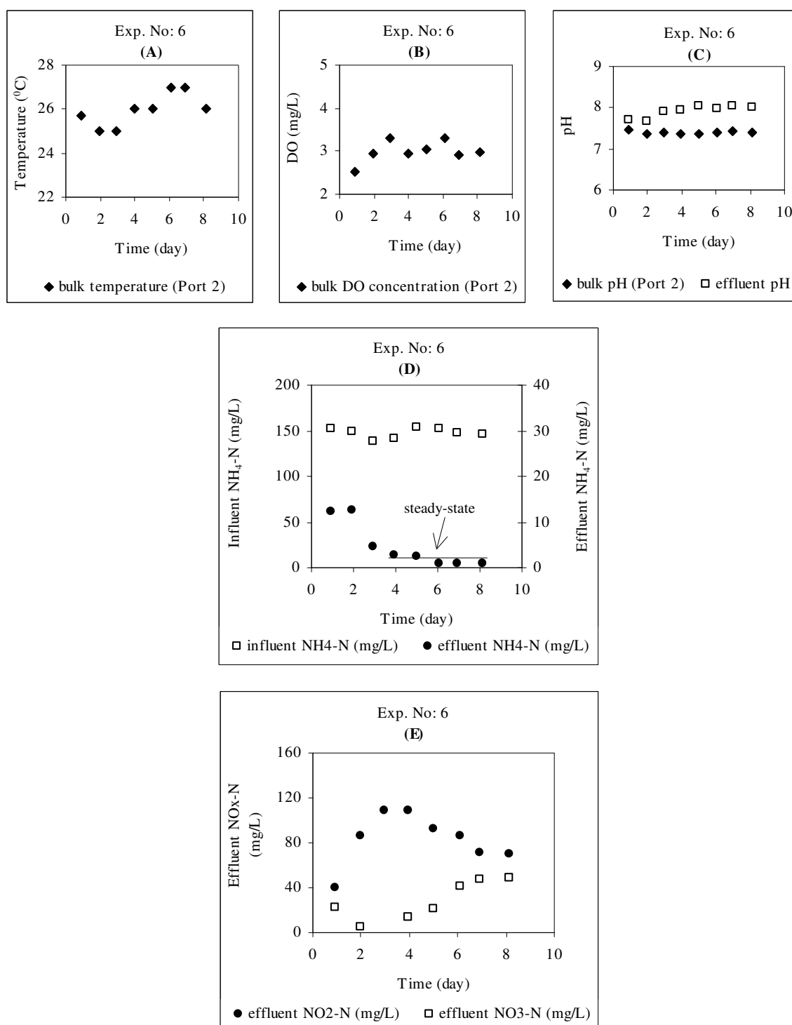
Figure R.6. Preliminary continuous-flow experiment No:6 measurements for (a) T, (b) DO, (c) pH, (d) \text{NH}_4\text{-N} and (e) \text{NO}_x\text{-N}
