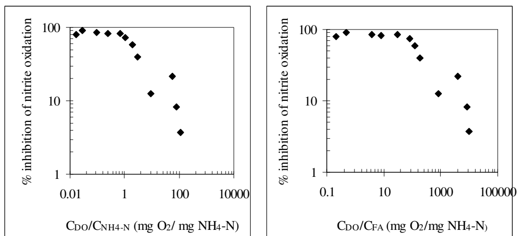
Figure 6.55. Dependence of nitrite accumulation on the ratio of (a) bulk dissolved oxygen to ammonium, (b) bulk dissolved oxygen to free ammonia
