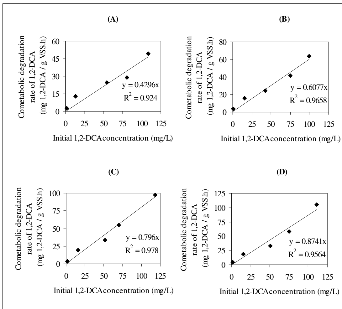
Figure 6.48. Cometabolic degradation rates of DCA ( q_{\text{DCA}} ) at initial \text{NH}_4\text{-N} concentrations of (a) 50 mg/L, (b) 100 mg/L, (c) 200 mg/L, (d) 400 mg/L with respect to the initial 1,2-DCA concentrations
