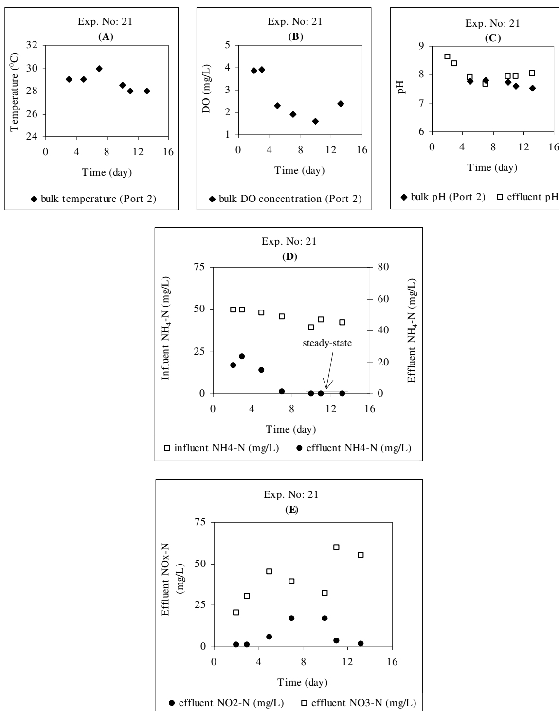
Figure S.21. Continuous-flow experiment with 1,2-DCA No:21 measurements for (a) T, (b) DO, (c) pH, (d) \text{NH}_4\text{-N} and (e) \text{NO}_x\text{-N}
