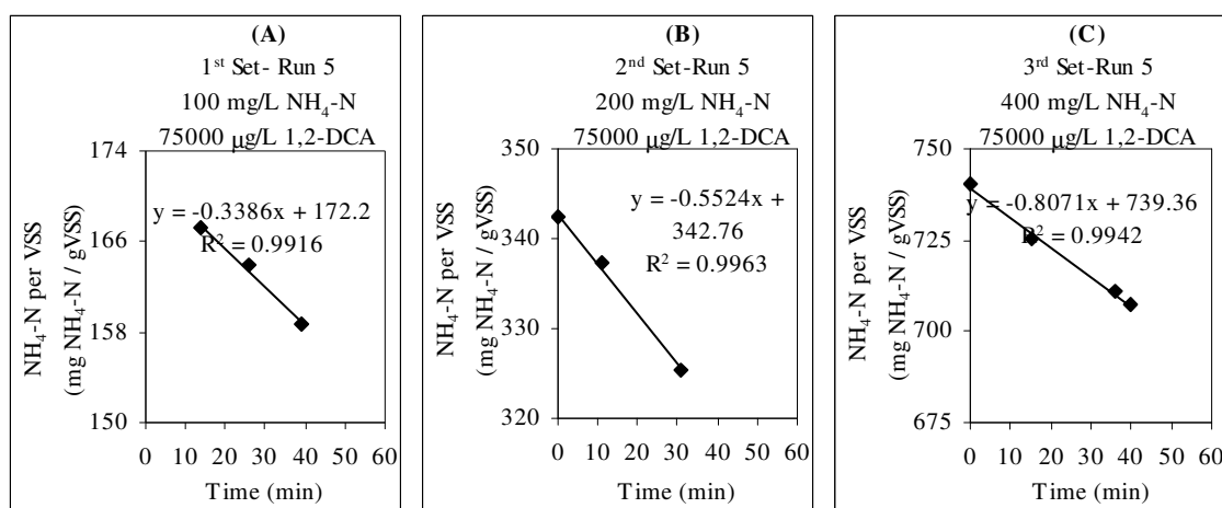
Figure P.5. Specific ammonium utilization in batch experiments with 1,2-DCA directed to kinetic modelling (a) 1 st Set-Run 5, (b) 2 nd Set-Run 5, (c) 3 rd Set-Run 5
