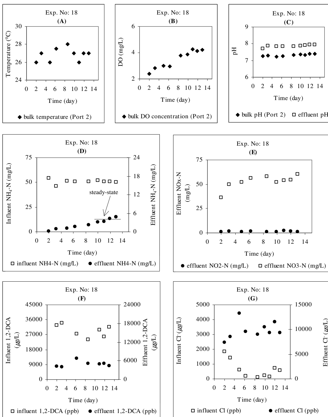
Figure S.18. Continuous-flow experiment with 1,2-DCA No:18 measurements for (a) T, (b) DO, (c) pH, (d) \text{NH}_4\text{-N} , (e) \text{NO}_x\text{-N} , (f) 1,2-DCA and (g) \text{Cl}^-
