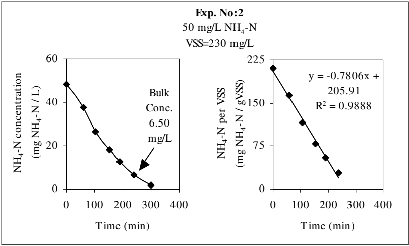
Figure B.2. Ammonium ( NH_4-N ) utilization under diffused air condition in Exp. No.2
