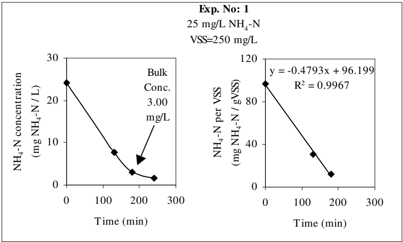
Figure B.1. Ammonium ( NH_4-N ) utilization under diffused air condition in Exp. No.1
