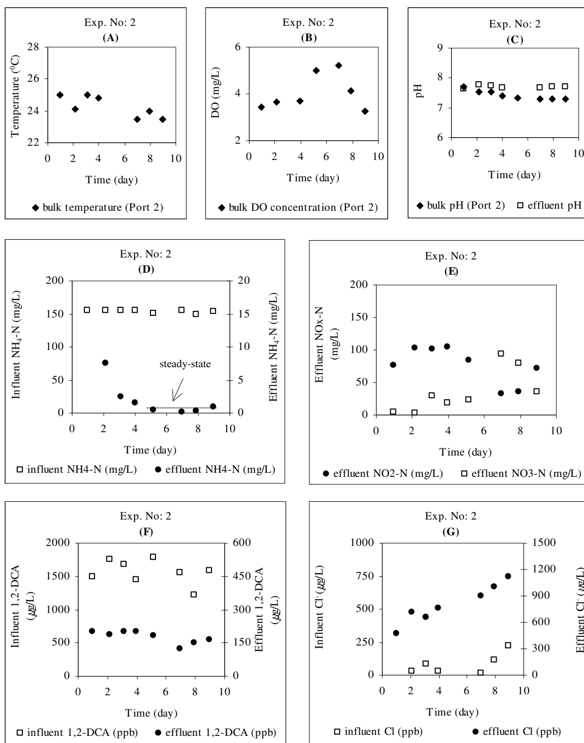
Figure S.2. Continuous-flow experiment with 1,2-DCA No:2 measurements for (a) T, (b) DO, (c) pH, (d) \text{NH}_4\text{-N} , (e) \text{NO}_x\text{-N} , (f) 1,2-DCA and (g) \text{Cl}^-
