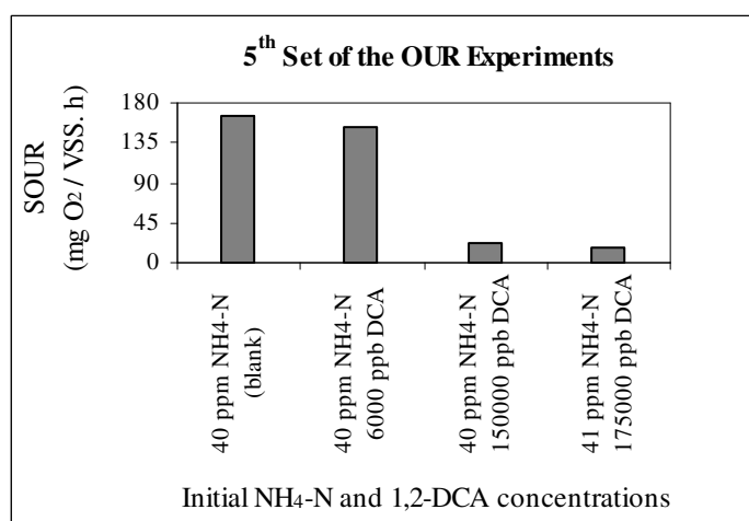
Figure 6.32. SOUR values observed in the 5 th set OUR experiments with 1,2-DCA [Initial NH 4 -N = 40 mg/L, Initial 1,2-DCA = 6000-175000 µg/L]
