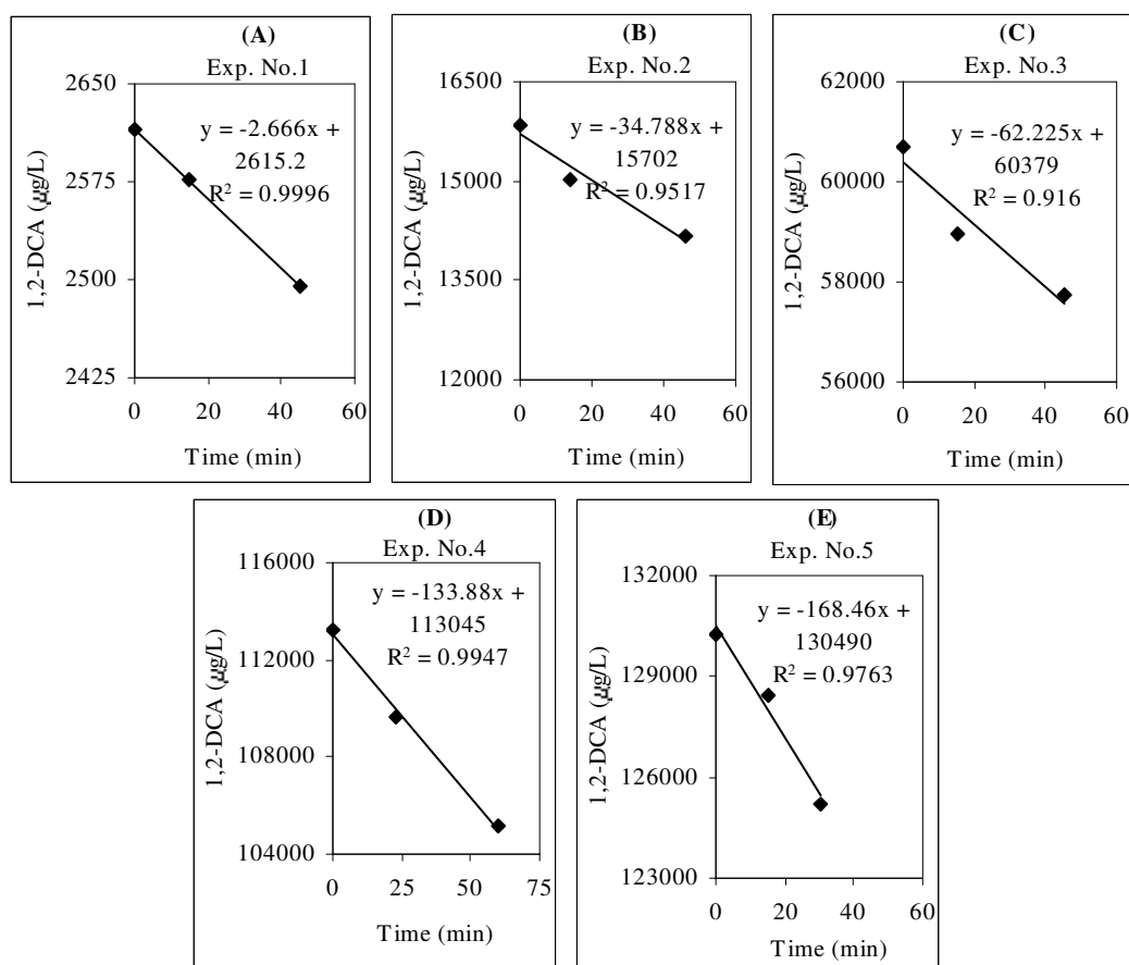
Figure N.1. Volatilization of 1,2-DCA for the initial concentration of (a) 2614 \mu\text{g/L} (b) 15847 \mu\text{g/L} , (c) 60705 \mu\text{g/L} , (d) 113254 \mu\text{g/L} , (e) 130262 \mu\text{g/L}
