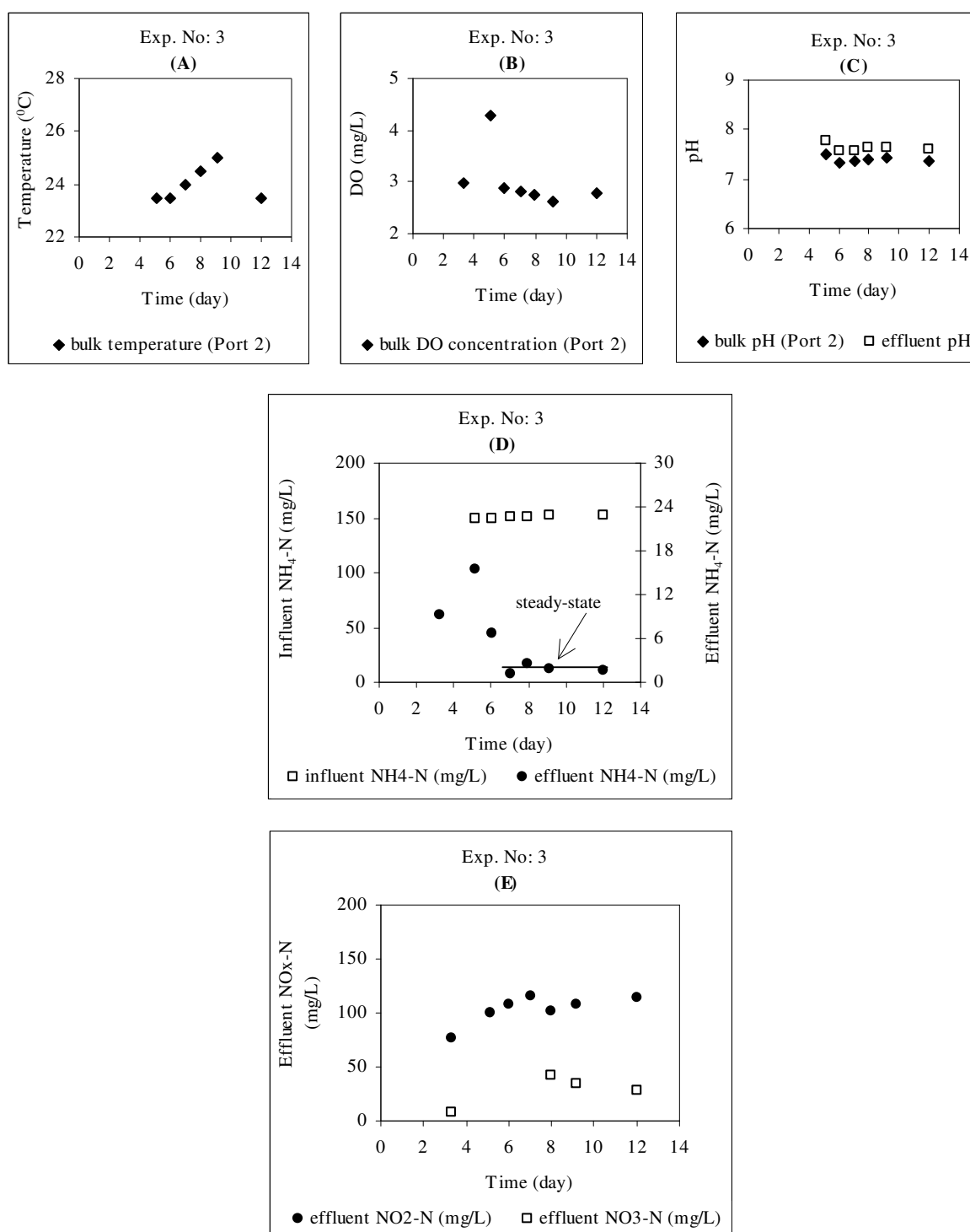
Figure S.3. Continuous-flow experiment with 1,2-DCA No:3 measurements for (a) T, (b) DO, (c) pH, (d) \text{NH}_4\text{-N} and (e) \text{NO}_x\text{-N}
