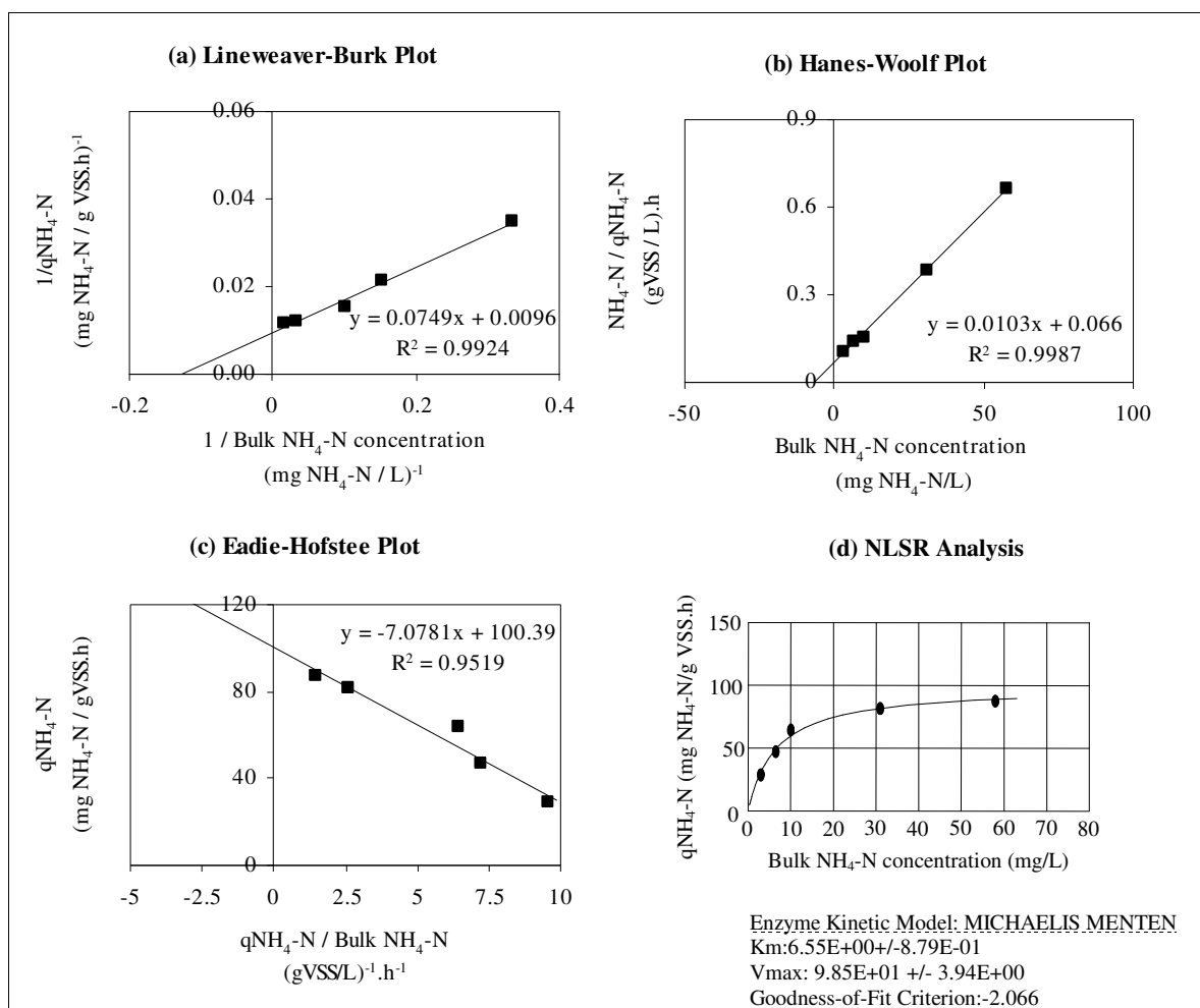
Figure 6.3. Determination of q_{\max, \text{NH}_4\text{-N}} and K_s with respect to bulk \text{NH}_4\text{-N} concentrations using (a) Lineweaver-Burk plot, (b) Hanes-Woolf plot, (c) Eadie-Hofstee plot, and (d) NLSR analysis
