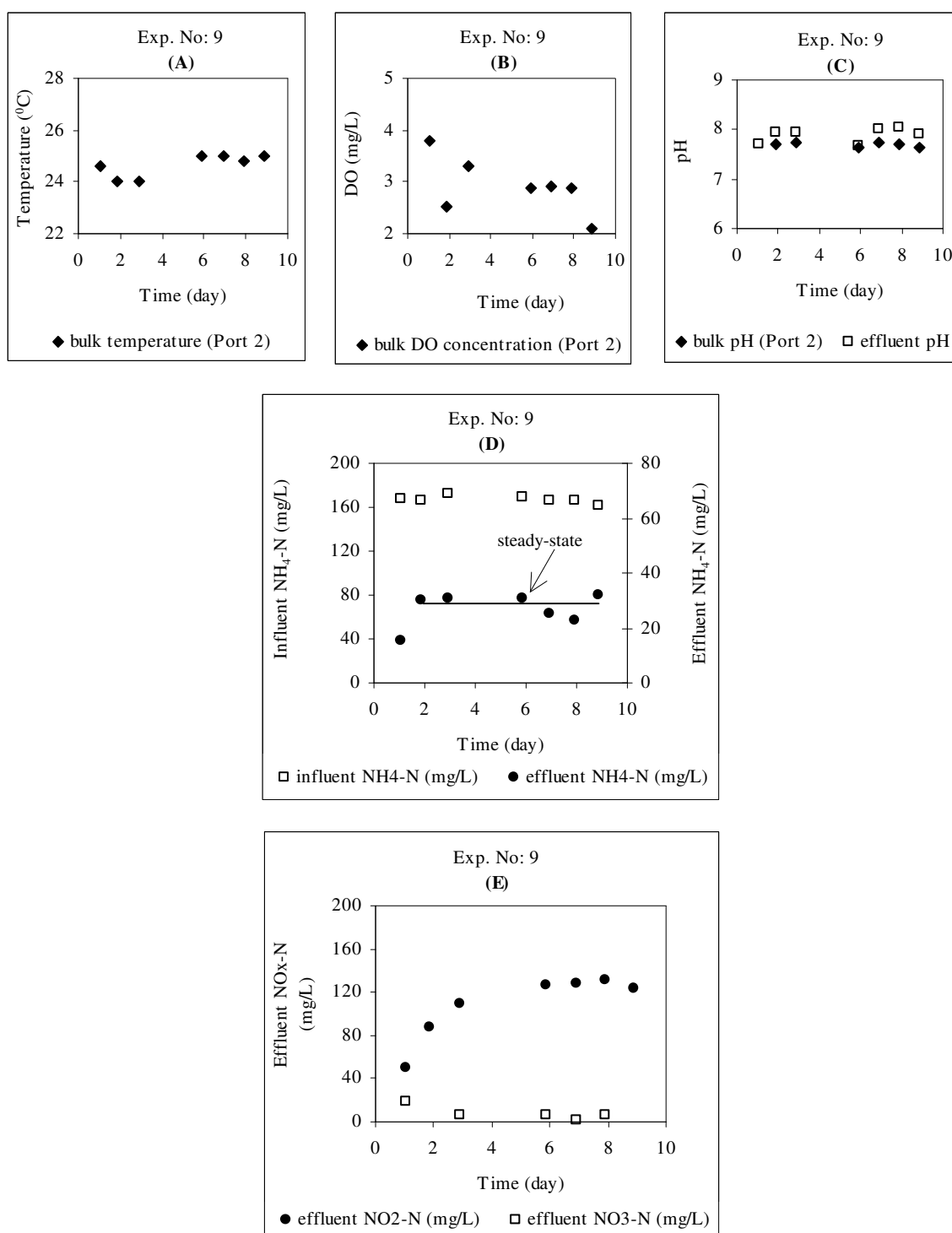
Figure R.9. Preliminary continuous-flow experiment No:9 measurements for (a) T, (b) DO, (c) pH, (d) \text{NH}_4\text{-N} and (e) \text{NO}_x\text{-N}
