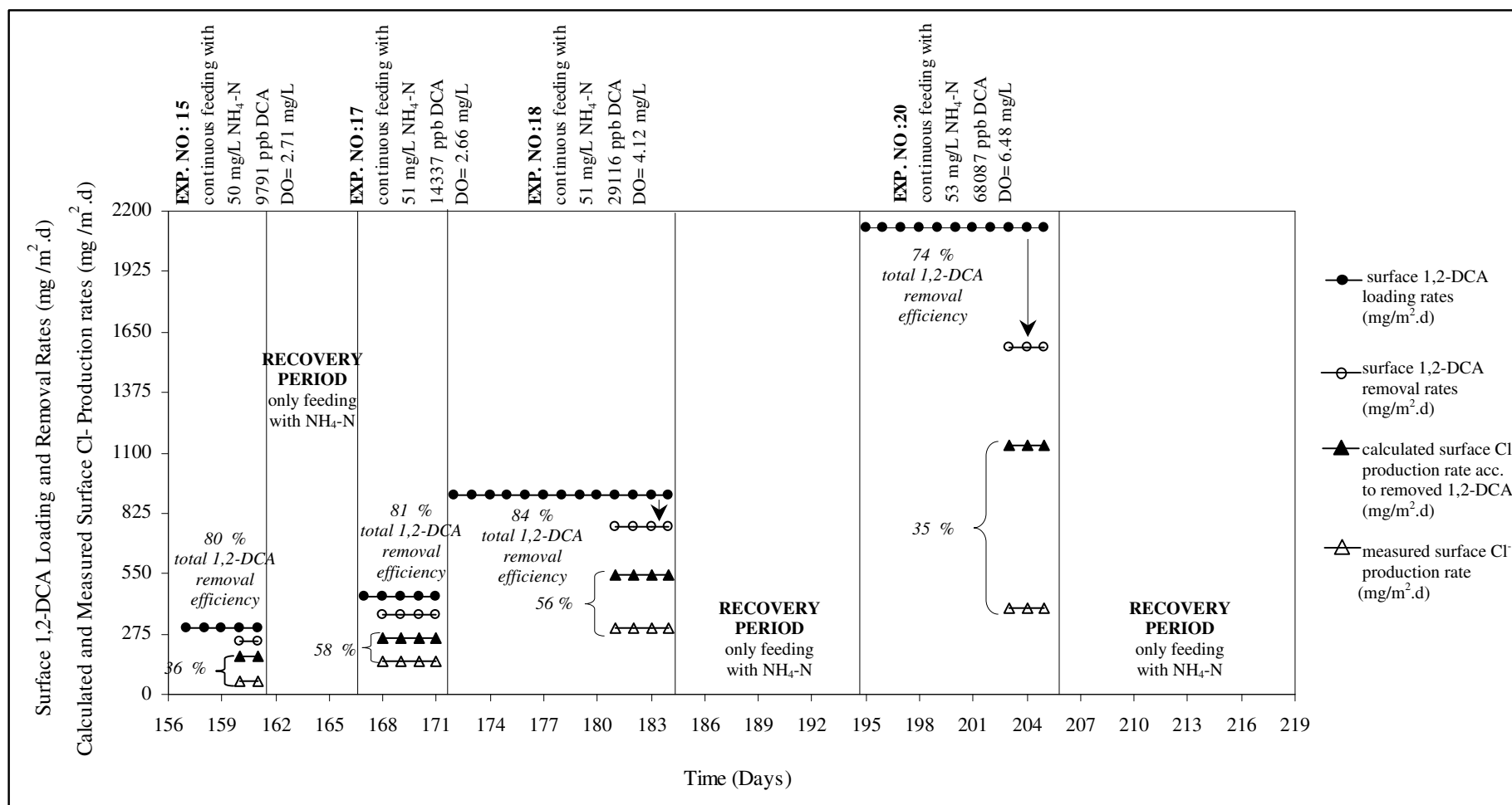
Figure 6.63. Chronological illustration of 1,2-DCA loading and removal rates, calculated and measured surface \text{Cl}^- production rates in the 2 nd set of experiments [initial \text{NH}_4\text{-N} = 42-53 \text{mg}/\text{L} , initial 1,2-DCA=9791-68087 \mu\text{g}/\text{L} ]
