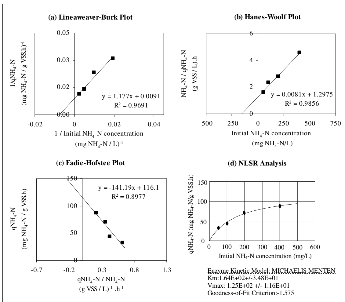
Figure 6.41. Determination of q_{max, NH_4-N}^{app} and K_s^{app} at an initial 1,2-DCA concentration of 15000 \mu\text{g/L} using (a) Lineweaver-Burk plot, (b) Hanes-Woolf plot, (c) Eadie-Hofstee plot, and (d) NLSR analysis
