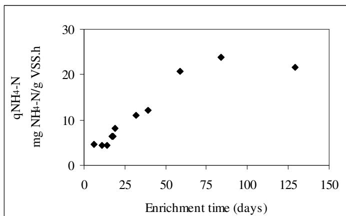
Figure 6.1. Specific ammonium utilization rates ( q_{\text{NH}_4\text{-N}} ) during the enrichment period of nitrifiers
