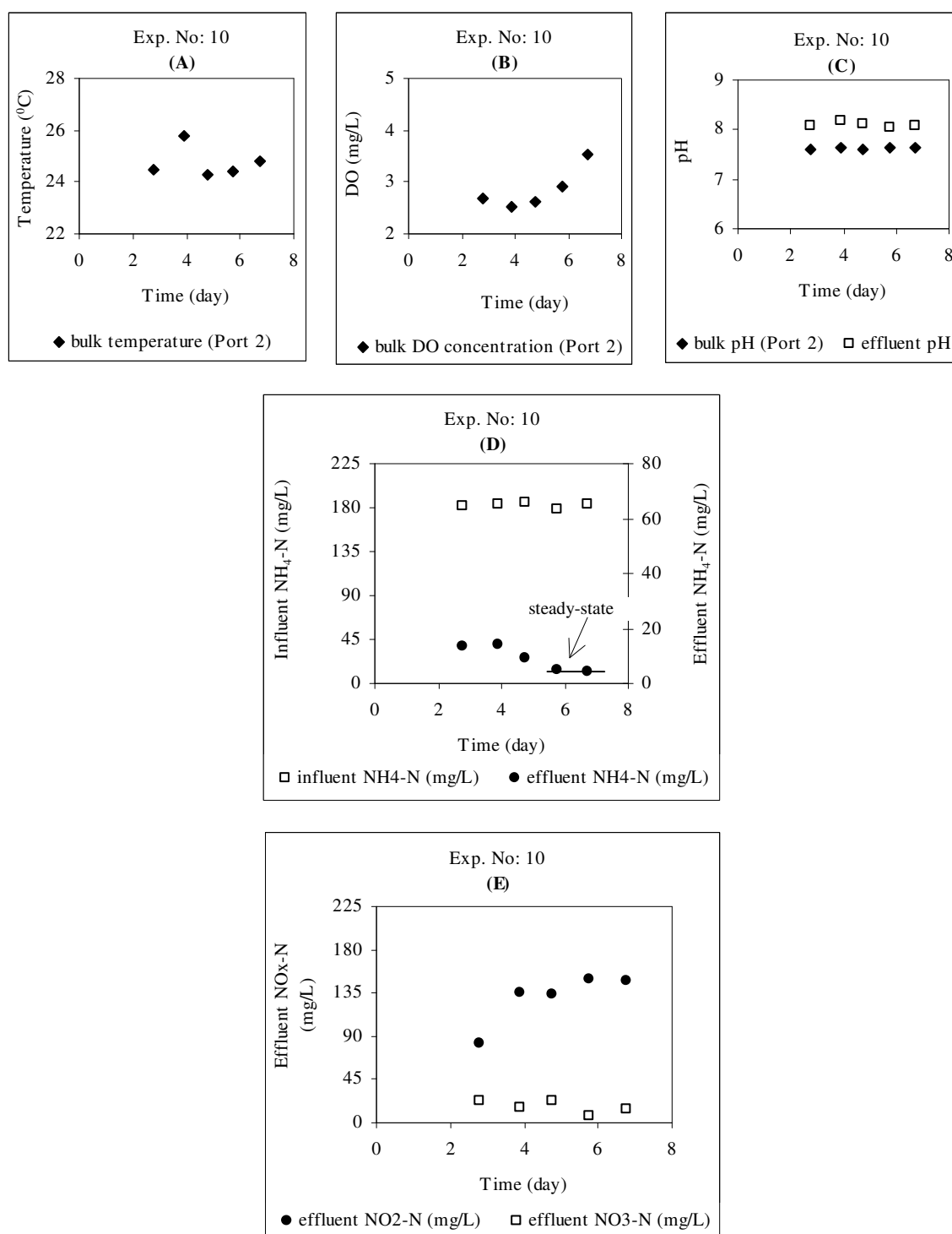
Figure R.10. Preliminary continuous-flow experiment No:10 measurements for (a) T, (b) DO, (c) pH, (d) \text{NH}_4\text{-N} and (e) \text{NO}_x\text{-N}
