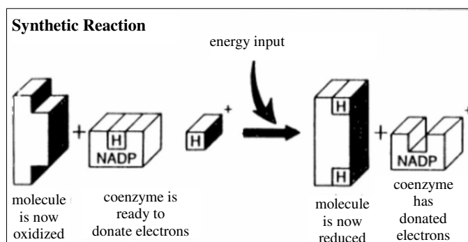
Figure 3.3. Synthetic reaction pathway (Mader, 1990)
