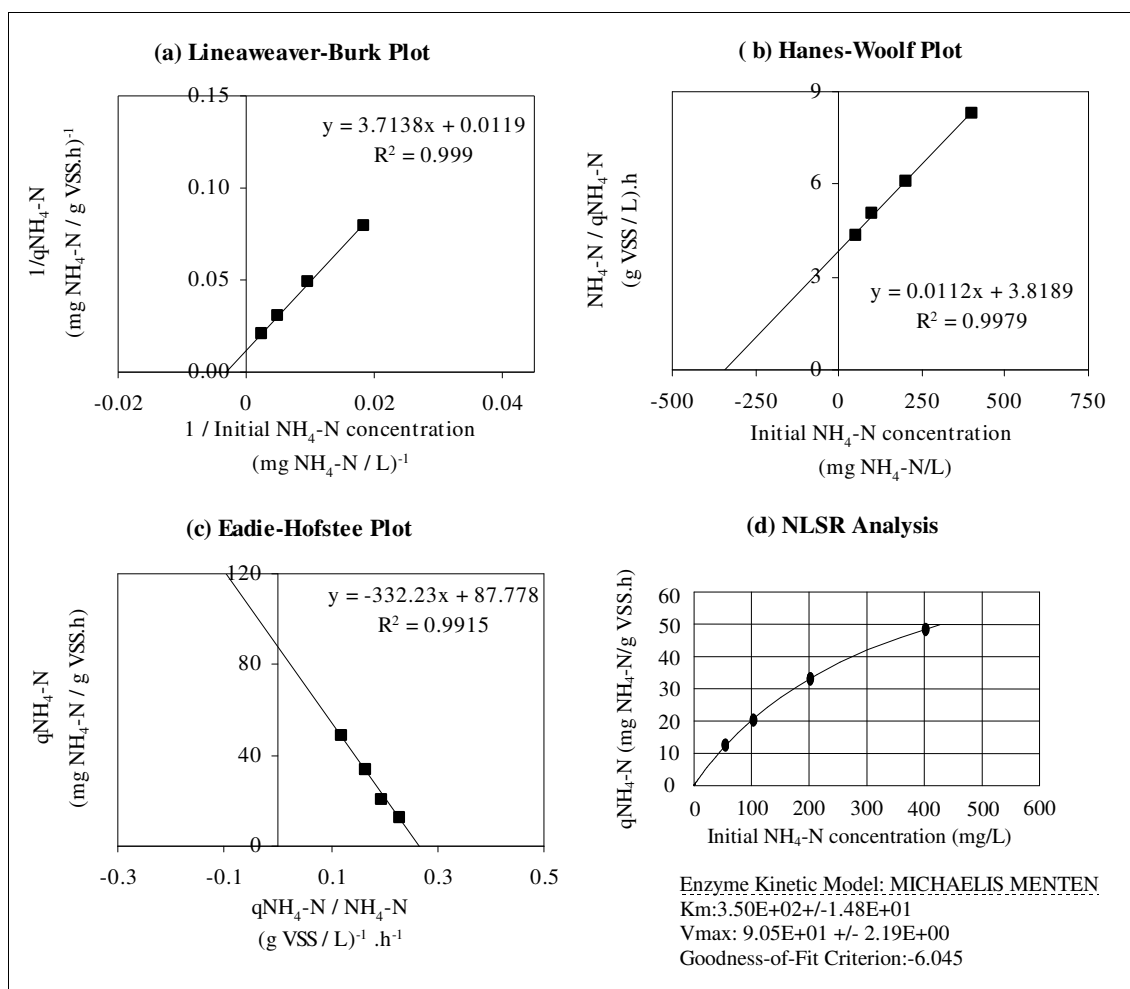
Figure 6.43. Determination of q_{max, NH_4-N}^{app} and K_s^{app} at an initial 1,2-DCA concentration of 75000 \mu\text{g/L} using (a) Lineweaver-Burk plot, (b) Hanes-Woolf plot, (c) Eadie-Hofstee plot, and (d) NLSR analysis
