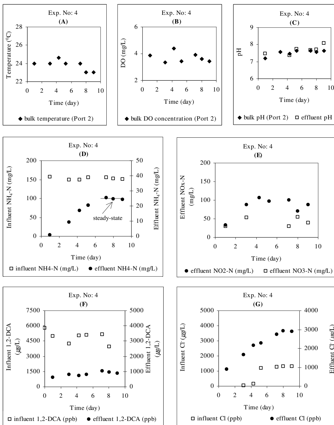
Figure S.4. Continuous-flow experiment with 1,2-DCA No:4 measurements for (a) T, (b) DO, (c) pH, (d) \text{NH}_4\text{-N} , (e) \text{NO}_x\text{-N} , (f) 1,2-DCA, and (g) \text{Cl}^-
