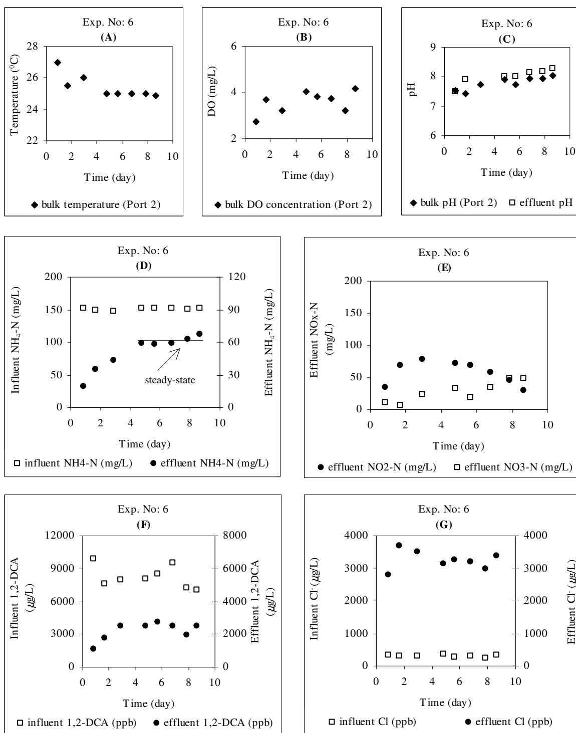
Figure S.6. Continuous-flow experiment with 1,2-DCA No:6 measurements for (a) T, (b) DO, (c) pH, (d) \text{NH}_4\text{-N} , (e) \text{NO}_x\text{-N} , (f) 1,2-DCA and (g) \text{Cl}^-
