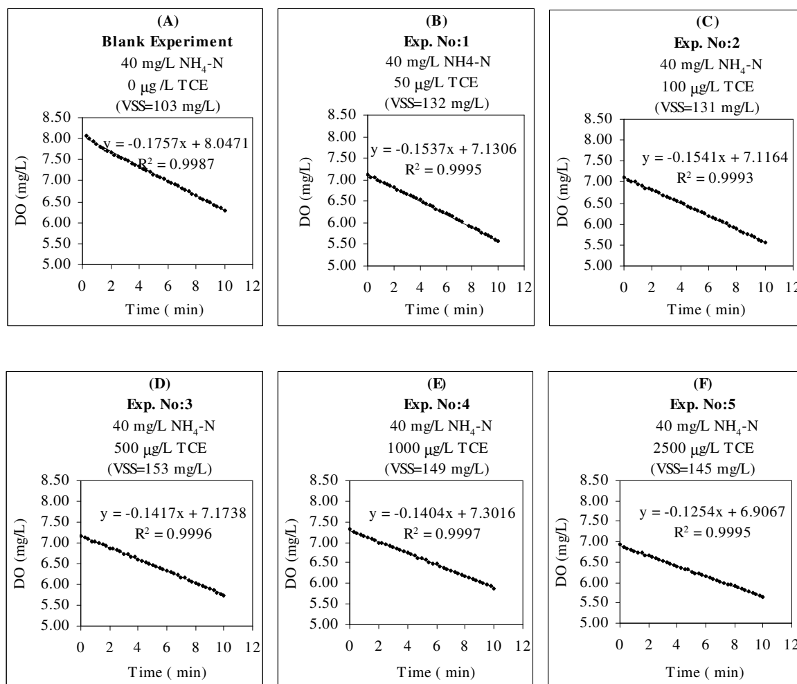
Figure C.1. Preliminary oxygen uptake with TCE (a) in the blank experiment (b) in Exp. No.1 (c) in Exp. No.2 (d) in Exp. No.3 (e) in Exp. No.4 and (f) in Exp. No.5
