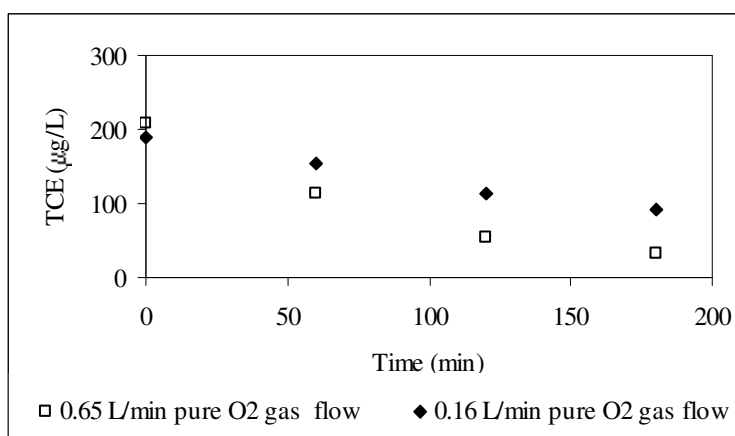
Figure 6.6. TCE stripping under micro-bubble diffused aeration with pure oxygen gas
