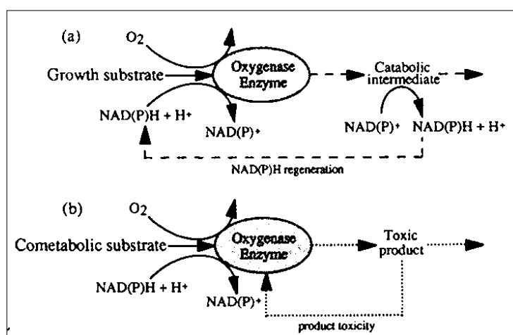
Figure 3.8. Typical oxygenase enzyme reactions for growth-substrate and cometabolic (non-growth) substrate (Chang and Alvarez-Cohen, 1995b)
