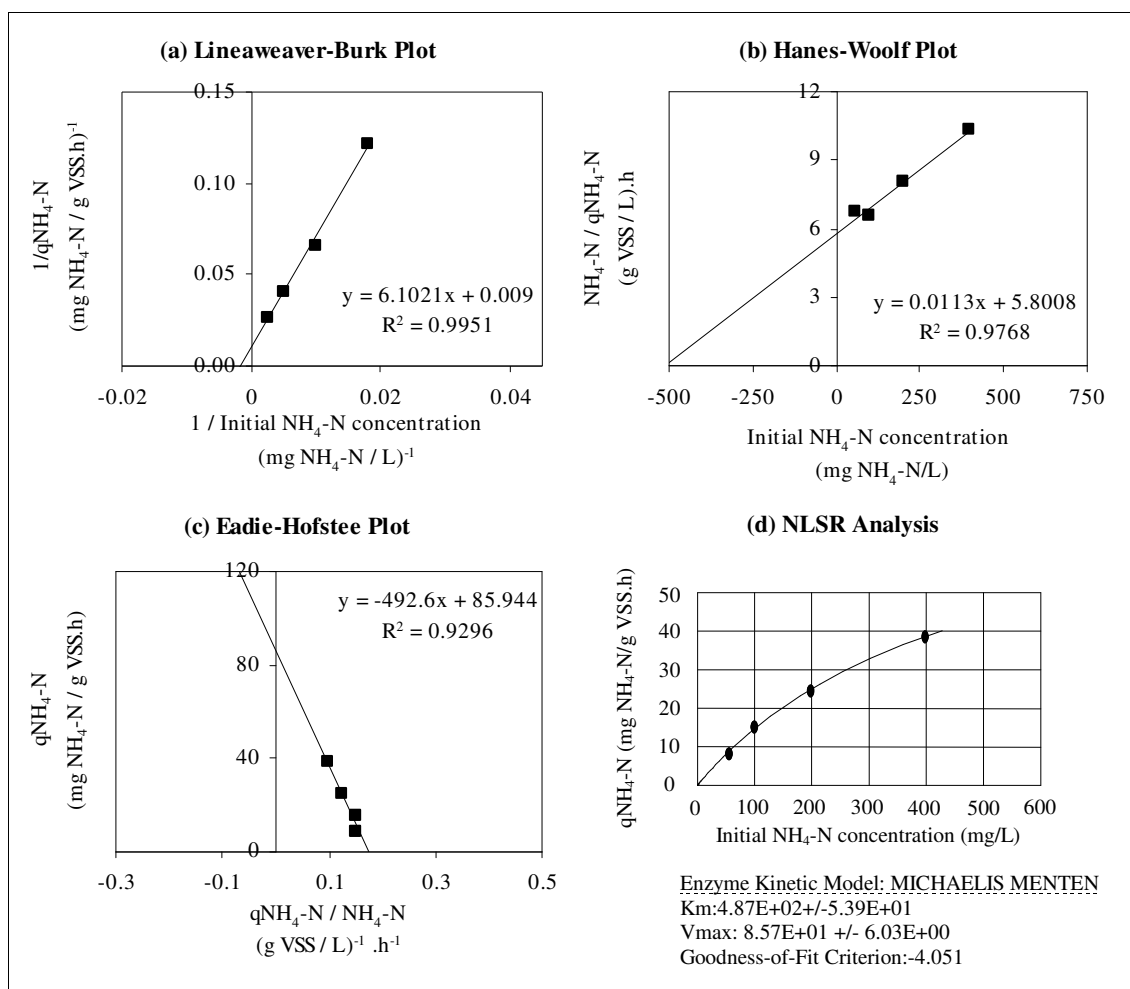
Figure 6.44. Determination of q_{max,app}^{NH_4-N} and K_s^{app} at an initial 1,2-DCA concentration of 100000 \mu\text{g/L} using (a) Lineweaver-Burk plot, (b) Hanes-Woolf plot, (c) Eadie-Hofstee plot, and (d) NLSR analysis
