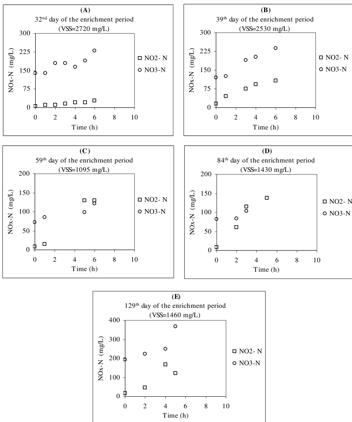
Figure A.3. Nitrite (NO 2 -N) and nitrate (NO 3 -N) measurements at the (a) 32 nd day, (b) 39 th day, (c) 59 th day, (d) 84 th day, (e) 129 th day of the enrichment period
