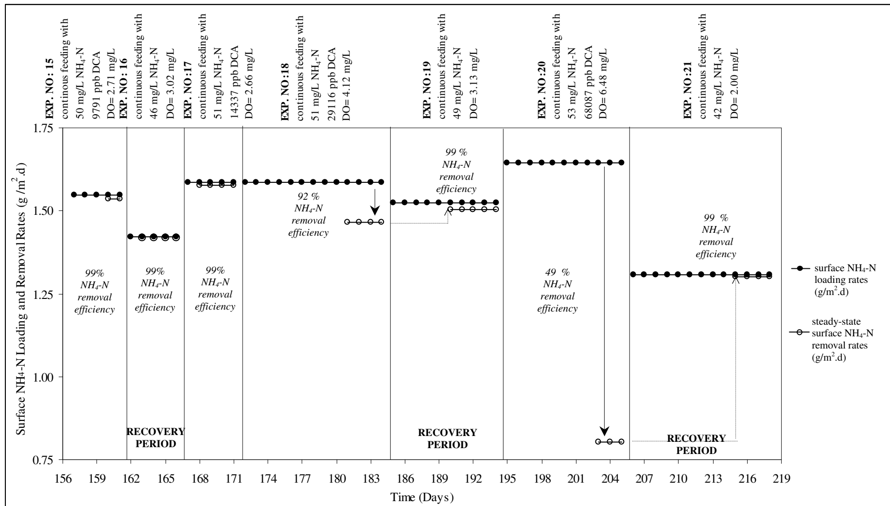
Figure 6.58. Chronological illustration of \text{NH}_4\text{-N} loading and removal rates in the 2 nd set of experiments [influent \text{NH}_4\text{-N} = 42-53 mg/L , influent 1,2-DCA=9791-68087 \mu\text{g/L} ]
