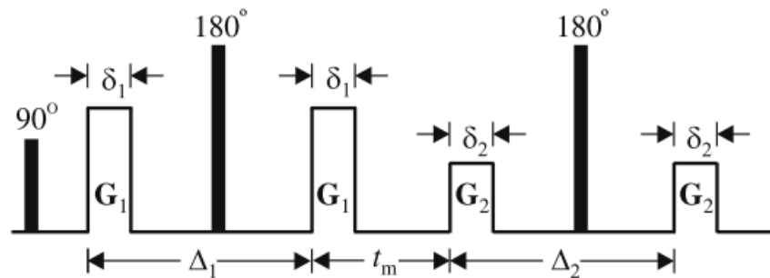
Figure 1.10. Spin echo version of the double-PFG pulse sequence which consists of two PFG blocks G_1 , and G_2 with the duration of \delta_1 and \delta_2 respectively separated by a mixing time t_m . The time between gradient pairs in each block is denoted as diffusion periods, namely, \Delta_1 and \Delta_2 [4].
