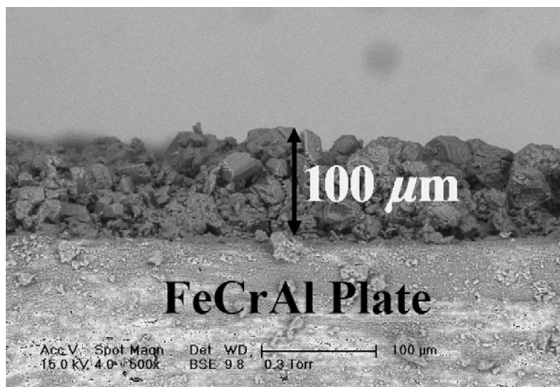
Figure 5.17. Lateral SEM image of a plate coated with Rh/ \delta\text{-Al}_2\text{O}_3 catalyst before reduction (500× magnification at 15 kV).
