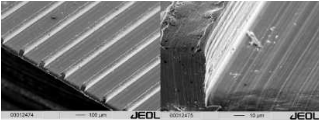
Figure 2.6. SEM of linear microchannels in stainless steel, generated by mechanical micromachining. The channels are about 200\ \mu\text{m} wide and 70\ \mu\text{m} deep. Right: SEM detail of the photo left [40].
