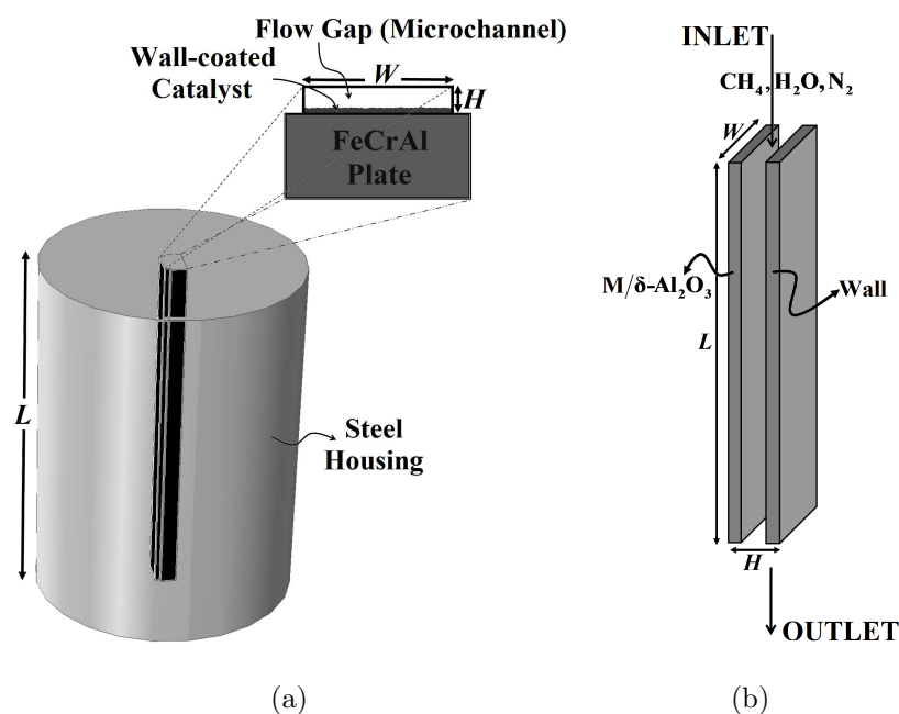
Figure 3.3. (a) Orthographic drawing of the steel housing and the microchannel used in the SRM experiments, (b) details of the catalytic microchannel configuration ( M = \text{Ni}, \text{Rh}, \text{Ru}, \text{Pt} ).
