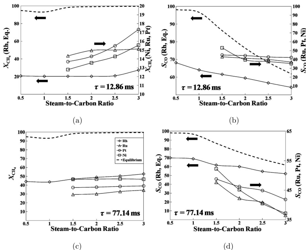
Figure 5.24. Variations of (a), (c) conversions of methane, and (b), (d) CO selectivities with steam-to-carbon ratio in the microchannel reactor ( T = 750^\circ\text{C} ). The residence times are (a), (b) \tau = 12.86 ms, and (c), (d) \tau = 77.14 ms. The legend is common to all. Left and right arrows designate the left and right ordinates, respectively.
