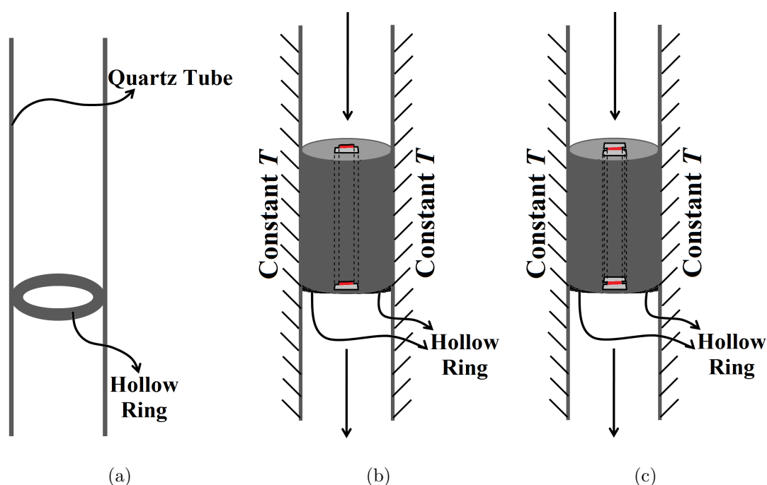
Figure 3.5. (a) The hollow ring inside the quartz tube, the microchannel reactor arrangement inside the quartz tube (b) for steam and (c) autothermal reforming of methane.
