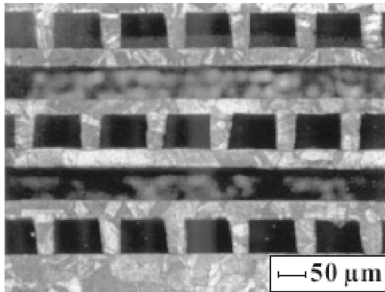
Figure 2.5. Cut view of a stack of microstructured plates of a cross-flow heat exchanger [38].
