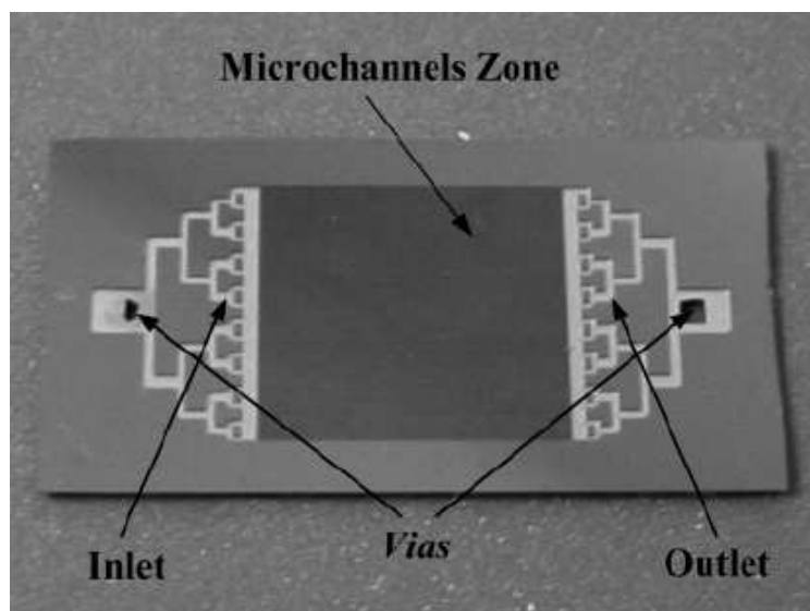
Figure 2.22. Typical silicon microreactor ( 3.1\text{ cm} \times 1.6\text{ cm} ) containing 239 channels, 25\text{ }\mu\text{m} wide and 100\text{ }\mu\text{m} deep, used for FT synthesis [225].
