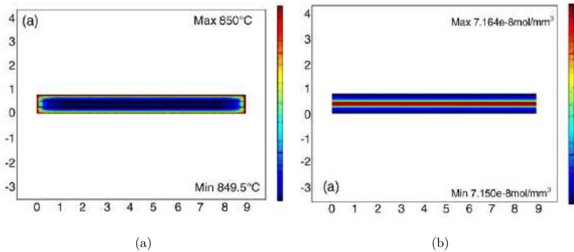
Figure 2.18. (a) Temperature distribution in SRM microchannel reactor (b) Methane concentration profile at z = 2.54 mm [207].
