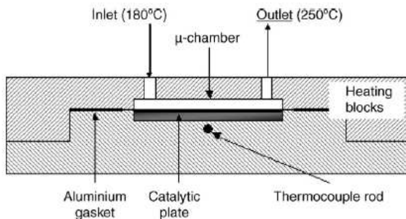
Figure 2.21. Micro-chamber test reactor for stainless steel supported catalysts [223].
