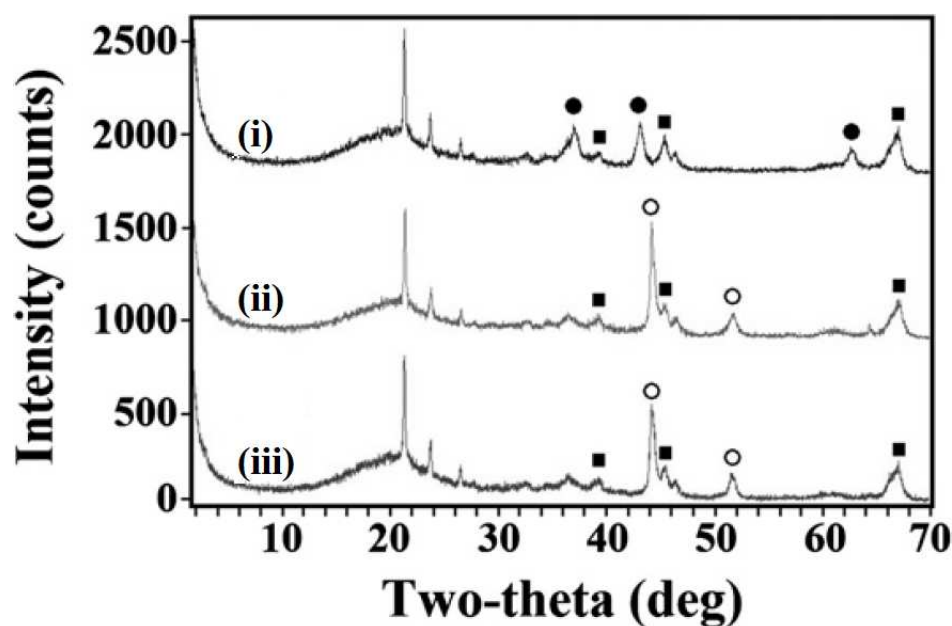
Figure 5.18. XRD patterns for the (i) calcined, (ii) calcined and reduced, and (iii) calcined, reduced and reacted Ni catalysts coated on plates ((■) \text{Al}_2\text{O}_3 , (●) \text{NiO} , (○) \text{Ni}^0 ).
