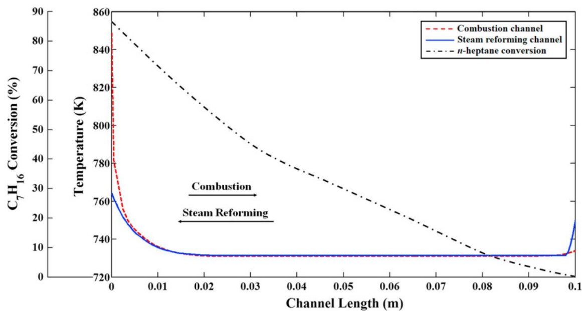
Figure 5.10. Simulation results of the methane combustion- n -heptane steam reforming coupling in the microchannel configuration.
