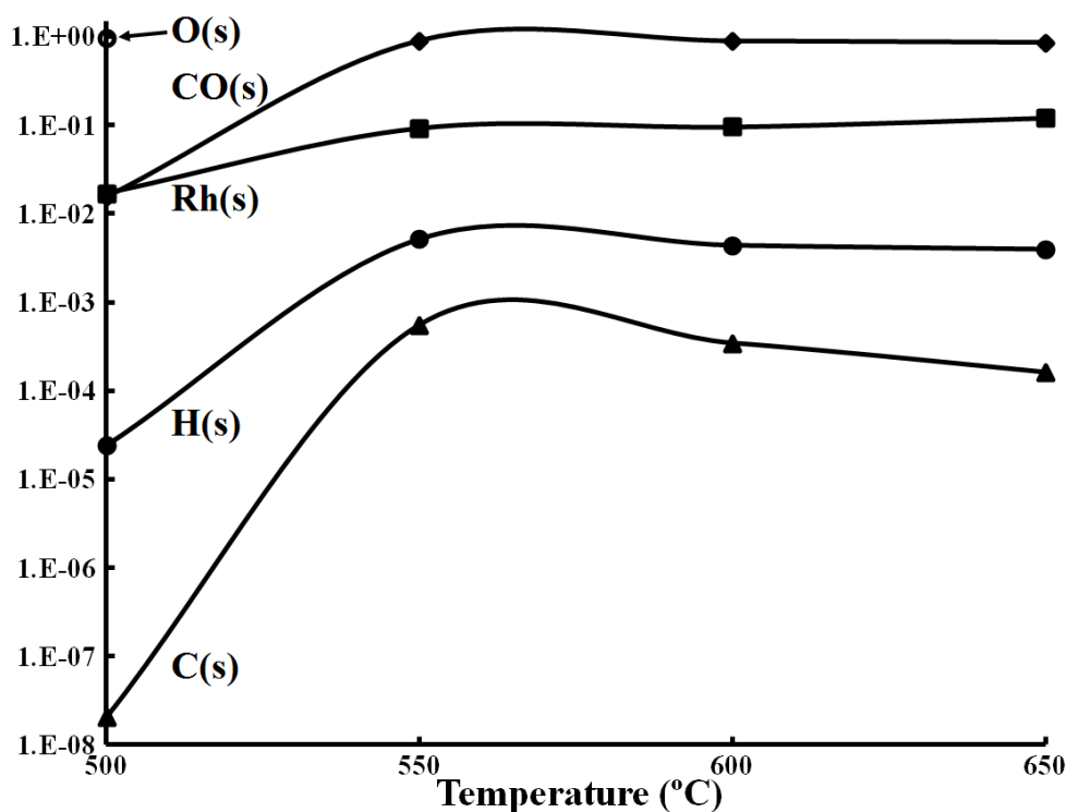
Figure 5.29. Surface coverages of CO, H and C as functions of the reaction temperature ( \tau = 12.86 ms, S : C = 3.0, O 2 : C = 0.47).
