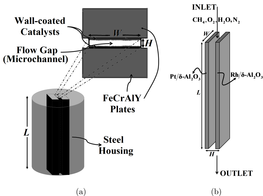
Figure 3.4. (a) Orthographic drawing of the steel housing and the microchannel used in methane ATR, (b) details of the catalytic microchannel configuration.
