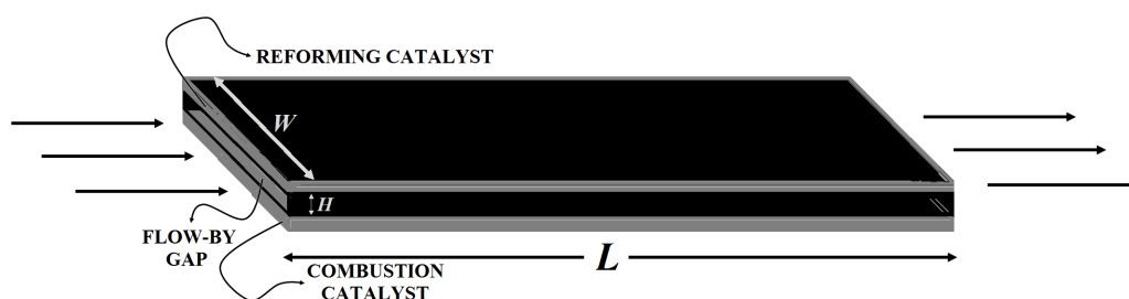
Figure 4.7. Schematic of the microchannel reactor used in methane ATR.
