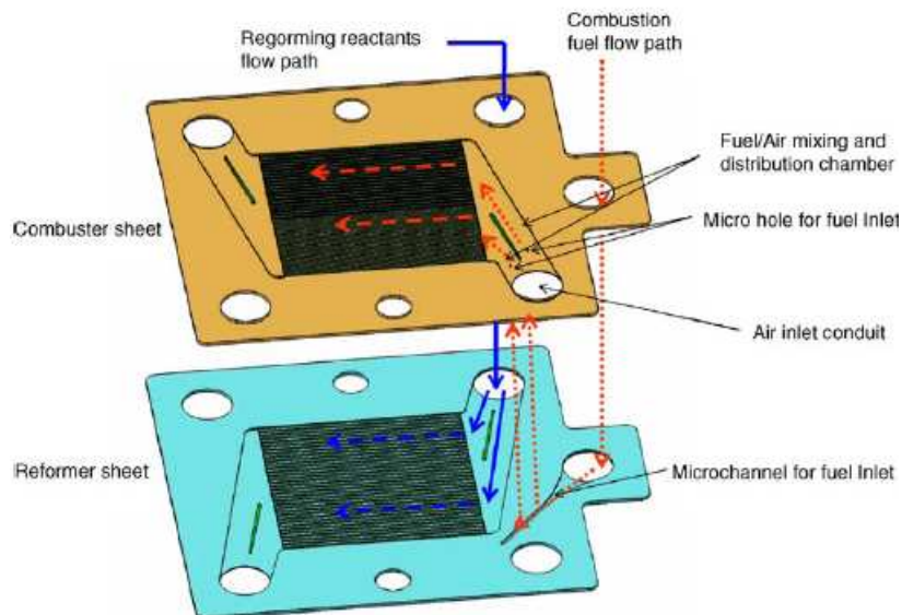
Figure 2.29. Schematic representation of the novel microchannel sheets and flow paths. Red dotted line: fuel for combustion flow path; red dashed line: fuel/air mixture and combustion off-gas flow path; blue solid line: reforming reactants flow path; blue dashed line: reformat flow path [13].
