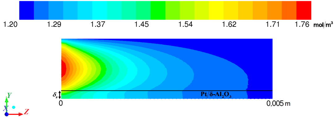
Figure 5.32. 2D plot of methane concentration in the \text{Pt}/\delta\text{-Al}_2\text{O}_3 catalyst between z = 0 and z = 5 \times 10^{-3} \text{ m} (no gradients in the x -direction).
