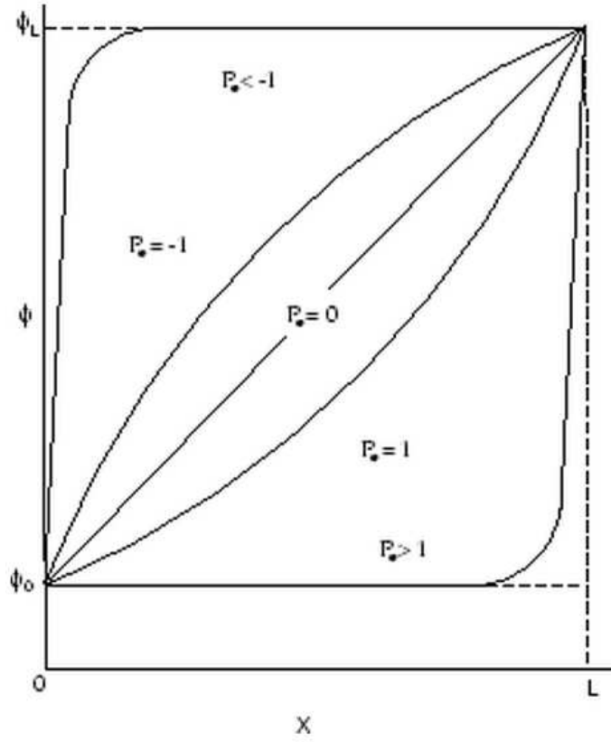
Figure 4.15. Variation of \phi between x = 0 and x = L for a one-dimensional convection-diffusion problem [295].
