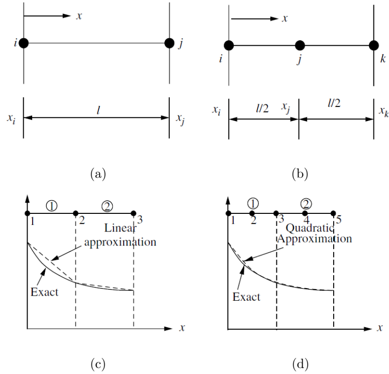
Figure 4.12. One dimensional finite elements. (a) A linear element, (b) a quadratic element, (c) linear and (d) quadratic variation of field variable \phi over an element, \circ —Element. \bullet —Node [291].
