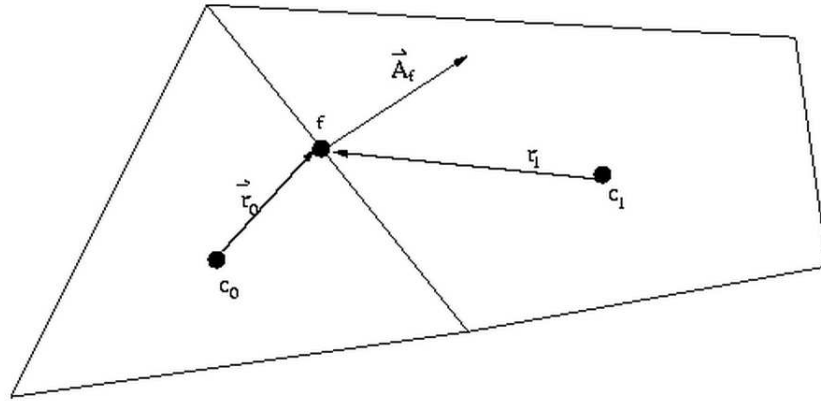
Figure 4.14. Control volume used to illustrate discretization of a scalar transport equation [295].
