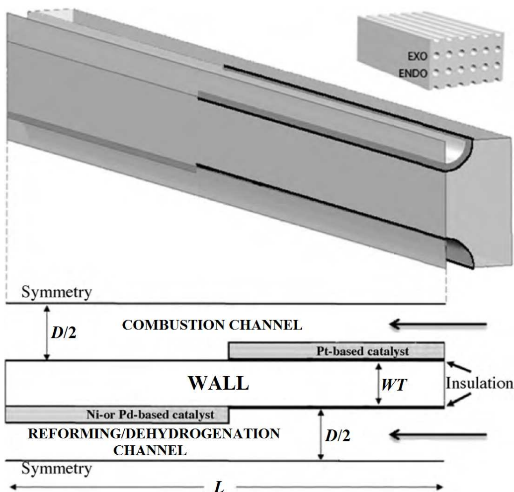
Figure 4.6. Description of the microchannel configuration used in combustion-steam reforming and combustion-dehydrogenation couplings.
