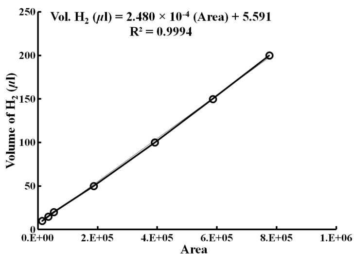
Figure B.2. GC calibration curve for hydrogen.
