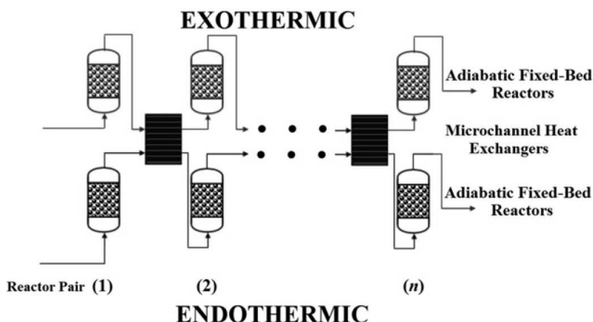
Figure 4.8. Description of the cascade reactor configuration.
