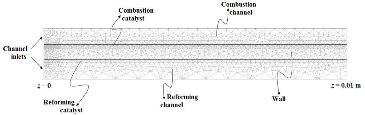
Figure 5.1. The first one-tenth of the computational grid used in the simulation of the parallel microchannel reactor for coupling of combustion and steam reforming of propane ( SL = 560 \mu\text{m} , WT = 200 \mu\text{m} ).
