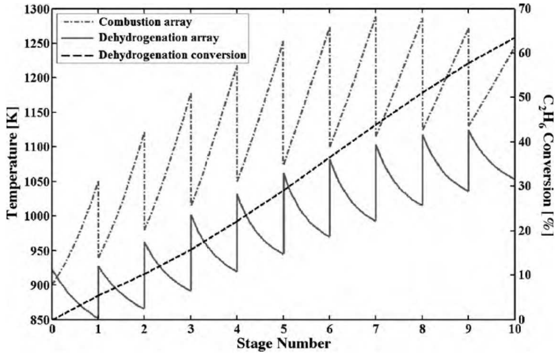
Figure 5.15. Simulation results of coupling of methane combustion and ethane dehydrogenation in the cascade configuration.
