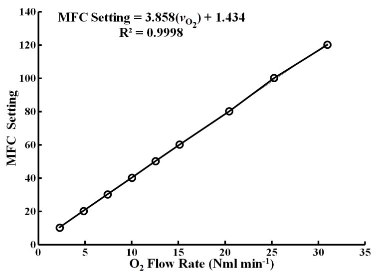
Figure A.4. Calibration curve of the dry air mass flow controller for oxygen.
