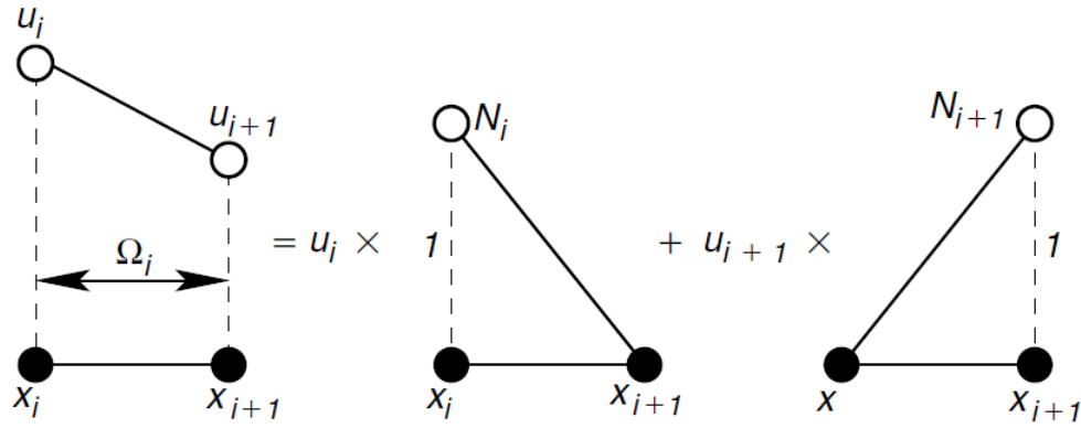
Figure 4.11. Shape functions for the finite element method [290].
