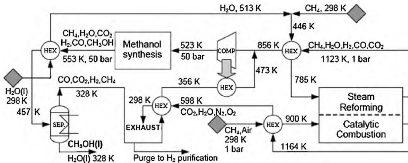
Figure 4.2. Process flow diagram of methanol production.
