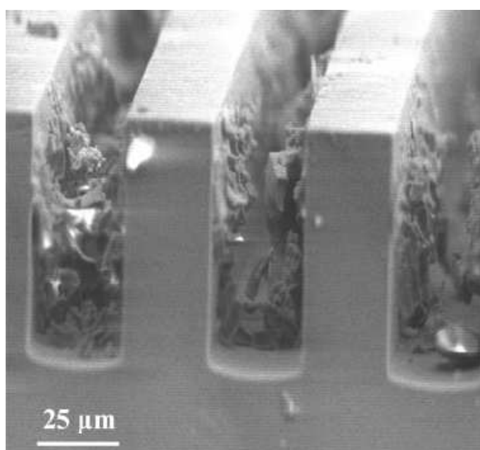
Figure 2.23. SEM image of silica-supported Fe-Co catalyst deposited in 25\text{ }\mu\text{m} wide and 100\text{ }\mu\text{m} deep microchannels [225].
