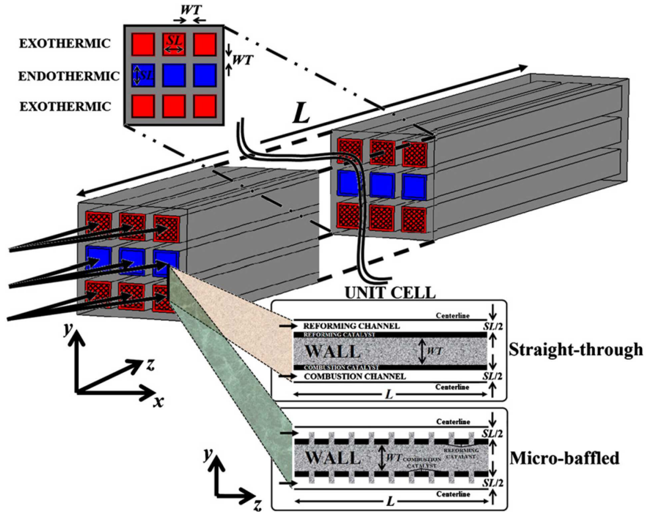
Figure 4.4. Depiction of the parallel microchannel reactor, the unit cell (lower inset) used in the 2D mathematical model and cross-sectional view of the microchannels (upper inset).
