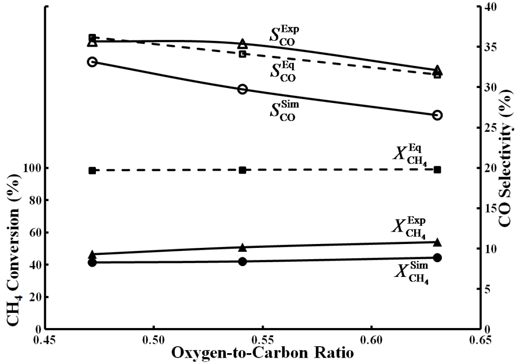
Figure 5.31. Variation of experimental and simulated CO selectivity with the oxygen-to-carbon ratio at the inlet ( \tau = 12.86 ms, T = 650^\circ\text{C} , S : C = 3.0 ).
