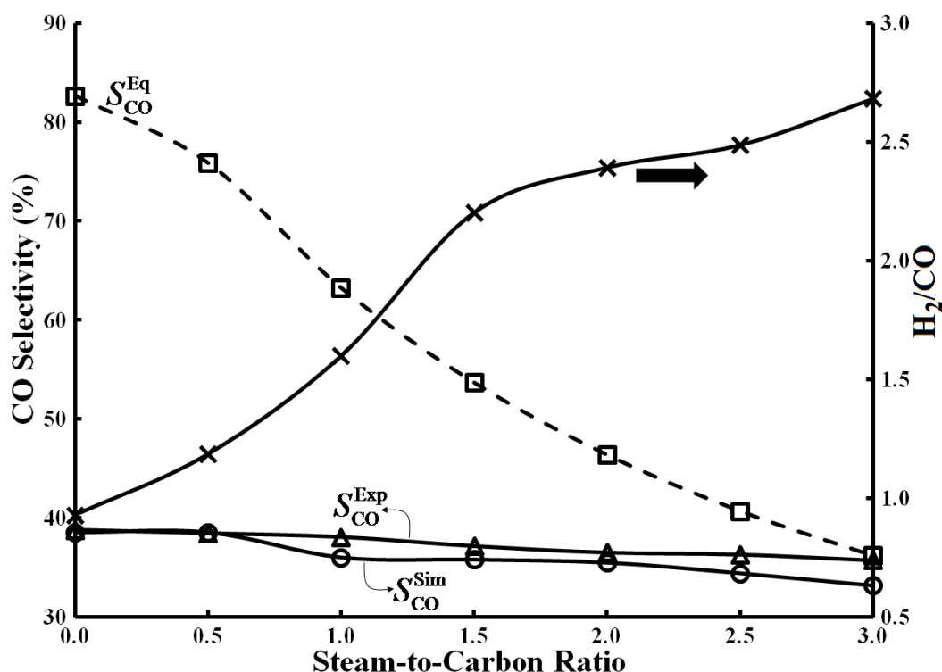
Figure 5.30. Variation of experimental and simulated CO selectivity with the steam-to-carbon ratio at the inlet ( \tau = 12.86 ms, T = 650^\circ\text{C} , O_2 : C = 0.47 ).
