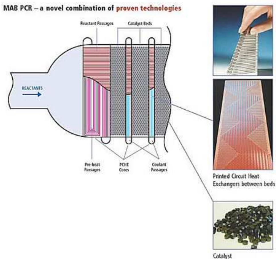
Figure 2.32. Schematic representation of catalyst bed and PCHE arrangement ( www.heatric.com )
