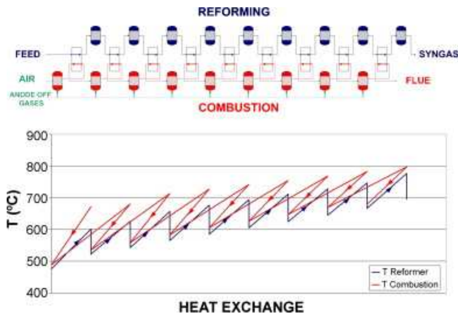
Figure 2.33. Saw-tooth pattern for the temperature profile in the reforming and combustion module [24]
