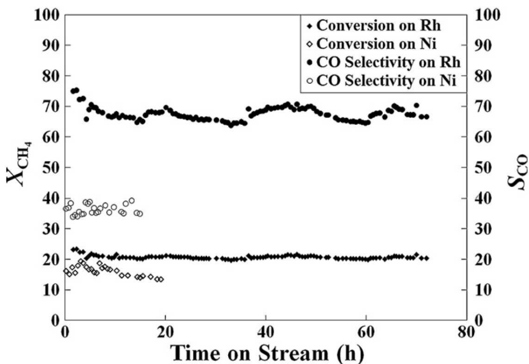
Figure 5.20. Time-on-stream methane conversion and CO selectivity on Rh/ \delta -Al 2 O 3 and Ni/ \delta -Al 2 O 3 in the microchannel reactor configuration. Operating conditions: T = 750^{\circ}\text{C} , \tau = 12.86 ms, S : C = 0.5 (Rh), S : C = 3.0 (Ni).
