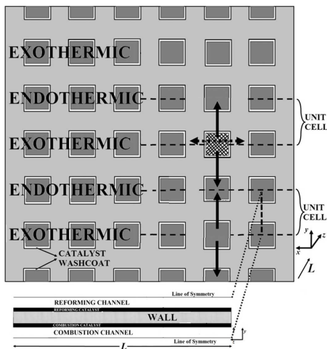
Figure 4.5. Frontal view of the microchannel array shown in Figure 4.4.
