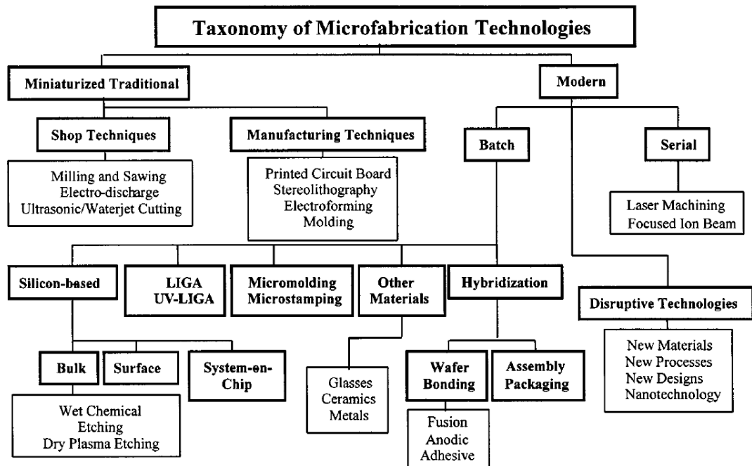
Figure 2.1. Taxonomic chart of microfabrication technologies [31].
