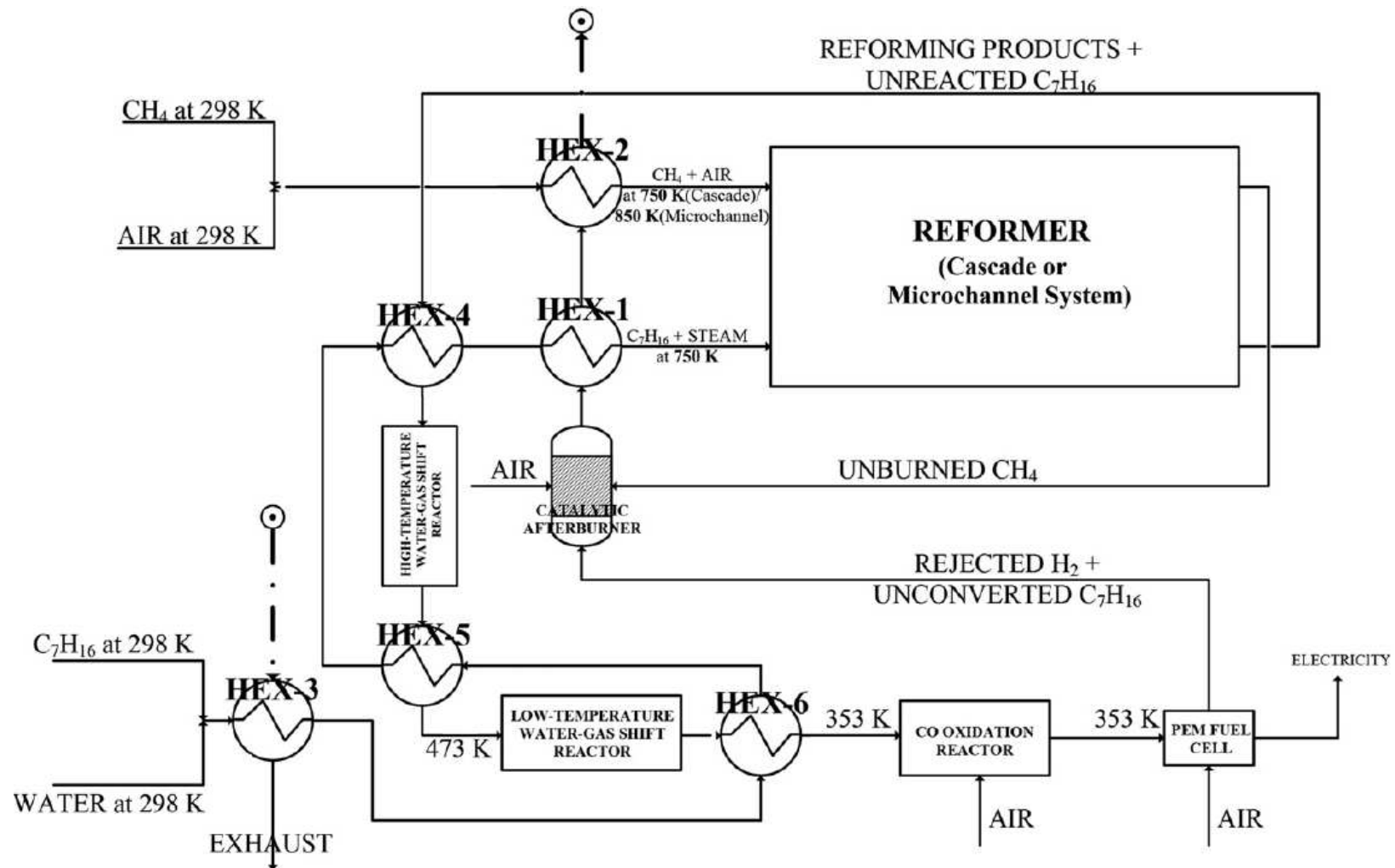
Figure 4.1. Process flow diagram of the fuel processor/PEM fuel cell assembly.
