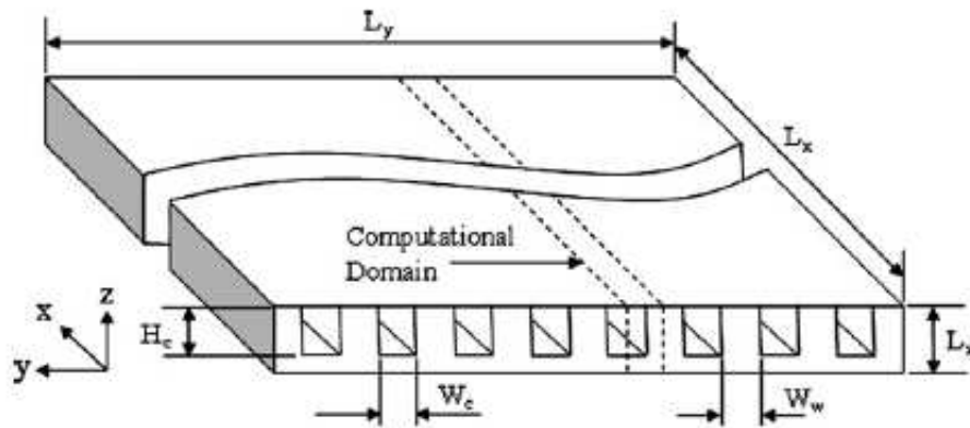
Figure 2.13. Microchannel heat sink with water flowing as the cooling fluid.
