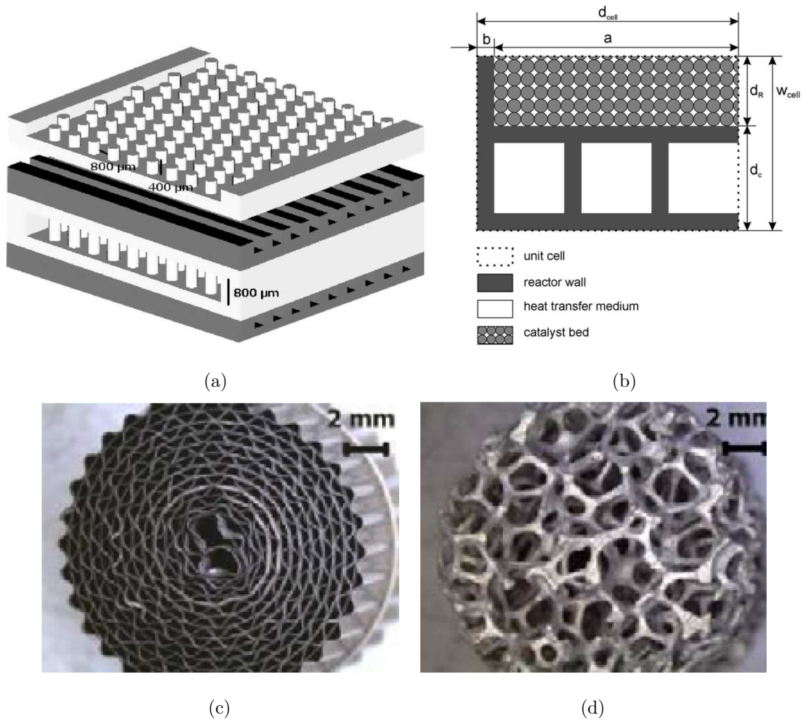
Figure 2.26. (a) Pillar structured catalyst foils and the cross-flow rectangular oil channels [227] (b) Milli-structured fixed-bed slit reactor [226] (c) Micromonolith (FeCrAlY) and (d) Foam (aluminum) reactors [228].
