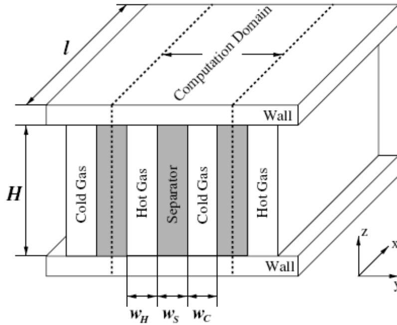
Figure 2.12. Counter-current heat transfer in alternating rectangular microchannels [57].
