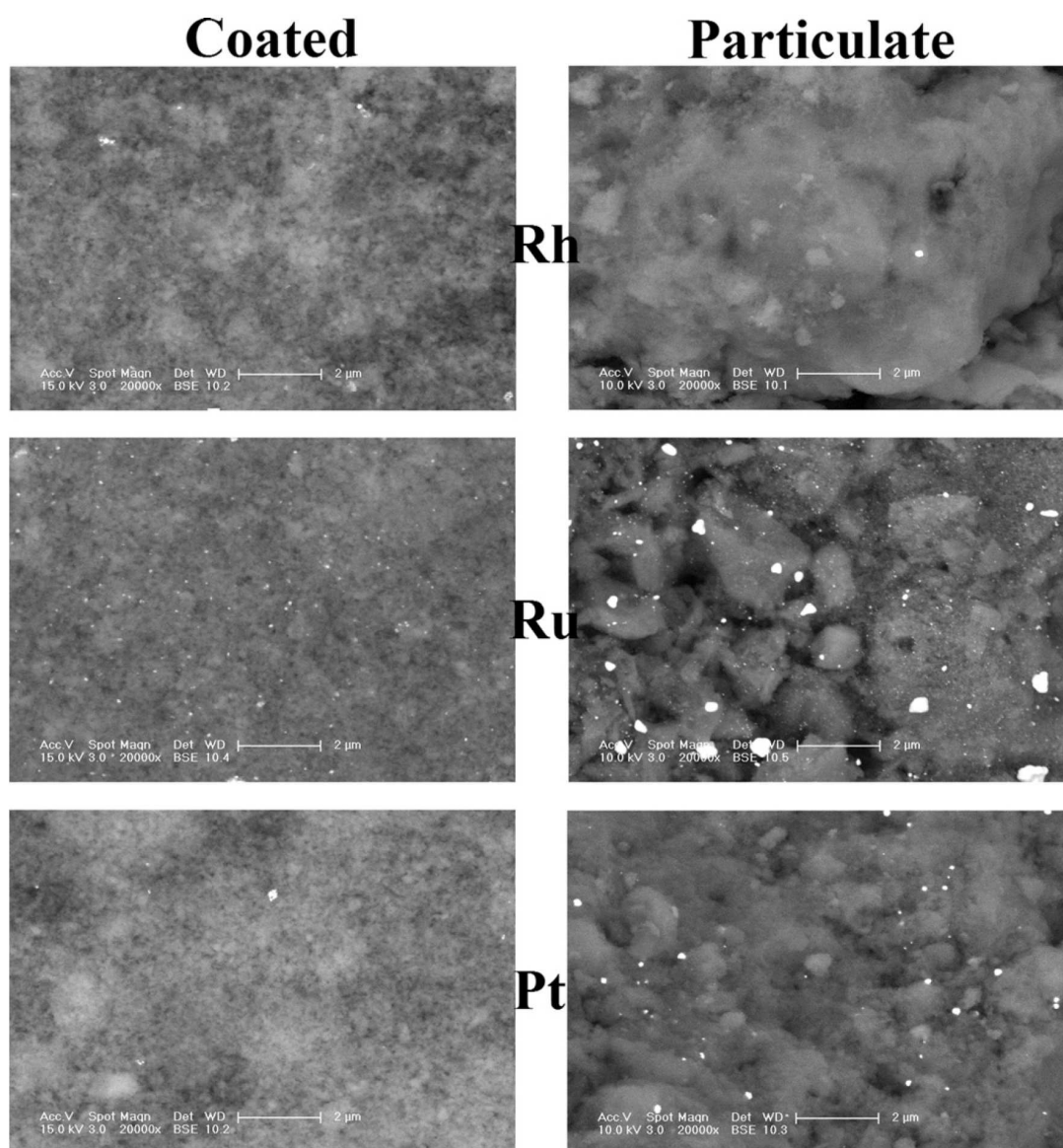
Figure 5.19. Backscattering electron (BSE) SEM micrographs of Rh, Ru and Pt on coated and particulate catalysts at 20000 \times magnification.
