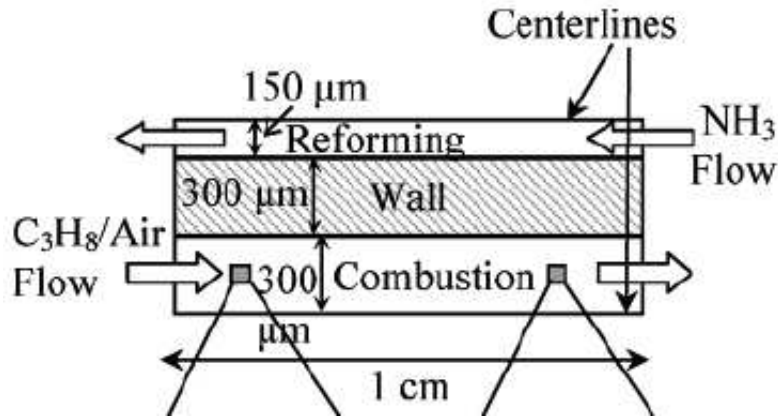
Figure 2.30. Schematic of a multifunctional microreformer/microcombustor device [15].
