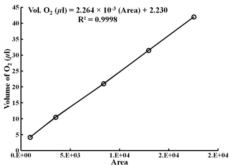
Figure B.4. GC calibration curve for oxygen.
