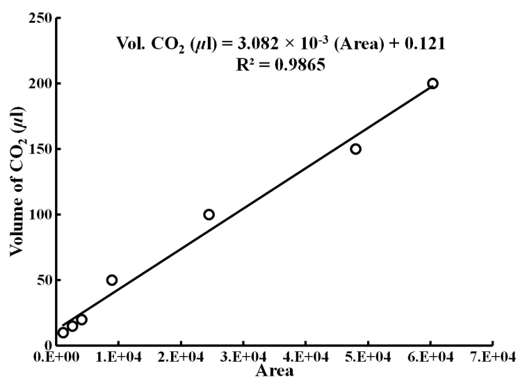
Figure B.6. GC calibration curve for carbon dioxide.
