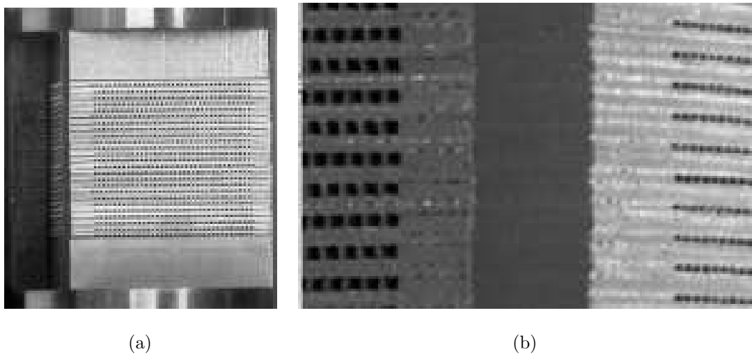
Figure 2.7. (a) Stacked metal foils (b) microstructured plates after diffusion bonding [40].
