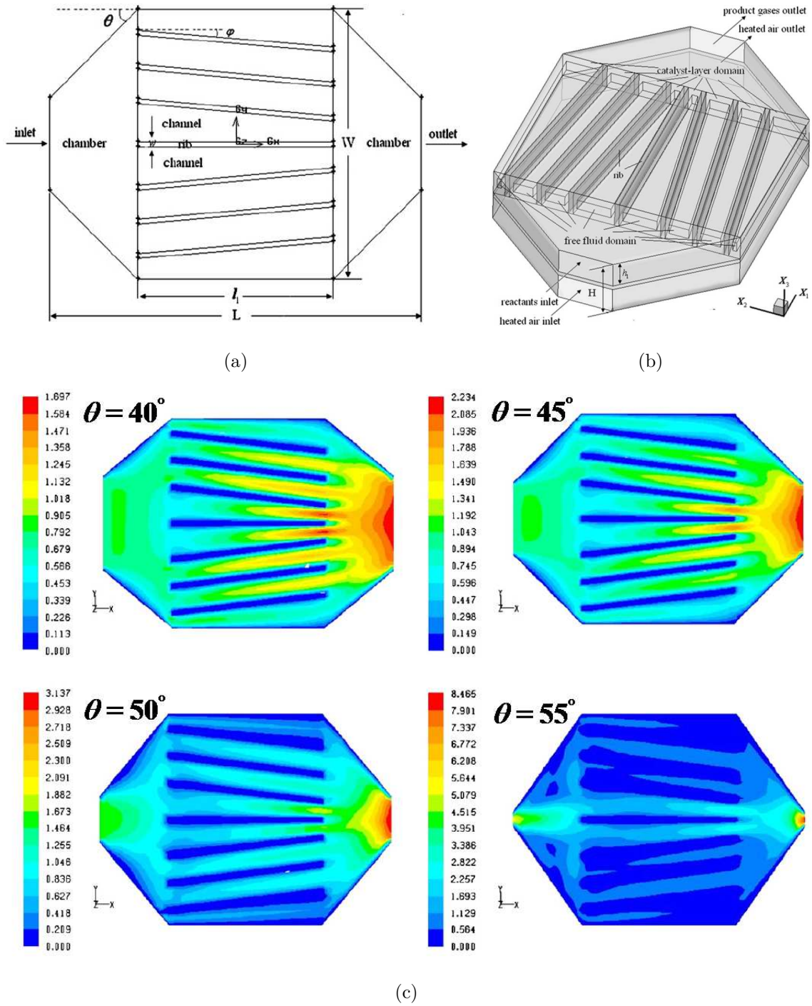
Figure 2.19. (a) 2D and (b) 3D schematic diagrams of the microreactor (c) Velocity distributions under different entrance angles \theta [218].
