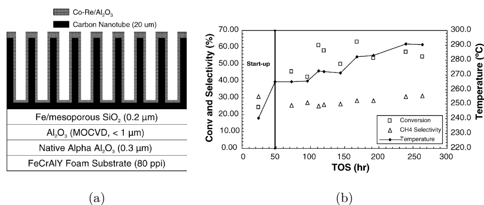
Figure 2.20. (a) Schematic and (b) performance of the microstructured catalyst based on carbon nanotube arrays for FT synthesis [222].
