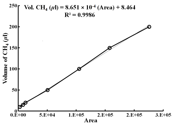
Figure B.1. GC calibration curve for methane.
