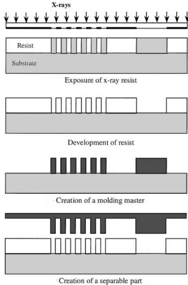
Figure 2.4. The LIGA process [31].
