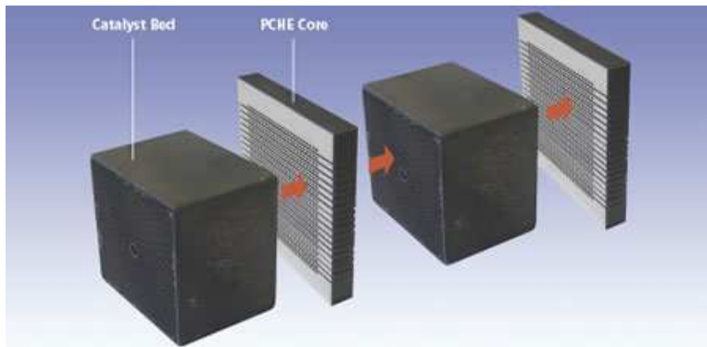
Figure 2.31. Assembly of adiabatic beds and PCHEs ( www.heatric.com ).
