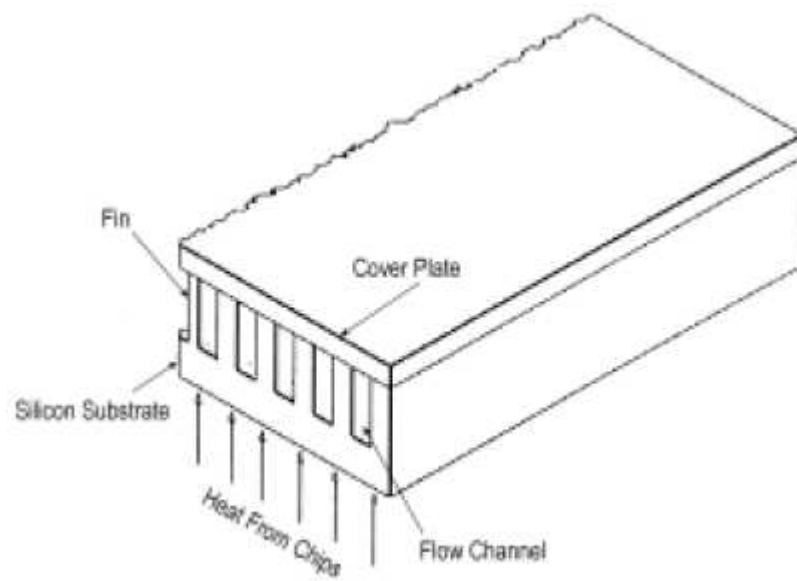
Figure 2.11. General structure of a microchannel heat sink.
