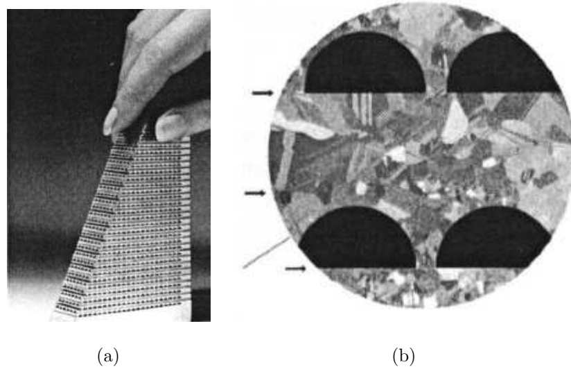
Figure 2.8. (a) Cross section of PCHE stack (b) photomicrograph of channel cross section [43].
