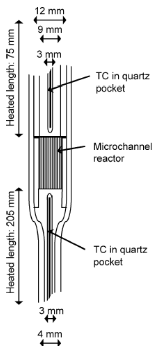
Figure 2.15. Schematic drawing of the quartz reactor loaded with microchannel monolith [193].
