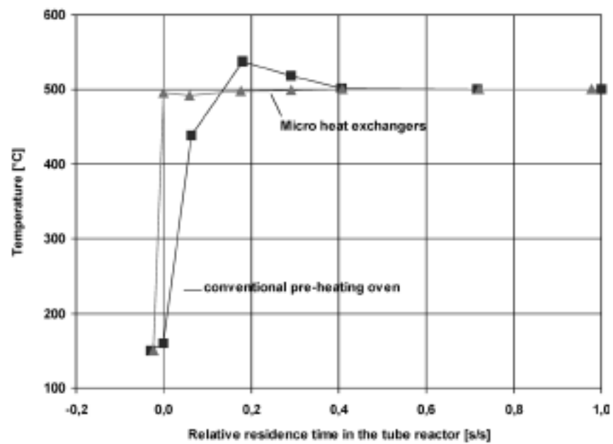
Figure 2.10. Performance comparison of preheating with conventional and microstructured heat exchangers [53].
