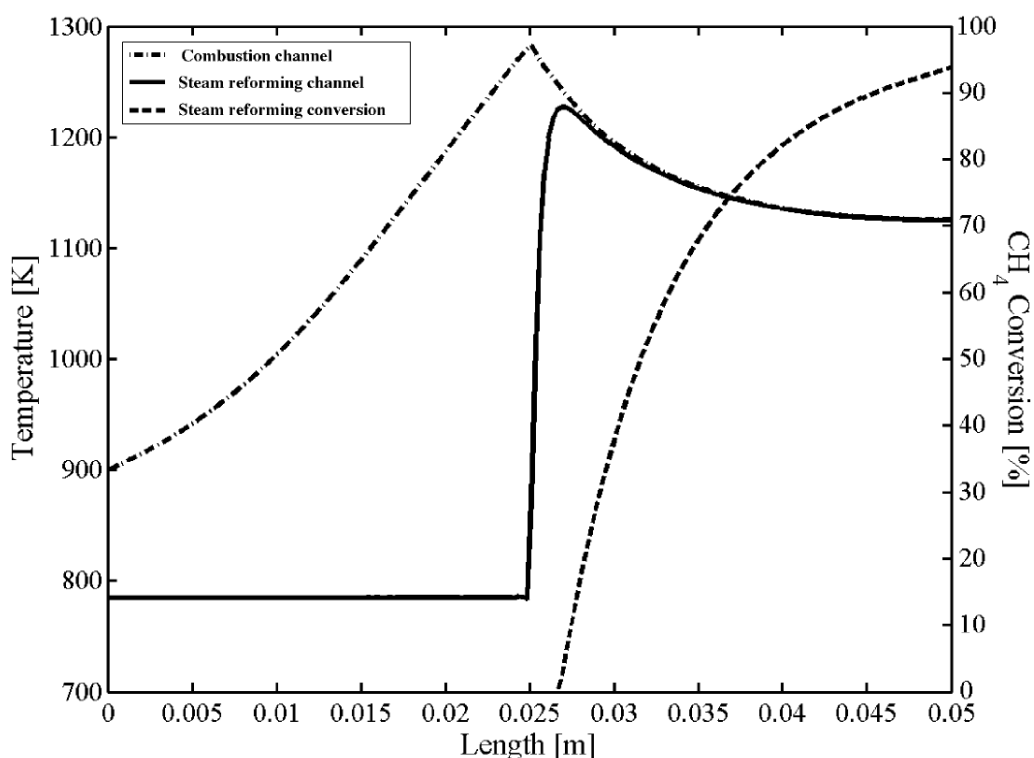
Figure 5.12. Simulation results of coupling of combustion and steam reforming of methane in the microchannel configuration.
