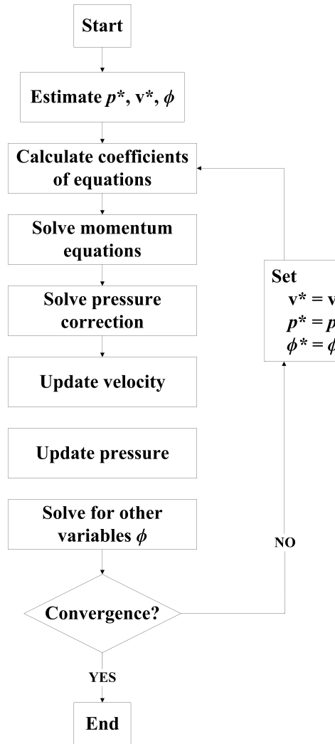
Figure 4.17. Flowchart of the SIMPLE algorithm.
