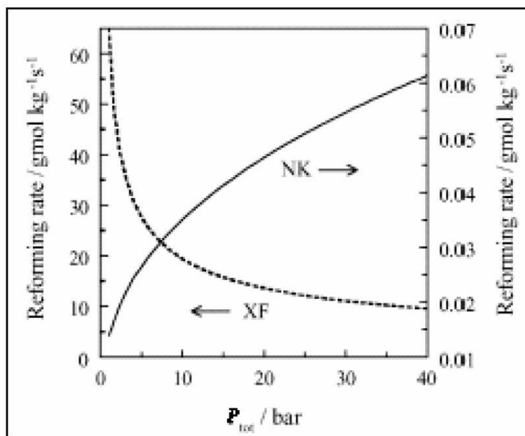
Figure 2.14. SRM rates calculated by XF and NK kinetic models versus total pressure [137].
