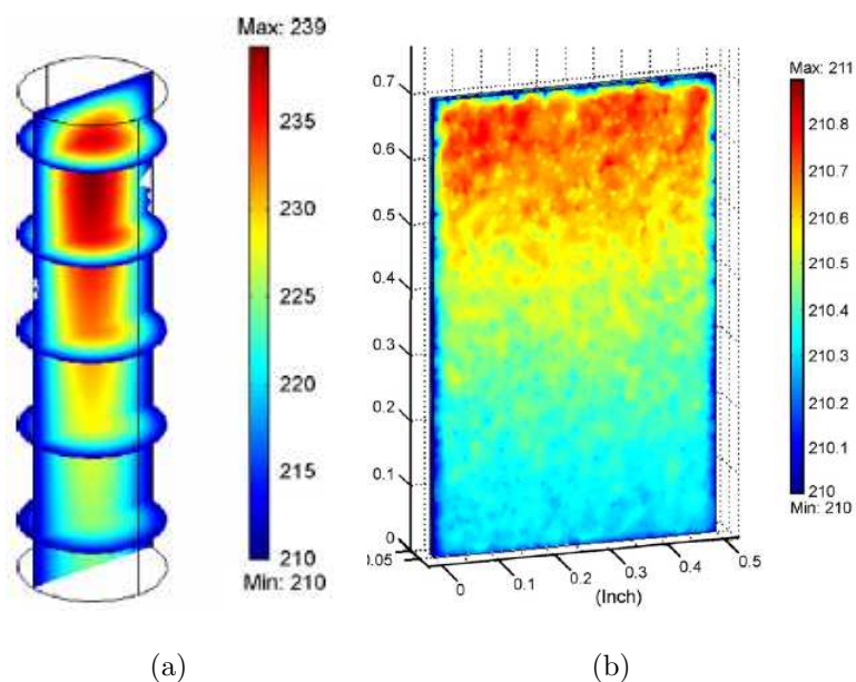
Figure 2.27. (a) Temperature profiles in a conventional tubular reactor for FTS. Overall CO conversion is 62% (b) Temperature profiles in a microchannel reactor for FTS. Overall CO conversion is 50% (In both cases, P = 20 atm, reactor wall temperature at 210^{\circ}\text{C} , \text{H}_2 : \text{CO} = 2.0 , \text{GHSV} = 18,000 \text{ h}^{-1} ) [229].
