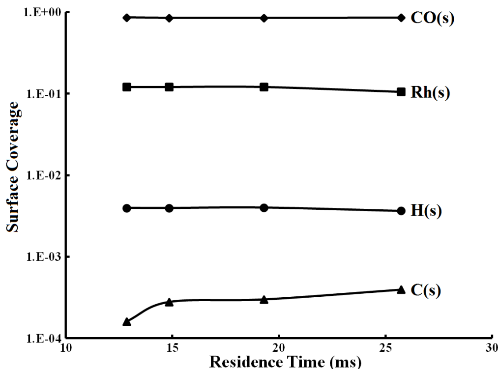
Figure 5.27. Surface coverages of CO, H and C as functions of the residence time ( T = 650^{\circ}\text{C} , \text{S} : \text{C} = 3.0 , \text{O}_2 : \text{C} = 0.47 ).
