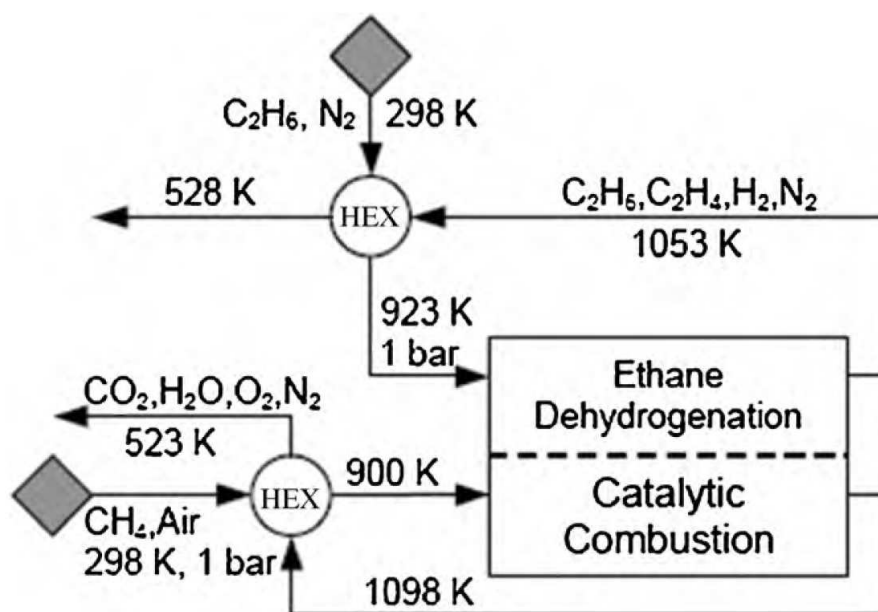
Figure 4.3. Process flow diagram of ethane dehydrogenation.
