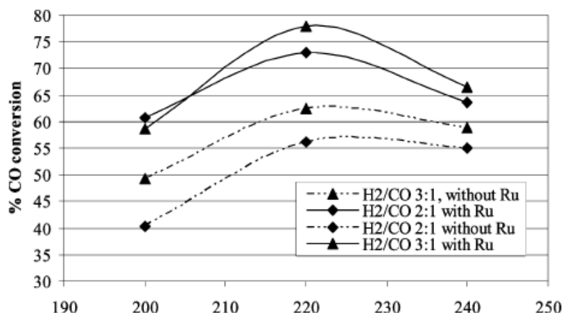
Figure 2.24. Comparative studies on CO conversion to alkanes at different temperatures and two H 2 : CO ratios, using silica-supported Fe-Co catalysts with and without Ru [225].
