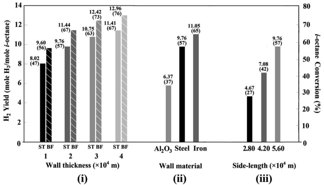
Figure 5.6. Hydrogen yields and iso -octane conversions (in parentheses) obtained for different (i) wall thickness, (ii) wall materials, and (iii) microchannel side lengths.
