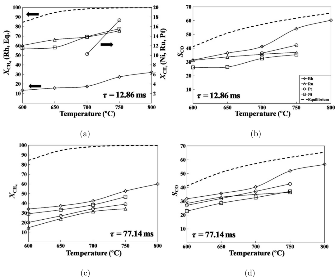
Figure 5.23. Variations of (a), (c) conversions of methane, and (b), (d) CO selectivities with temperature in the microchannel reactor ( S : C = 3.0 ). The residence times are (a), (b) \tau = 12.86 ms, and (c), (d) \tau = 77.14 ms. The legend is common to all. Left and right arrows designate the left and right ordinates, respectively.
