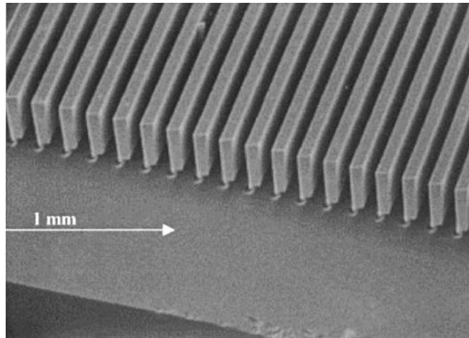
Figure 2.3. Microchannel array formed by dry ion etching [41].
