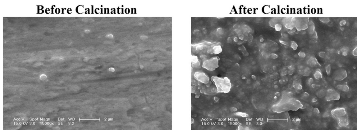
Figure 5.16. SEM micrographs of the uncoated plates before and after treatment at 900°C (500× magnification at 15 kV).
