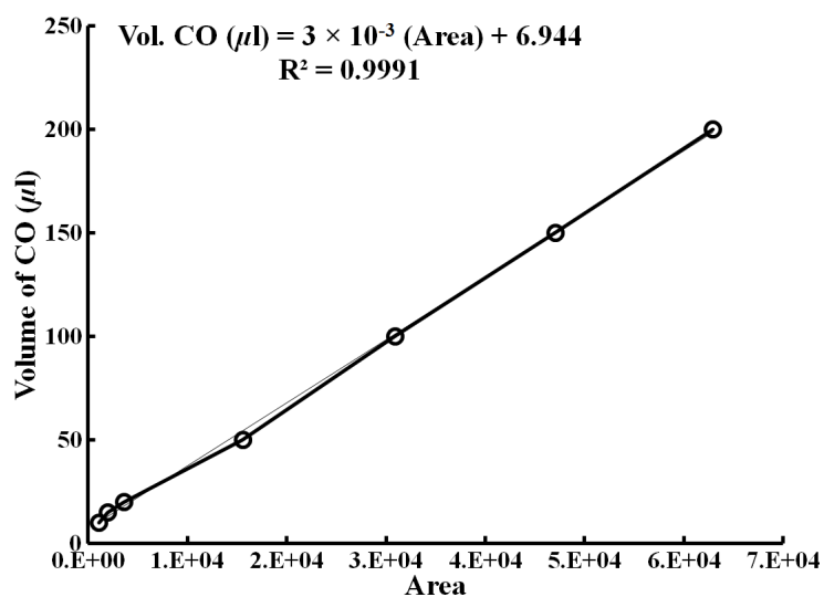
Figure B.5. GC calibration curve for carbon monoxide.
