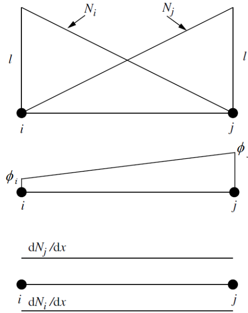
Figure 4.13. Variation of shape functions, \phi and derivatives within a linear element [291].
