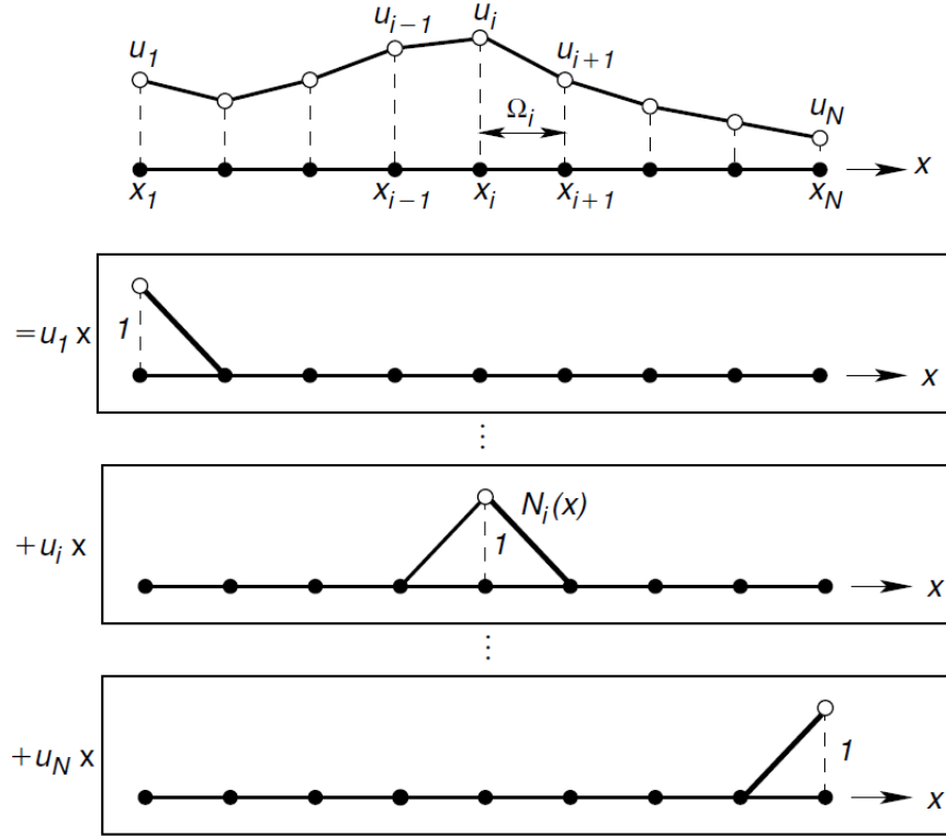
Figure 4.10. A piecewise linear approximation u^\delta(x, t) = \sum_{i=1}^N u_i(t) N_i(x) [290].
