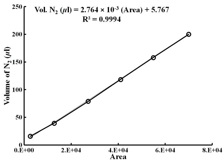
Figure B.3. GC calibration curve for nitrogen.
