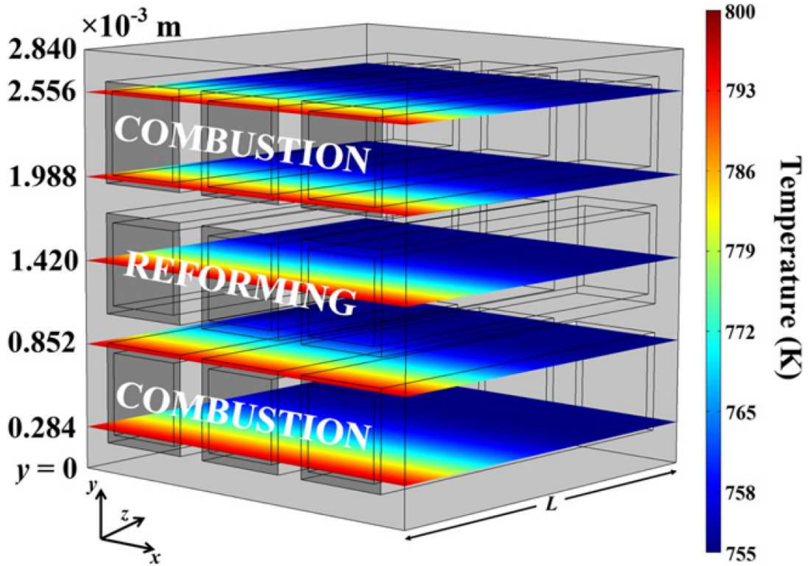
Figure 5.4. Temperature variation in x - and z -directions at different levels of y -coordinate for the base case ( SL = 5.6 \times 10^{-4} m, WT = 2 \times 10^{-4} m, material: AISI steel) using the 3D 9-channel model.
