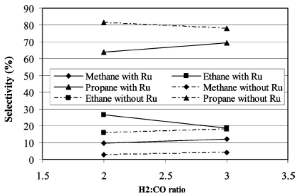
Figure 2.25. Selectivity to various alkanes at different H 2 : CO ratios using silica-supported Fe-Co catalysts with and without Ru [225].
