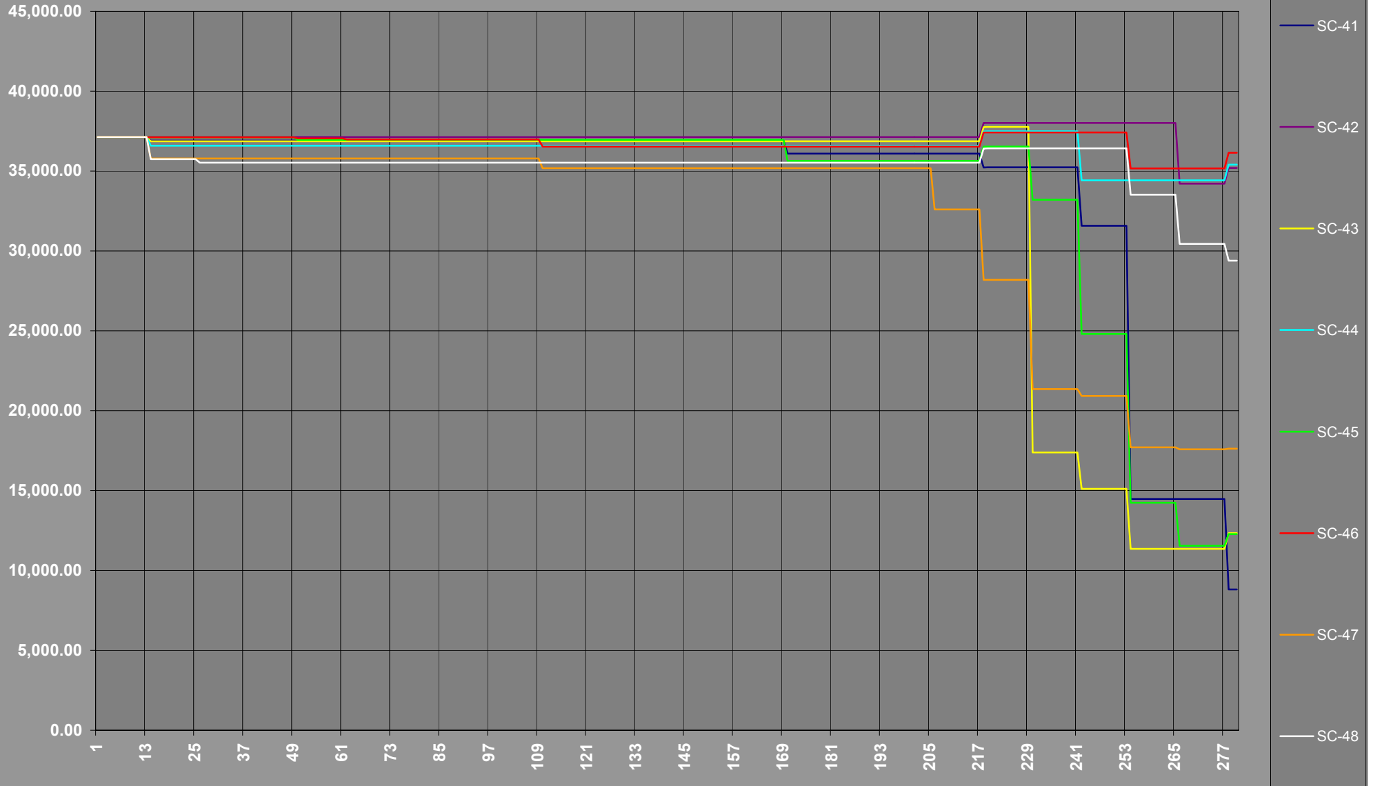
Restriction on New Plant Construction Based on Diesel Oil Reserve (MW)
