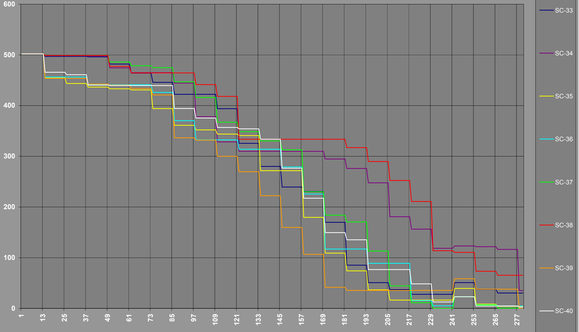
Restriction on New Plant Construction Based on Geothermal Reserve (MW)
