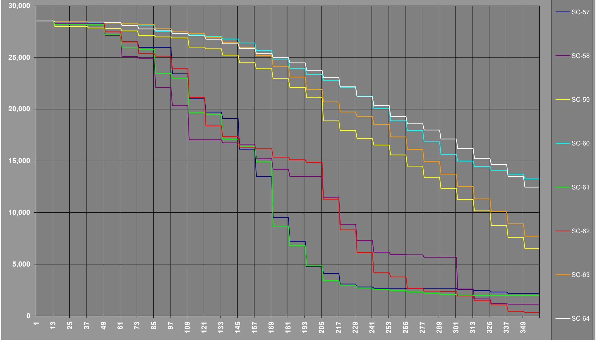
Restriction on New Plant Construction Based on Hydro Reserve (MW)
