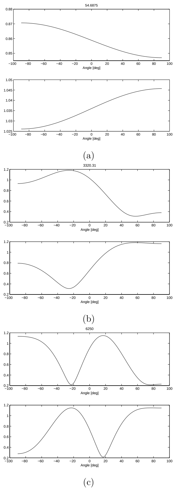
Figure 5.15. Directivity patterns for frequencies (a) 54 Hz (b) 3320 Hz (c) 6250 Hz
