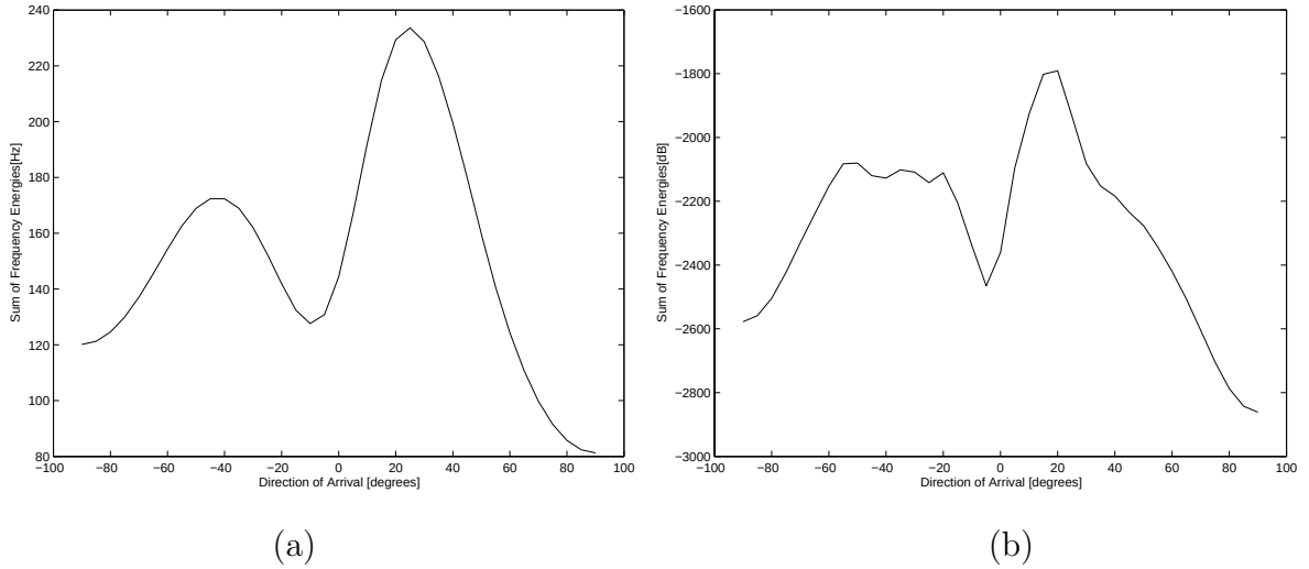
Figure 5.8. Sum of energies at each frequency bin (a) in [Hz] and (b) in [dB]
