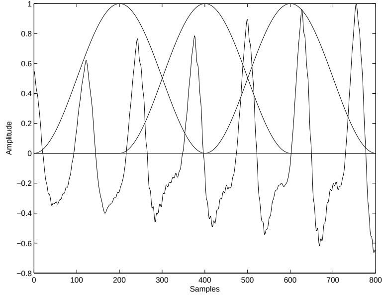
Figure 4.2. Overlapping Hanning window with length=400 samples
