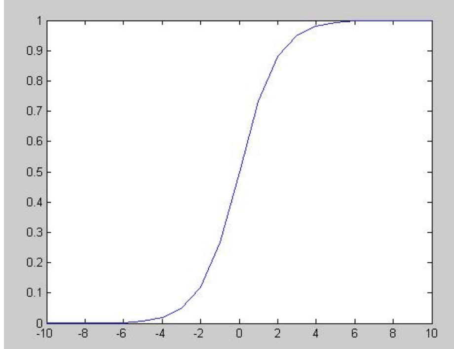
Figure 1.5 Sigmoid Function
