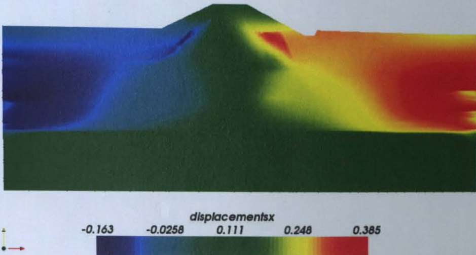
Figure 8 - 15: Horizontal displacements under seismic excitation at t = 20 seconds on the deformed shape of the structure. (meter).
