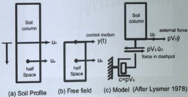
Figure 7 - 6: Effective seismic input model [44].
