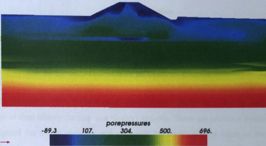
Figure 8 - 21: Pore pressures under seismic excitation at t = 30 seconds on the deformed shape of the structure. (kPa).
