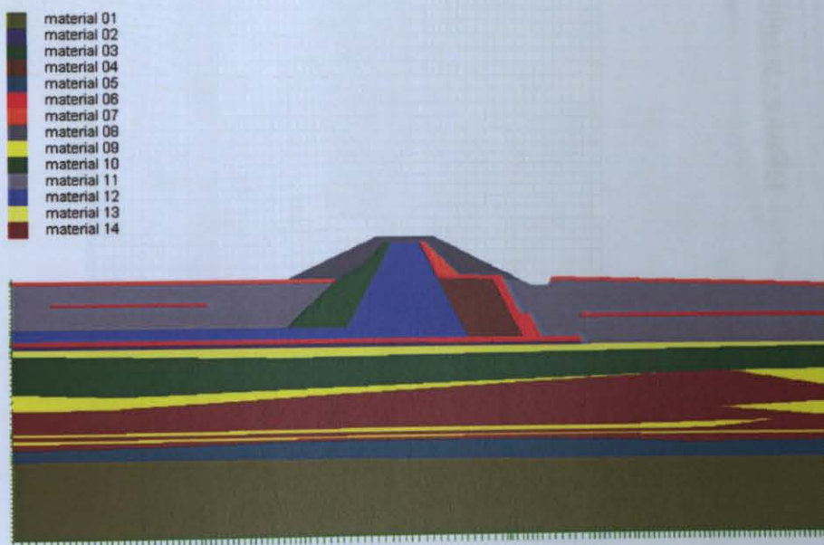
Figure 6 - 1: Cross-section of Alibey Dam according to its material properties.
