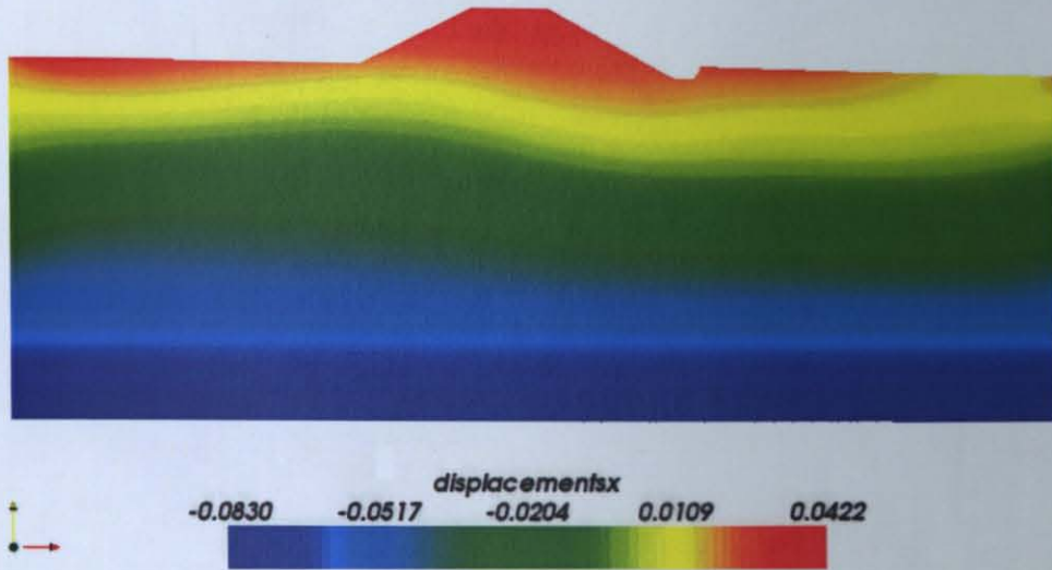
Figure 8 - 5: Horizontal displacements under seismic excitation at t = 30 seconds on the deformed shape of the structure. (meter).
