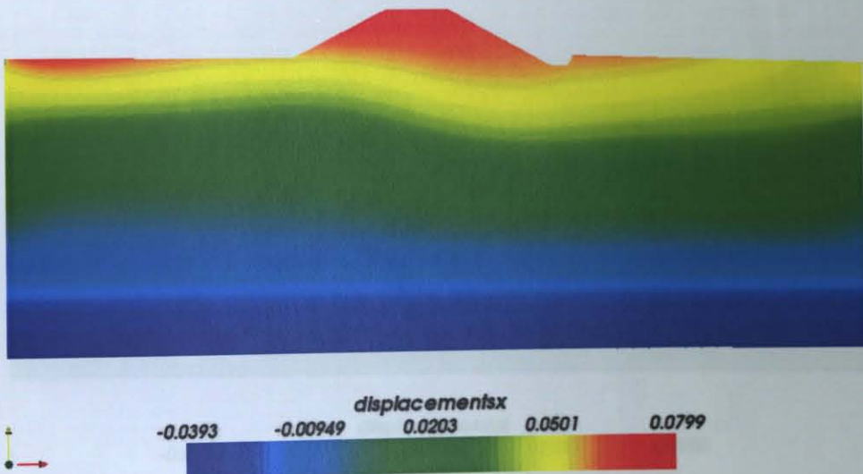
Figure 8 - 2: Horizontal displacements under gravity loads on the deformed shape of the structure. (meter).
