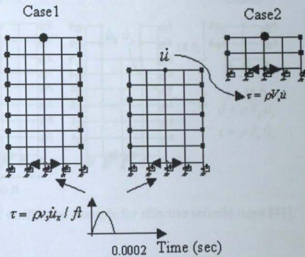
Figure 7 - 7: Effective seismic input verification example 1 [44].
