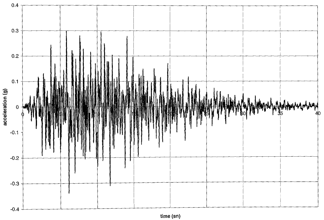
Figure 4 - 16: Acceleration time history plot.
