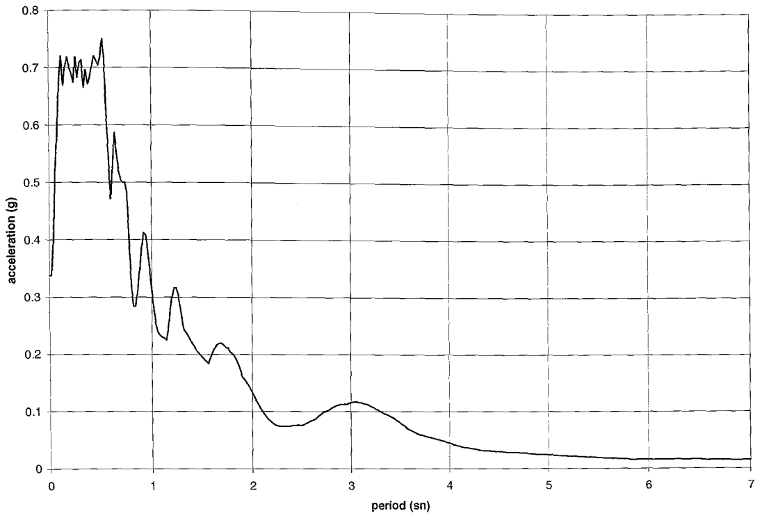
Figure 4 - 17: Acceleration response spectrum.
