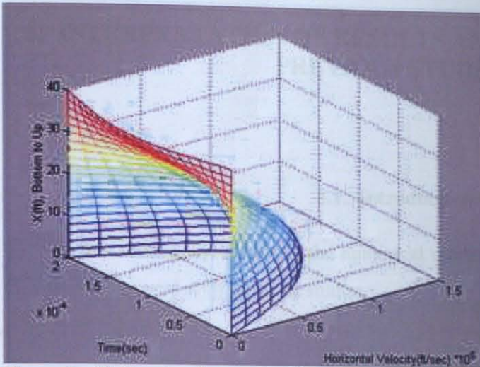
Figure 7 - 11: Results of second verification example for effective seismic input [44].
