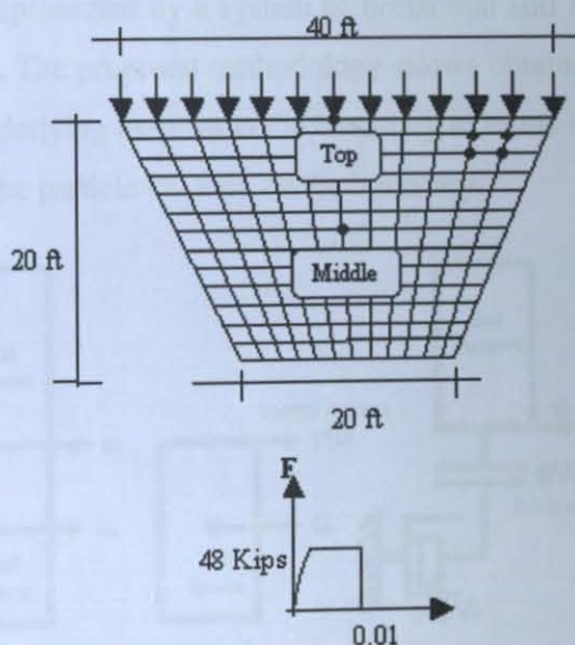
Figure 7 - 4: Second verification example [44].
