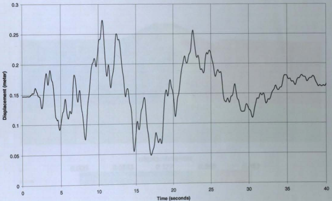
Figure 8 - 12: Dam's crest's horizontal displacements under seismic excitation.
