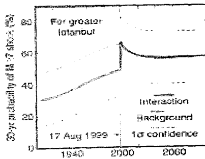
Figure 4 - 8: Probability for the occurrence of a M_w \geq 7.0 earthquake affecting Istanbul for the next 30 years [37].
