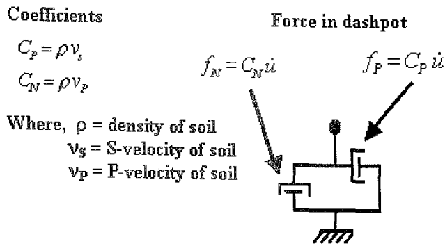
Figure 7 - 1: Energy absorption elements [44].
