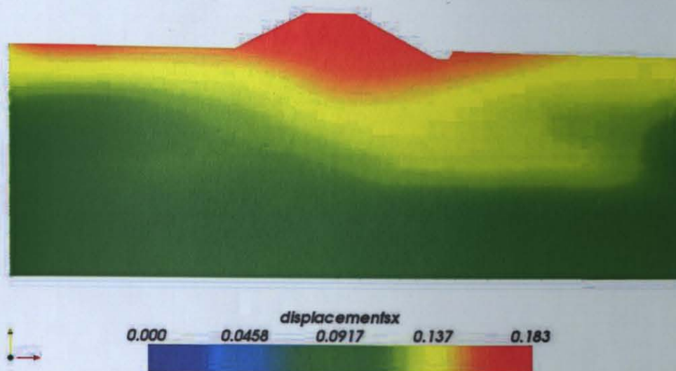
Figure 8 - 3: Horizontal displacements under seismic excitation at t = 10 seconds on the deformed shape of the structure. (meter).
