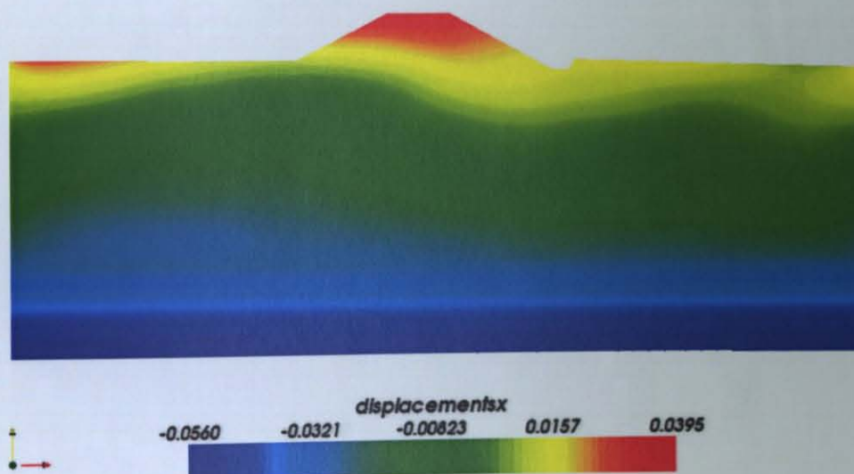
Figure 8 - 4: Horizontal displacements under seismic excitation at t = 20 seconds on the deformed shape of the structure. (meter).
