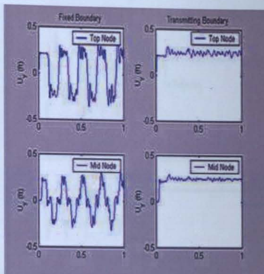
Figure 7 - 3: Results of the 1 st verification example [44].
