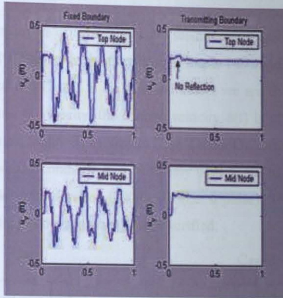
Figure 7 - 5: Results of the second verification example [44].
