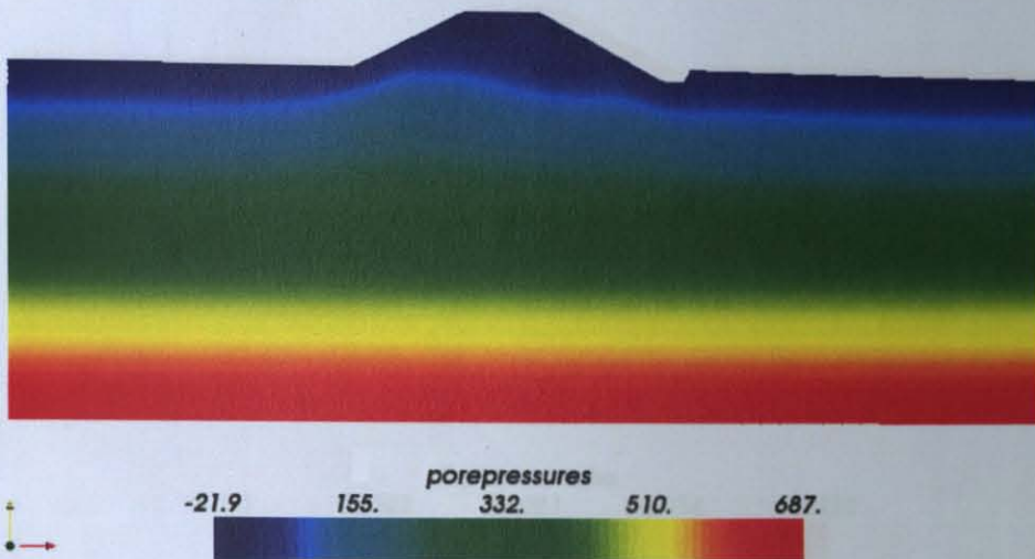
Figure 8 - 11: Pore pressures under seismic excitation at t = 40 seconds on the deformed shape of the structure. (kPa).
