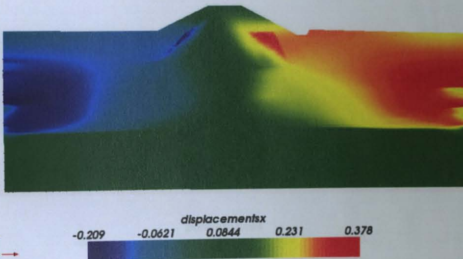
Figure 8 - 16: Horizontal displacements under seismic excitation at t = 30 seconds on the deformed shape of the structure. (meter).
