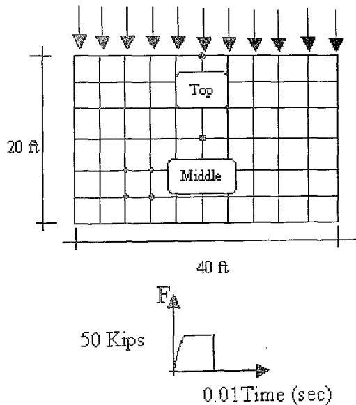
Figure 7 - 2: First verification example [44].
