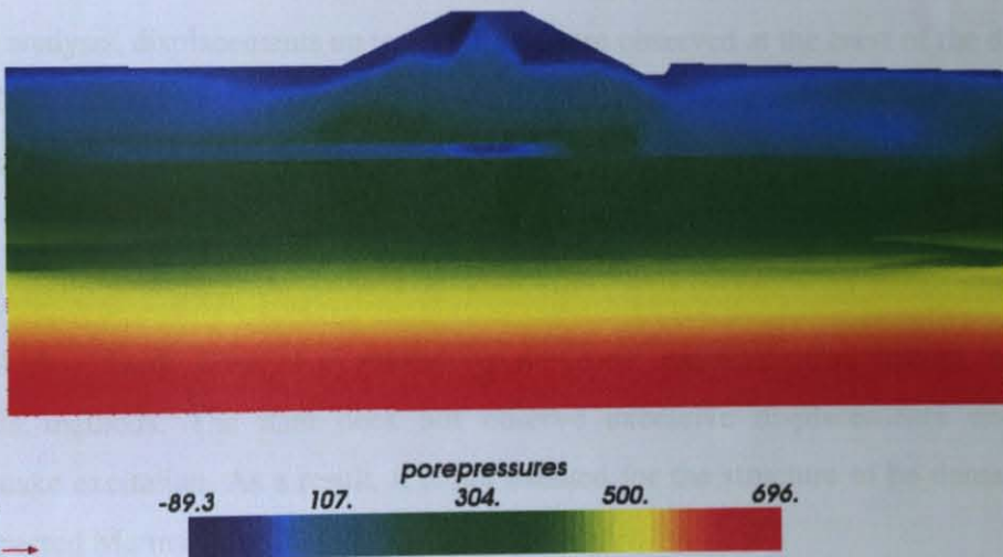
Figure 8 - 22: Pore pressures under seismic excitation at t = 40 seconds on the deformed shape of the structure. (kPa).
