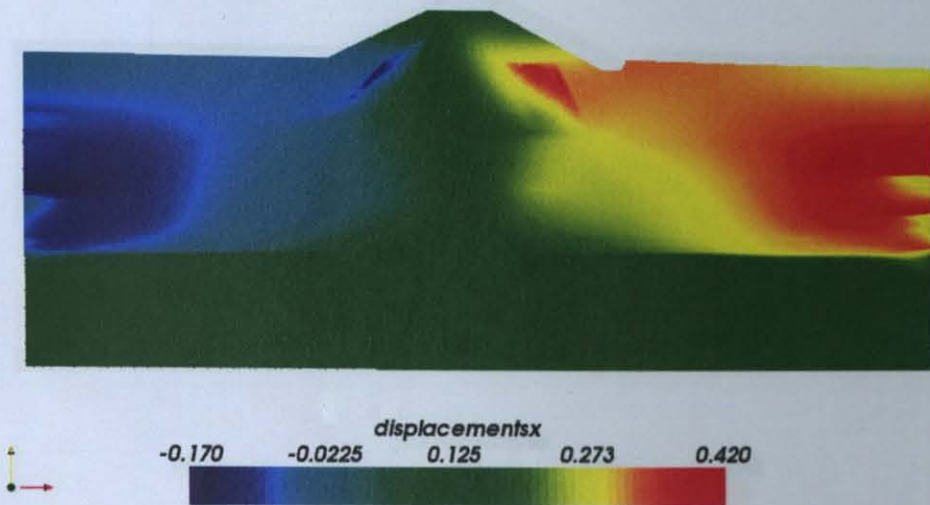
Figure 8 - 17: Horizontal displacements under seismic excitation at t = 40 seconds on the deformed shape of the structure. (meter).
