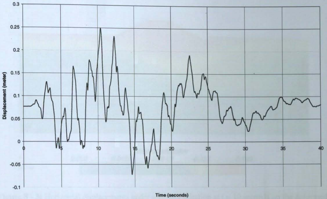
Figure 8 - 1: Dam's crest's horizontal displacements under seismic excitation. Linear elastic case.
