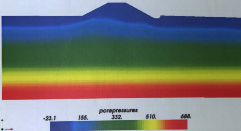
Figure 8 - 10: Pore pressures under seismic excitation at t = 30 seconds on the deformed shape of the structure. (kPa).
