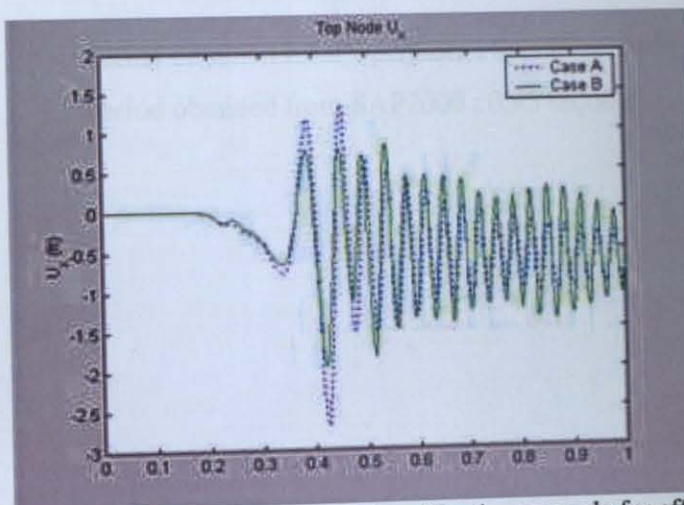
Figure 7 - 10: Results of second verification example for effective seismic input [44].
