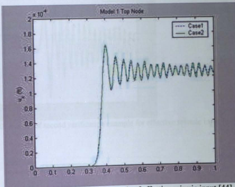
Figure 7 - 8: Results of the first verification example of effective seismic input [44].
