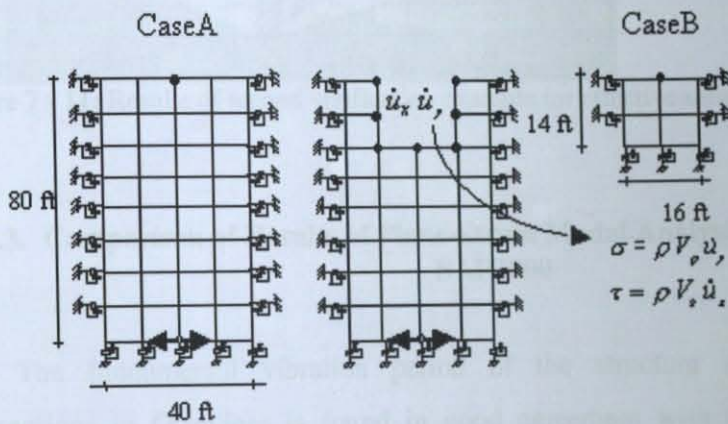
Figure 7 - 9: Second verification example for effective seismic input [44].
