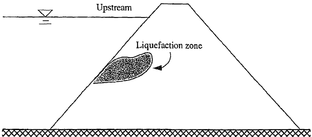
Figure 3 - 2: Liquefaction failure of an earth dam [14].
