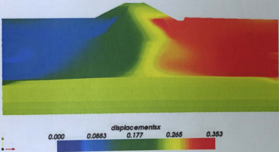
Figure 8 - 14: Horizontal displacements under seismic excitation at t = 10 seconds on the deformed shape of the structure. (meter).
