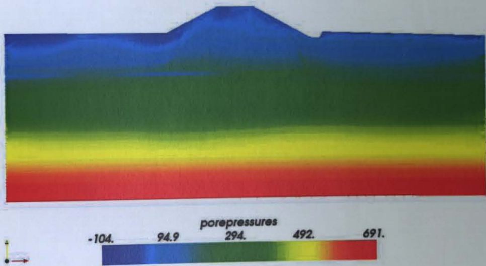
Figure 8 - 8: Pore pressures under seismic excitation at t = 10 seconds on the deformed shape of the structure. (kPa).
