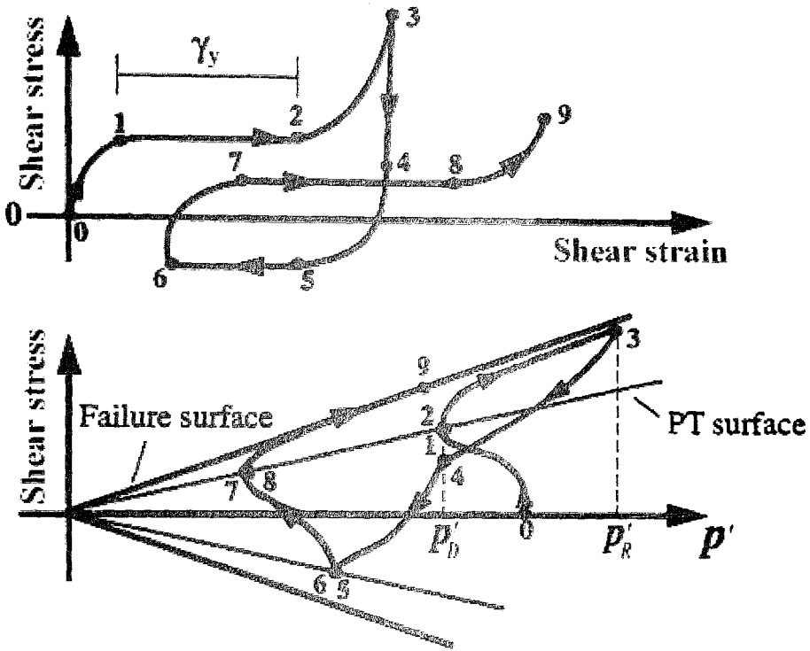
Figure 5 - 1: Constitutive model response showing shear stress, effective confinement, and shear strain [41].
