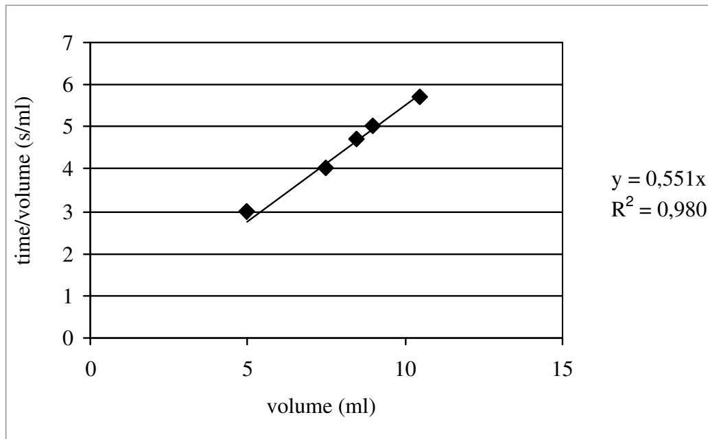
Figure B.1. Volume versus time/volume during the filtration of control sludge
