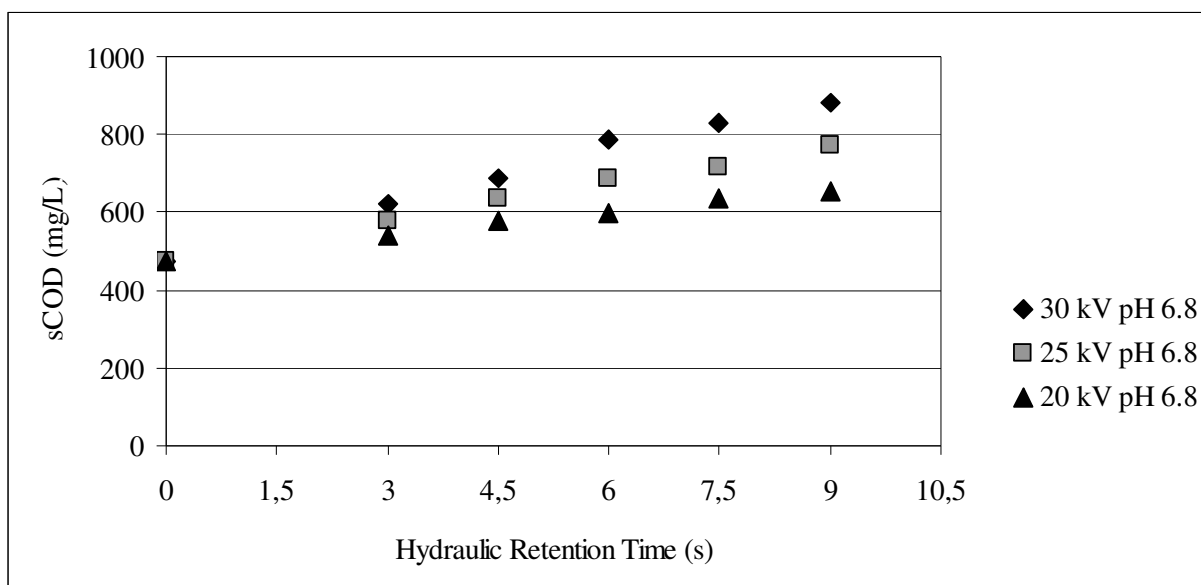
Figure 5.1. sCOD versus hydraulic retention time at different PEF intensities
