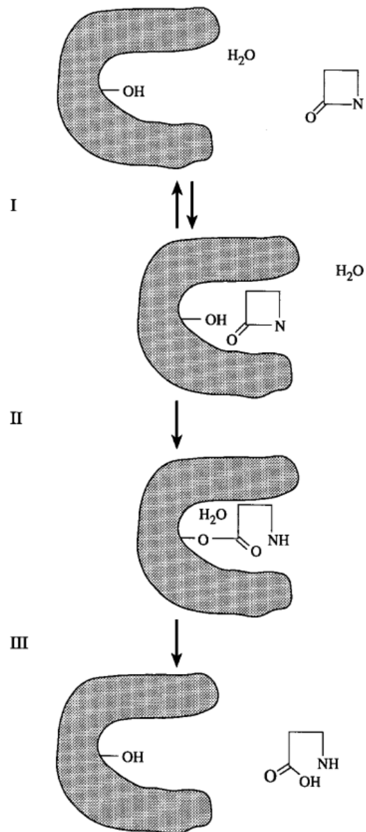
Figure 2.2. Hydrolysis of a \beta -lactam ring by \beta -lactamase using serine ester mechanism. \text{-OH} group of the active site serine is also shown [1].
