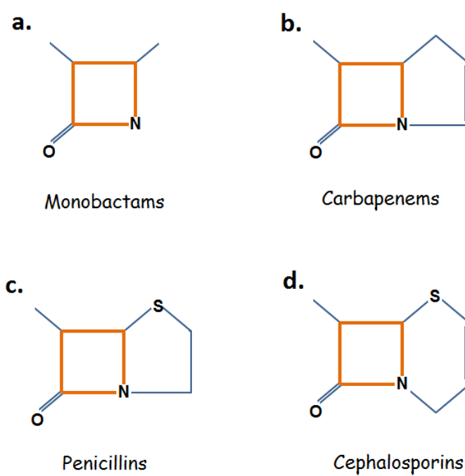
Figure 2.1. Structure of some \beta -lactam antibiotics. (a) Monobactams. (b) Carbapenems (c) Penicillins (d) Cephalosporins.
