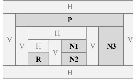
Figure 6.5. Floorplan for the circuit in Figure 6.4.
