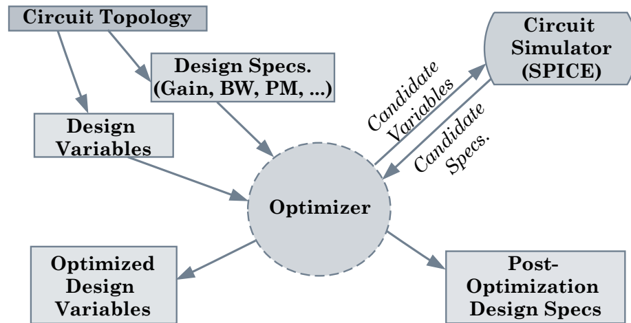
Figure 6.2. Conceptual flow diagram of the optimizer.
