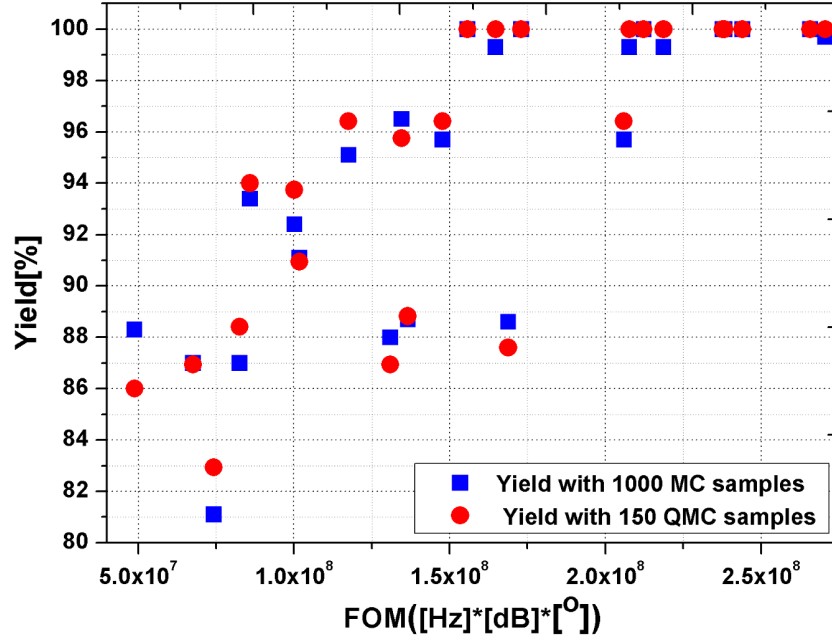
Figure 5.9. FOM vs Yield for multi objective optimization.
