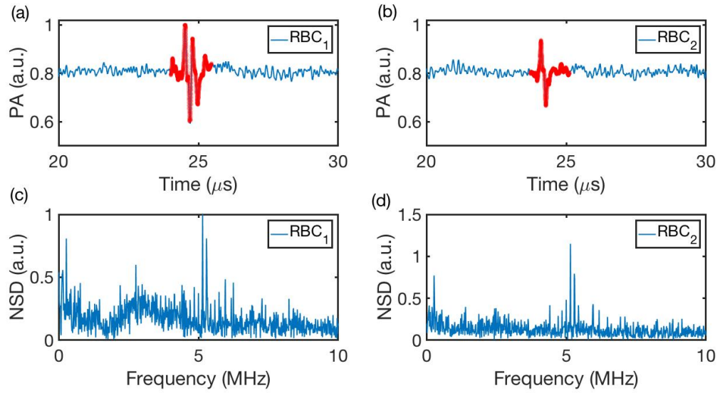
Figure 3.12. Normalized PA wave generated by (a) first (b) second RBC clusters vs time, and the frequency spectra of (c) the first (d) the second RBC clusters, an ultrasonic detector was located at position 3 mm (approximately)
