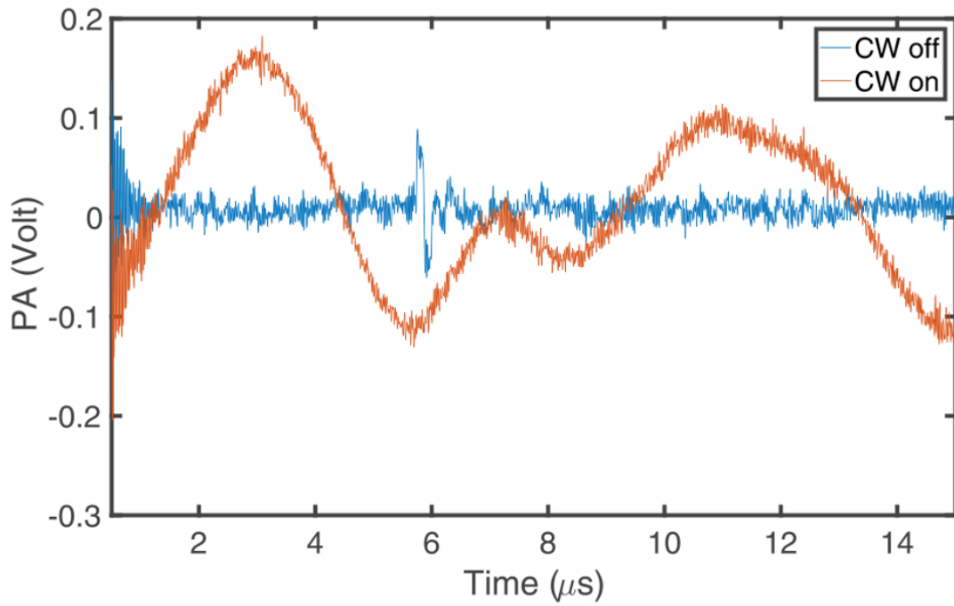
Figure 6.6. Comparison of the PA signal in absence of bubble (blue line) and the presence of bubble (red line).
