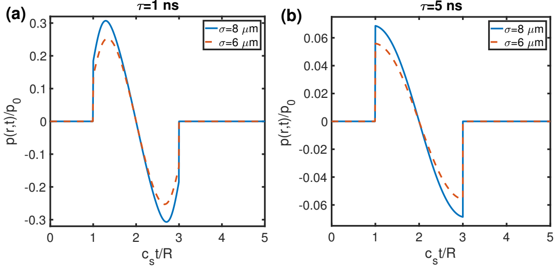
Figure 4.5. Normalized PA wave p(r,t)/p_0 generated by first source vs normalized time c_s t/R , an ultrasonic detector located at position r = 2R for the two different pulse durations (a) \tau = 1 and (b) 5 ns with different beamwidths \sigma = 6 \mu\text{m} (dashed line) and 8 \mu\text{m} (solid line), where R = 8 \mu\text{m} .
