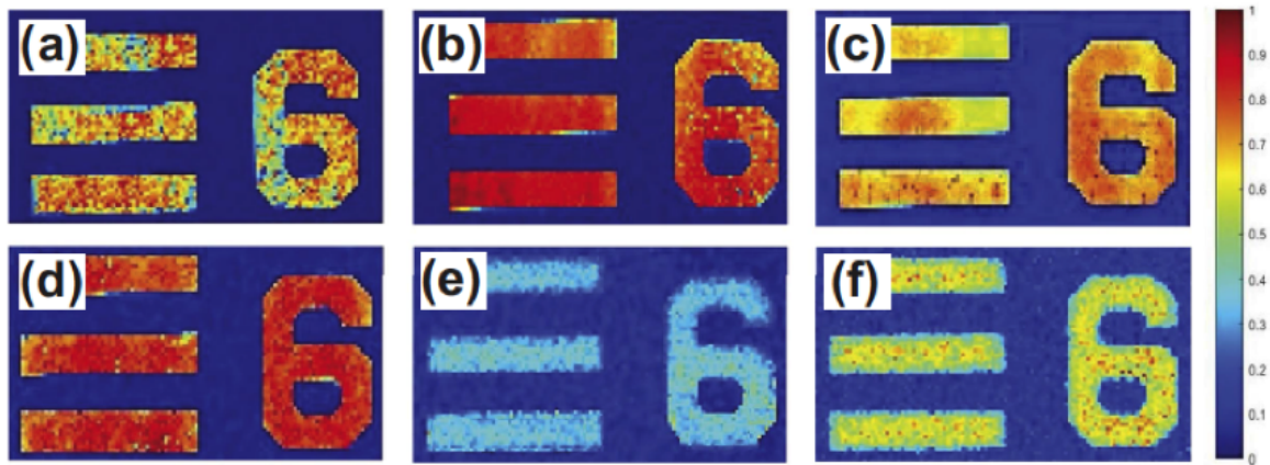
Figure 2.7. The PA image of Group 5 Element 6 scanned within an area of 56 \times 101 \mu m^2 with steps of 1 \mu m acquired at optical wavelength (a) 532 nm from harmonic generation unit, (b) 650 nm, (c) 697 nm, (d) 732 nm, (e) 785 nm, and (f) 880 nm, respectively from supercontinuum output.
