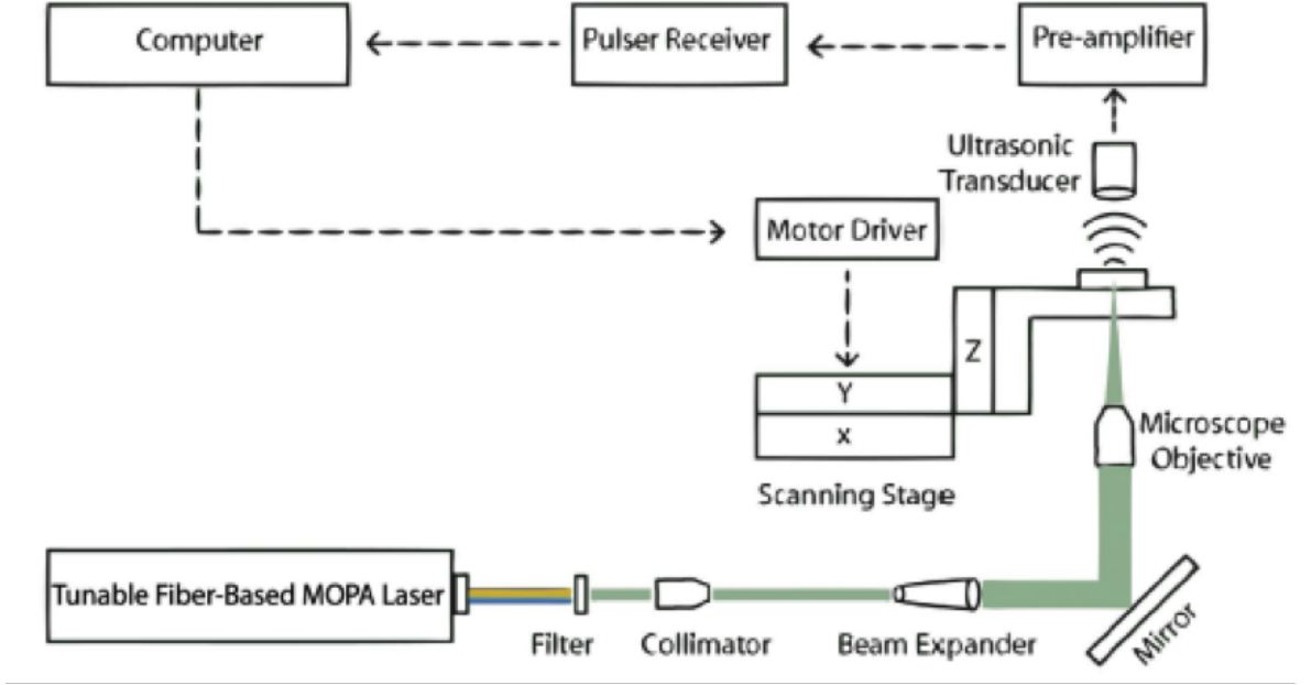
Figure 2.5. The schematics of experimental setup for transmission mode OR-PAM system.
