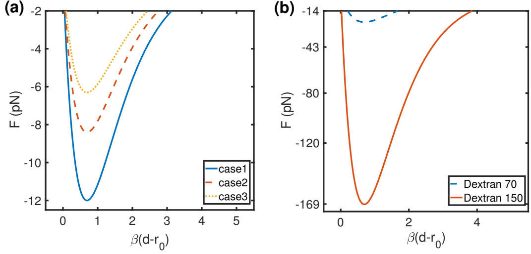
Figure 4.2. Aggregation force ( F ) corresponding to the various aggregation rates vs function of separation between cell surfaces ( \beta(d-r_0) ) for (a) case 1 [1,2]: D = 3 \times 10^{-17} \text{ J/m}^2 , \beta = 8 \times 10^5 \text{ m}^{-1} , r_0 = 3 \mu\text{m} ; case 2 [1,2]: D = 2.1 \times 10^{-17} \text{ J/m}^2 , \beta = 8 \times 10^5 \text{ m}^{-1} , r_0 = 2.5 \mu\text{m} ; case 3 [1,2]: D = 2.1 \times 10^{-17} \text{ J/m}^2 , \beta = 6 \times 10^5 \text{ m}^{-1} , r_0 = 2 \mu\text{m} , (b) Dextran 70 [3]: D = 5.75 \times 10^{-17} \text{ J/m}^2 , \beta = 6 \times 10^5 \text{ m}^{-1} , r_0 = 2 \mu\text{m} ; Dextran 150 [3]: D = 56.4 \times 10^{-17} \text{ J/m}^2 , \beta = 8 \times 10^5 \text{ m}^{-1} , r_0 = 3 \mu\text{m} .
