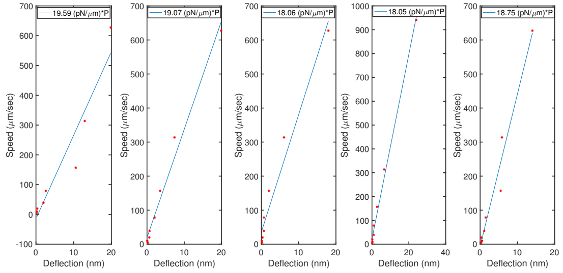
Figure 4.17. The relationship between deflection vs speed. Each graph is obtained at different laser trapping powers.
