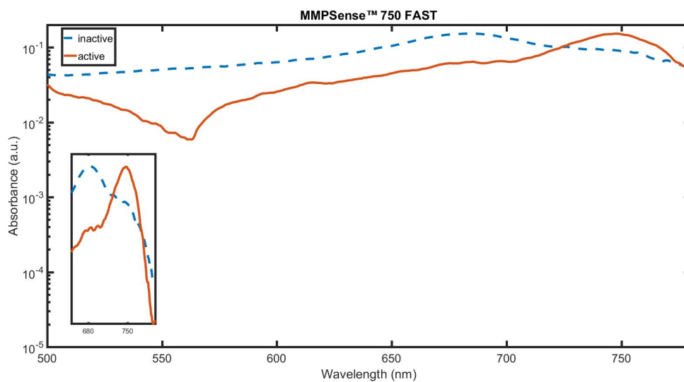
Figure 5.3. Measured absorbance spectrum of inactive (dotted line) versus activated (solid gray line) MMPsense™ 750 FAST probe.
