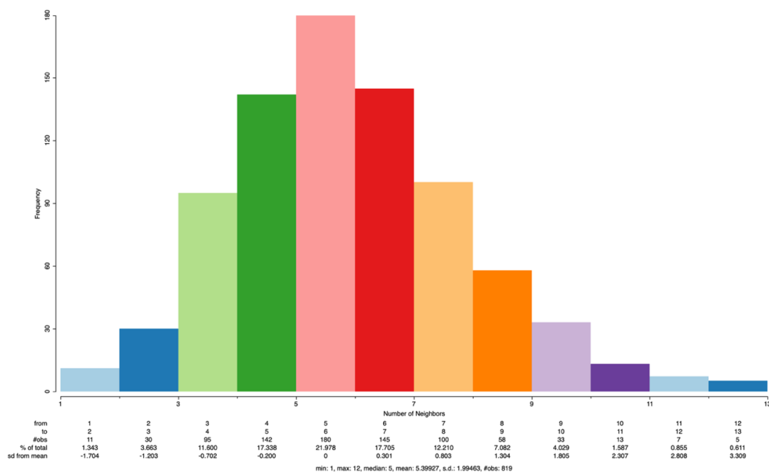
Figure 3. Connectivity histogram
