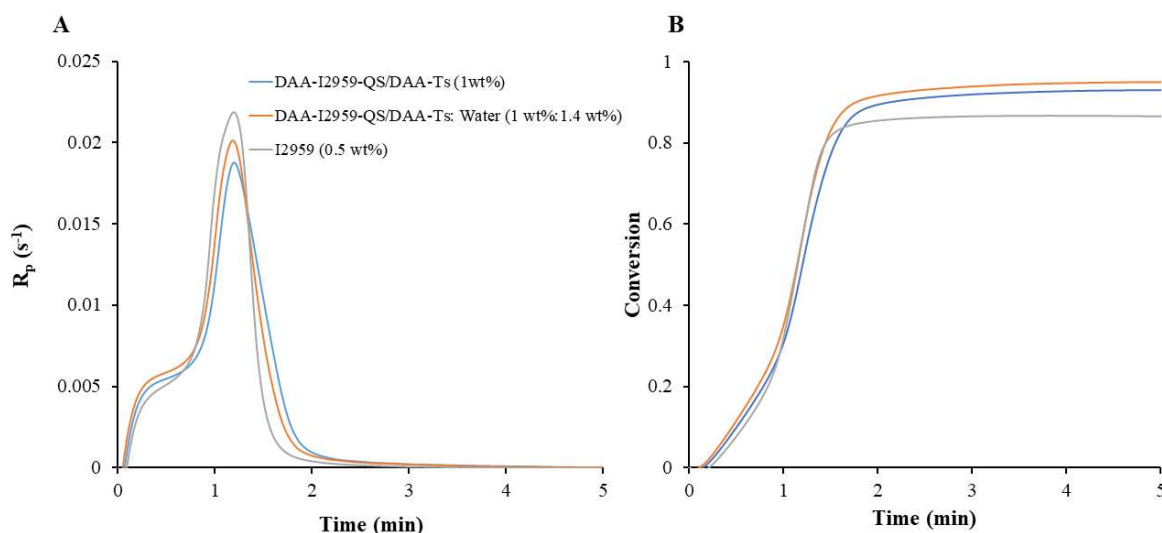
Figure 4.8. (a) Rate-time and (b) conversion-time plots for HEMA containing DAA-I2959-QS/DAA-Ts (1 wt% PI approximately contains 0.5 wt% I2959) and I2959 (0.5 wt%) at 25 °C under nitrogen and 320-500 nm irradiation.
