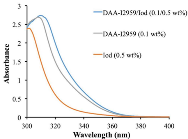
Figure 3.22. Absorption spectra of DAA-I2959/Iod (0.1/0.5 wt%), DAA-I2959 (0.1 wt%) and Iod (0.5 wt%) in HEMA.
