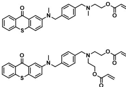
Figure 1.7. Structures of one component visible light PIs [24]. Permission from [24] WILEY-VCH Verlag GmbH & Co. KGaA, Weinheim, Copyright (2017).
