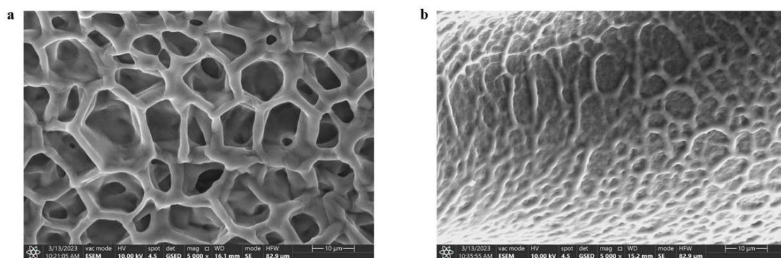
Figure 4.10. SEM images of the hydrogels (a) PEGDA:DAA-I2959-QS/DAA-Ts 95:5 (I2959 equivalent wt%:wt%) and (b) PEGDA:I2959 95:5 (wt%:wt%).
