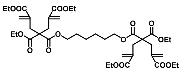
Figure 1.11. Cyclopolymerizable monomer based cross-linker synthesized by Peer et al. [88]. Permission from [88] American Chemical Society Copyright (2020).
