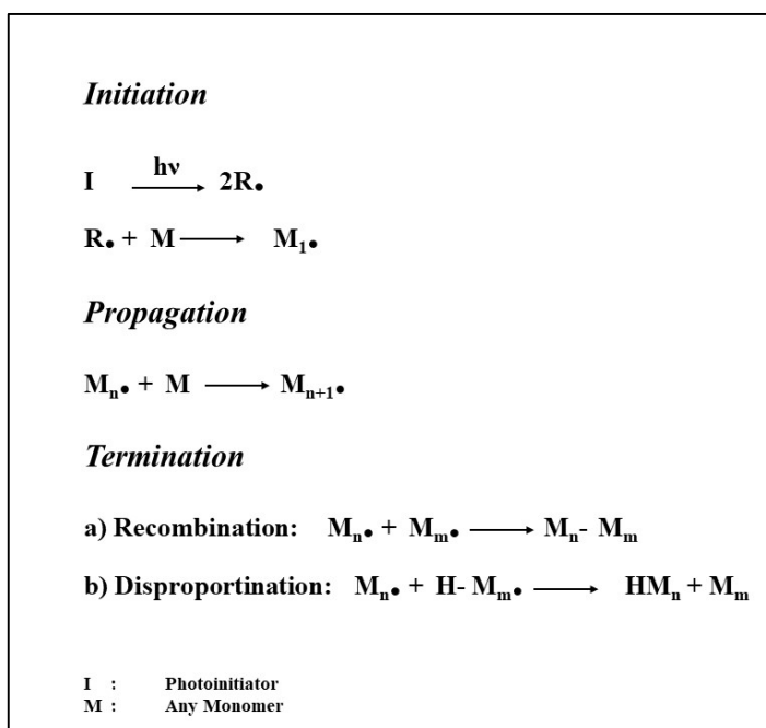
Figure 1.1. The steps of a free radical photopolymerization reaction [7,8]. Permission from [8] American Institute of Chemical Engineers (AIChE), Copyright (2008). No permission is required from [7].
