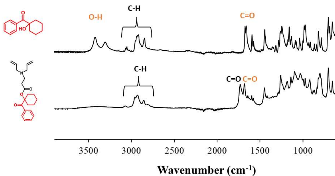
Figure 3.8. FTIR spectra of DAA-I184 and I184.
