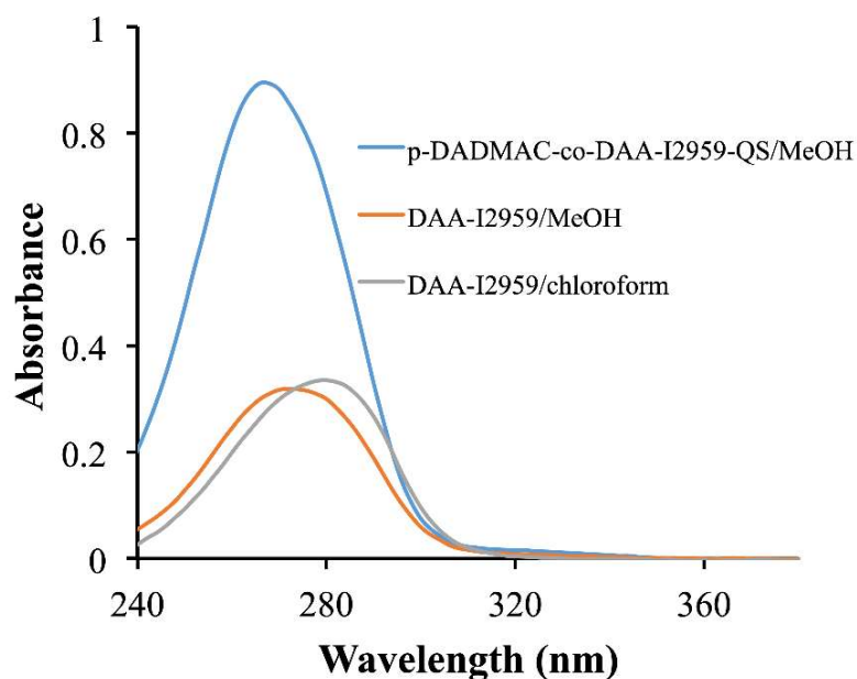
Figure 3.13. UV-vis absorption spectra of DAA-I2959 ( 2 \times 10^{-5} M) in MeOH and \text{CHCl}_3 and p-DADMAC-co-DAA-I2959-QS ( 0.2 \times 10^{-6} M) in methanol.
