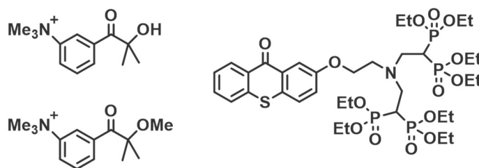
Figure 1.8. Some water soluble PIs in the literature [38], [53]. Permission from [53] Elsevier Ltd. Copyright (2020). No permission is required from [38].
