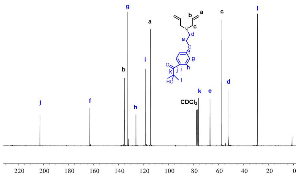
Figure 3.5. 13 C NMR spectrum of DAA-I2959.
