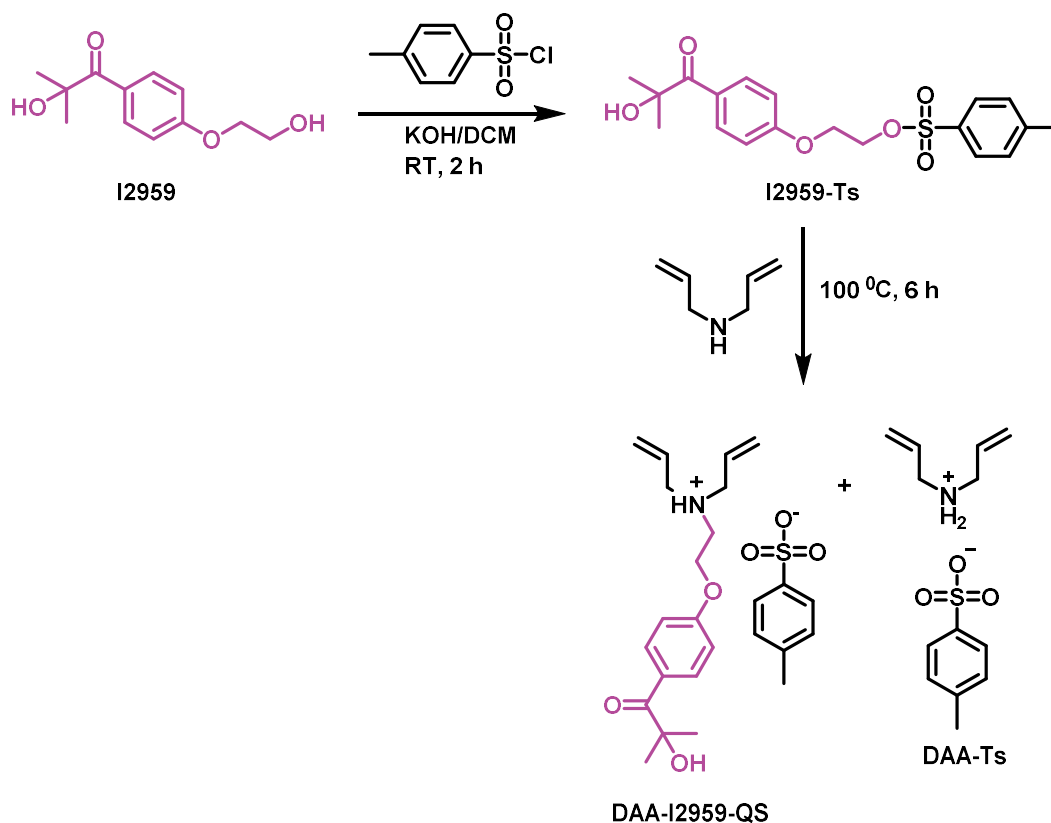
Figure 4.1. Synthesis of DAA-I2959-QS/DAA-Ts.
