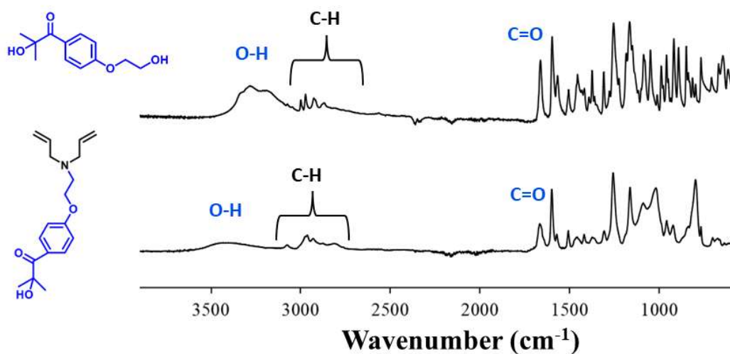
Figure 3.7. FTIR spectra of DAA-I2959 and I2959.
