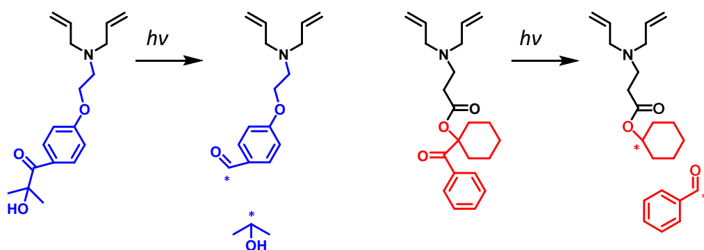
Figure 3.16. Type I cleavage of DAA-I2959 and DAA-I184 to generate benzoyl-ketyl radical pairs.
