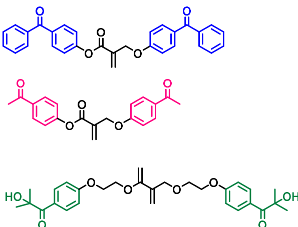
Figure 1.9. Structures of monomeric PIs synthesized by Cesur et al. [58]. Permission from [58] Elsevier B.V. Copyright (2015).
