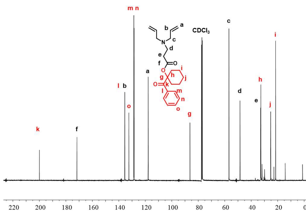
Figure 3.6. 13 C NMR spectrum of DAA-I184.
