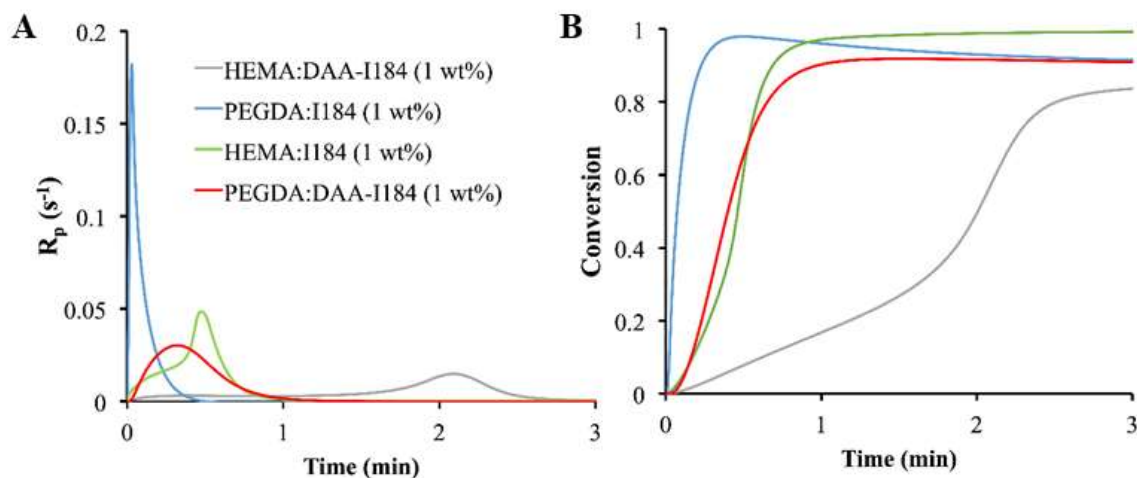
Figure 3.18. (a) Rate–time and (b) conversion–time plots for HEMA and PEGDA containing DAA-I184 (1 wt%) and I184 (1 wt%) at 25 °C under nitrogen and 320–500 nm irradiation.
