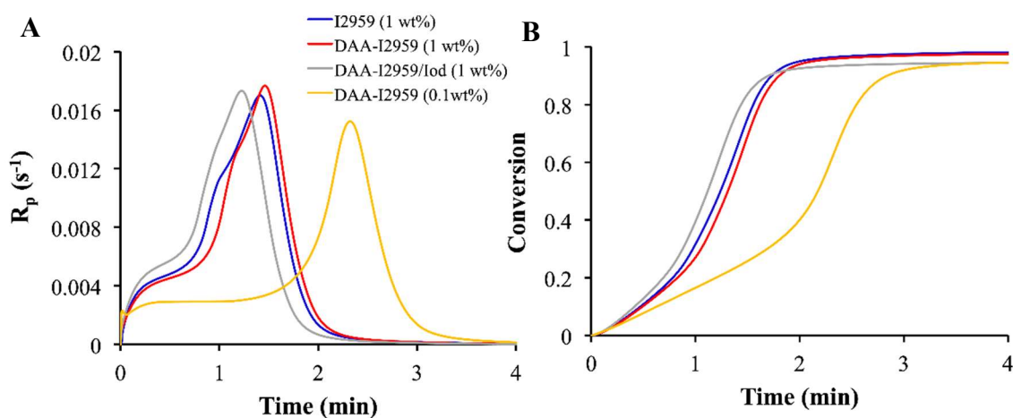
Figure 3.17. (a) Rate–time and (b) conversion–time plots for HEMA containing DAA-I2959 (0.1 wt%), DAA-I2959 (1 wt%), DAA-I2959 (1 wt%)/Iod (1 wt%), and I2959 (1 wt%) at 25 °C under nitrogen and 320–500 nm irradiation.
