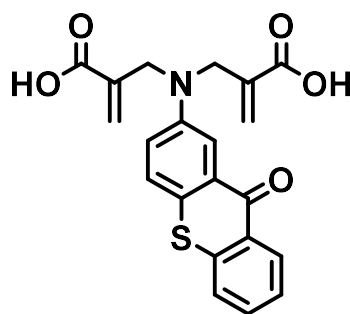
Figure 1.12. Structure of thioxanthone-functionalized 1,6-heptadiene monomeric PI [59].
