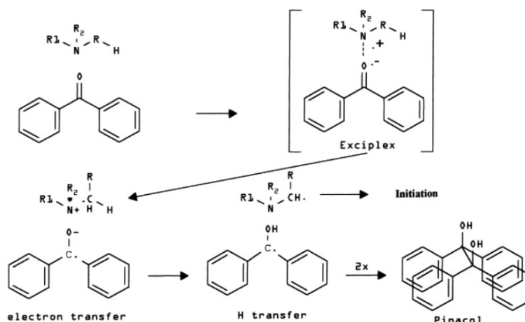
Figure 1.5. The schematic representation of electron and hydrogen atom abstraction processes between benzophenone and an amine. Permission from [21] Copyright 1999 Elsevier Science S.A.
