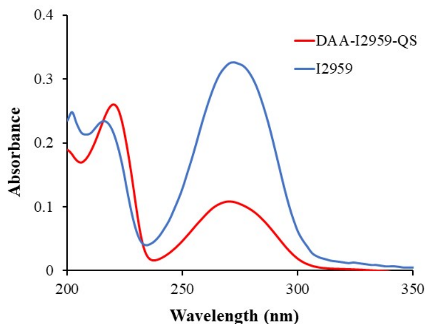
Figure 4.6. UV-vis absorption spectra of DAA-I2959-QS/DAA-Ts ( 0.78 \times 10^{-5} M DAA-I2959-QS) and I2959 ( 2.00 \times 10^{-5} M) in methanol.
