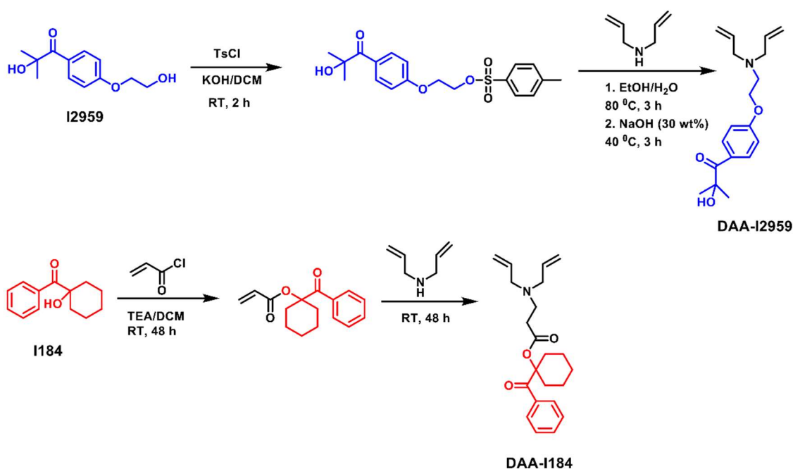
Figure 3.1. Synthesis of cyclopolymerizable PIs.
