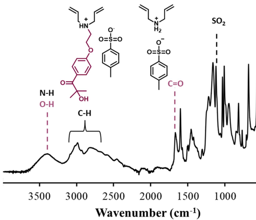
Figure 4.4. FTIR spectrum of DAA-I2959-QS/DAA-Ts.
