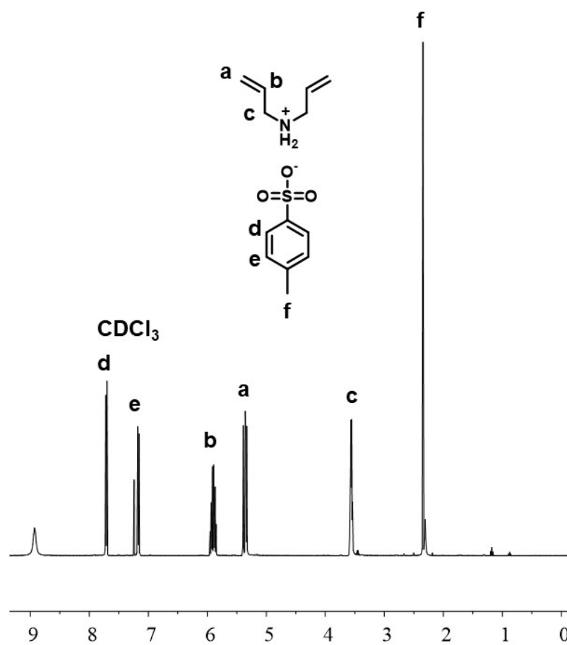
Figure 4.3. ^1\text{H} NMR spectrum of p-toluene sulphonate salt of DAA.
