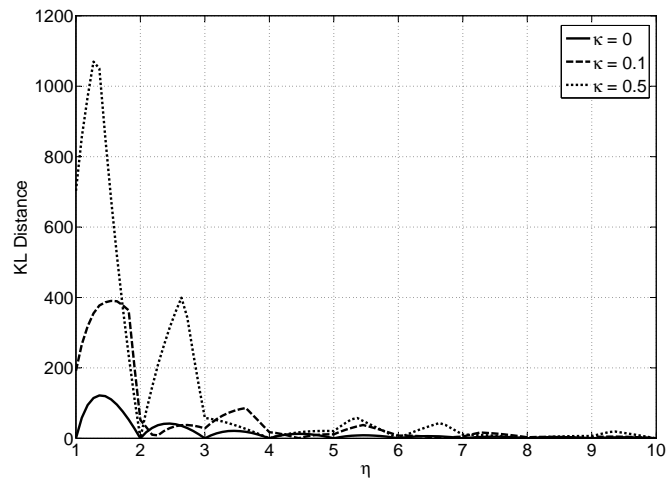
Figure 5.7. KL Distance between \{W_n\} and \{\tilde{W}_n\} versus \eta for \kappa = 0, 0.1, 0.5
