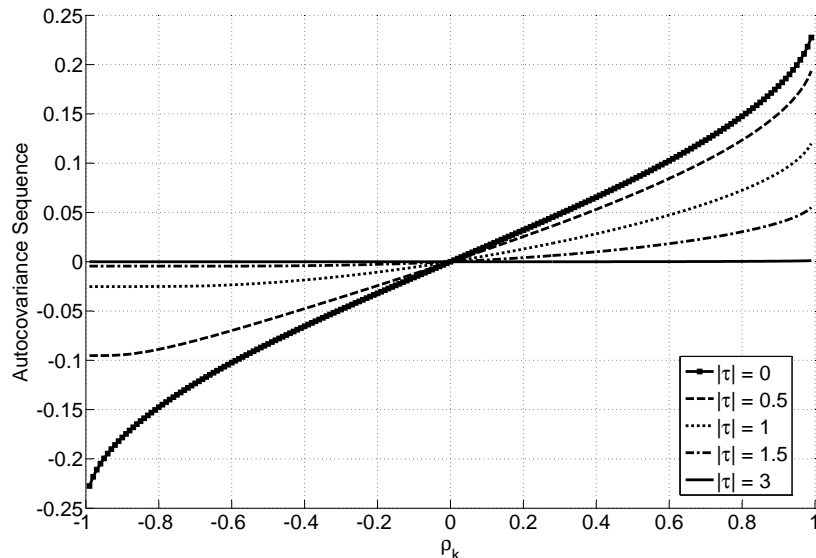
Figure 5.1. Autocovariance Sequence of Z_n versus \rho_k
