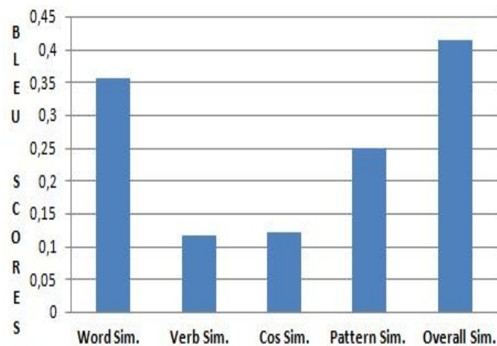
Figure 4.5. BLEU Scores
