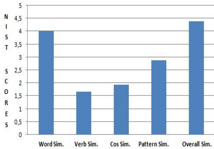
Figure 4.6. NIST Scores
