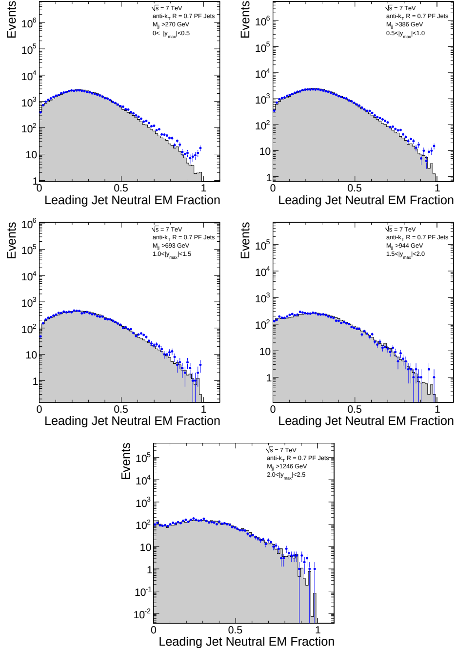
Figure 5.9. The neutral electromagnetic fraction of the leading jet for the five different |y|_{\max} bins and for the HLT_Jet70U sample. The plots for data (points) and simulated (dashed histogram) events are compared.
