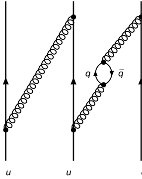
Figure 2.4. An illustration of the inner structure of the proton. At any given time, there might be one or several quark anti-quark pairs inside the proton.
