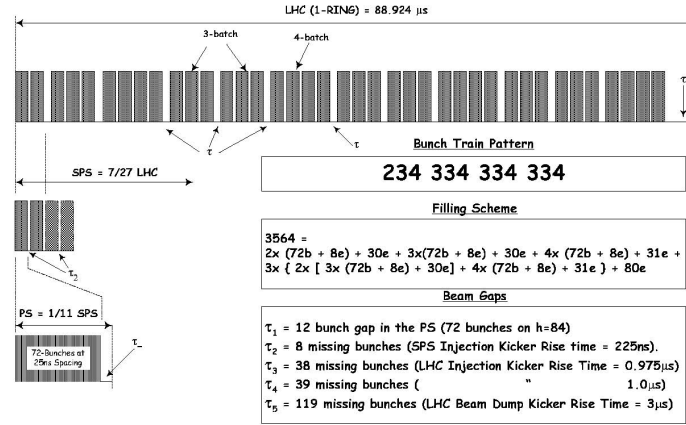
Figure 3.2. The bunch structure of the LHC beam. Notice the large gap at the end.
