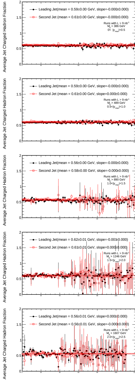
Figure C.10. The charged hadron fraction of the leading and second jet for the five different y_{max} bins and for the HLT_Jet100U trigger as a function of time (run number), fitted with a first degree polynomial.
