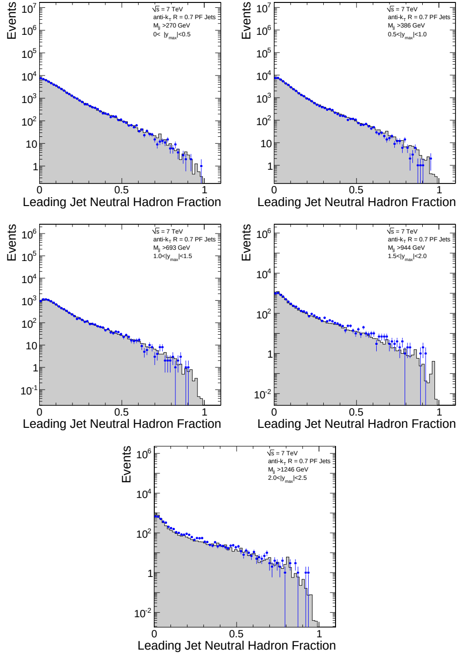
Figure 5.8. The neutral hadron fraction of the leading jet for the five different |y|_{\max} bins and for the Jet70U sample. The plots for data (points) and simulated (dashed histogram) events are compared.
