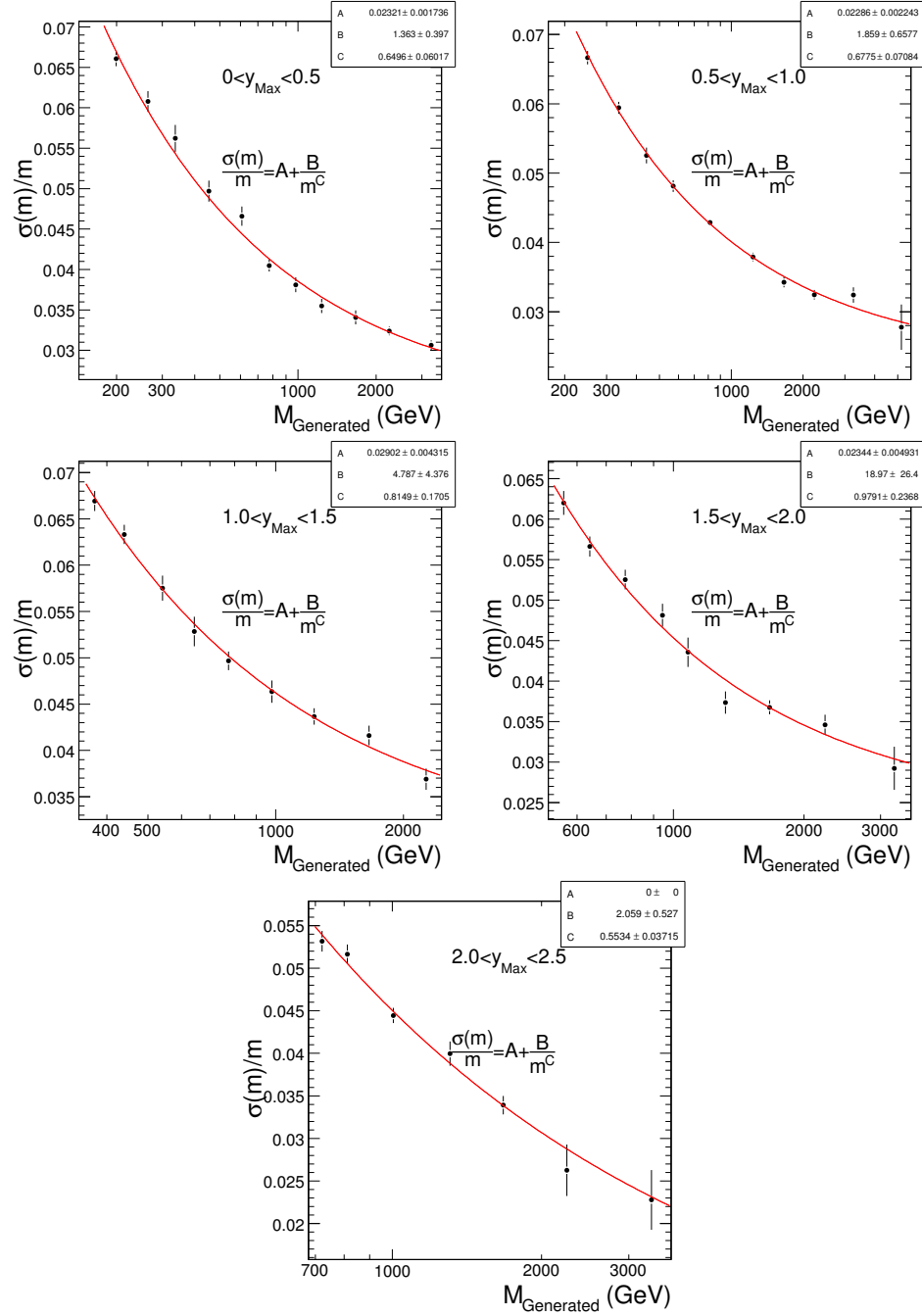
Figure 5.25. Relative dijet mass resolution, as a function of the generated mass in all |y|_{\text{max}} bins.
