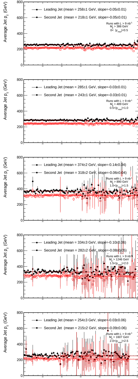
Figure C.9. The p_T of the leading and second jet for the five different y_{max} bins and for the HLT_Jet100U trigger as a function of time (run number), fitted with a first degree polynomial.
