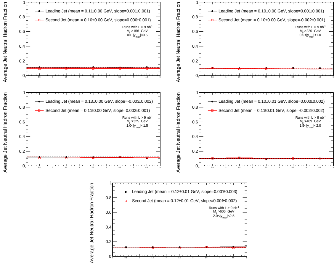
Figure B.31. The neutral hadron fraction of the leading and second jet for the five different y_{max} bins and for the HLT_Jet30U trigger as a function of time (run number), fitted with a first degree polynomial.
