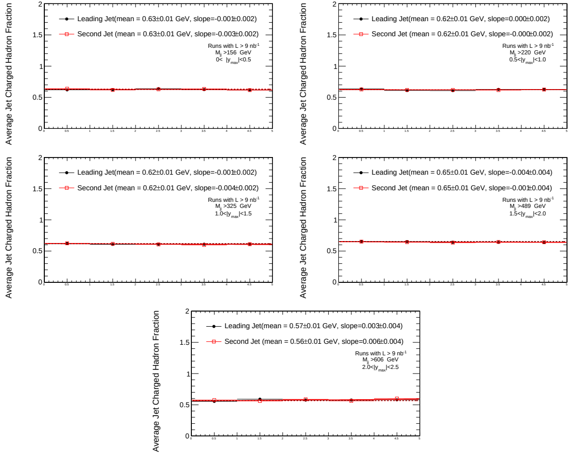
Figure B.30. The charged hadron fraction of the leading and second jet for the five different y_{max} bins and for the HLT_Jet30U trigger as a function of time (run number), fitted with a first degree polynomial.
