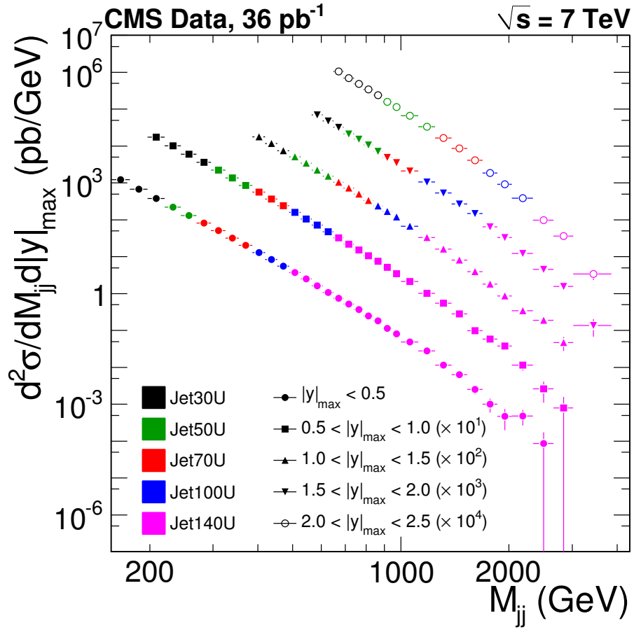
Figure 5.27. Dijet mass spectrum formed by the combination of the different samples.
