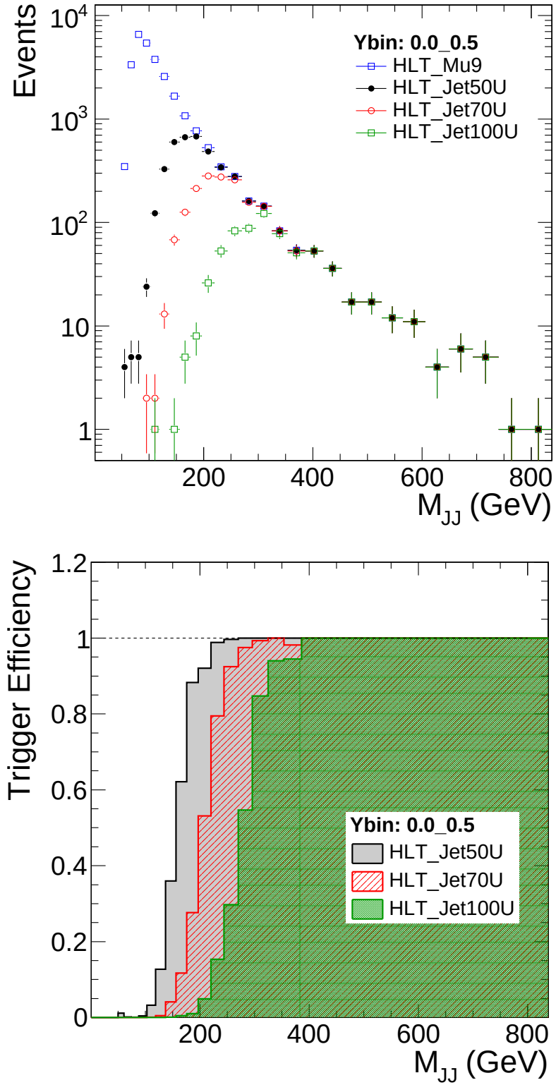
Figure 5.3. Trigger efficiencies measured with respect to the HLT_Mu9 trigger.
