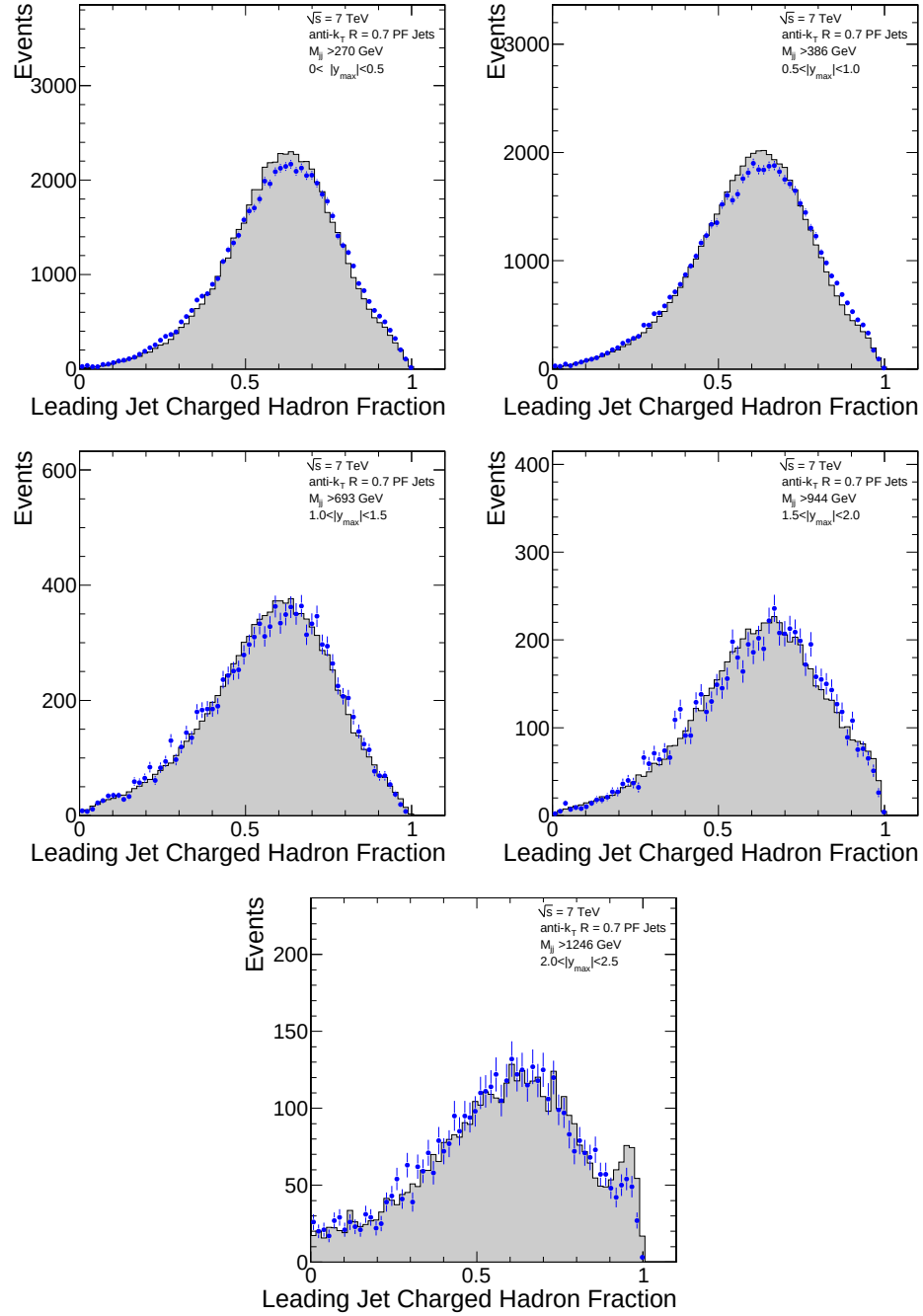
Figure 5.7. The charged hadron fraction of the leading jet for the five different |y|_{\max} bins and for the Jet70U sample. The plots for data (points) and simulated (dashed histogram) events are compared.
