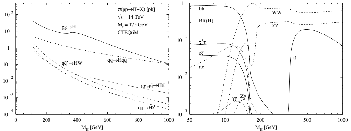
Figure 3.3. Higgs production cross sections at the LHC for the various production mechanisms as a function of the Higgs mass (left). Branching ratios of the dominant decay modes of the SM Higgs particle (right)
