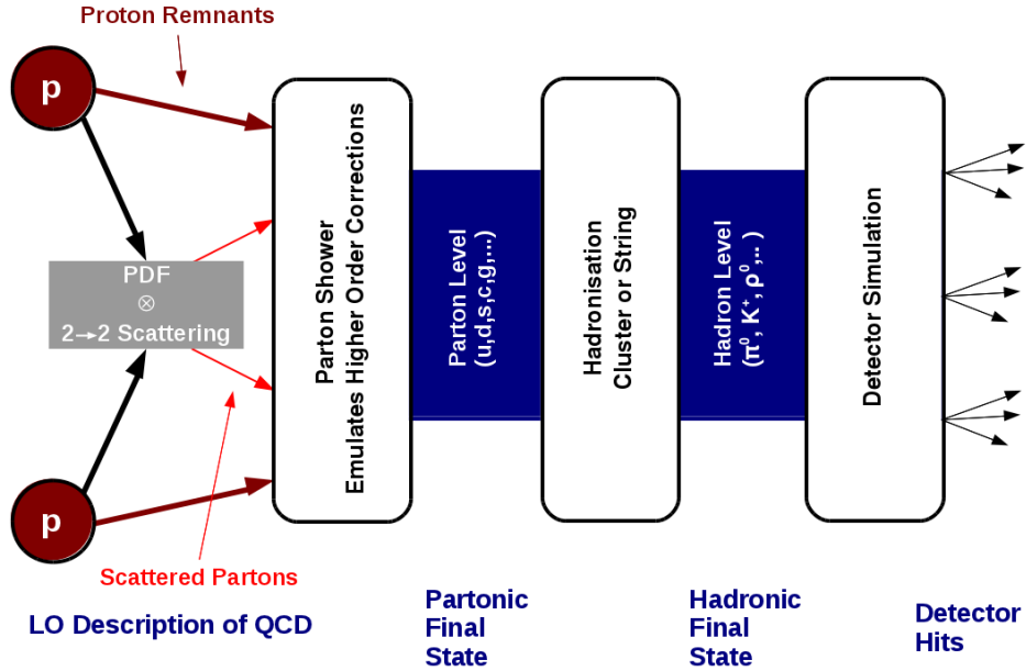
Figure 4.1. The basic steps in the generation of a simulated event.
