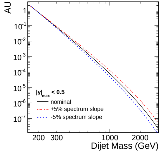
Figure 6.3. Simulated dijet mass spectrum (continuous line) in the rapidity bin |y|_{\max} < 0.5 which is used for the evaluation of the smearing effect. The dashed and the dashed-dotted lines correspond to softer and harder spectra respectively, systematically shifted by changing the slope by 5%.
