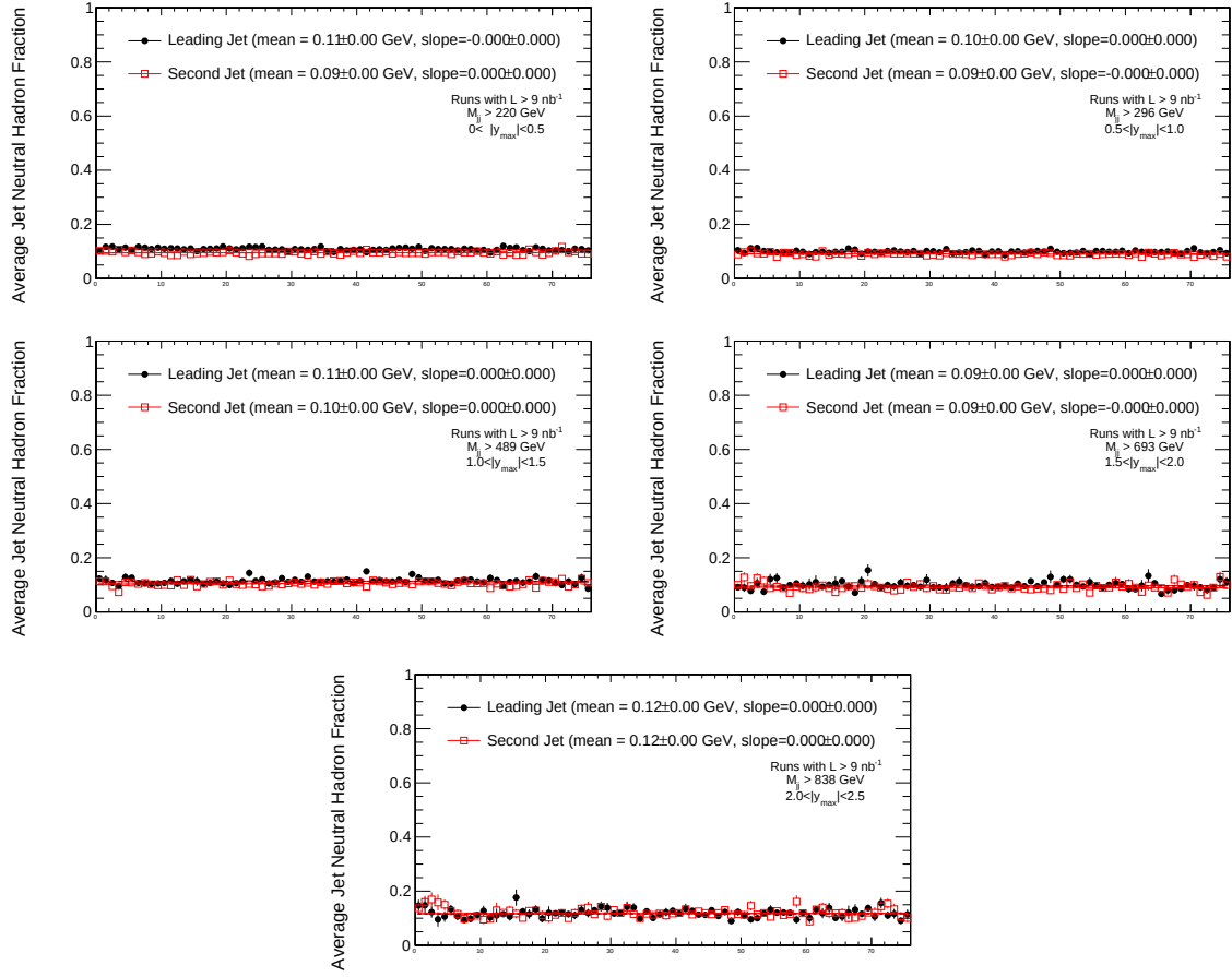
Figure B.35. The neutral hadron fraction of the leading and second jet for the five different y_{\text{max}} bins and for the HLT_Jet50U trigger as a function of time (run number), fitted with a first degree polynomial.
