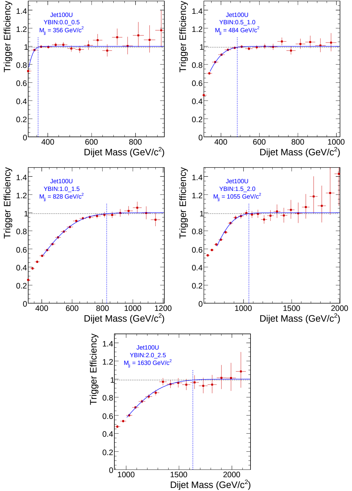
Figure B.3. Relative trigger efficiencies as a function of dijet mass for the five different |y|_{\text{max}} bins and for the HLT_Jet100U trigger. The 100% efficiency point is determined by performing a fit with an error function.
