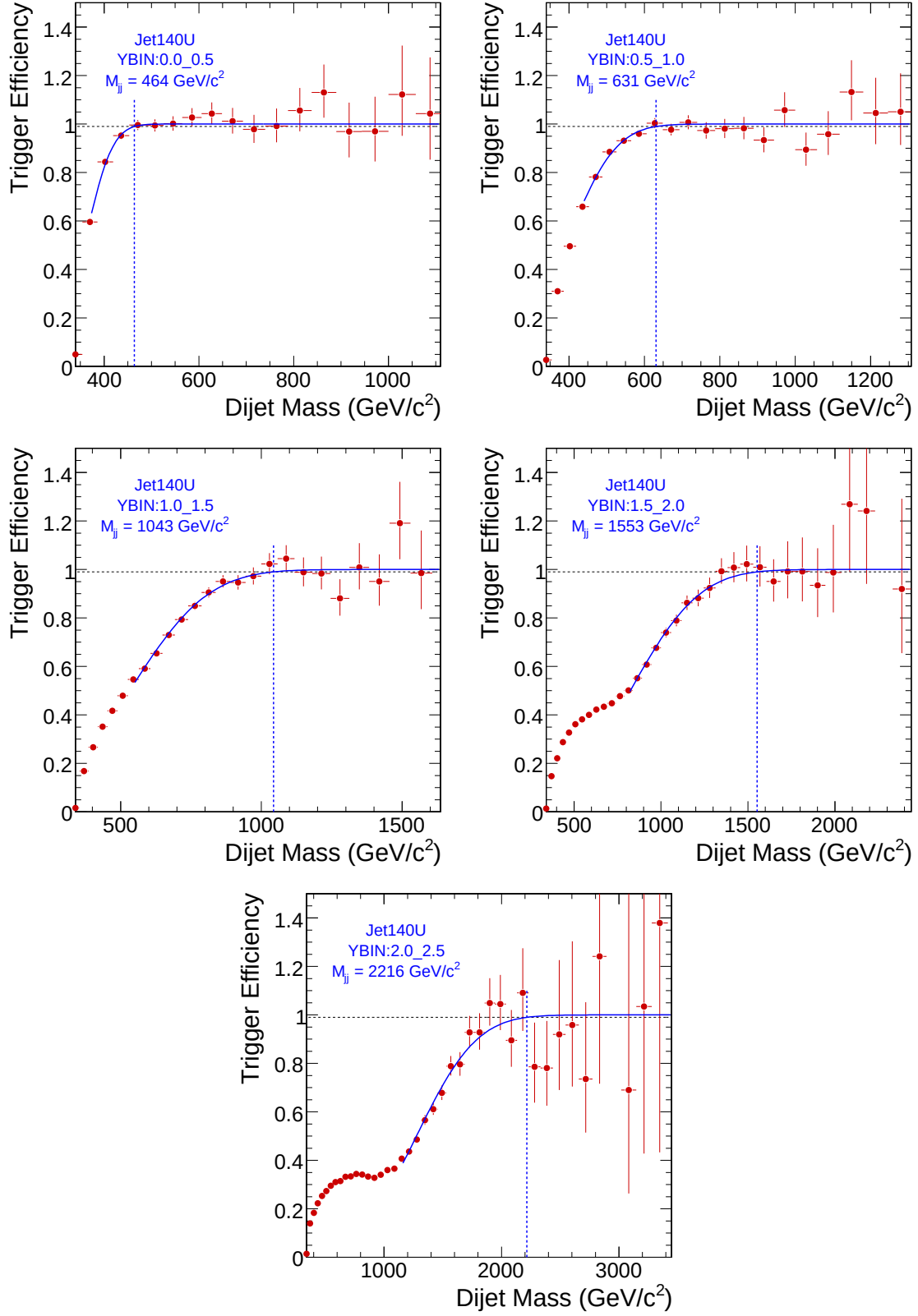
Figure B.4. Relative trigger efficiencies as a function of dijet mass for the five different |y|_{\max} bins and for the HLT_Jet140U trigger. The 100% efficiency point is determined by performing a fit with an error function.
