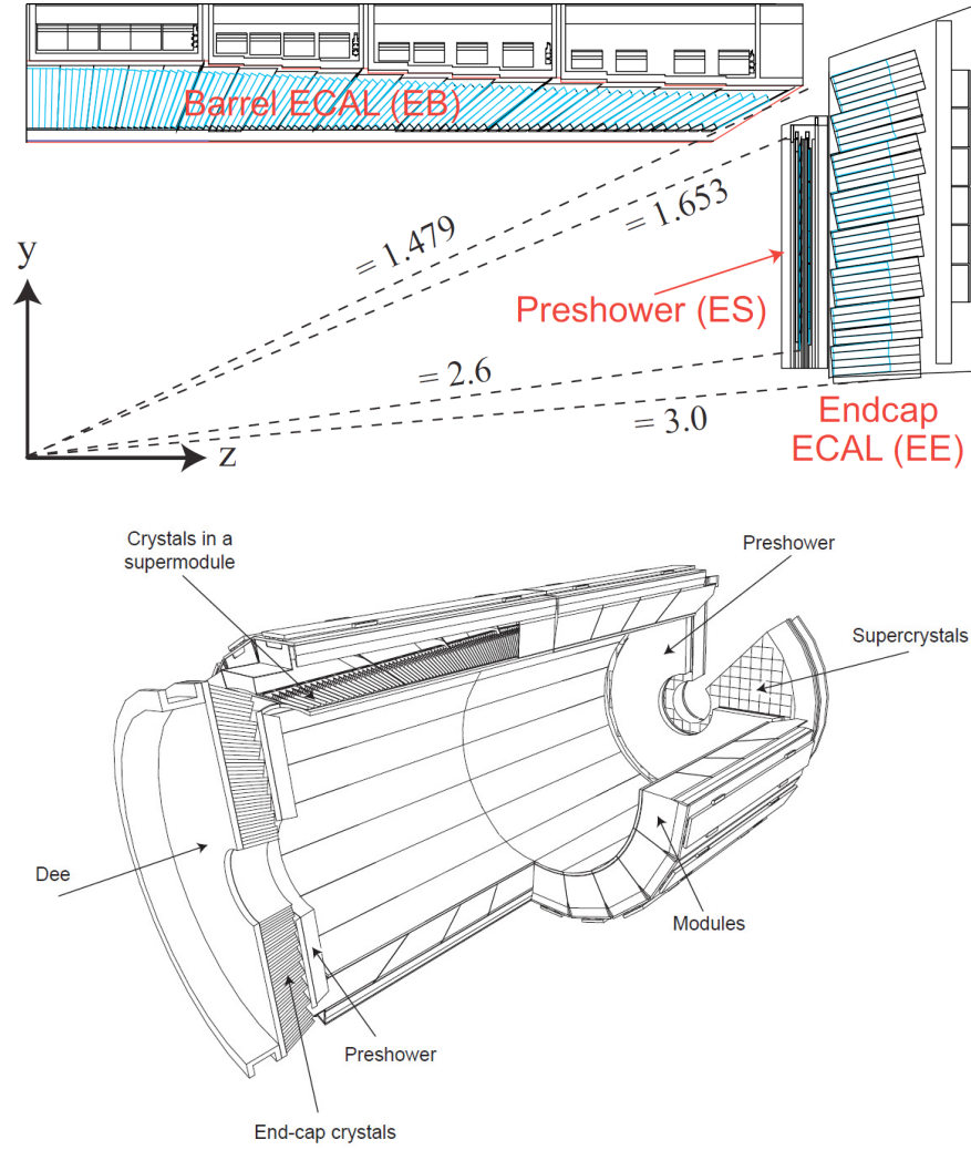
Figure 3.8. Geometric view of one quarter of the ECAL (top). Layout of the CMS electromagnetic calorimeter presenting the arrangement of crystal modules, supermodules, endcaps and the preshower in front (bottom) [13].
