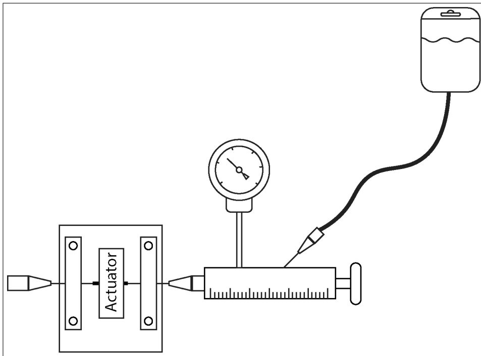
Figure 3.6 Schematic of the pressure measurement setup.
