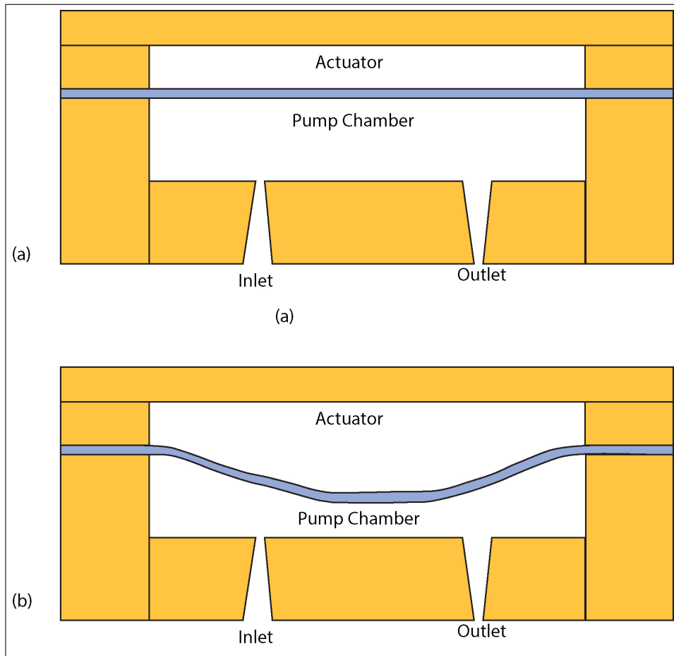
Figure 1.1 Illustration of a micropump with a diaphragm. Different actuation mechanisms can be used for the diaphragm displacement.
