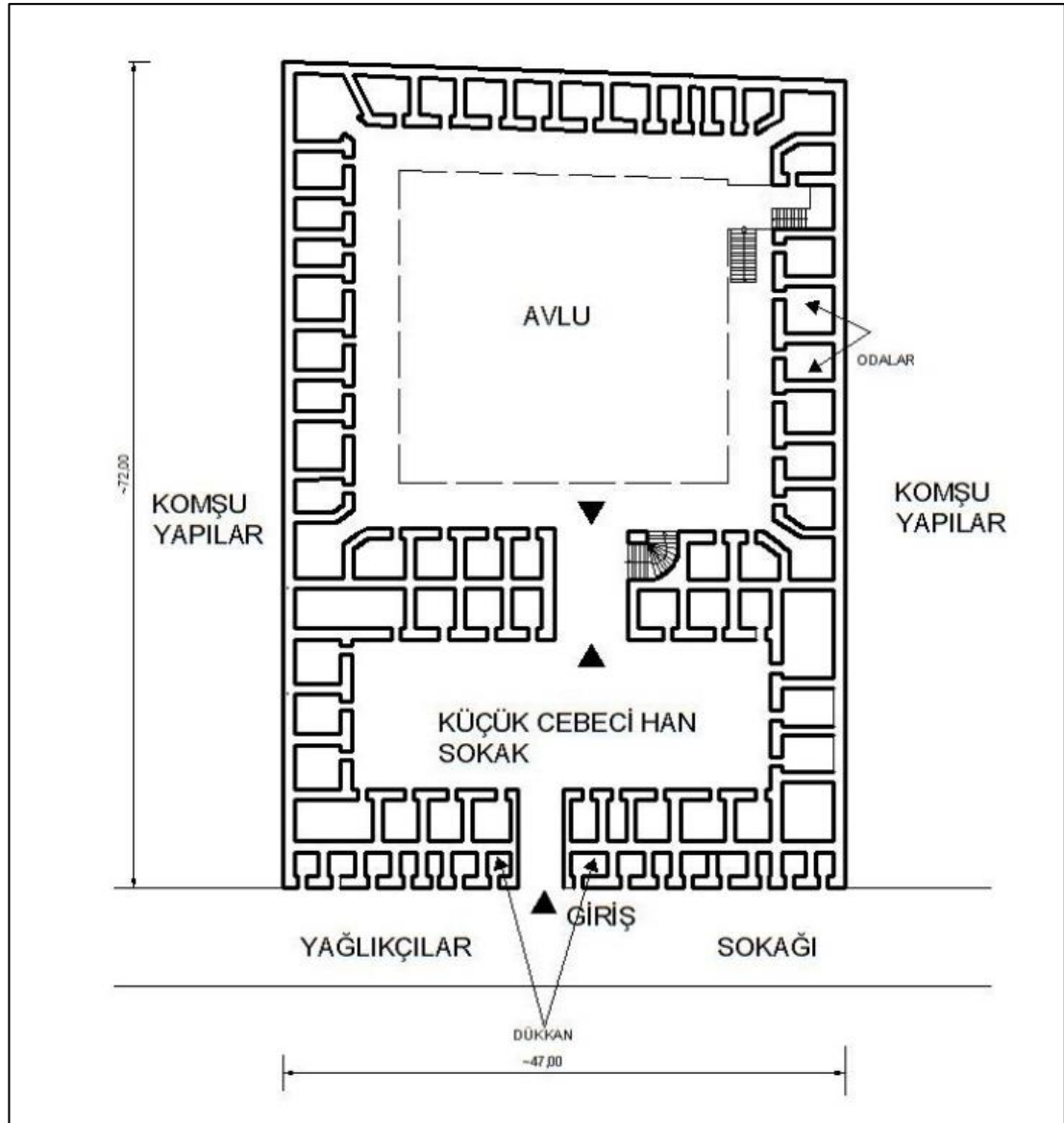
Figure 84. The plan of Cebeci Han. (Sökmen, 83).
