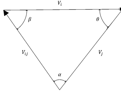
Figure 2.10. Relative Velocity and the Related Angles for the Calculations.
