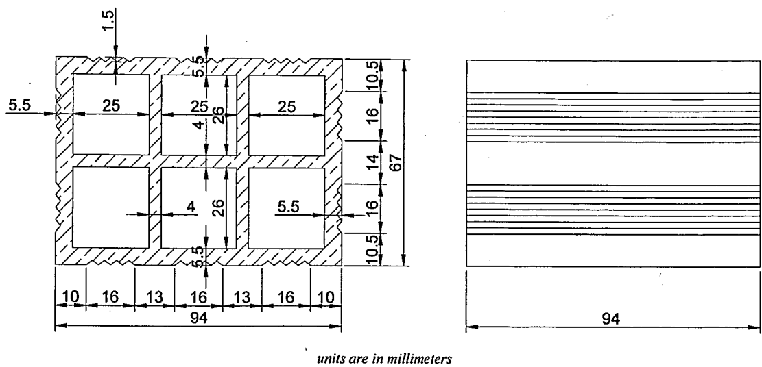
Figure 2.2. HCT Type II – Light hollow clay tile unit with thinner shells
