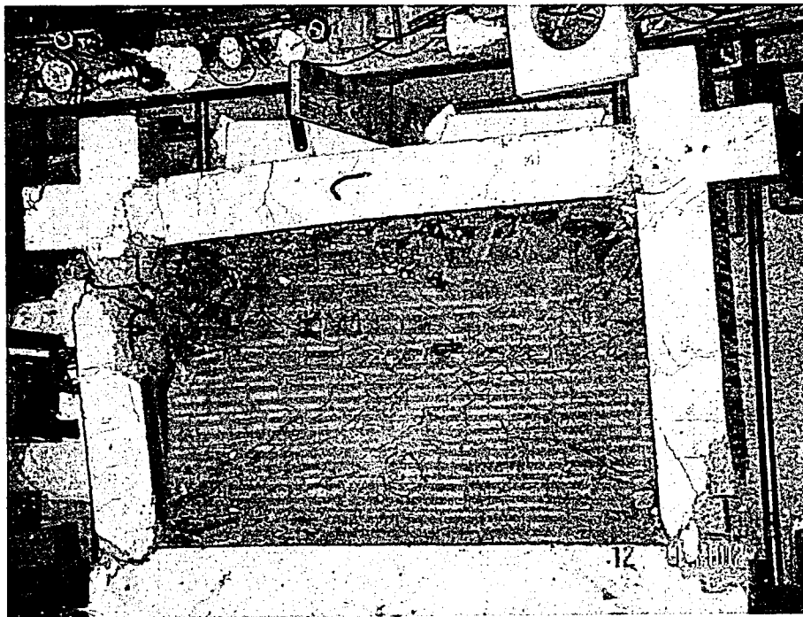
Figure 4.12. Failure of non-ductile HCT infilled frame 07NC-GS
