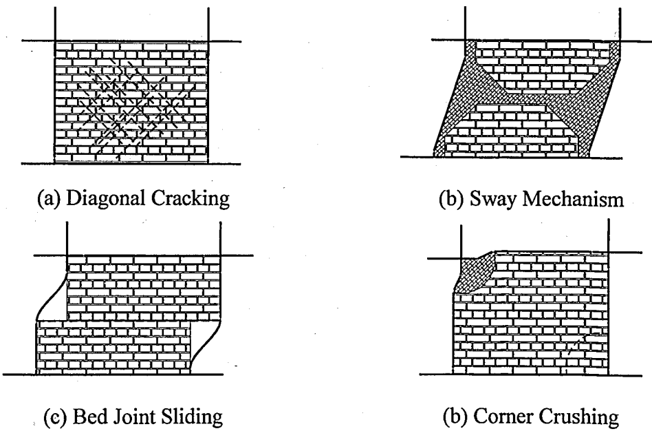
Figure 1.3. Failure mechanisms commonly observed for one story infilled frames
