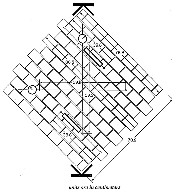
Figure 2.4. Small wall specimen (wallette) diagonal compression test arrangement
