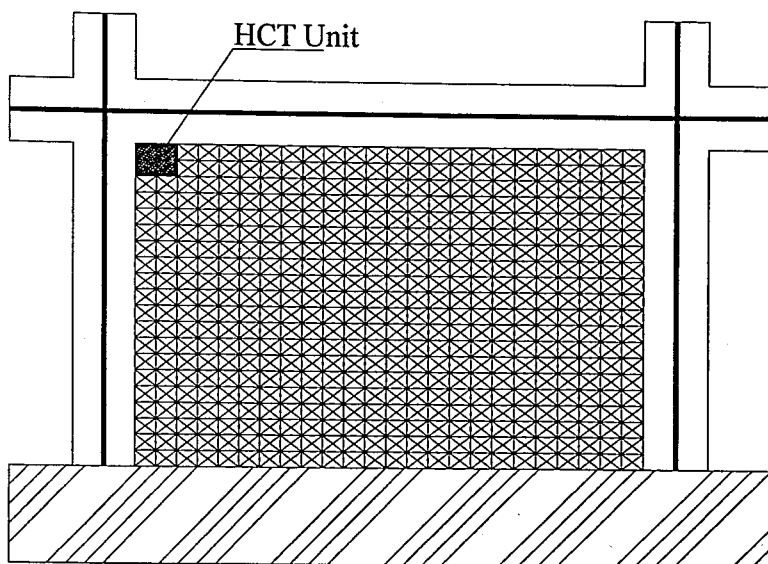
Figure 5.5. Meso-scale model detail for the HCT infill
