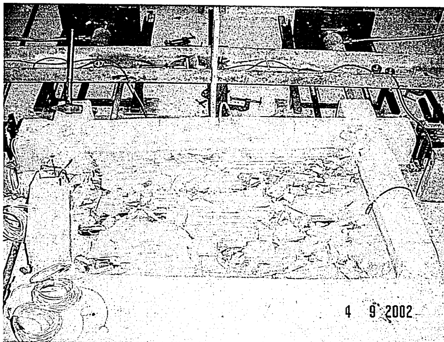
Figure 4.9. Failure of non-ductile HCT infilled frame 01NC-IN
