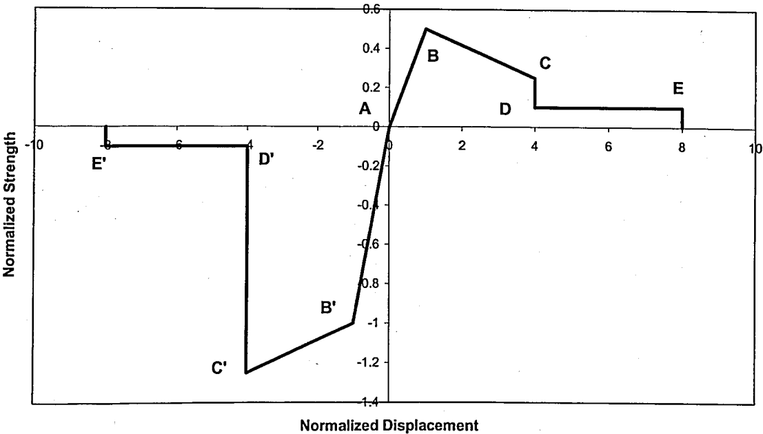
Figure 5.4. Sample curve for backbone point definition
