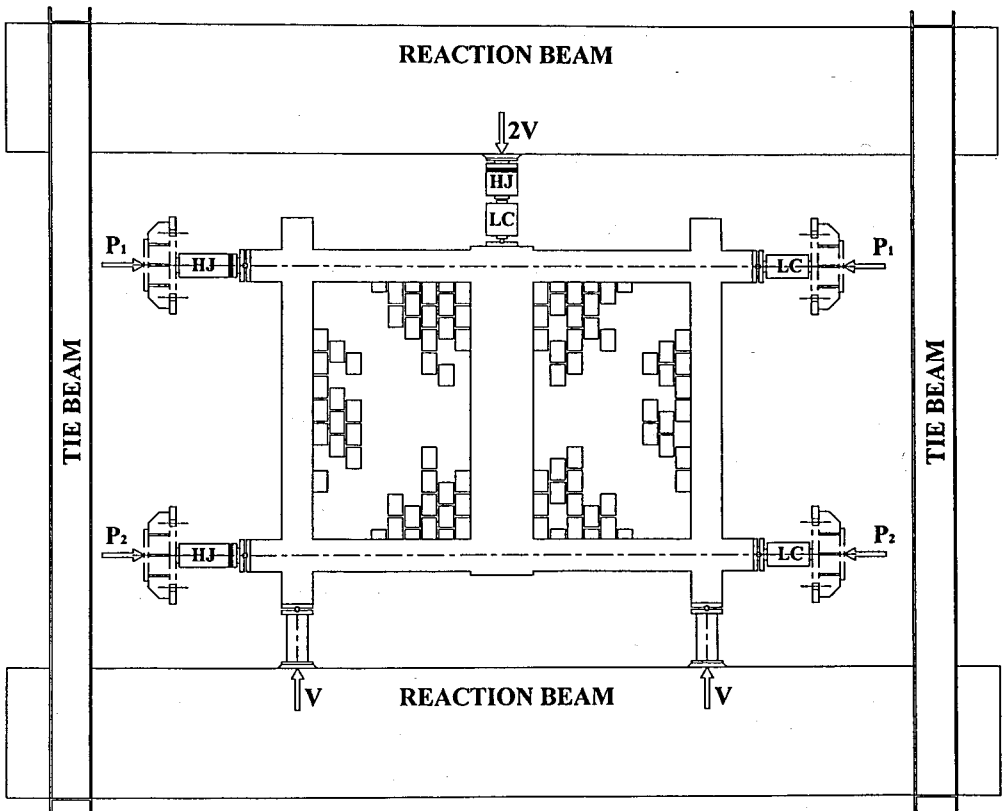
Figure 4.1. Setup for horizontal back-to-back testing of infilled frames
