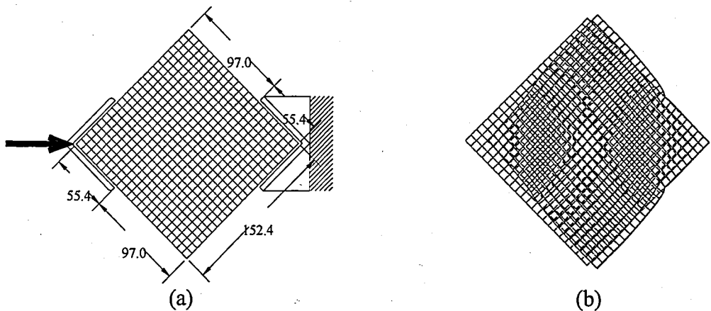
Figure 5.3. Plane stress analysis for accuracy check under 1.9kN
