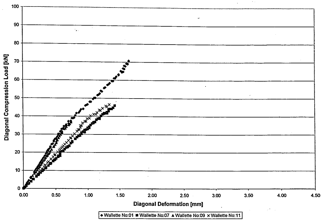
Figure 3.1. Bare Type I brick wall under diagonal compression
