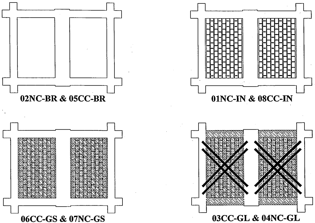
Figure 4.2. Tested specimen types and their code numbers
