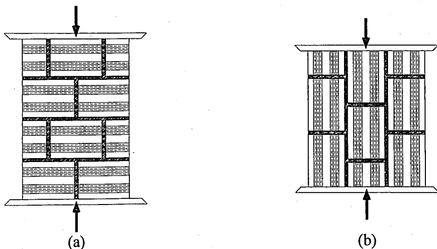
Figure 2.3. Standardized tests on brick prisms
