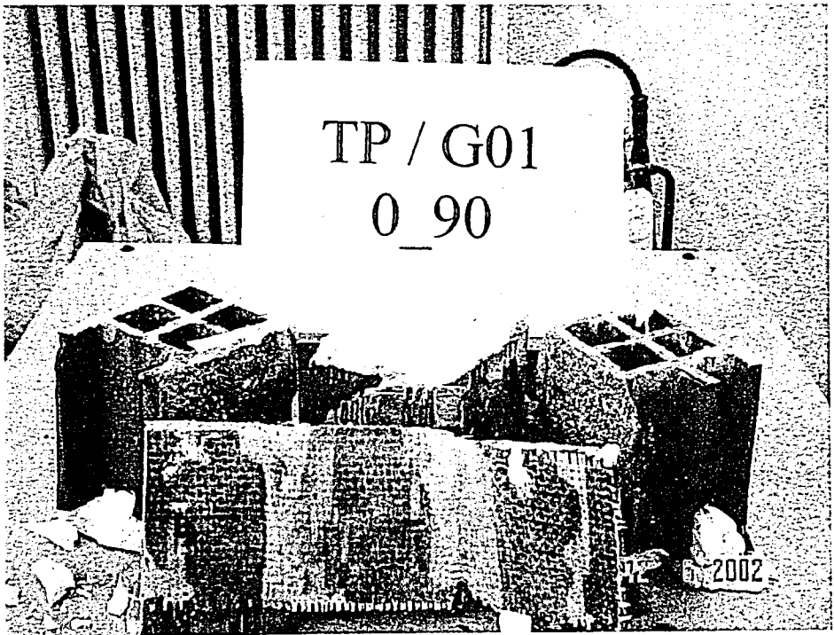
Figure 3.6. Triplet pieces after testing
