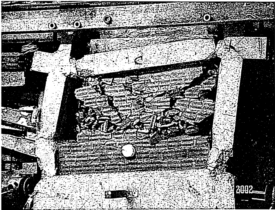
Figure 4.8. Failure of ductile HCT infilled frame 08CC-IN
