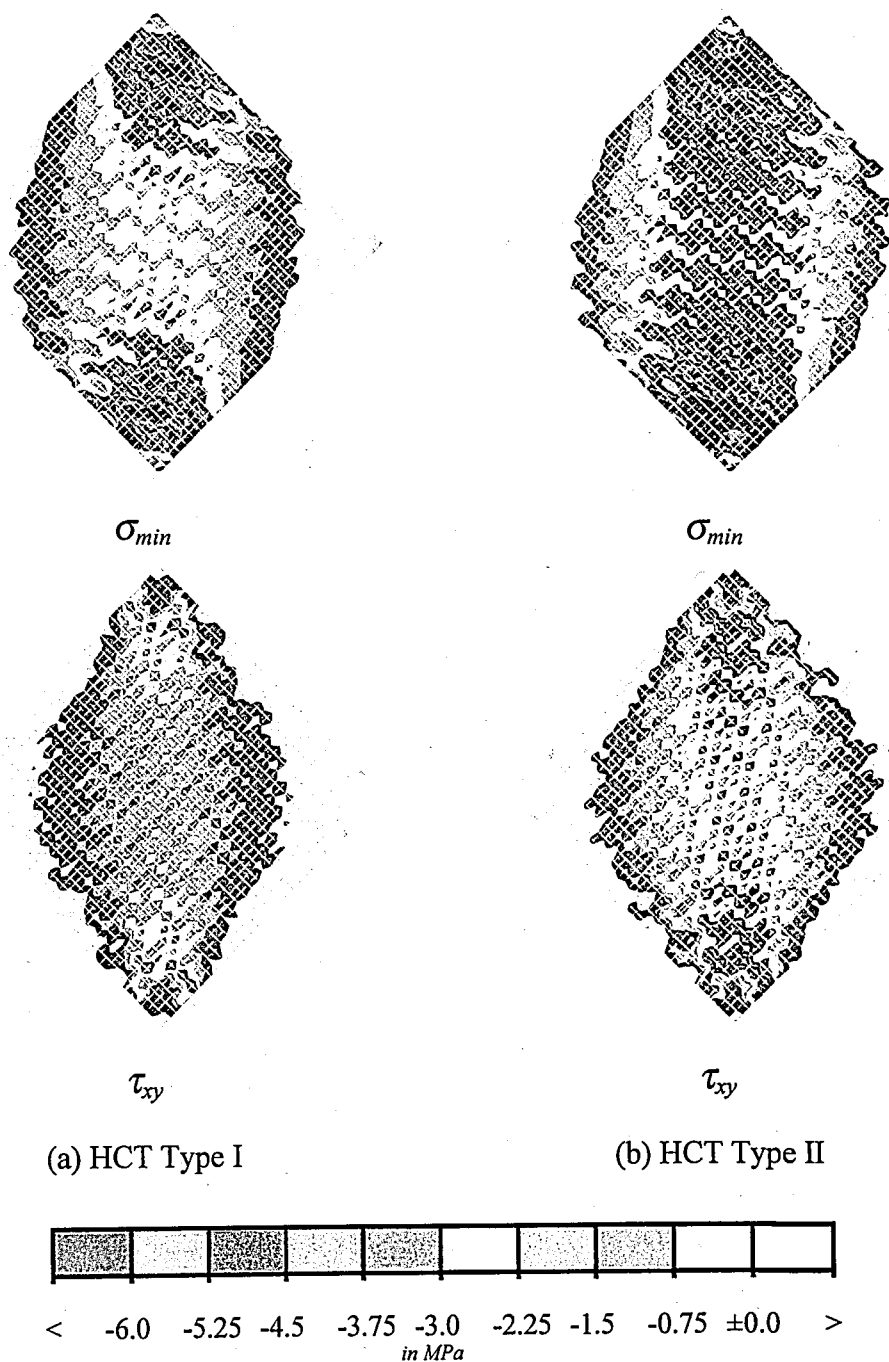
Figure 3.4. Minimum principal and shear stresses in diagonally loaded HCT panels
