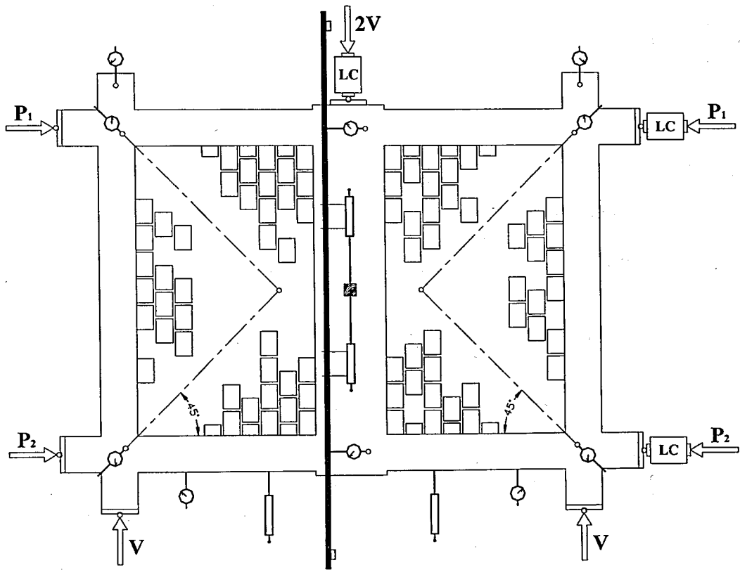
Figure 4.3. Load Introduction and Measurement Devices
