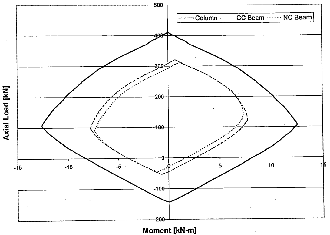
Figure 2.11. Axial force – moment interaction diagrams for columns and beams
