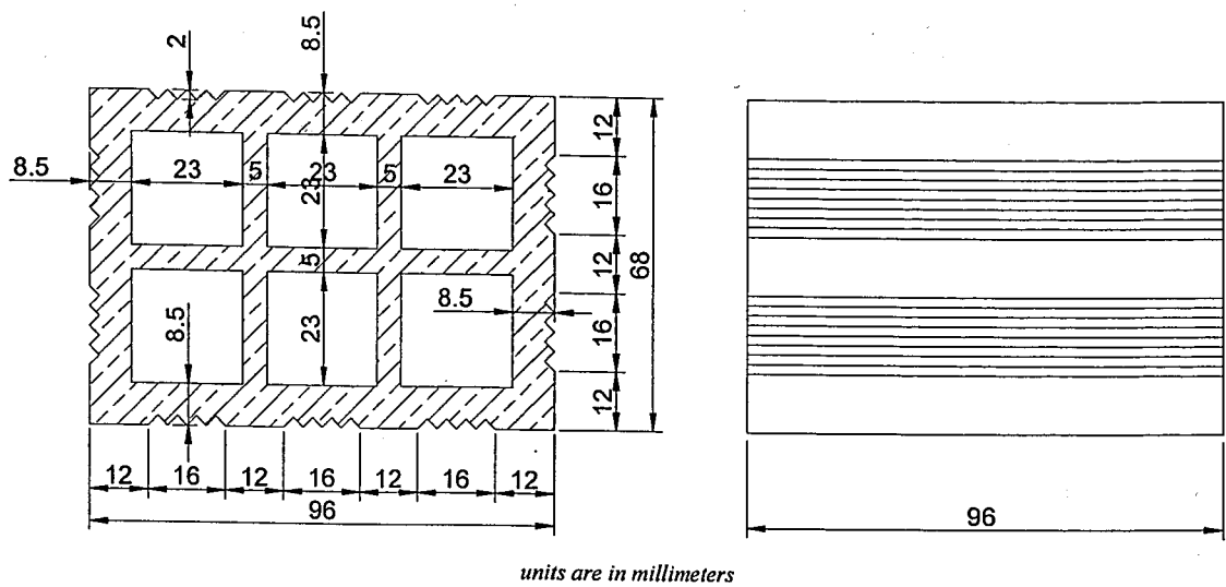
Figure 2.1. HCT Type I – Heavy hollow clay tile unit with thick shells
