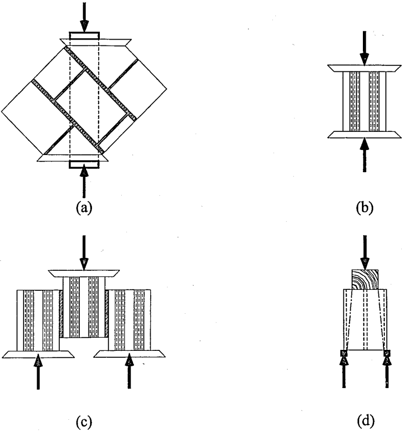
Figure 2.5. Non-standard hollow clay tile masonry tests
