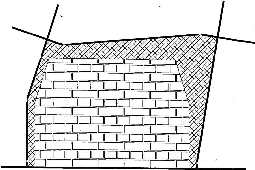
Figure 4.16. Sway mechanism with column mid-height pivoting
