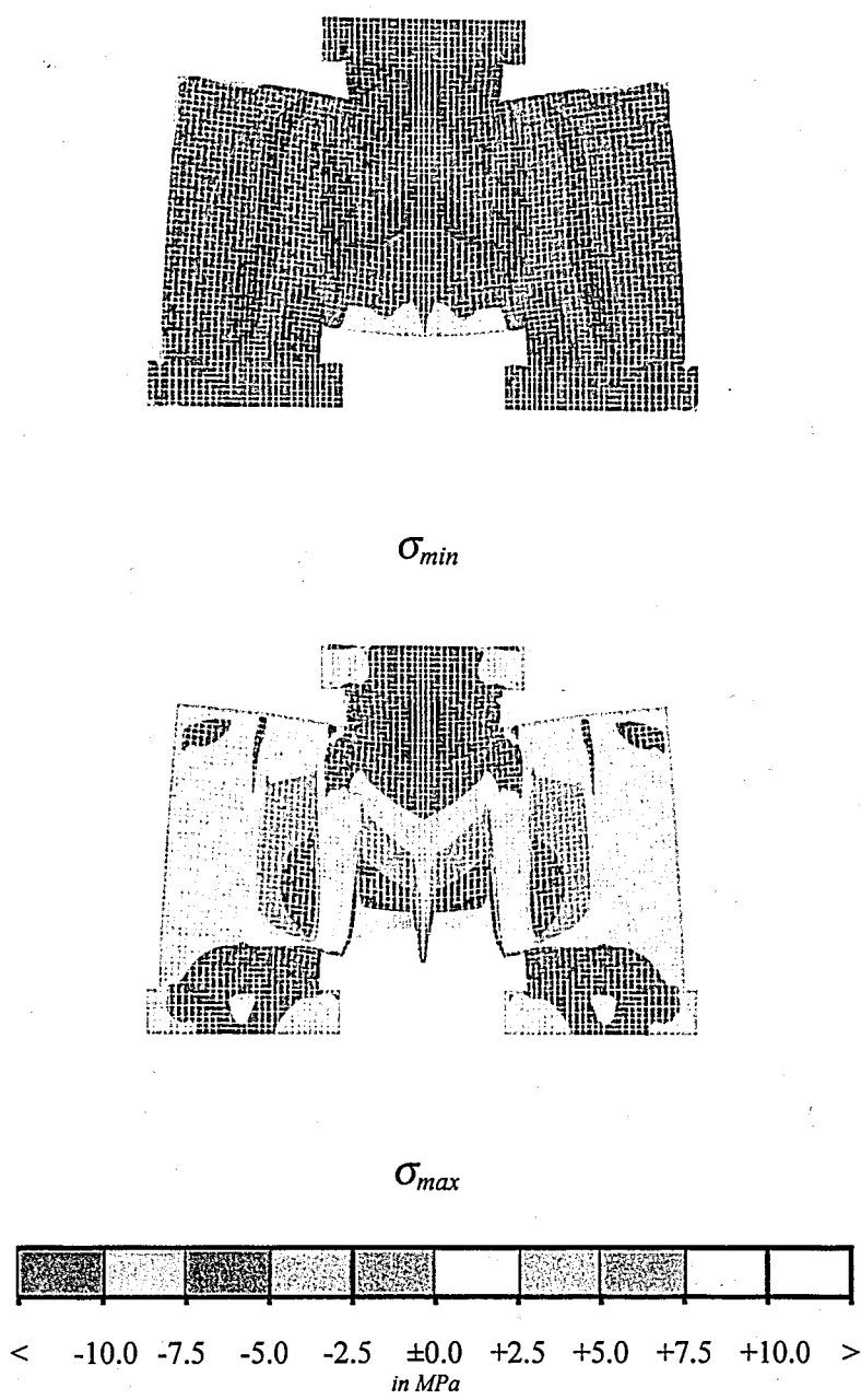
Figure 3.7. Plane-stress analysis results of HCT triplet under 30kN
