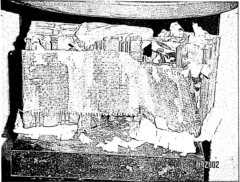
Figure 3.5. Glass-sheeted triplet after testing
