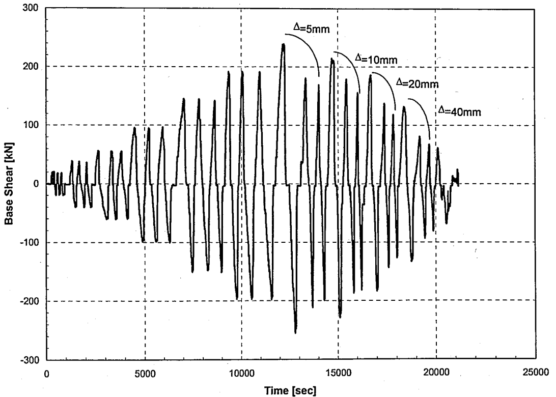
Figure 4.4. Lateral loading time-history of 01NC-IN
