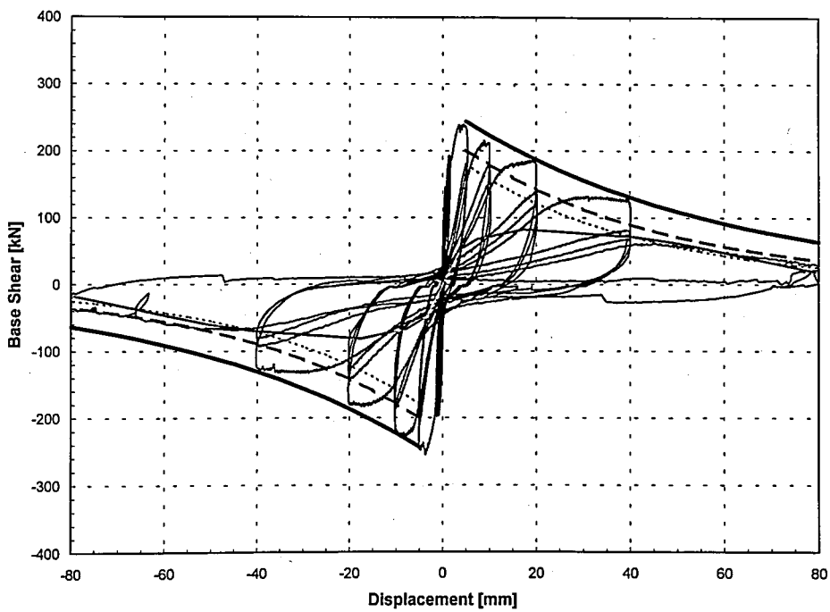
Figure 4.17. Force-displacement trace of 08CC-IN
