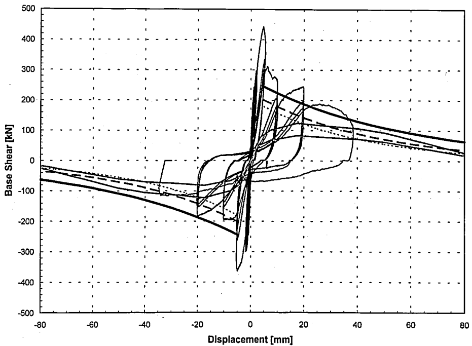
Figure 4.21. Force-displacement trace of 03CC-GL
