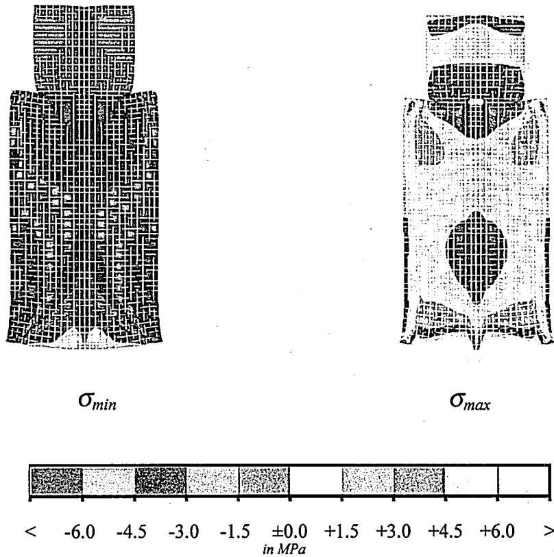
Figure 3.8. Plane-stress analysis results of HCT web shear test under 10kN
