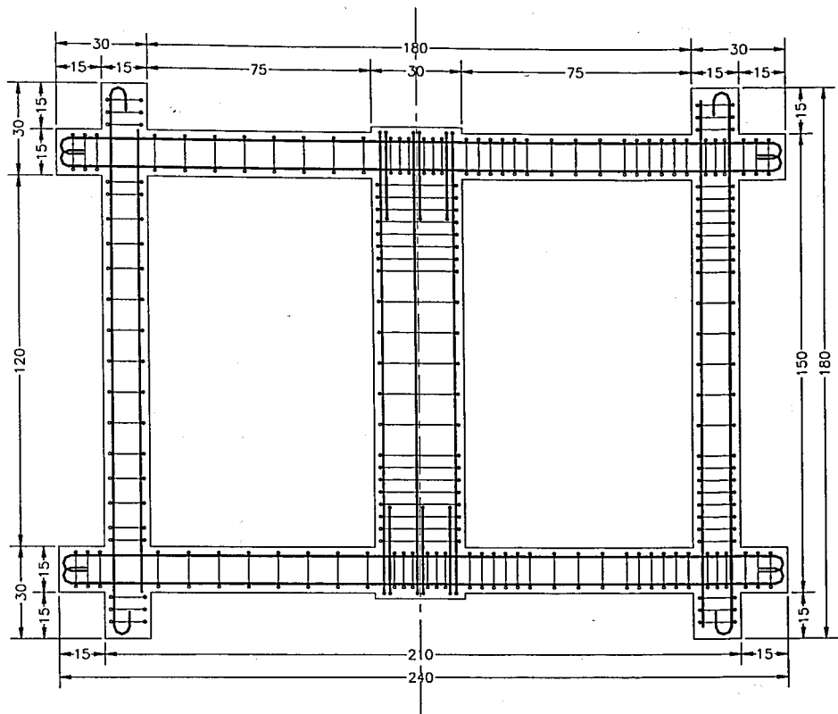
Figure 2.7. Frame specimen overall dimensions
