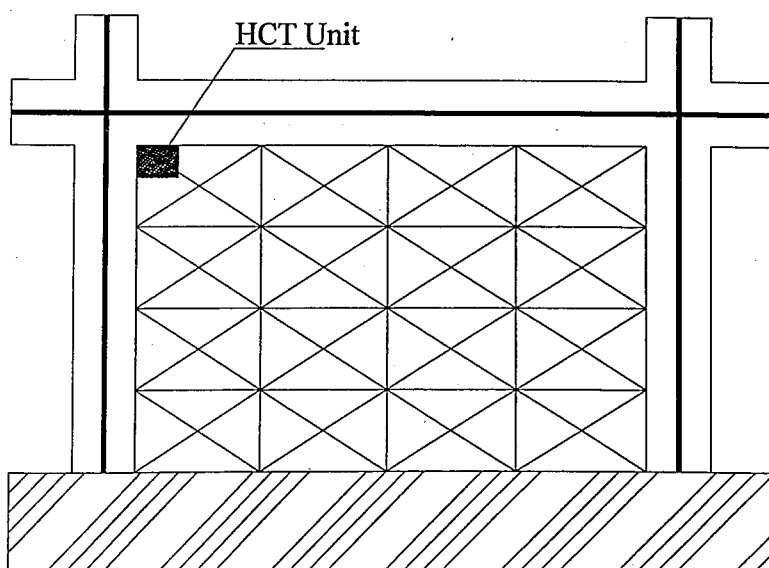
Figure 5.6. Macro-scale model detail for the HCT infill
