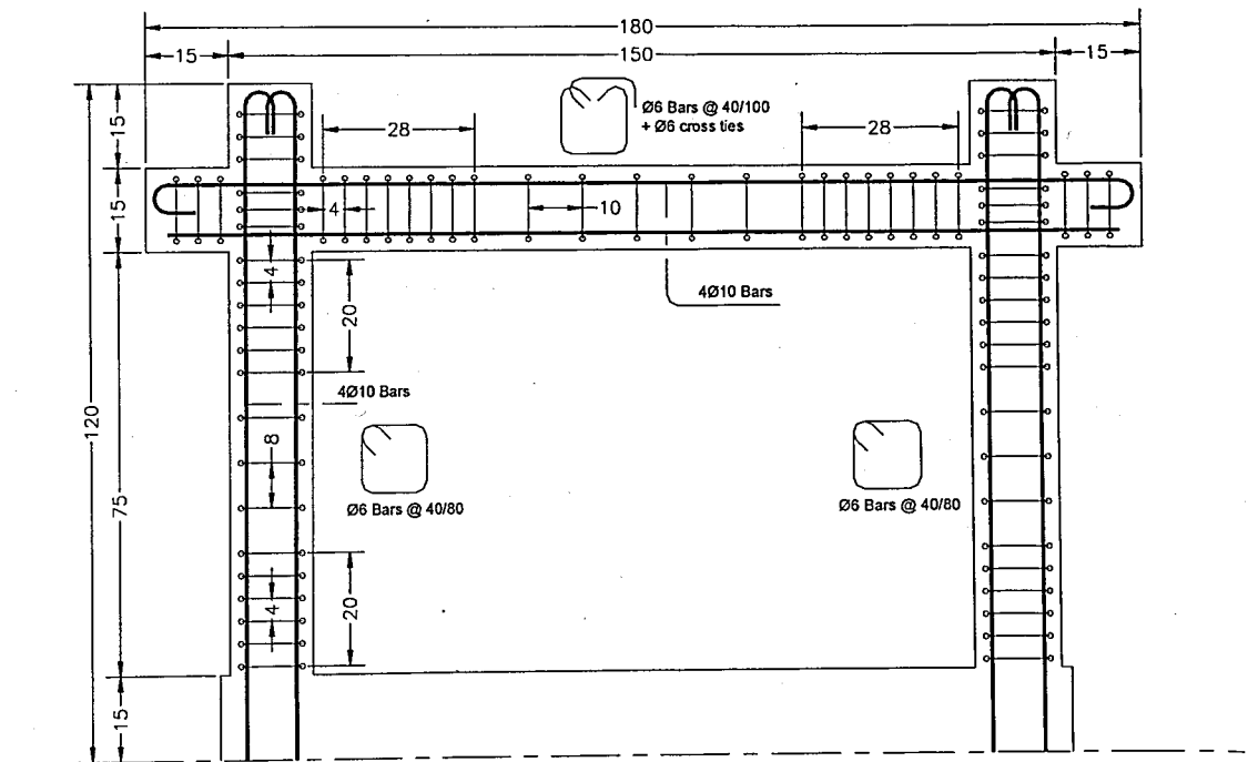
Figure 2.8. Code-compliant ductile frame detailing
