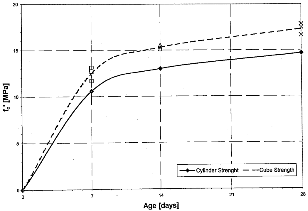
Figure 2.10. Strength development of the concrete used
