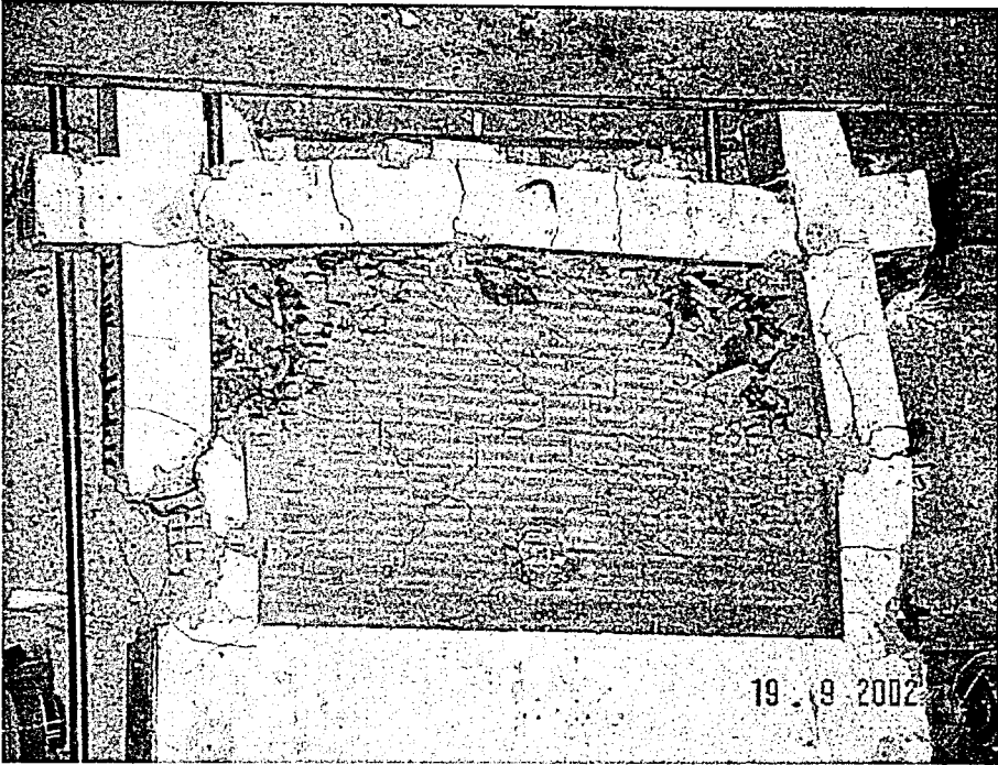
Figure 4.14. Failure of ductile HCT infilled frame 03CC-GL
