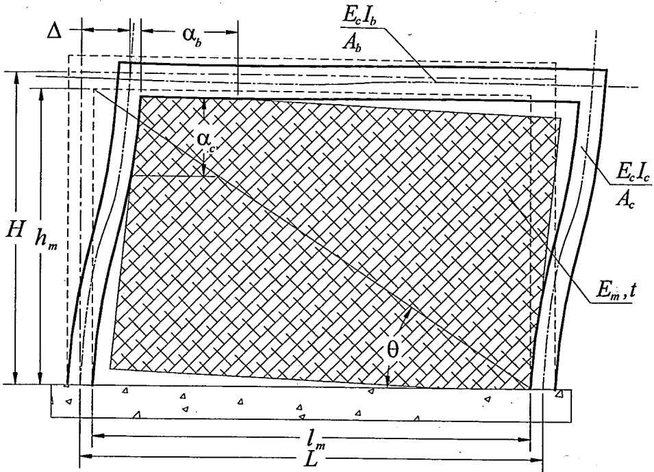
Figure 1.1. Infilled frame geometry and notation
