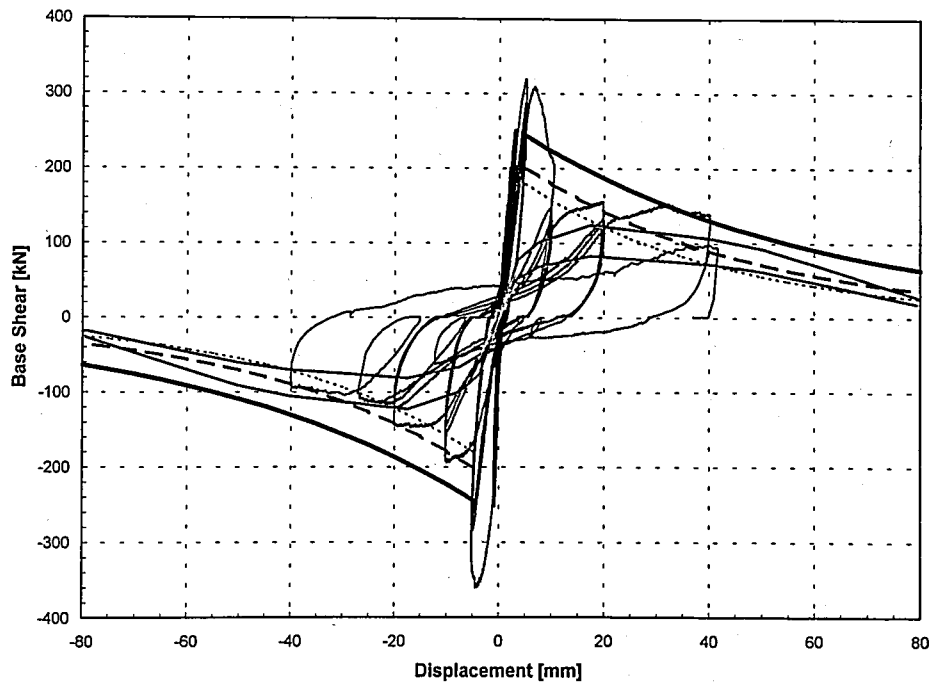
Envelope of first (—), second (· ·), and third (- -) cycles of 01NC-IN & Envelope of 02NC-BR (—) and plastic collapse mode (—)
