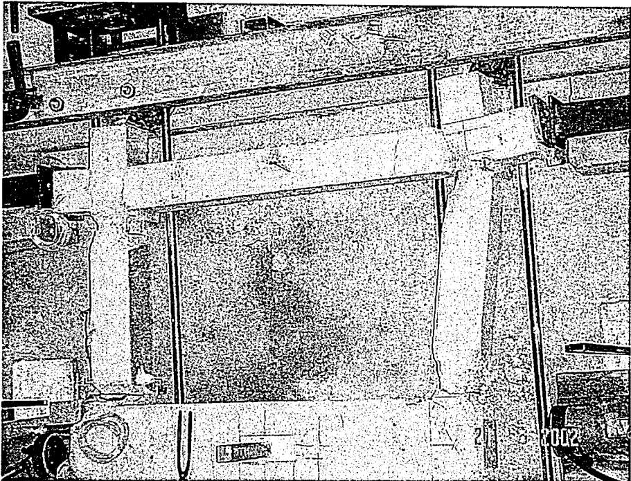
Figure 4.7. Failure of non-ductile bare frame 02NC-BR
