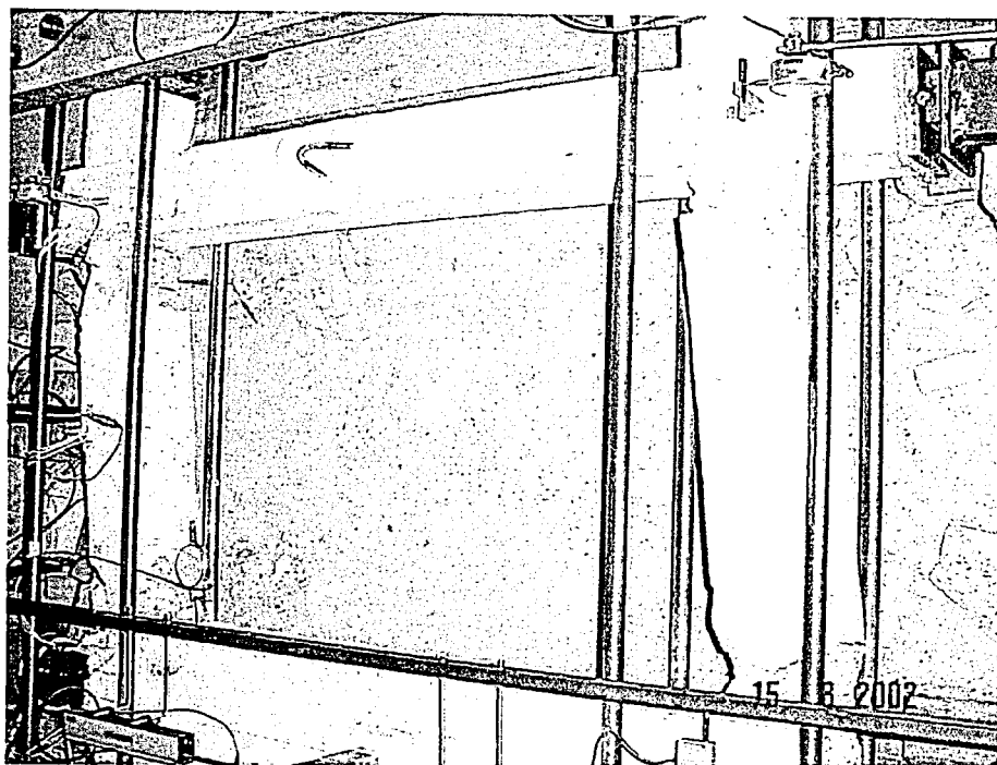
Figure 4.6. Failure of ductile bare frame 05CC-BR
