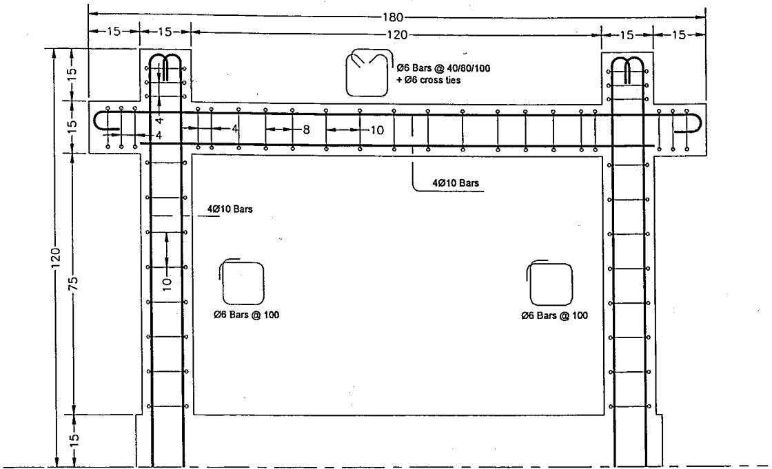
Figure 2.9. Non-compliant non-ductile frame detailing
