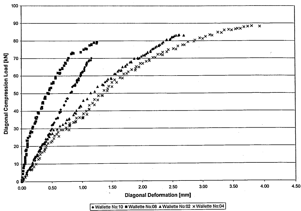
Figure 3.2. Glass-sheeted Type I brick wall under diagonal compression
