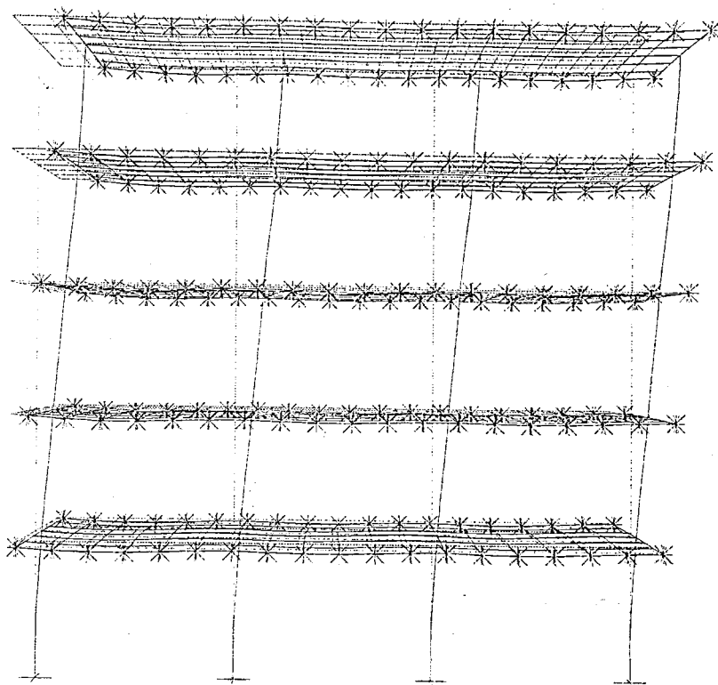
Figure 2.6. Plane frame building model with symmetry boundary conditions
