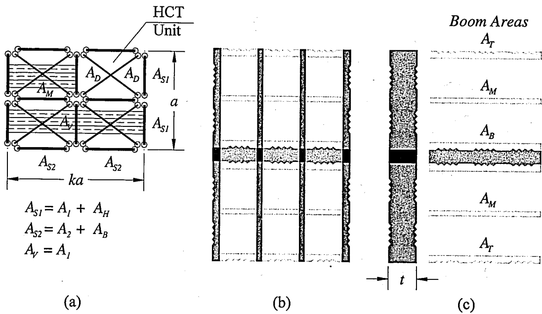
Figure 5.2. Hrennikoff truss equivalent of plane stress element
