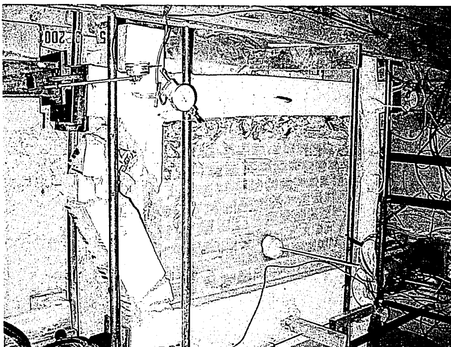
Figure 4.11. Failure of ductile HCT infilled frame 06CC-GS
