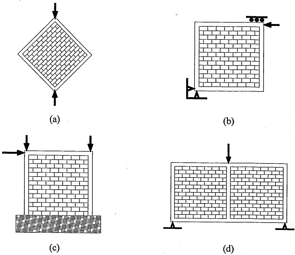
Figure 1.2. Loading arrangements frequently used for infilled frame testing
