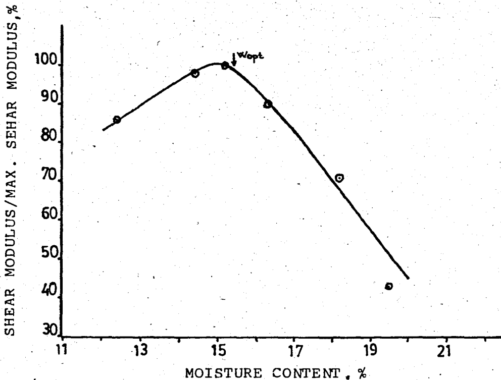
FIG 5.10 Variation of shear modulus and normalized Shear Modulus with Moisture Content for İçerenköy Sample 4
