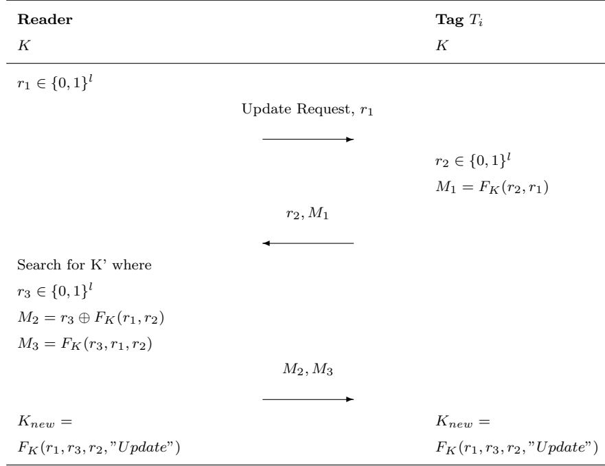
Figure 5.7. Dimitriou's protocol
