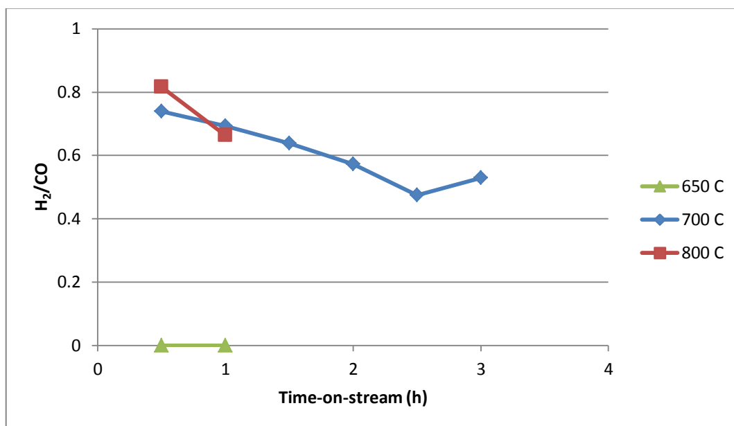
Figure 4.6. H 2 /CO ratio with respect to time-on-stream for CH 4 /CO 2 feed ratio of 1/1.
