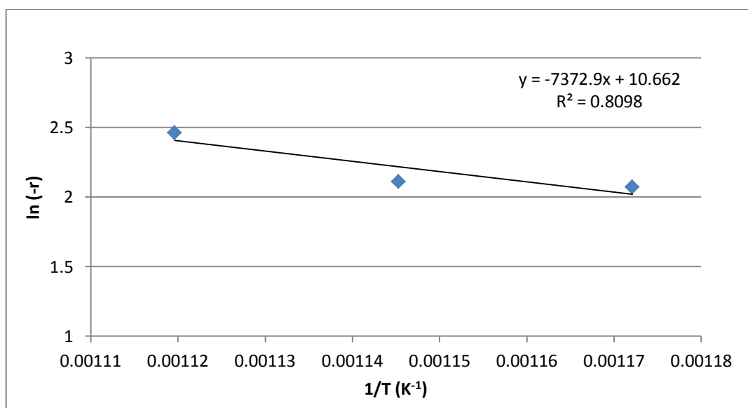
Figure 4.16. Arrhenius plot for CH 4 .
