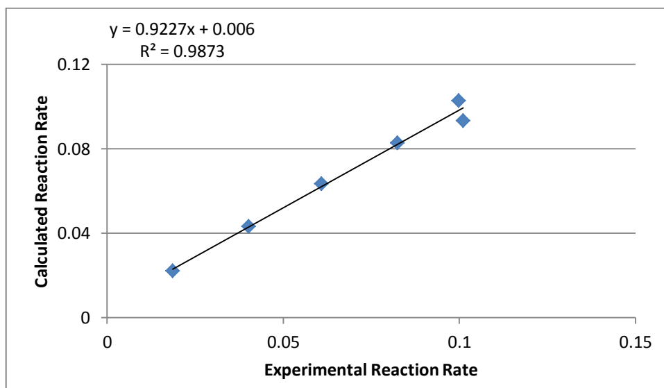
Figure D.2. Experimental and calculated reaction rates for Model 3.
