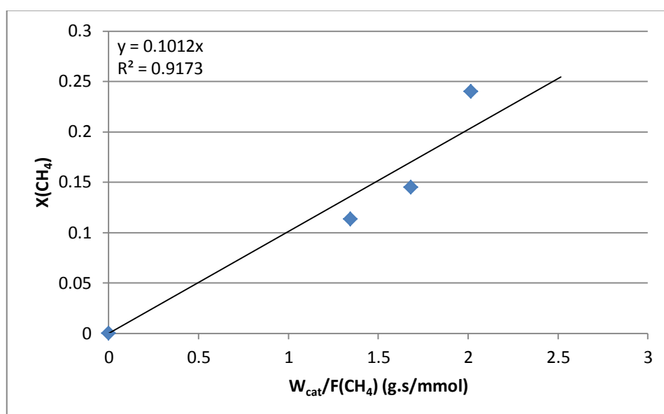
Figure A.5. Fractional \text{CH}_4 conversion vs. residence time graph of experiments 13-15.
