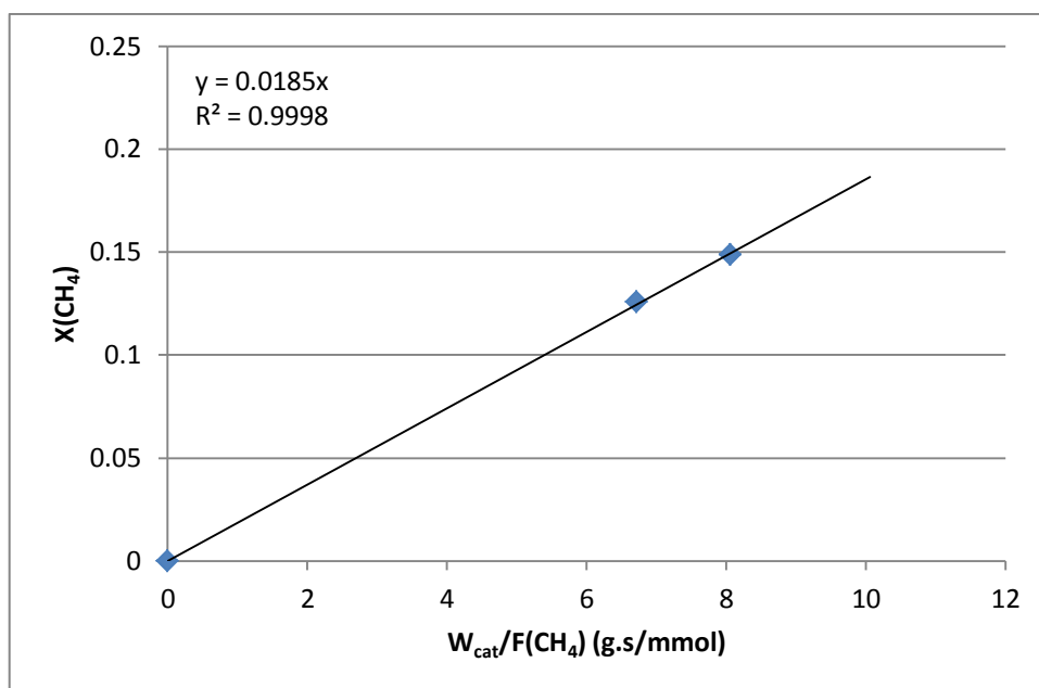
Figure A.1. Fractional CH 4 conversion vs. residence time graph of experiments 1-3.
