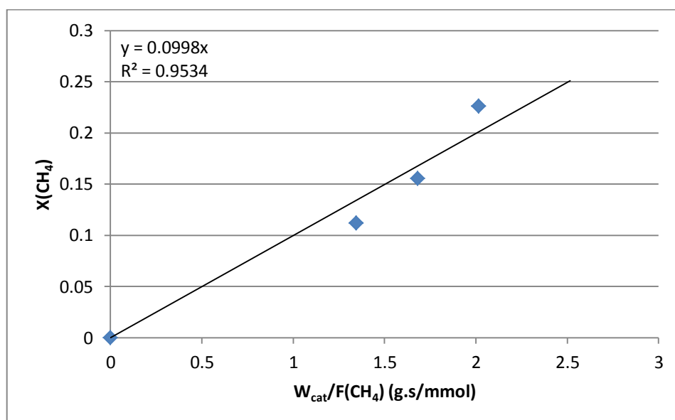
Figure A.6. Fractional \text{CH}_4 conversion vs. residence time graph of experiments 16-18.
