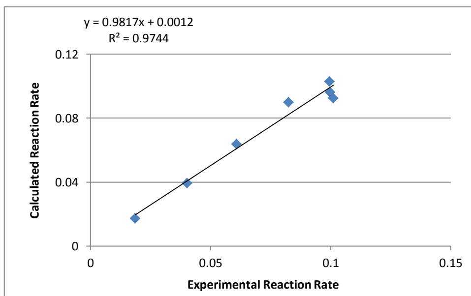
Figure B.1. Experimental and calculated reaction rates for power-law type CDRM kinetics.
