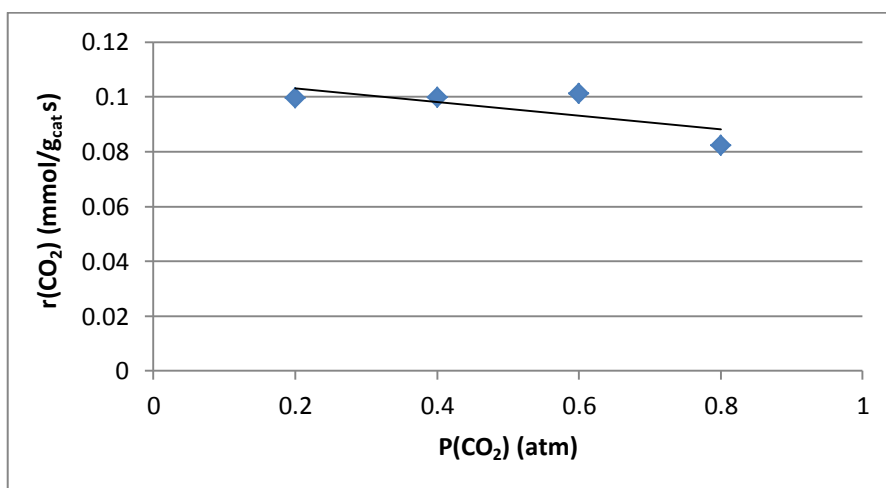
Figure 4.19. Variation of the reaction rate as a function of carbon dioxide partial pressure.
