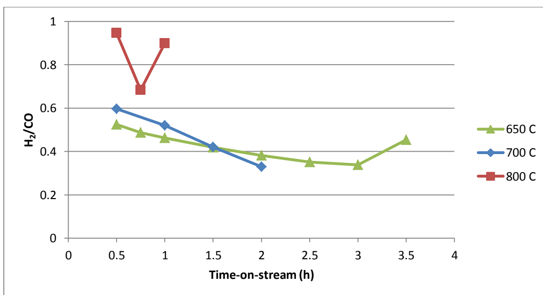
Figure 4.9. H 2 /CO product ratio with respect to time-on-stream for CH 4 /CO 2 feed ratio of 1/2.
