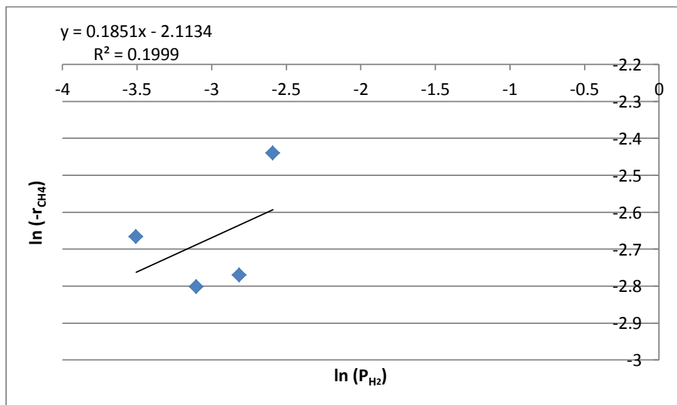
Figure 4.21. The effect of H 2 partial pressure on CDRM rate.
