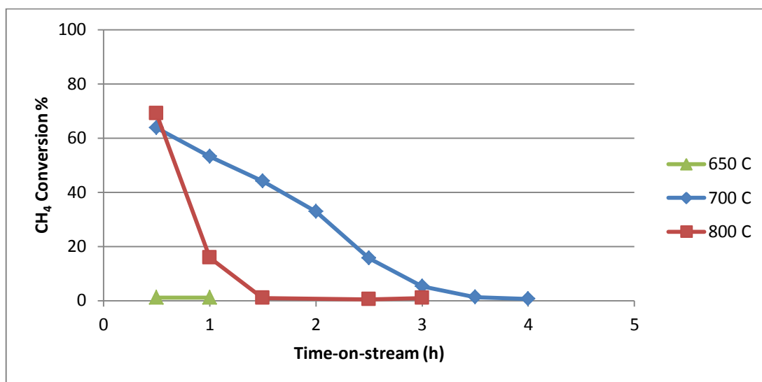
Figure 4.4. CH 4 conversion with respect to time-on-stream for CH 4 /CO 2 feed ratio of 1/1.
