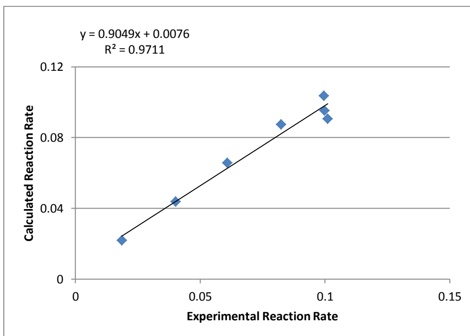
Figure D.4. Experimental and calculated reaction rates for Model 7.
