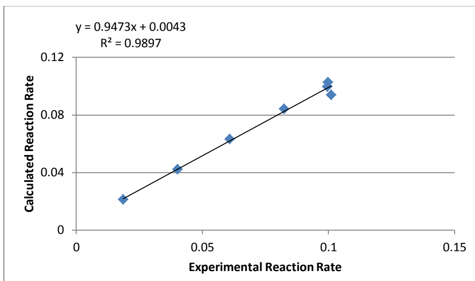
Figure D.3. Experimental and calculated reaction rates for Model 4.
