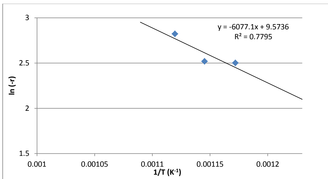
Figure 4.17. Arrhenius plot for CO 2 .
