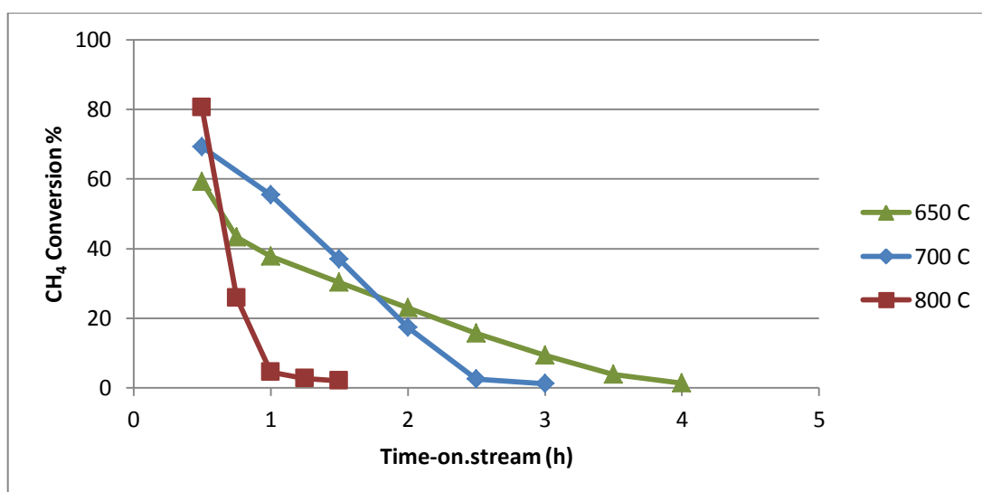
Figure 4.7. CH 4 conversion with respect to time-on-stream for CH 4 /CO 2 feed ratio of 1/2.
