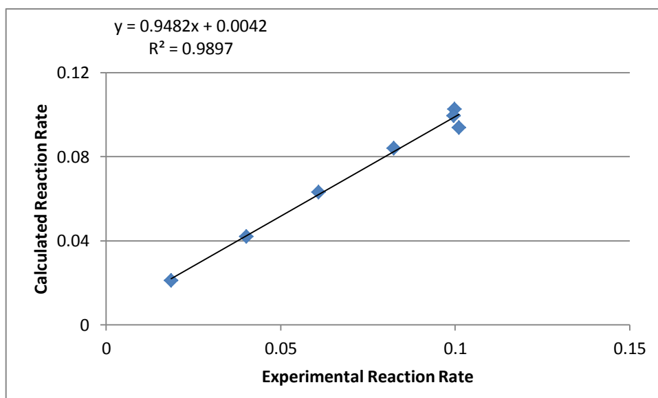
Figure D.1. Experimental and calculated reaction rates for Model 1.
