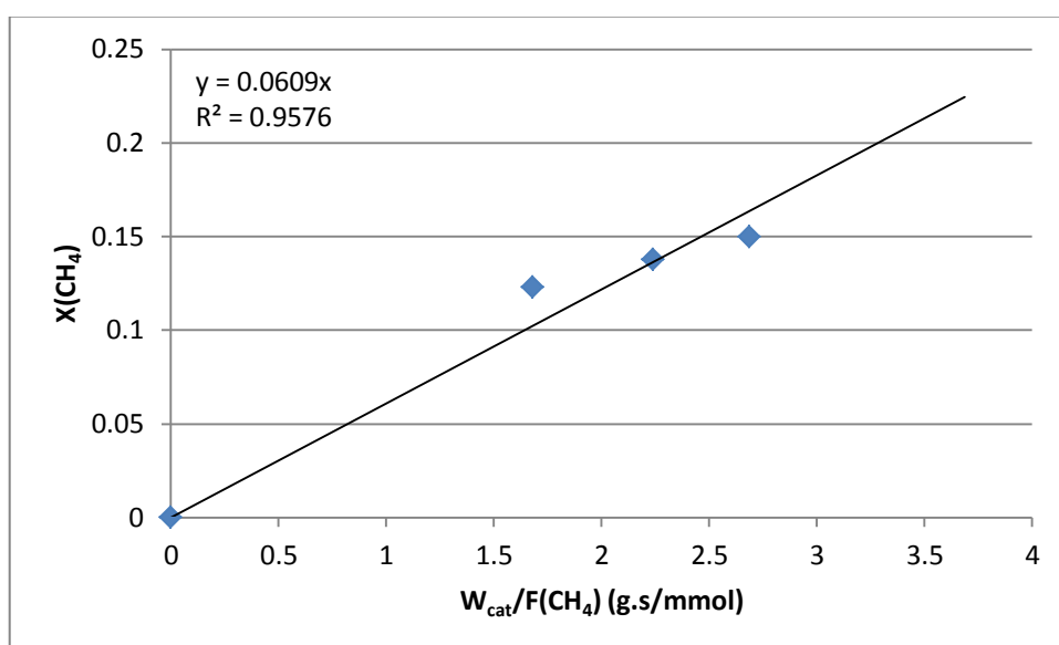
Figure A.3. Fractional \text{CH}_4 conversion vs. residence time graph of experiments 7-9.
