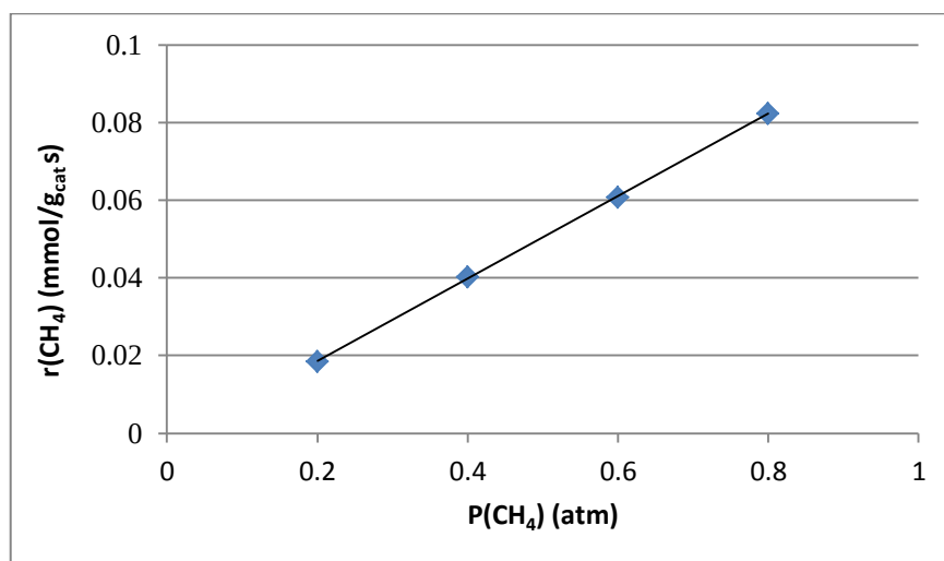
Figure 4.18. Variation of the reaction rate as a function of methane partial pressure.
