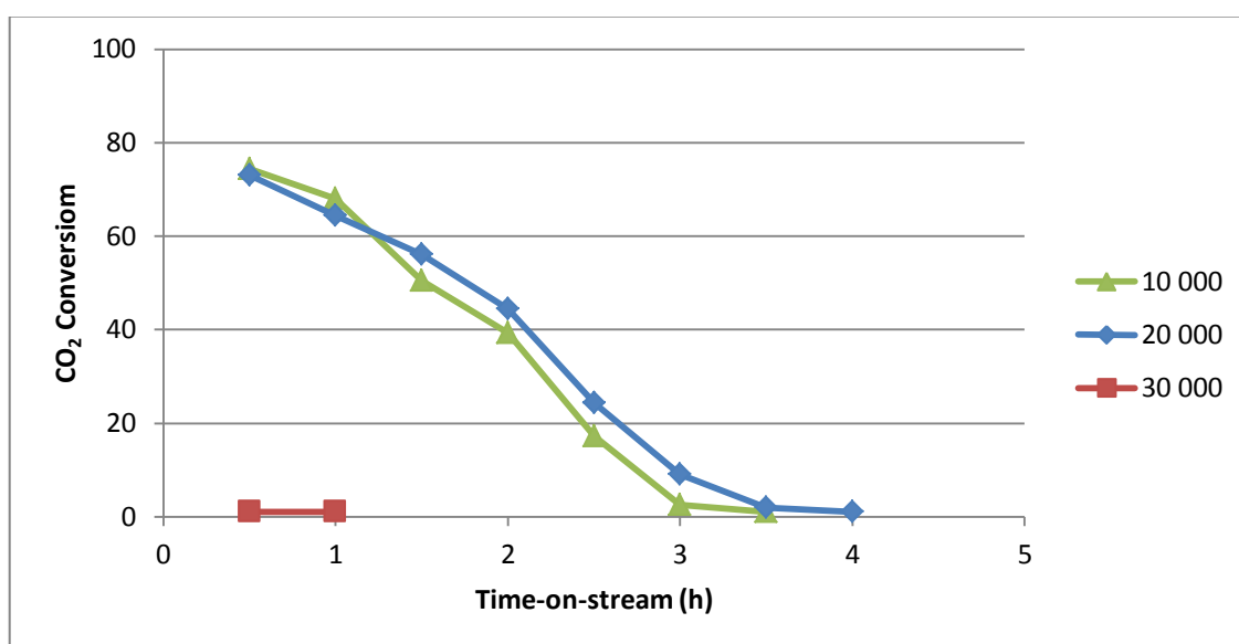
Figure 4.11. CO 2 conversion with respect to time-on-stream for CH 4 /CO 2 feed ratio of 1/1 T=700°C.
