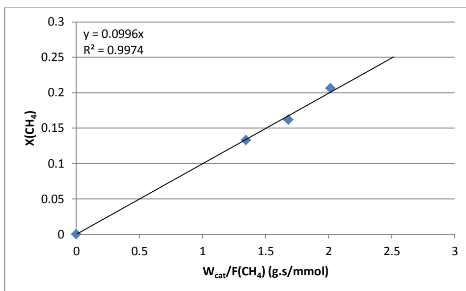
Figure A.7. Fractional \text{CH}_4 conversion vs. residence time graph of experiments 19-21.
