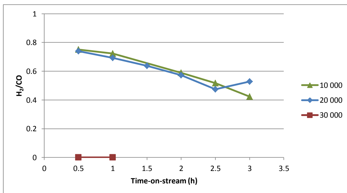
Figure 4.12. H 2 /CO product ratio with respect to time-on-stream for CH 4 /CO 2 feed ratio of 1/1 T=700°C.
