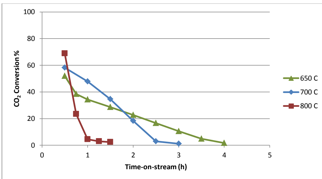
Figure 4.8. CO 2 conversion with respect to time-on-stream for CH 4 /CO 2 feed ratio of 1/2.
