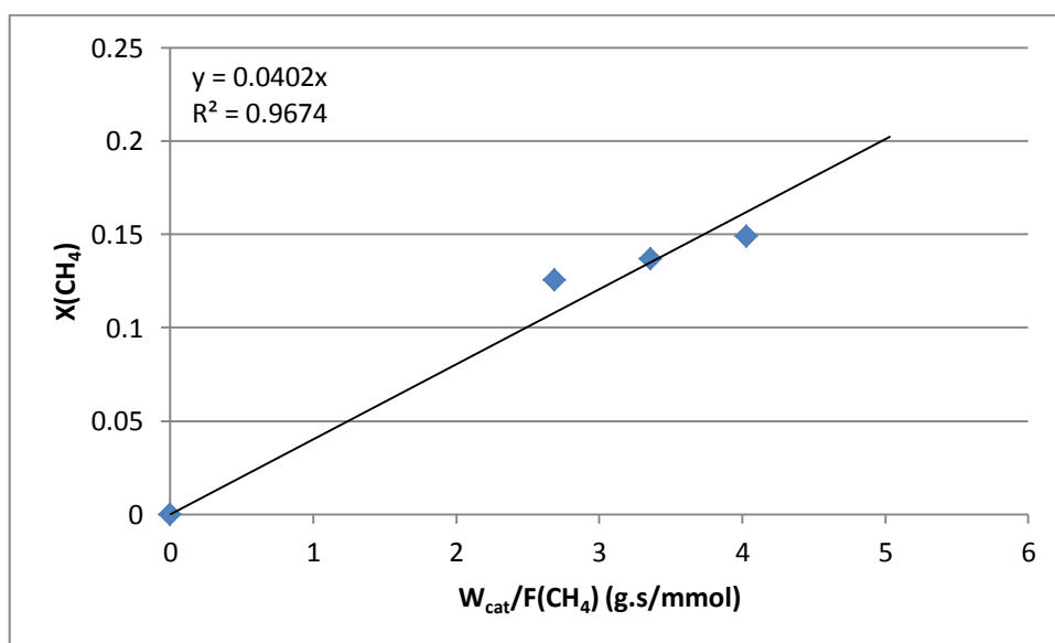
Figure A.2. Fractional CH 4 conversion vs. residence time graph of experiments 4-6.
