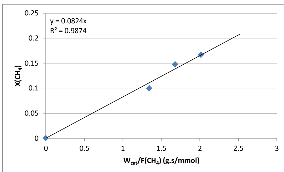
Figure A.4. Fractional \text{CH}_4 conversion vs. residence time graph of experiments 10-12.
