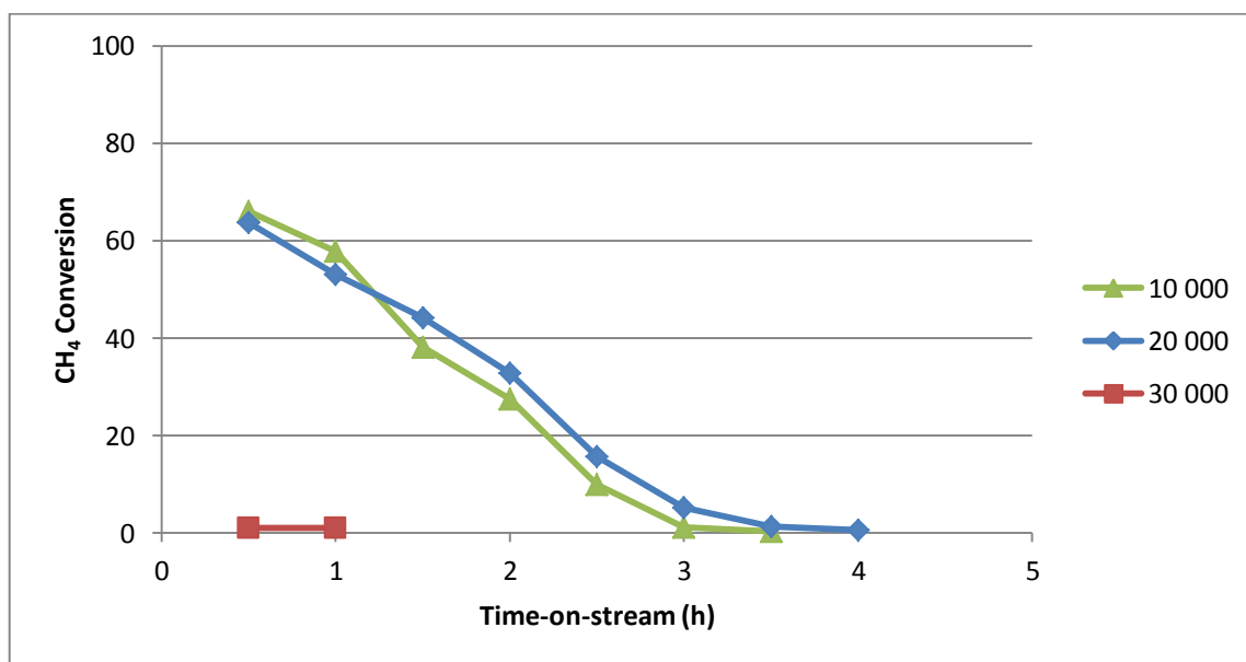
Figure 4.10. \text{CH}_4 conversion with respect to time-on-stream for \text{CH}_4/\text{CO}_2 feed ratio of 1/1 T = 700^\circ\text{C} .
