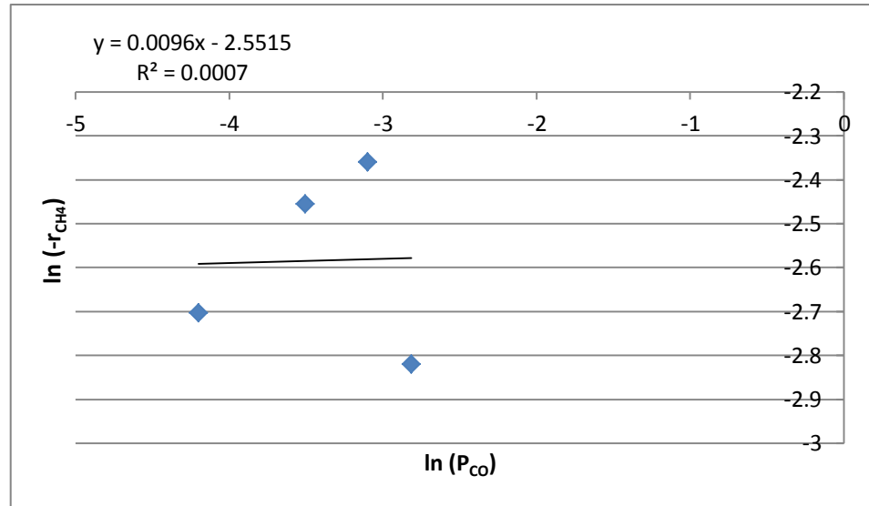
Figure 4.20. The effect of CO partial pressure on CDRM rate.
