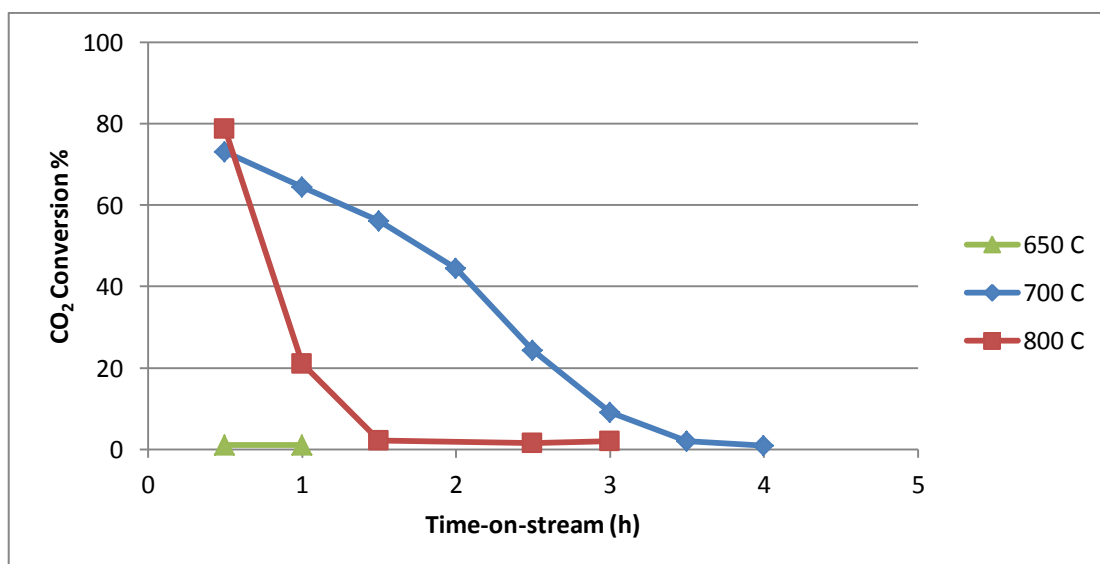
Figure 4.5. CO 2 conversion with respect to time-on-stream for CH 4 /CO 2 feed ratio of 1/1.
