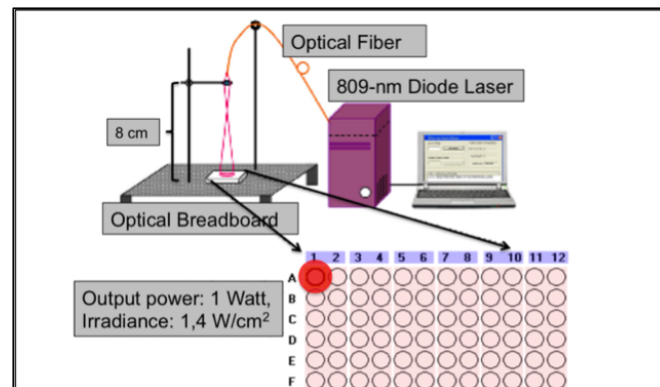
Figure 3.1 Laser Setup. 809-nm diode laser is a computer-controlled system. The optical fiber of the laser system was adjusted to apply 1.4 \text{ W/cm}^2 on the plate surface. The distance between the laser probe and the plate surface was 8 cm.
