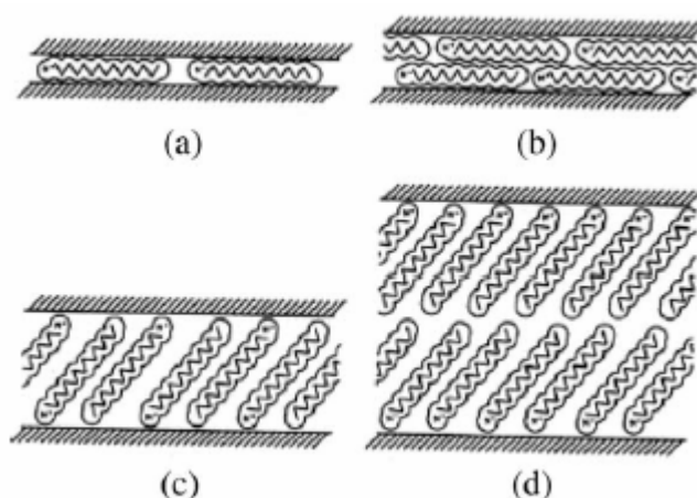
Figure 1.3. Arrangements of alkylammonium ions in mica-type layered silicates with different layer charges. Hatch areas are silicate layers [32]
