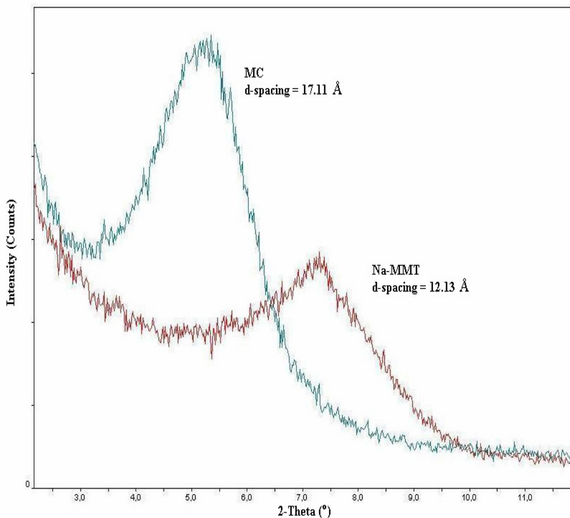
Figure 3.4. XRD patterns of Na-MMT and MC
