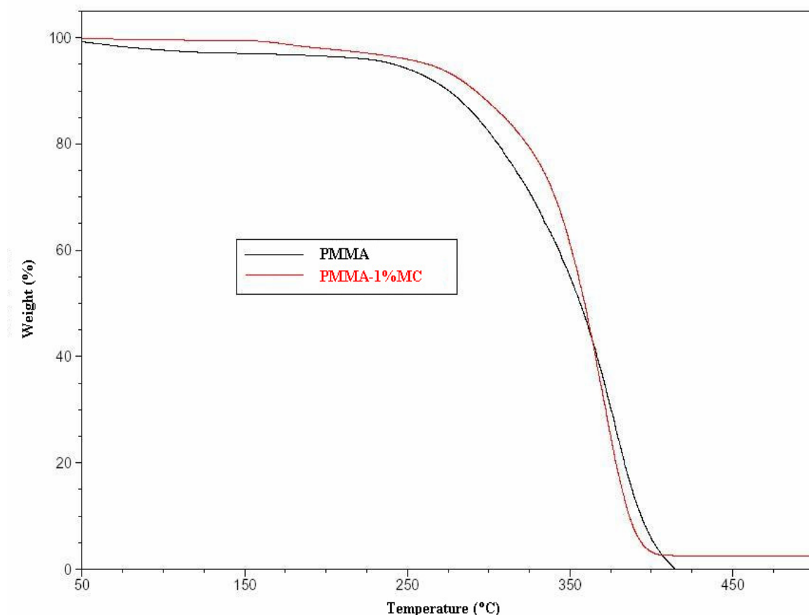
Figure 3.7 TGA graphs of PMMA and PMMA-1%MC
