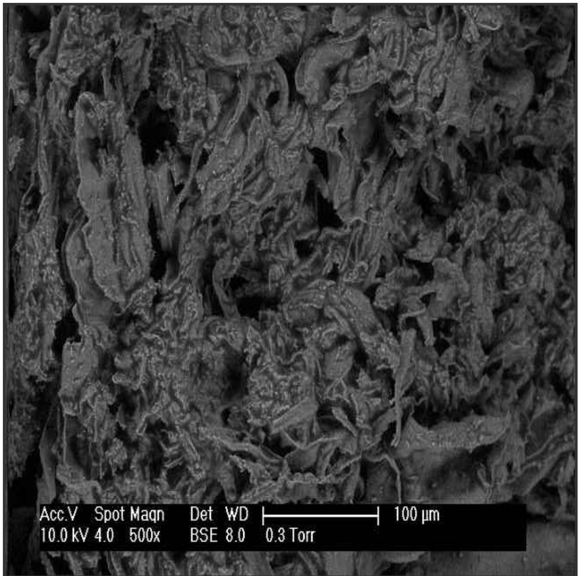
Figure 3.14 SEM image of fracture surface of PMMA-1%MC
