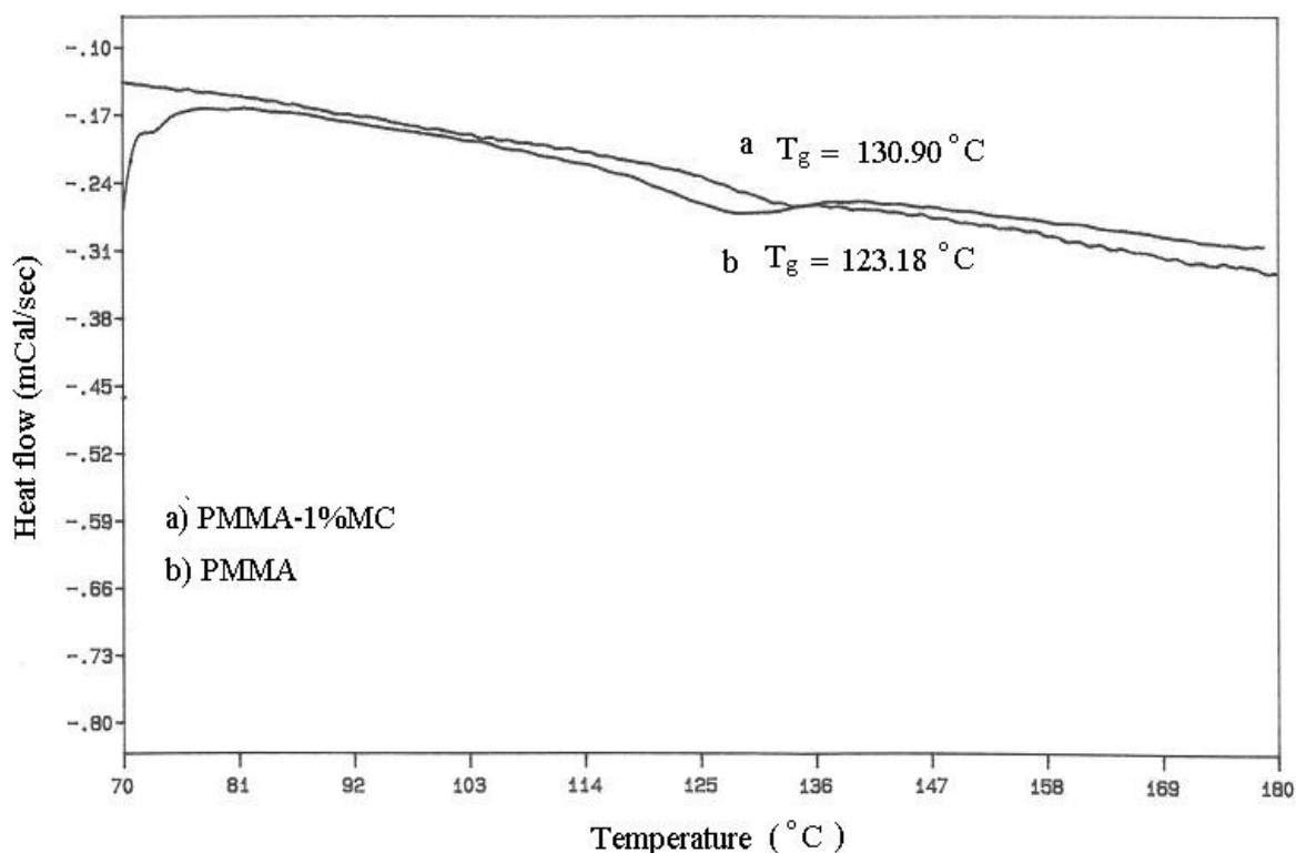
Figure 3.8 DSC graphs of PMMA and PMMA-1%MC
