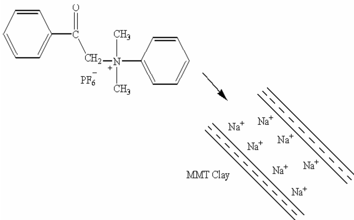
Figure 3.3. Modification of Na-MMT with PDA
