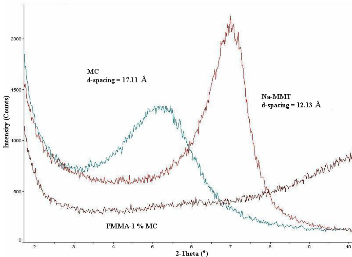
Figure 3.6 XRD patterns of Na-MMT, MC and PMMA-1%MC
