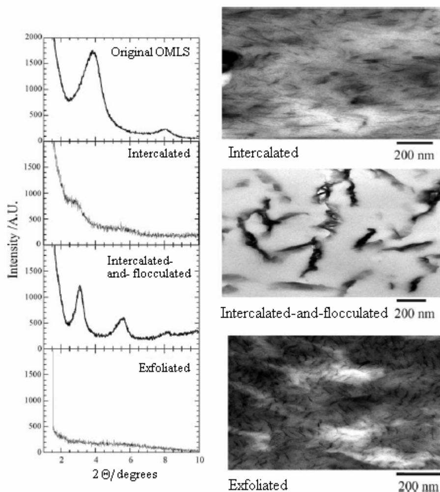
Figure 1.7. (a) WAXD patterns and (b) TEM images of three different types of nanocomposites [6]
