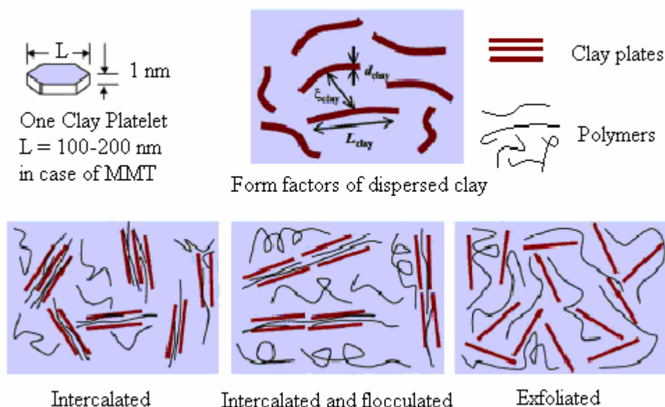
Figure 1.5. Schematically illustration of three different types of thermodynamically achievable PLS nanocomposites [34]
