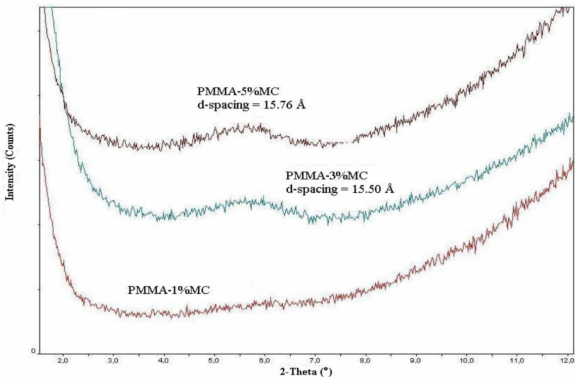
Figure 3.10. XRD patterns of nanocomposites
