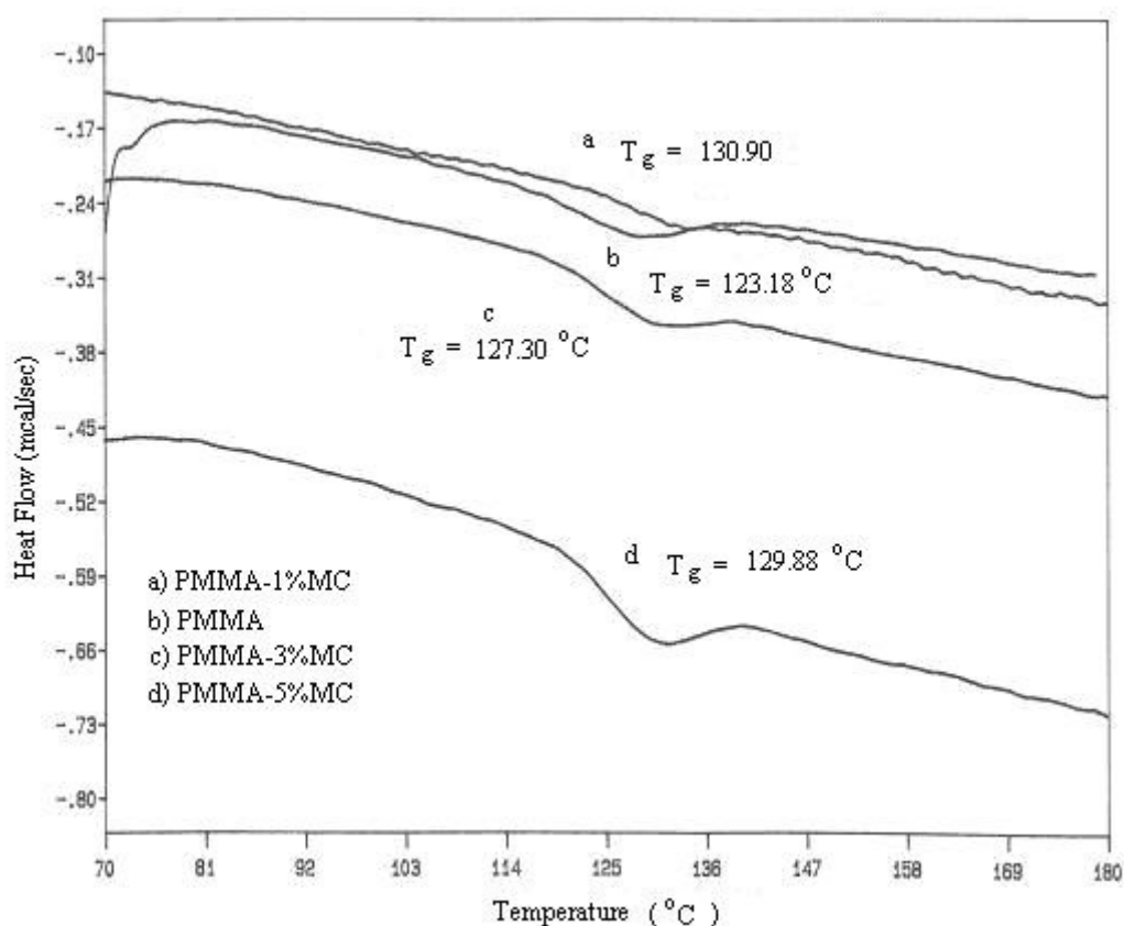
Figure 3.12 DSC graphs of PMMA and nanocomposites
