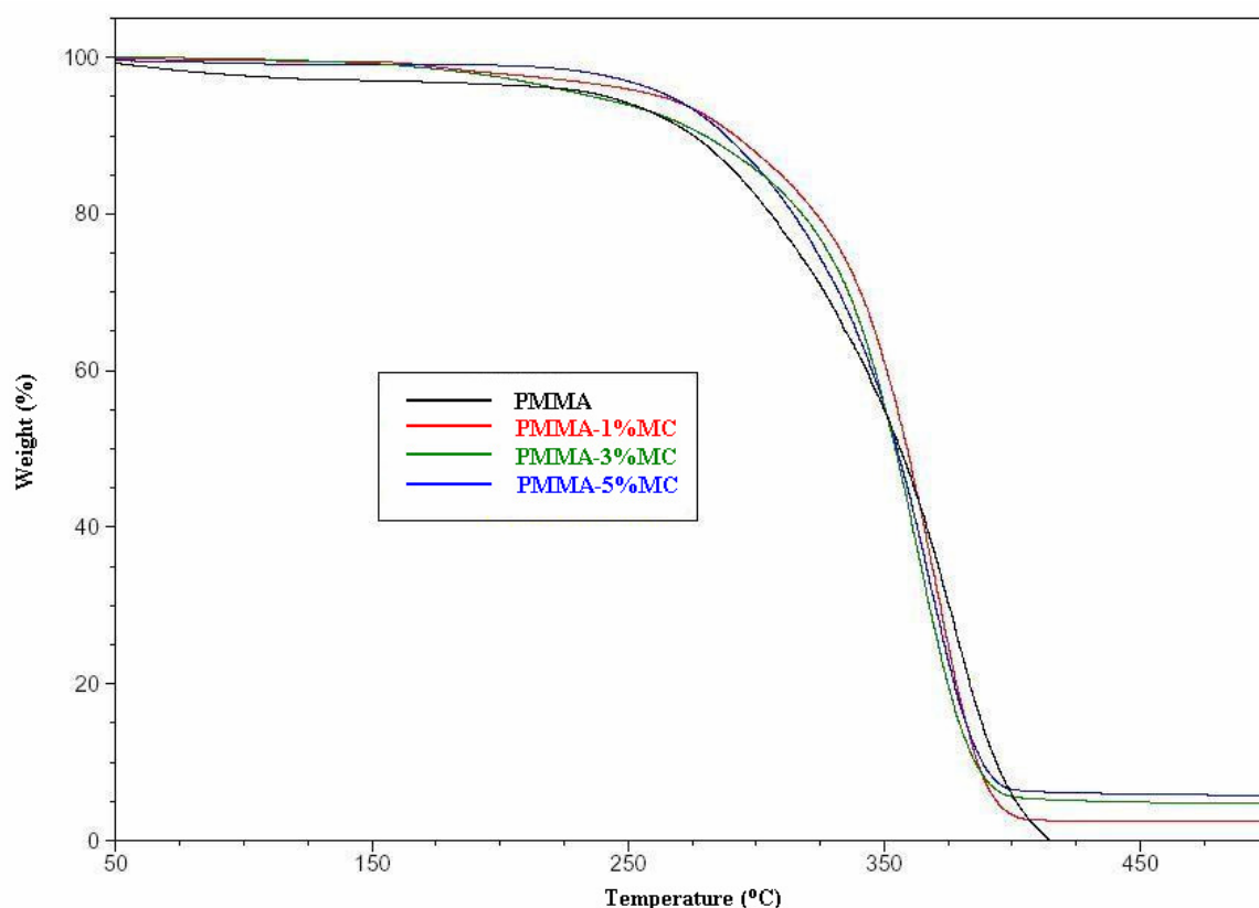
Figure 3.11. TGA graphs of PMMA and nanocomposites
