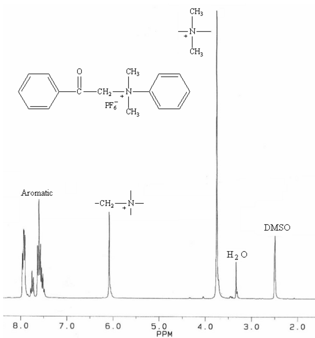
Figure 3.1. ^1\text{H} -NMR spectrum of PDA in DMSO [93]
