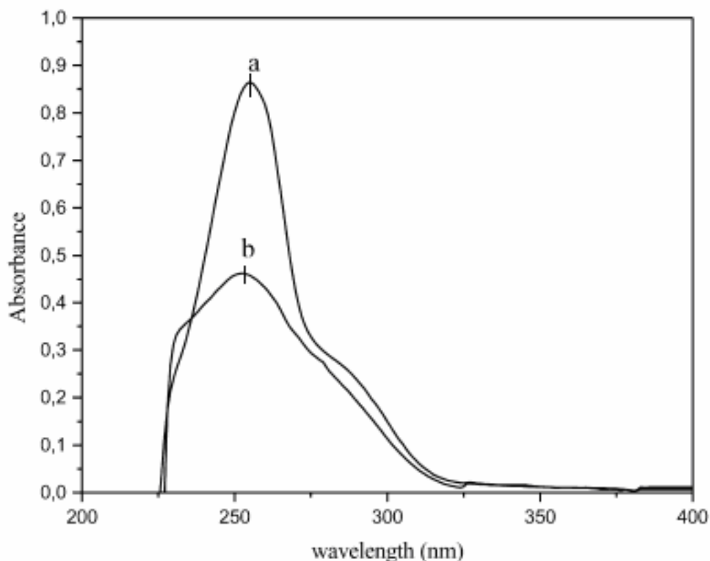
Figure 3.2 Absorption spectra of PDA in dichloromethane before (a) and after 15 minutes of irradiation (b) [93]
