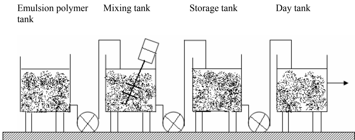
Figure 2.6. The typical emulsion polymer preparation scheme.
