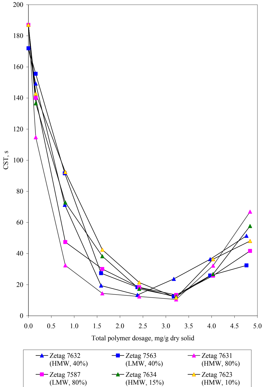
Figure 4.2. The relationship between the sludge dewaterability and the dosage of cationic polymers.
