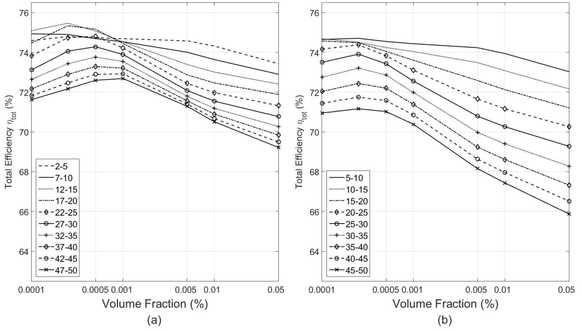
Figure A.8. Total efficiency results for water \text{SiO}_2 -Au nanofluid with shell thickness (a) 3 nm (b) 5 nm.
