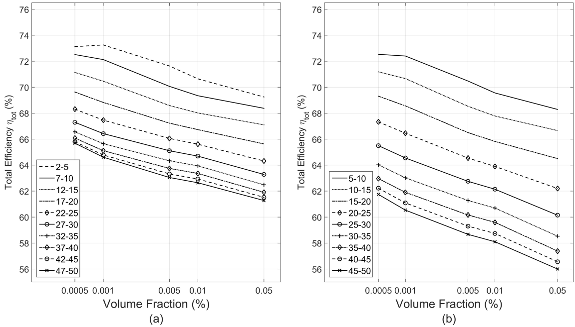
Figure A.3. Total efficiency results for EG \text{SiO}_2 -Al nanofluid with shell thickness (a) 3 nm (b) 5 nm.
