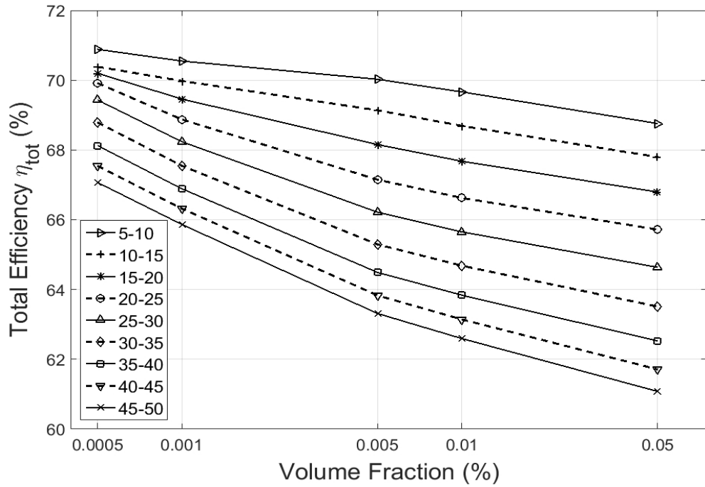
Figure 4.24. Total efficiency values for EG based SiO 2 /Au nanofluid with shell thickness of 5 nm.
