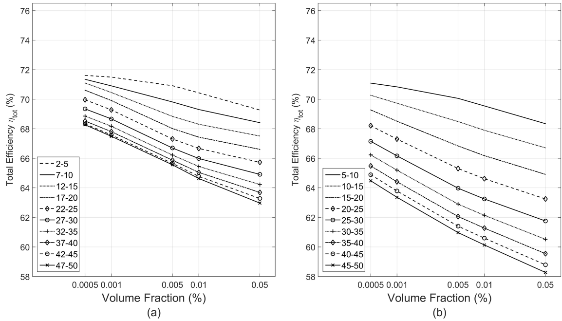
Figure A.1. Total efficiency results for EG \text{SiO}_2 -Ag nanofluid with shell thickness (a) 3 nm (b) 5 nm.
