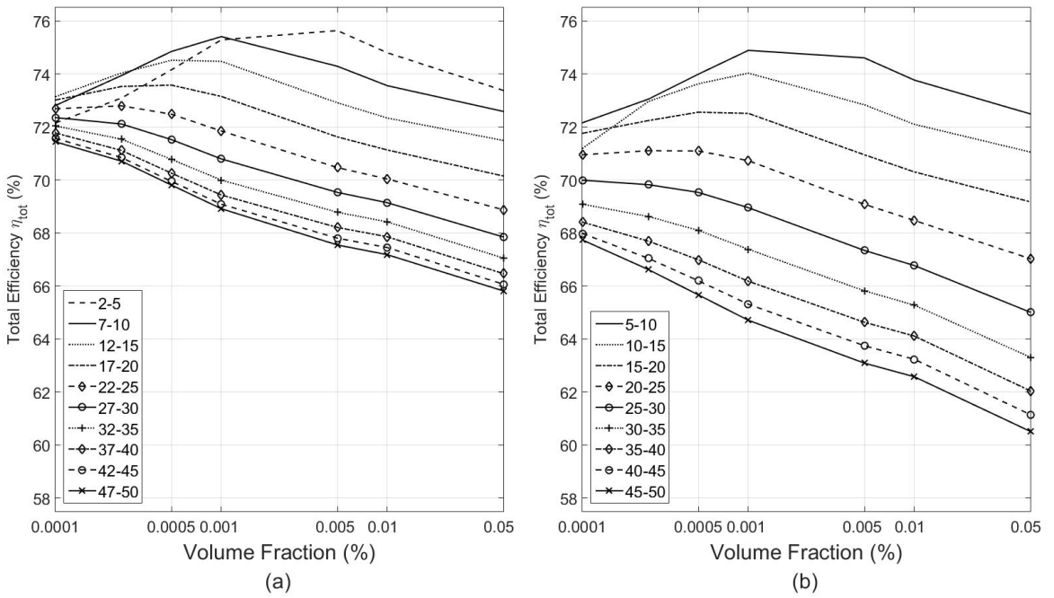
Figure 4.30. Total efficiency results for water \text{SiO}_2\text{-Al} nanofluid with shell thickness 3 nm and 5 nm.
