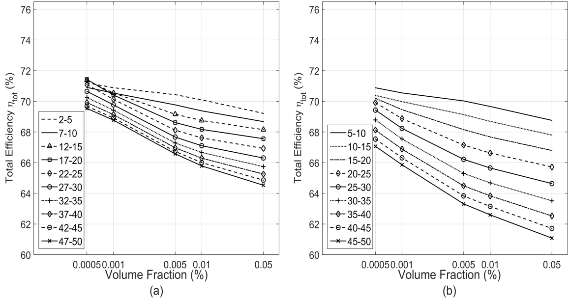
Figure A.2. Total efficiency results for EG \text{SiO}_2 -Au nanofluid with shell thickness (a) 3 nm (b) 5 nm.
