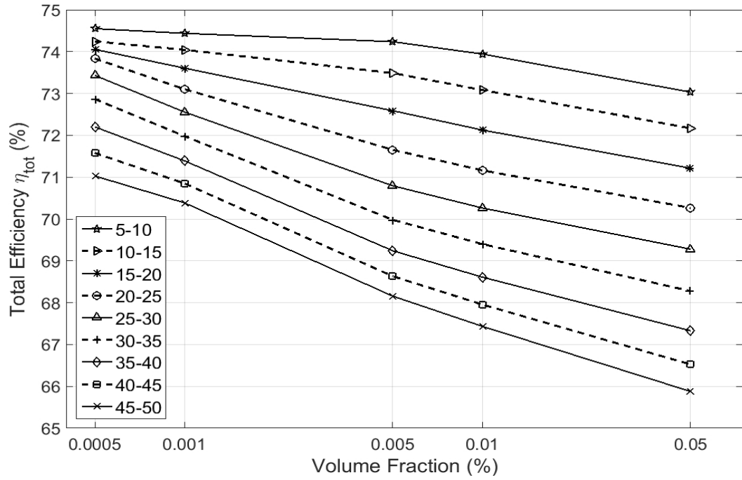
Figure 4.23. Total efficiency values for water based SiO 2 /Au nanofluid with shell thickness of 5 nm.
