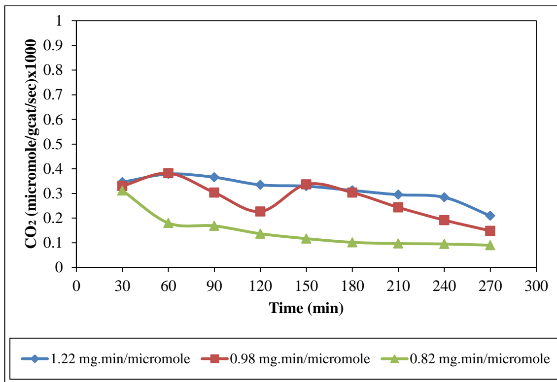
Figure 4.16. Effect of W/F_{CO} ratio on CO_2 production over 2wt\%Rh/\delta-Al_2O_3 at 270^\circ C .
