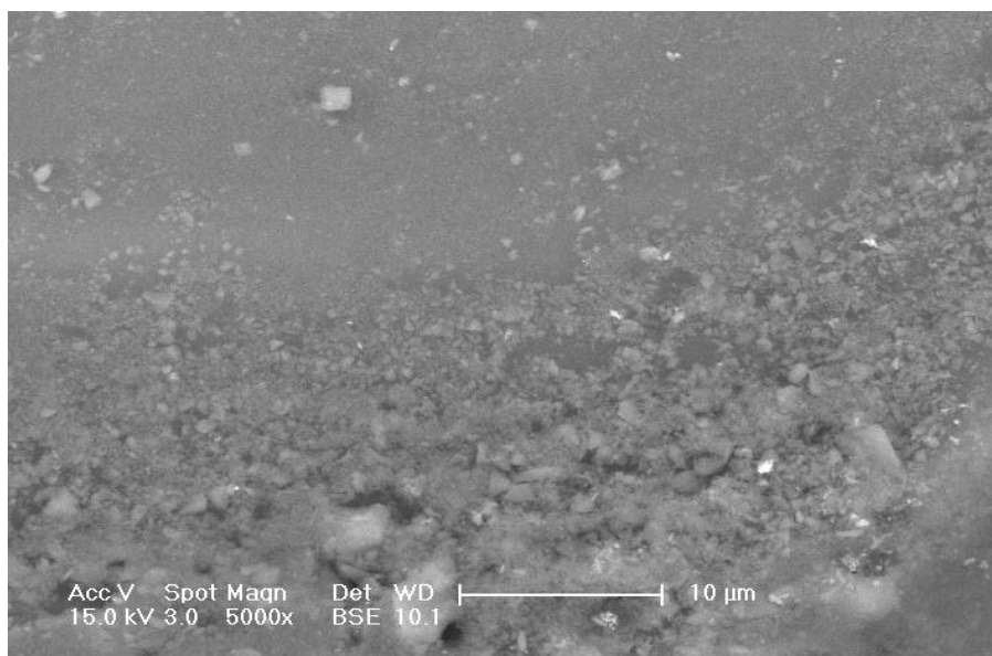
Figure 4.8. SEM image of freshly reduced 1.5wt%Rh-2.6wt%La-1.5wt% V/SiO 2 (5000x).
