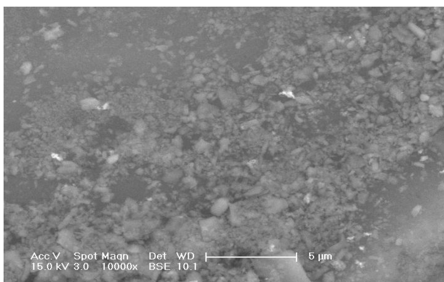
Figure 4.9. SEM image of freshly reduced 1.5wt%Rh-2.6wt%La-1.5wt% V/SiO 2 (10000x).
