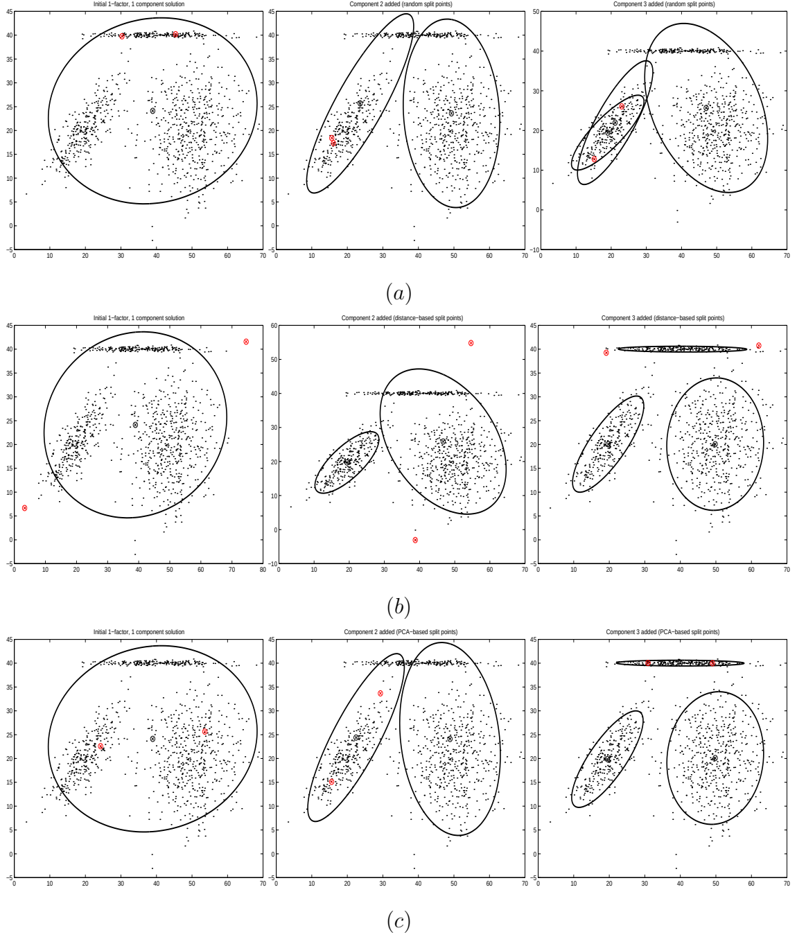
Figure 4.4. Addition of components to the artificial dataset. The components are selected by looking at the univariate kurtosis . The initial means for the next split are shown on the figures. They also indicate which component is split. Three methods for splitting are shown successively: (a) Random split. (b) Distance-based split. (c) PCA-based split.
