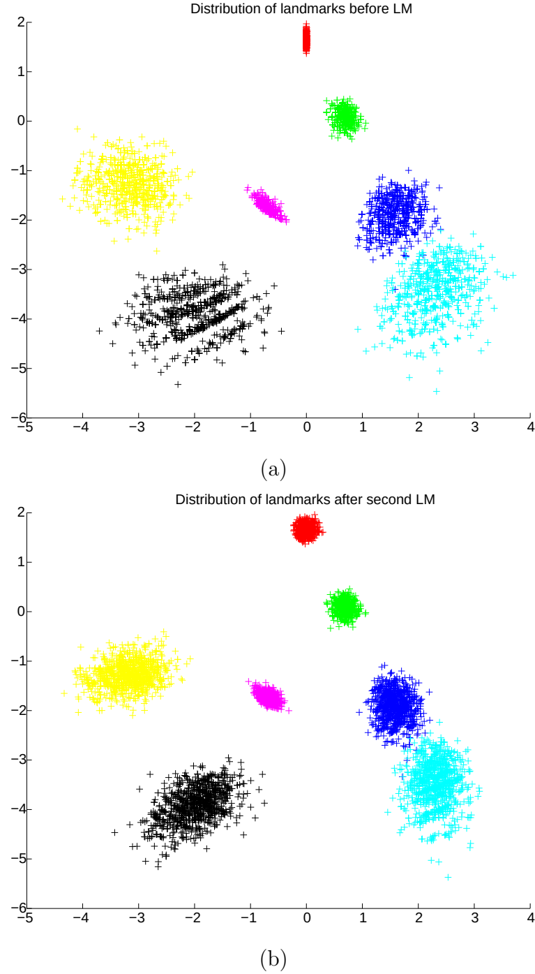
Figure 5.14. The distribution of landmarks after normalization (a) without Levenberg-Marquardt step (b) with Levenberg-Marquardt step
