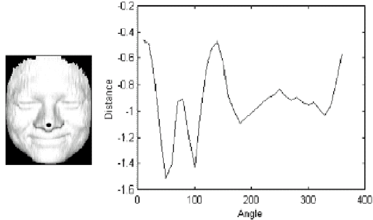
Figure A.2. Point signature of a 3D point (from Wang et al., 2002).
