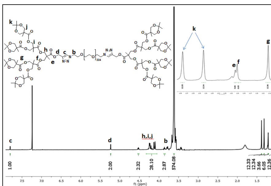
Figure 3.17. ^1H NMR spectrum of 13 .
