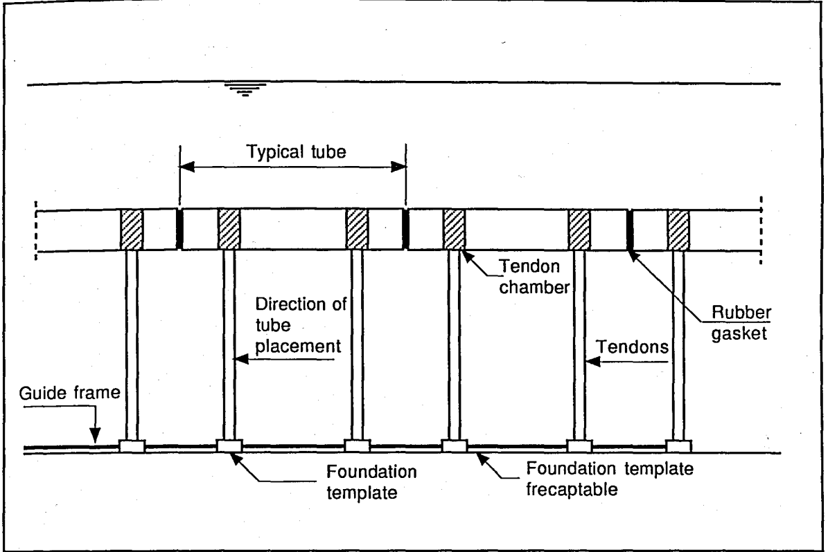
FIGURE 17.3. LONGITUDINAL ELEVATION
