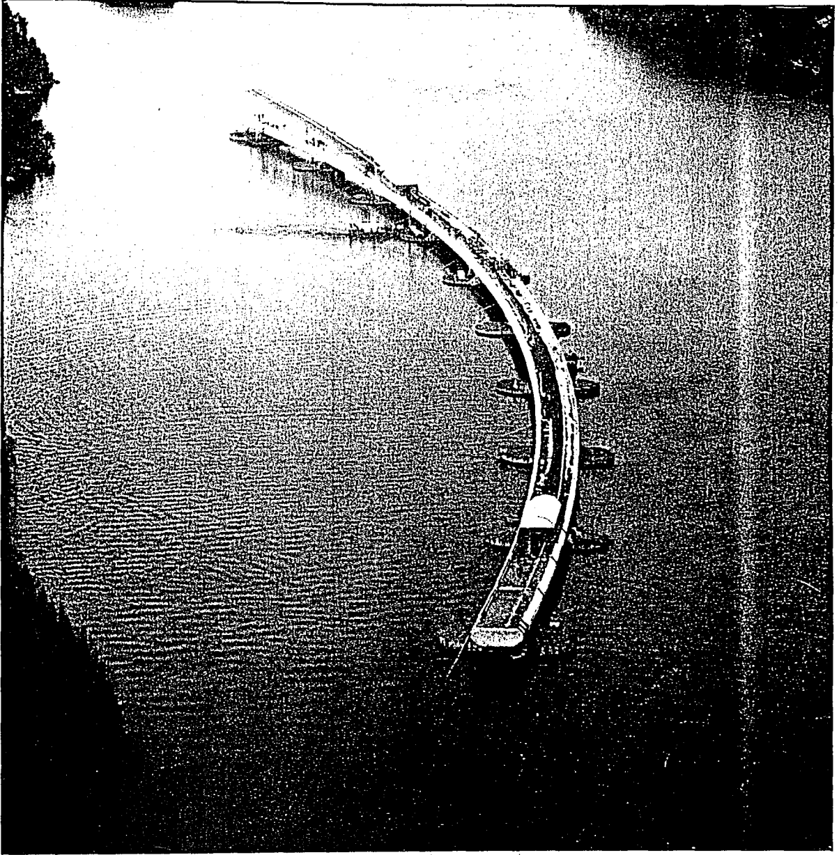
FIGURE 15.7. SALHUS FLOATING BRIDGE, NORWAY (Courtesy of G. Brekke, 1994)
