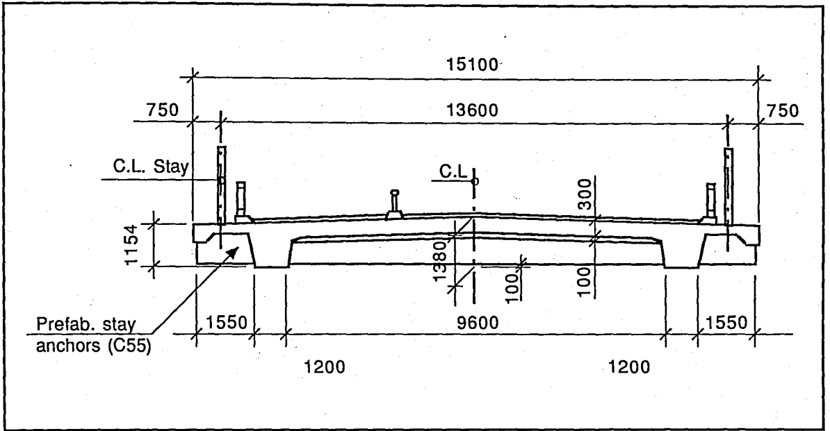
FIGURE 15.3. MAIN SPAN BRIDGE BEAM (In mm)
