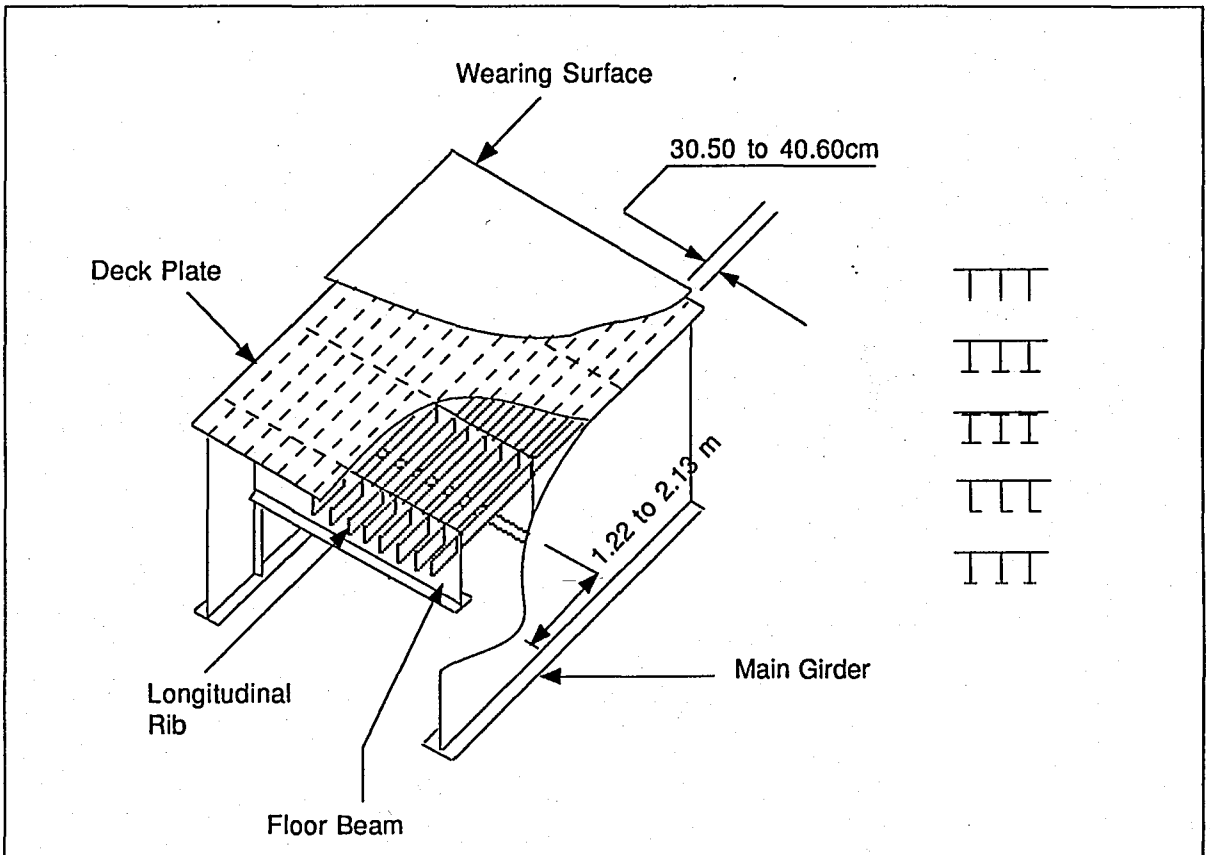
FIGURE 2.6. ORTHOTROPIC DECK BRIDGES; OPEN RIBS
