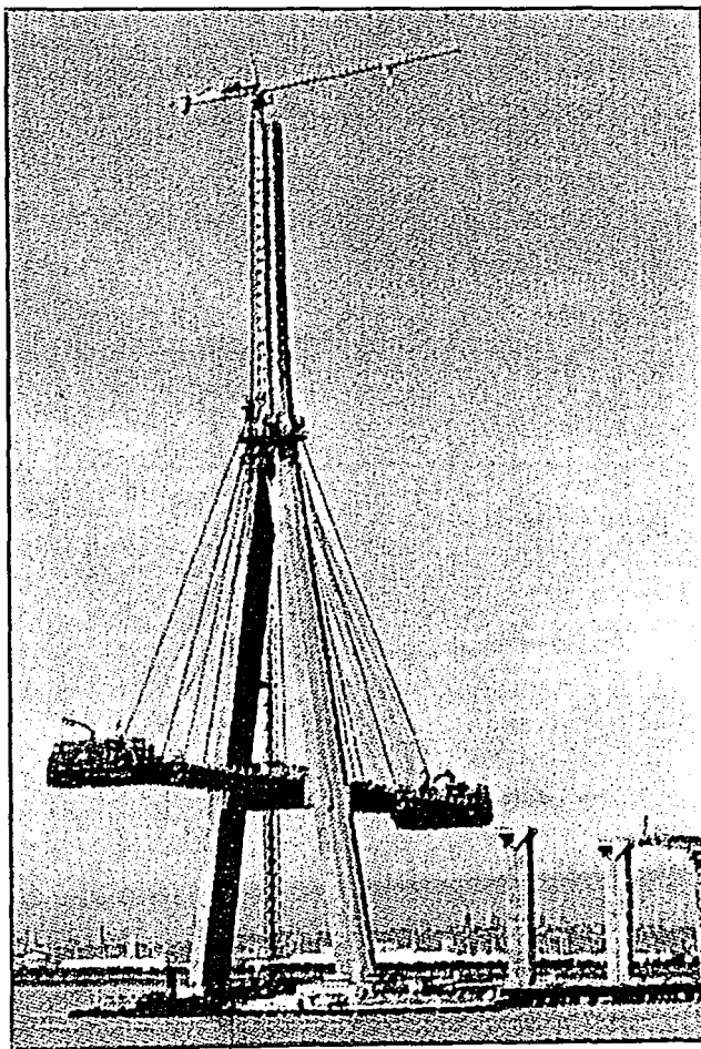
FIGURE 13.8. CONSTRUCTION OF THE DECK AT THE SOUTH PYLON (Courtesy of AFPC, 1994)
