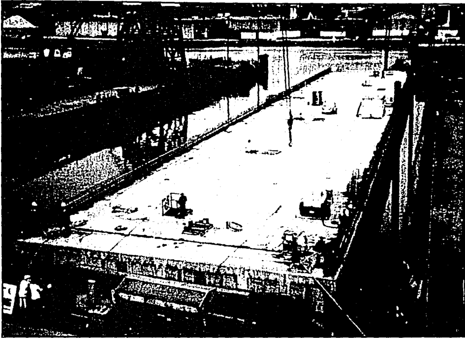
FIGURE 14.4. COMPLETED AND FLOATED PONTOON (Courtesy of J. Krokeborg, 1994)
