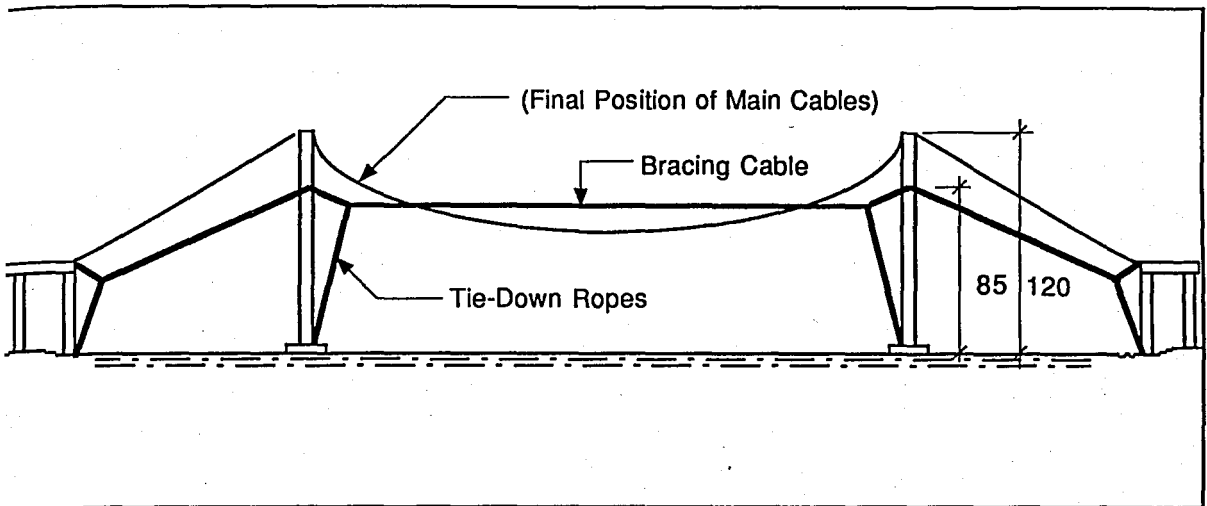
FIGURE 5.8. BRACING CABLES OF THE LITTLE BELT BRIDGE, DENMARK (In meters)
