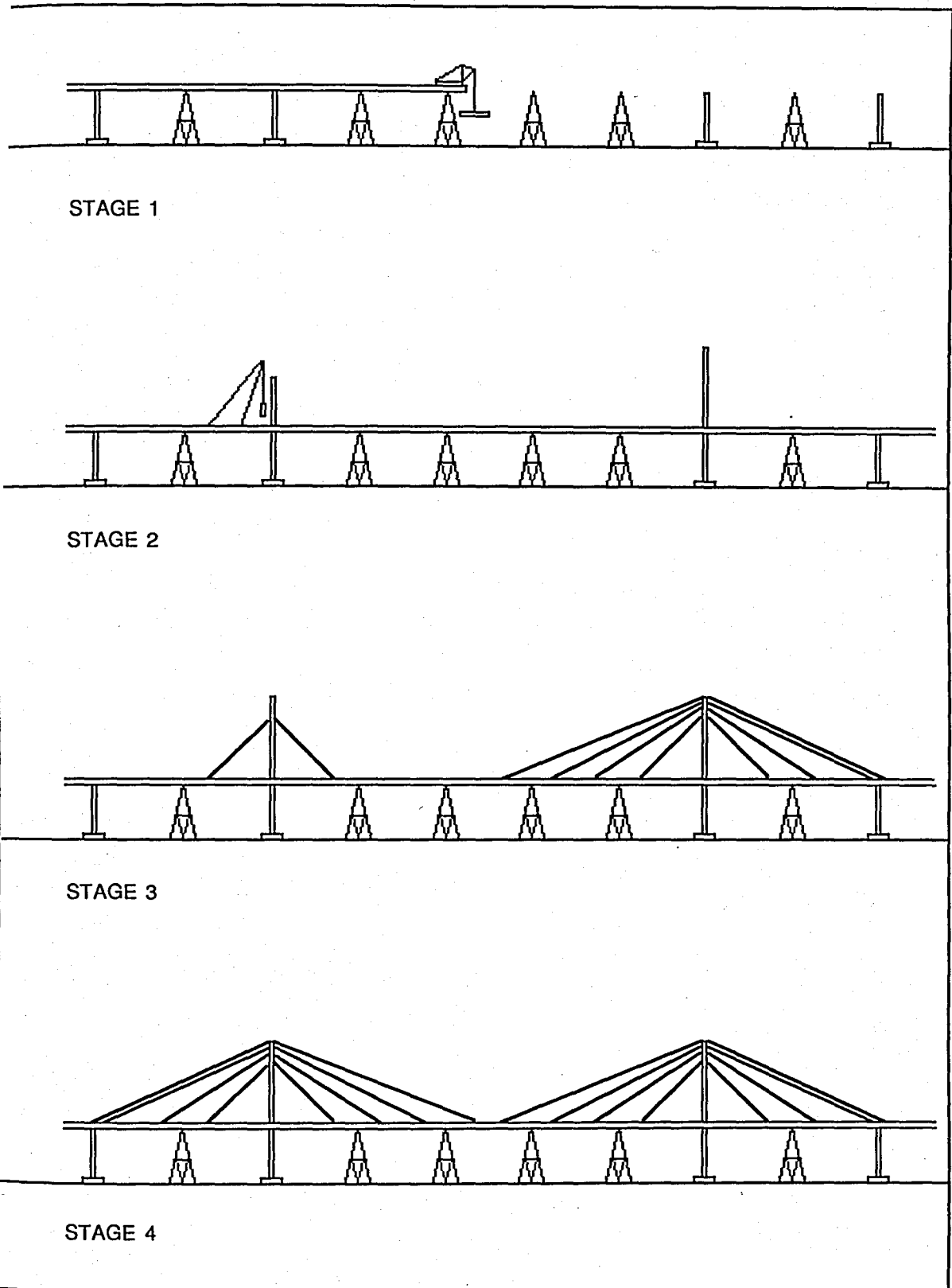
FIGURE 5.3. ERECTION ON TEMPORARY SUPPORTS
