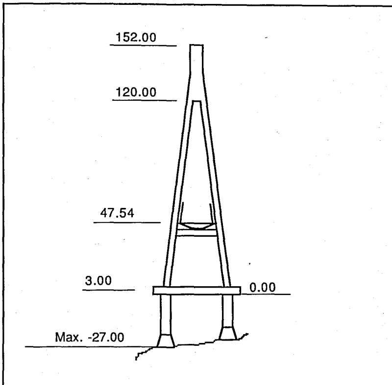
FIGURE 10.4. MAIN TOWER (In meters)
