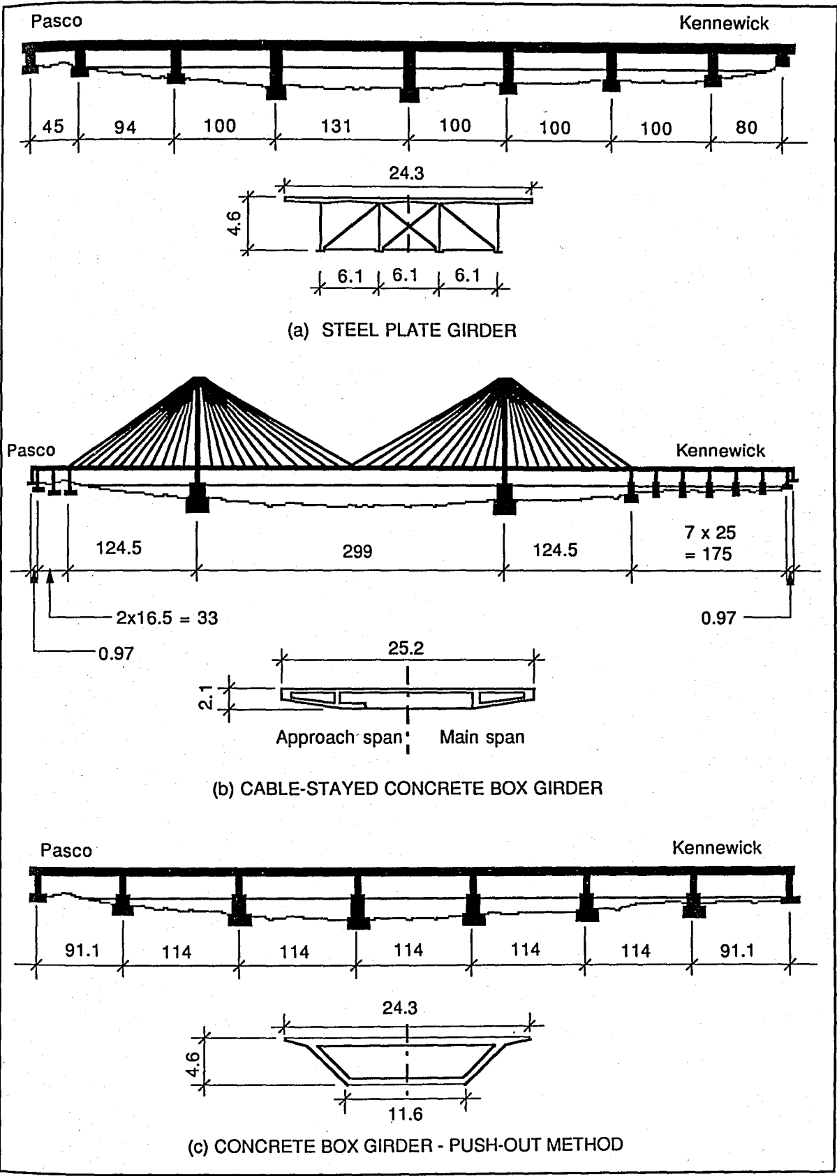
FIGURE 6.10. PRELIMINARY DESIGN ALTERNATIVES FOR PASCO-KENNEWICK BRIDGE (In meters)
