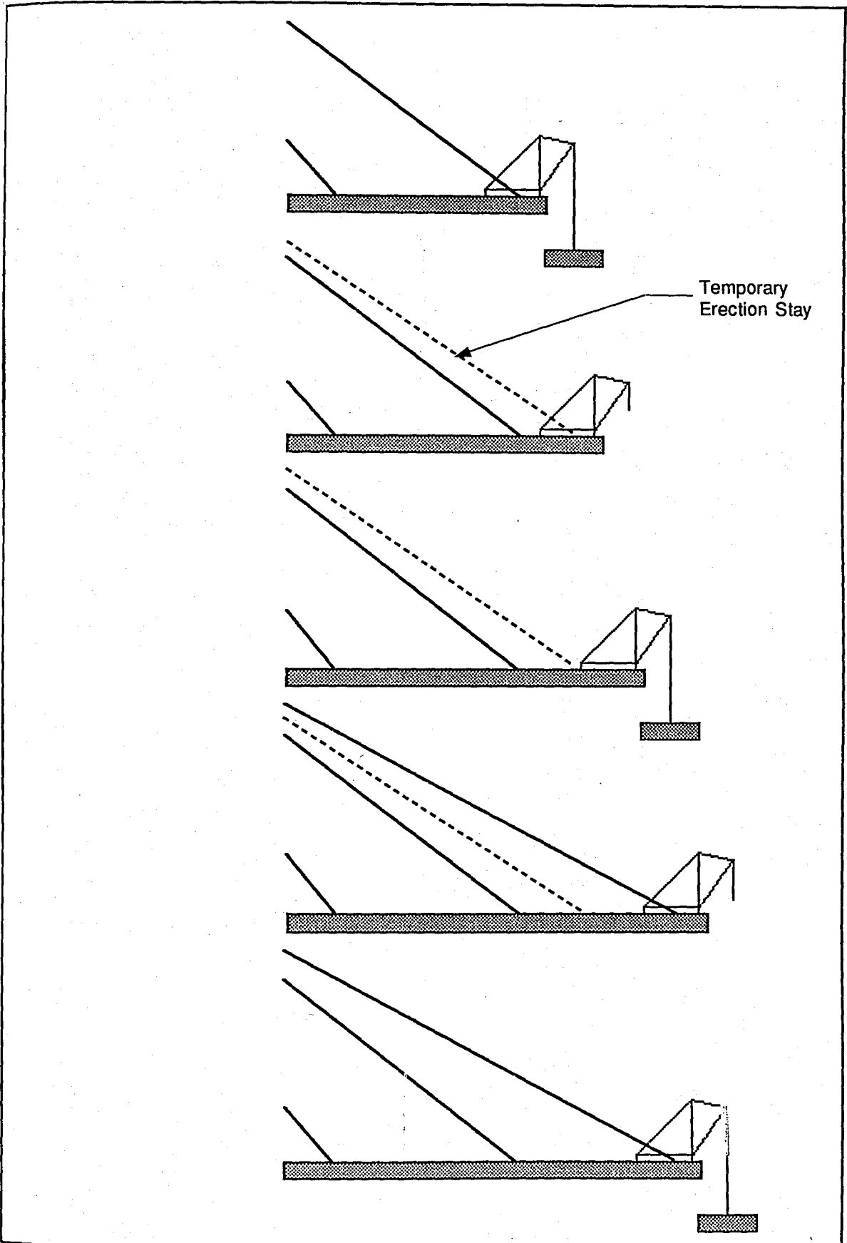
FIGURE 5.16. APPLICATION OF A TEMPORARY ERECTION STAY
