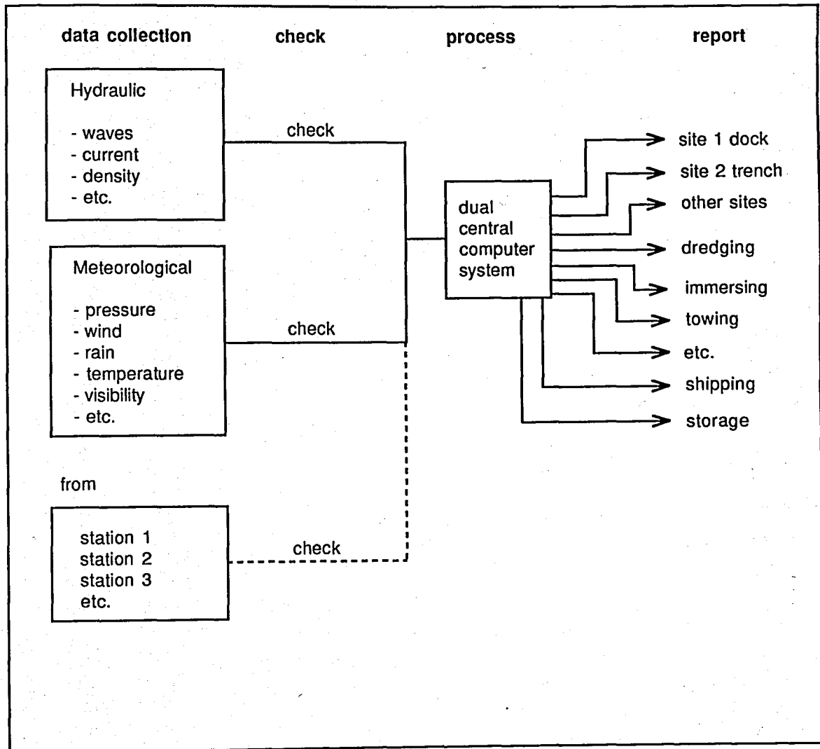
FIGURE 16.2. SCHEME OF DATA COLLECTION
