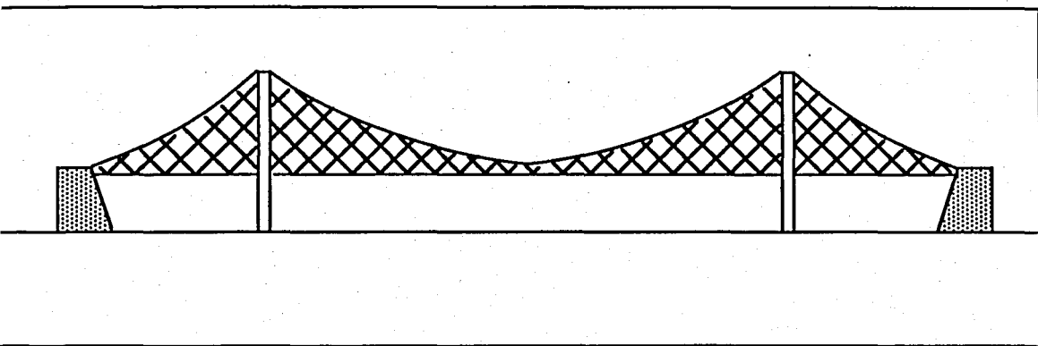
FIGURE 3.13. SUSPENSION SYSTEM WITH A HANGER NET BETWEEN THE MAIN CABLE AND THE STIFFENING GIRDER
