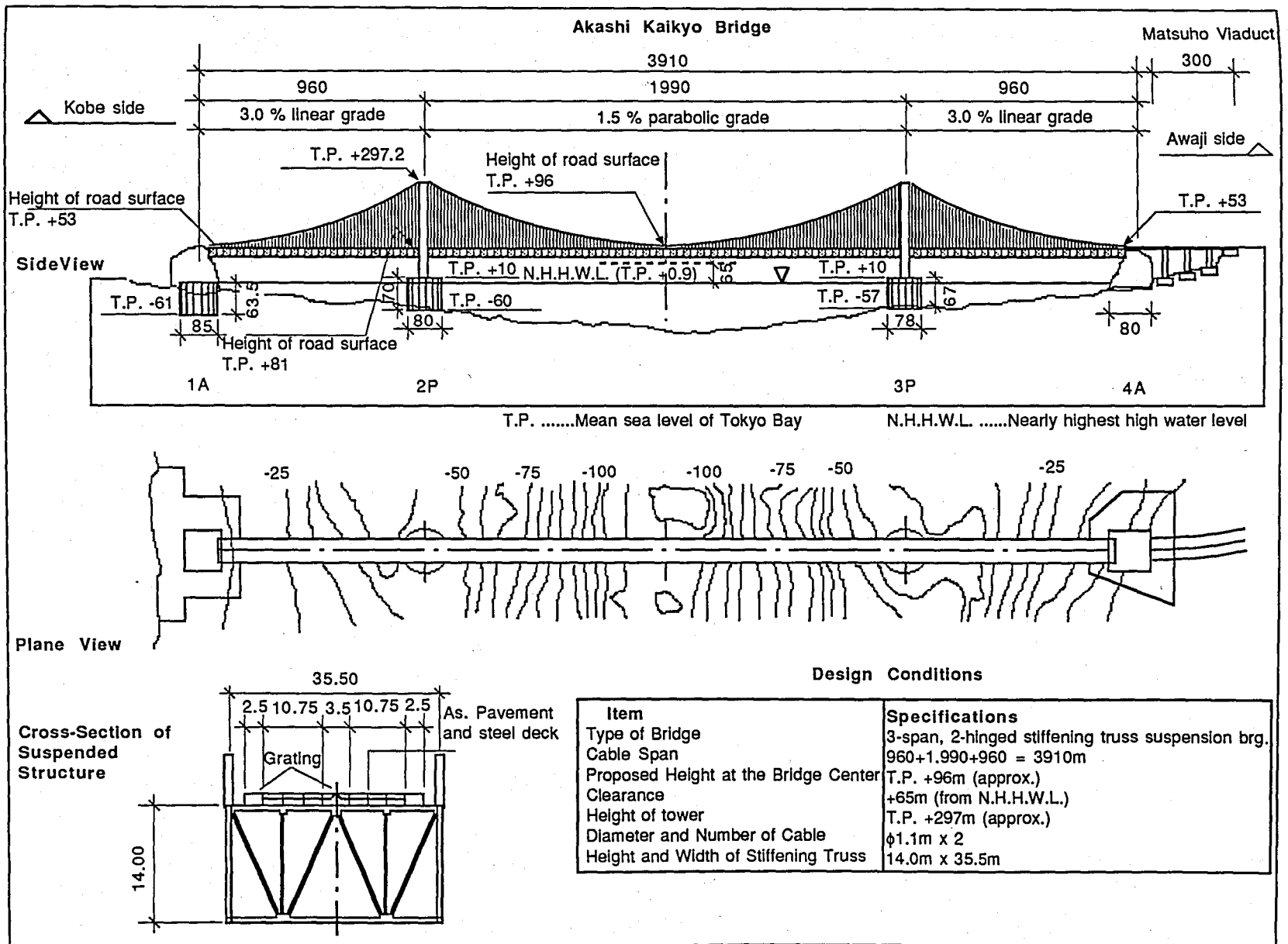
FIGURE 11.1. GENERAL VIEW (in meters)
