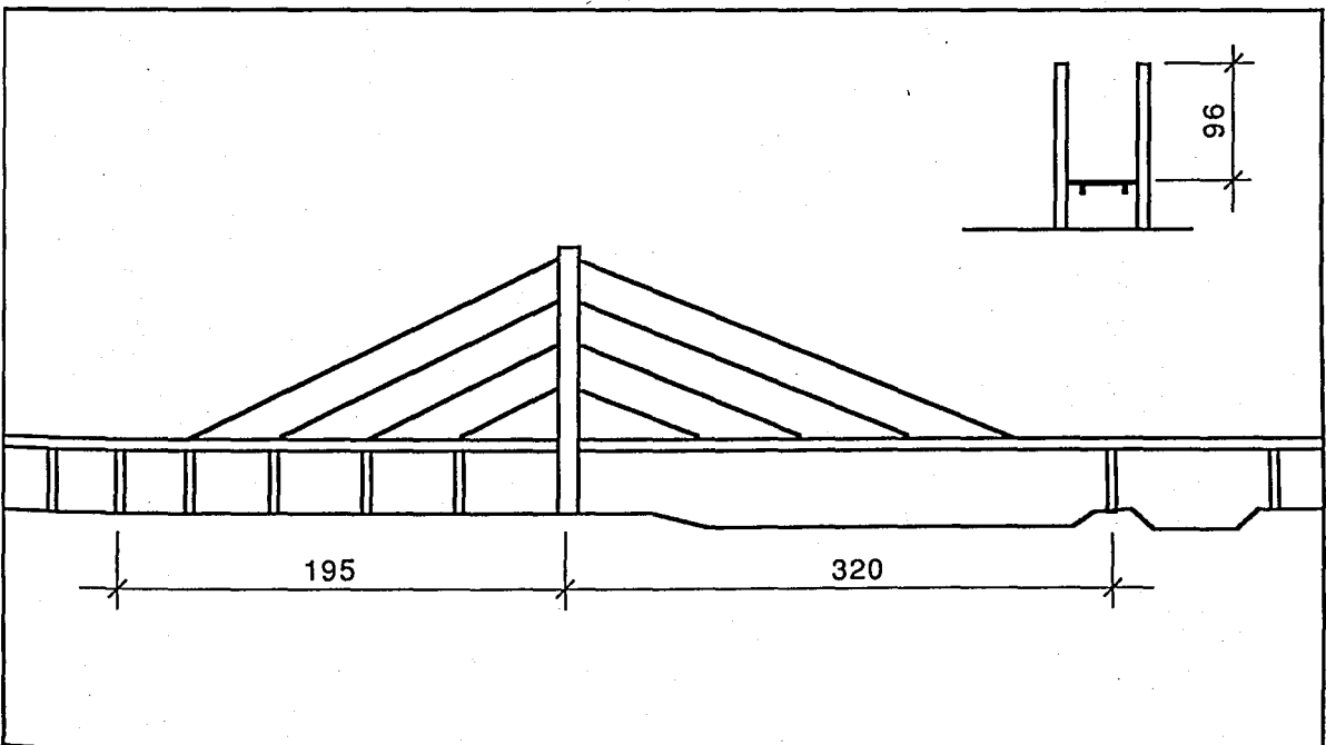
FIGURE 6.3. KNIEBRÜCKE BRIDGE, GERMANY (in meters)
