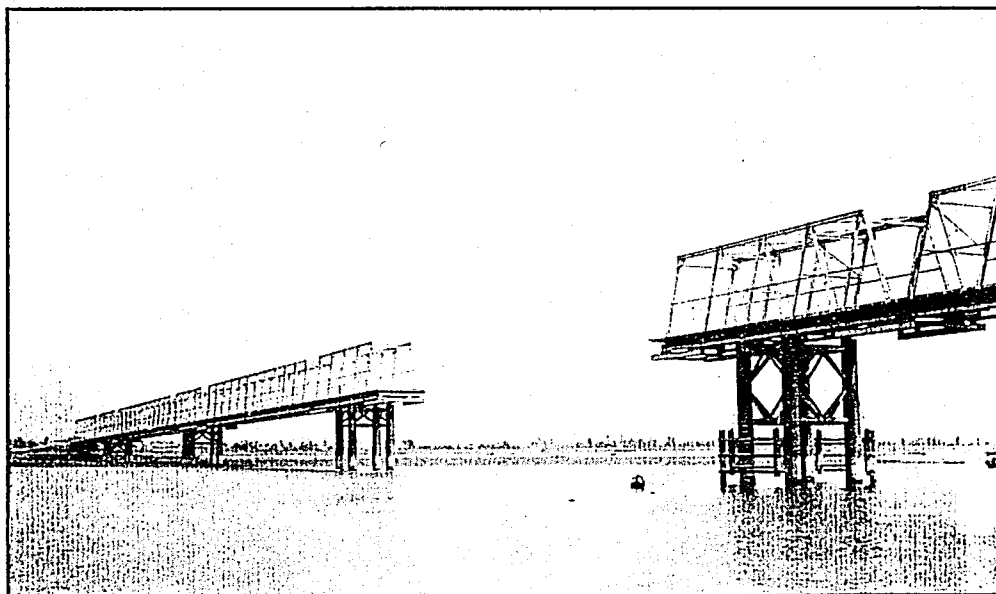
FIGURE 9.7. THE CARNAFULI BRIDGE ACCIDENT, BURMA, 1991 (Courtesy of O. D. Larsen, 1994)
