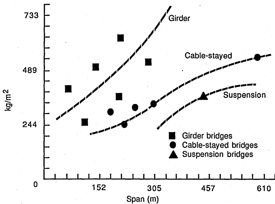
FIGURE 6.4. WEIGHT OF STRUCTURAL STEEL FOR ORTHOTROPIC STEEL BRIDGES
