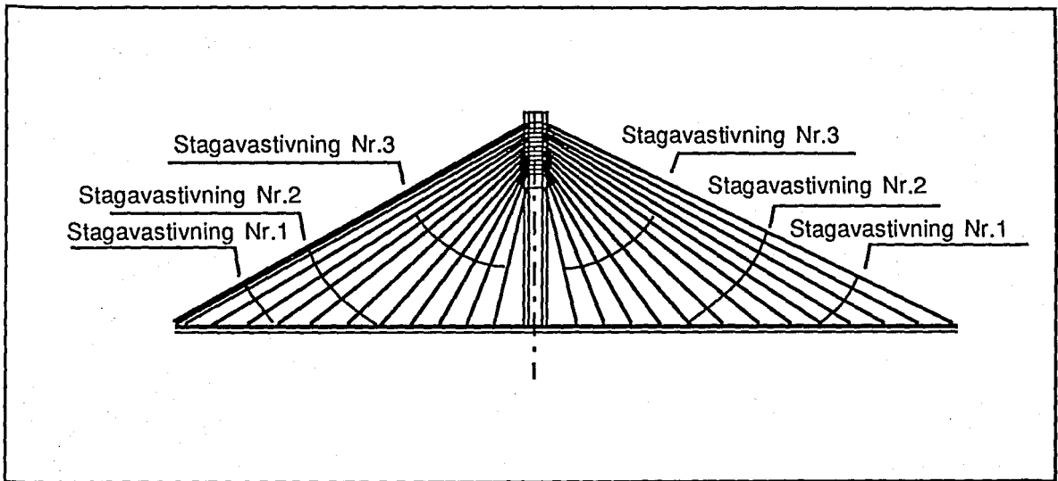
FIGURE 10.13. CROSS STIFFENING OF CABLES
