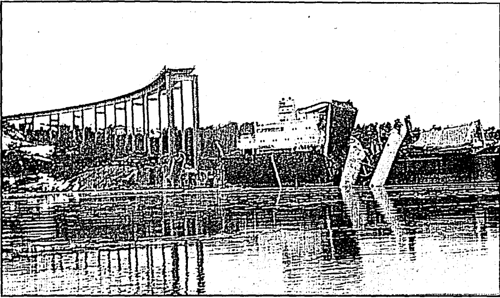
FIGURE 9.4. THE TJÖRN BRIDGE ACCIDENT, SWEDEN , 1980 (Courtesy of O. D. Larsen, 1994)
