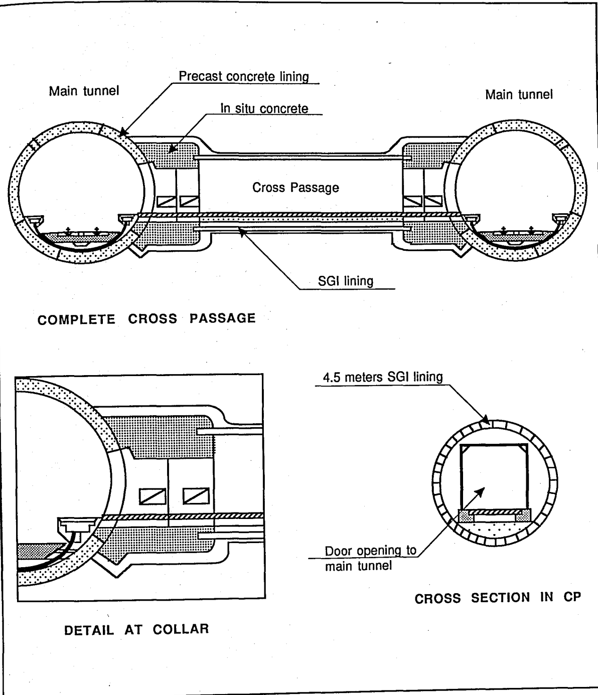
FIGURE 21.5. CROSS PASSAGE COMPLETED
