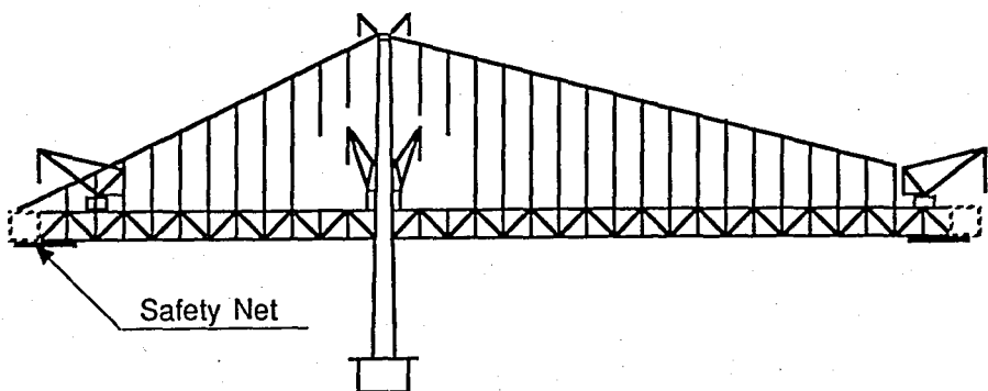
FIGURE 11.9. STIFFENING GIRDER ERECTION
