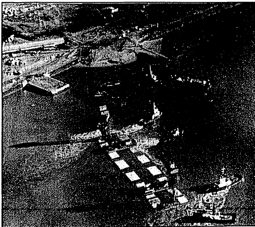
FIGURE 20.6. MOORING OF THE TUNNEL UNITS (Courtesy of J. Krokeborg, 1990)
