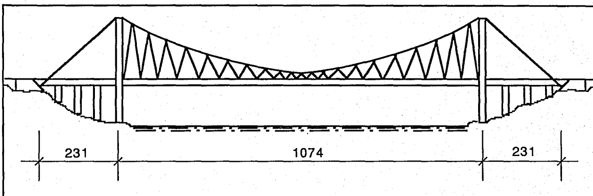
FIGURE 3.3. BOSPHORUS BRIDGE (In meters)
