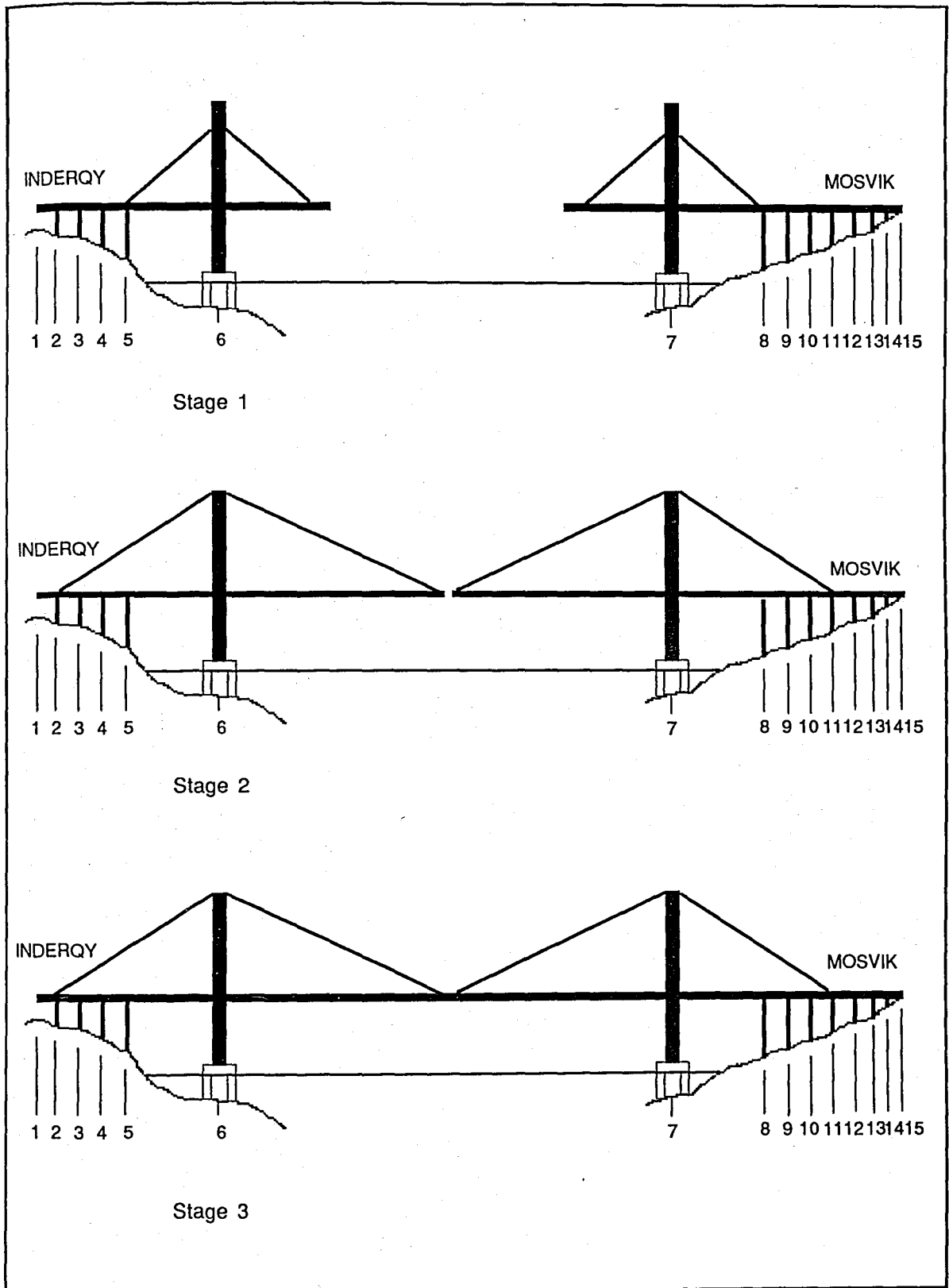
FIGURE 10.5. CONSTRUCTION PROCEDURE
