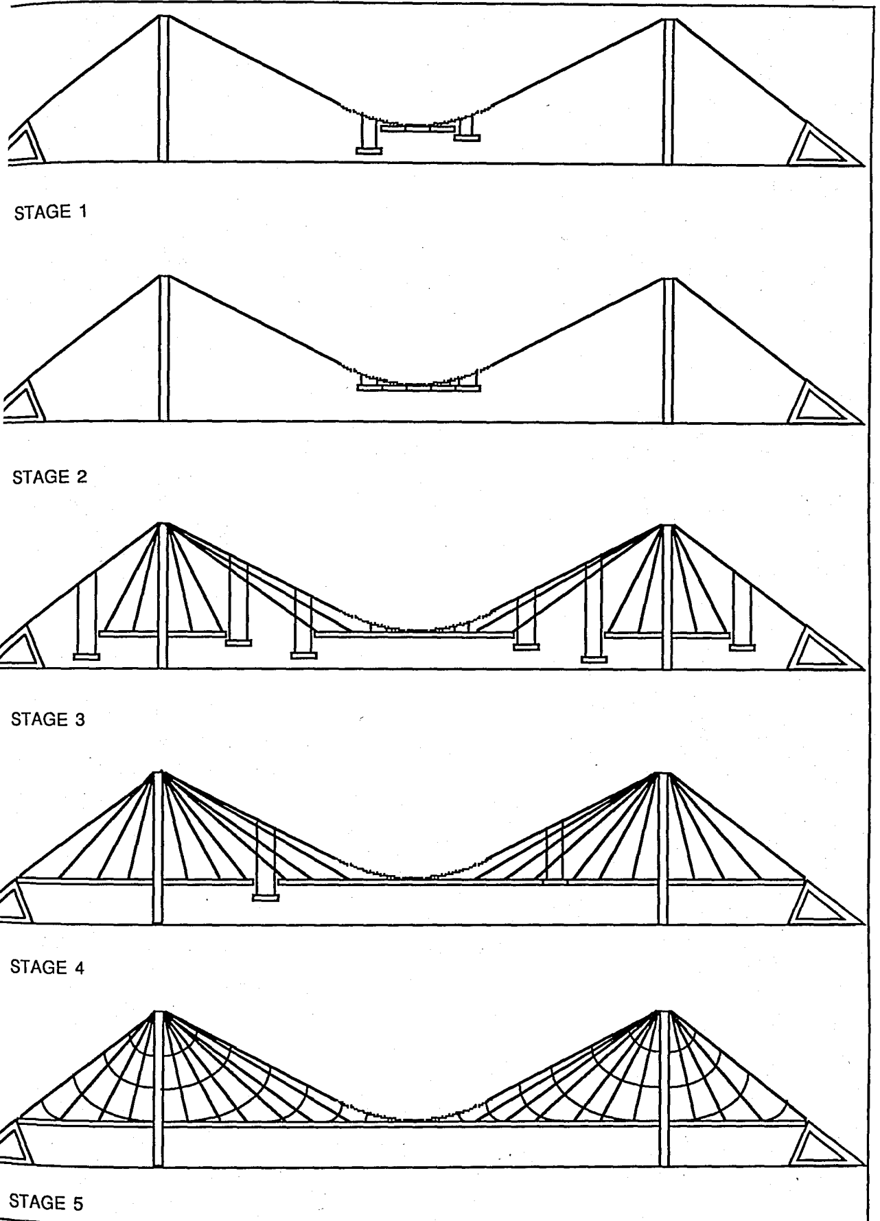
FIGURE 5.7. ERECTION PROCEDURE FOR A CABLE NET BRIDGE
