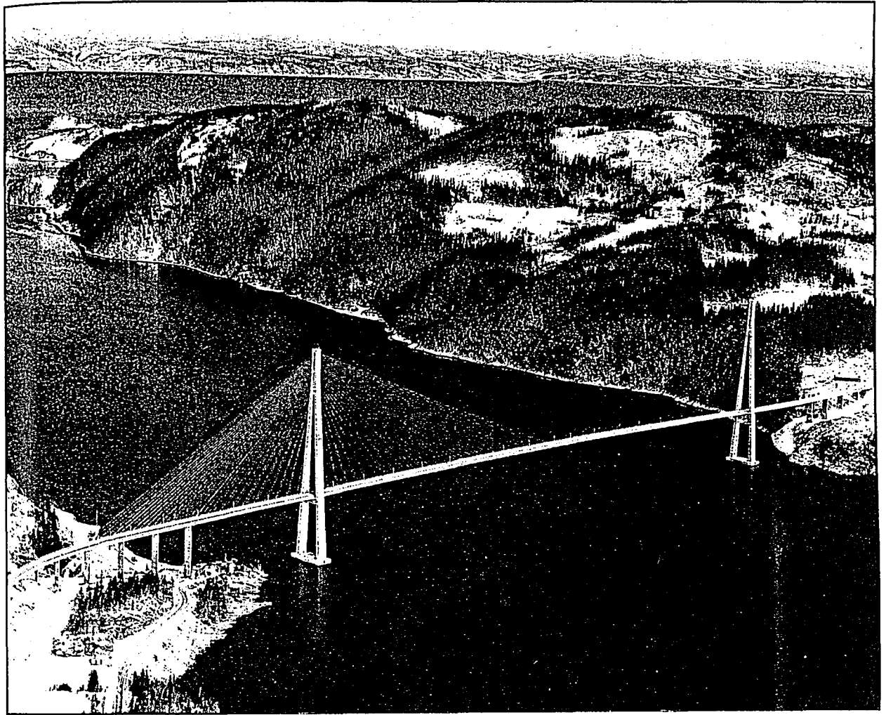
FIGURE 10.2. SKARNSUNDET BRIDGE, NORWAY (Courtesy of P. Schoen, 1993)
