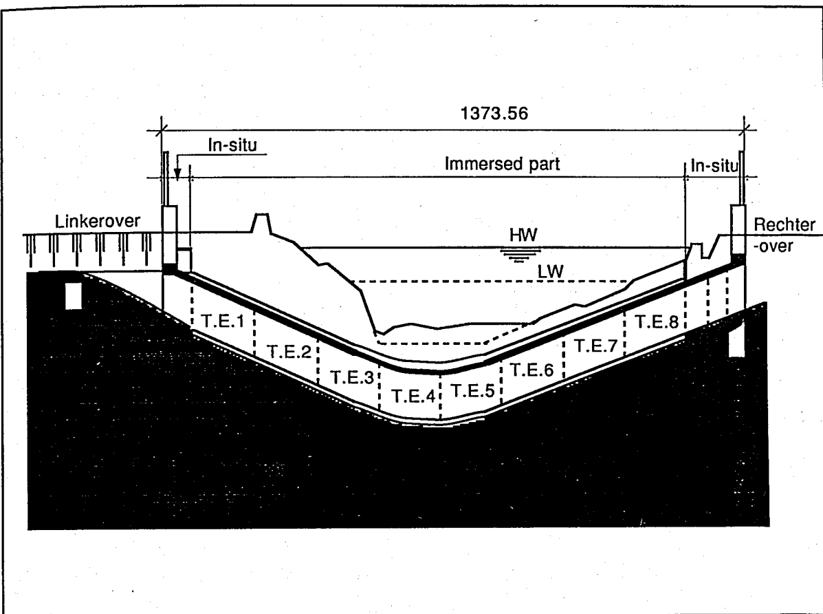
FIGURE 20.2. LONGITUDINAL SECTION (In meters)
