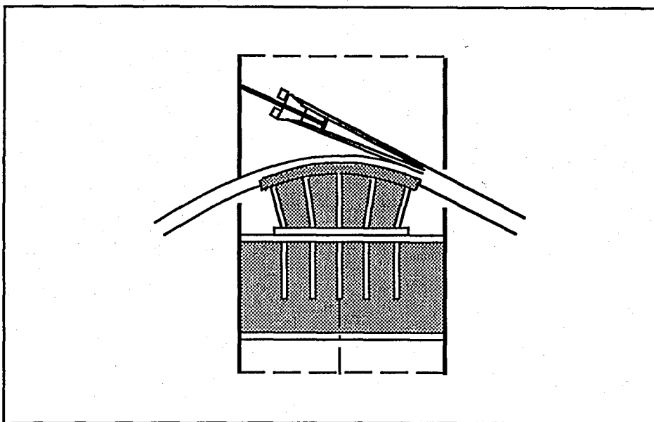
FIGURE 4.25. ADDITIONAL STRANDS
