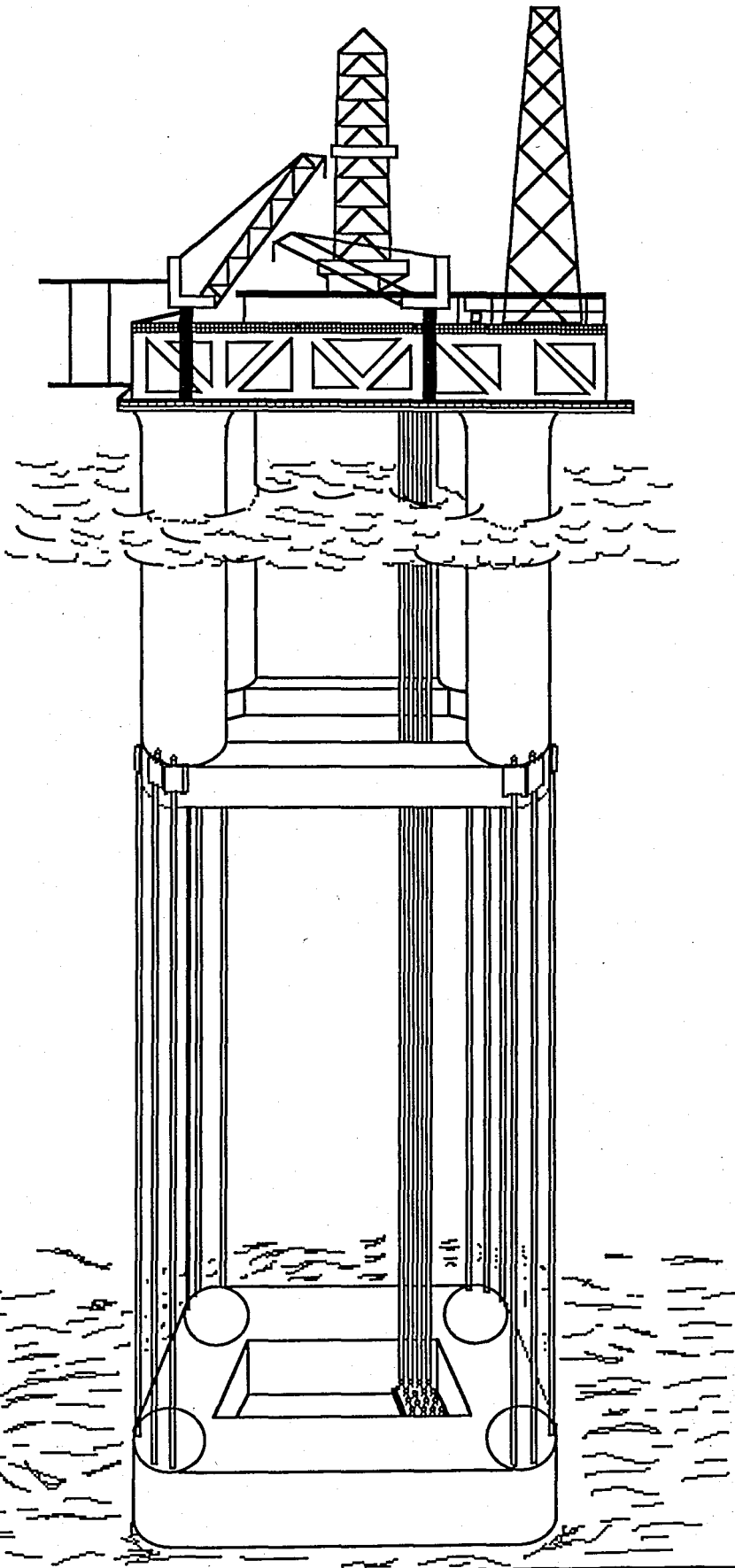
FIGURE 8.1. THE TENSION LEG PLATFORM
