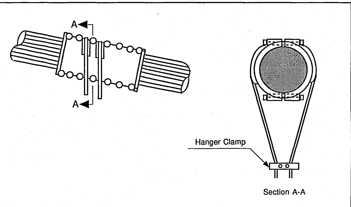
FIGURE 4.17. GROOVED CABLE BAND
