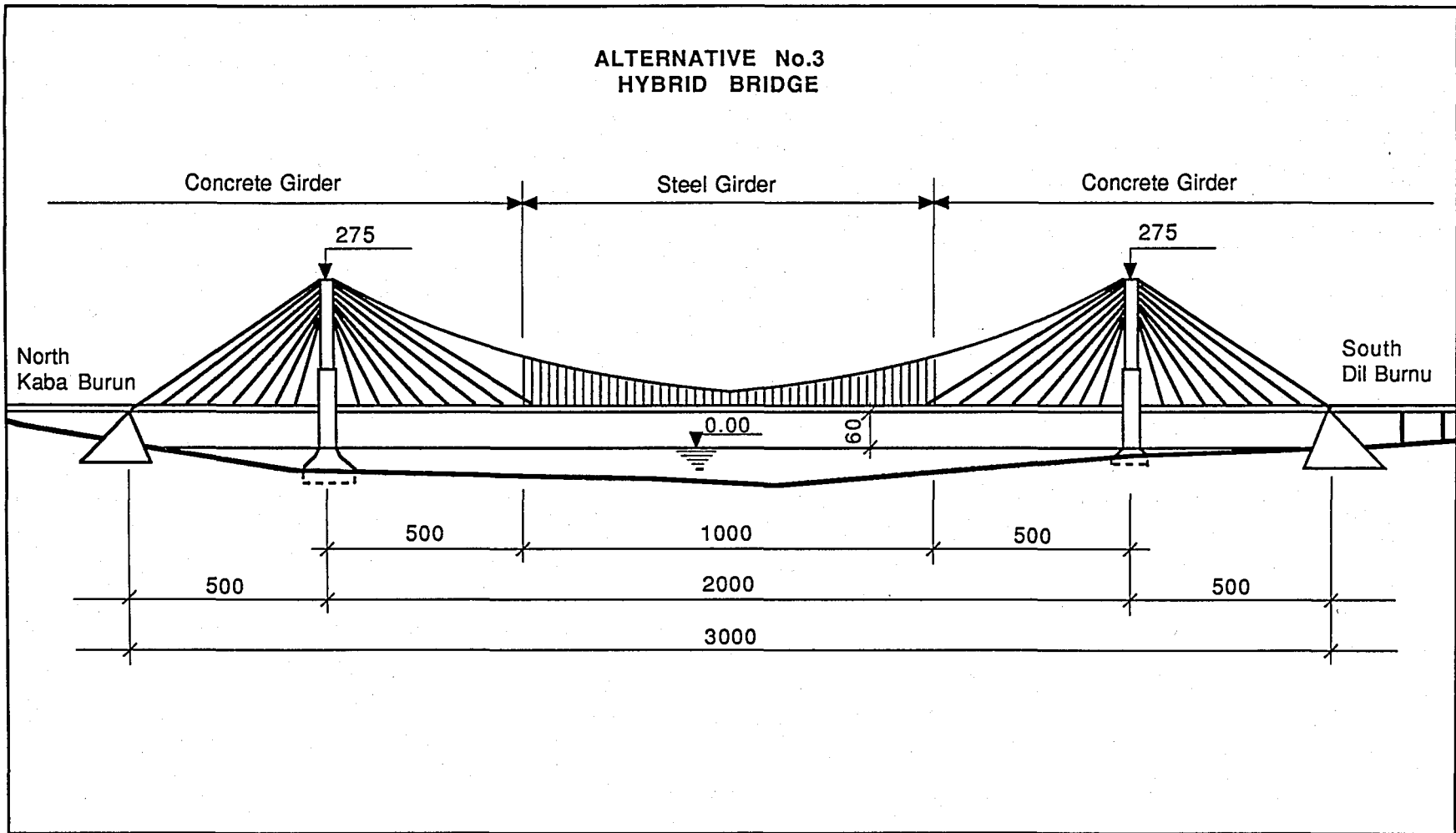
FIGURE 25.12. ELEVATION (In meters)
