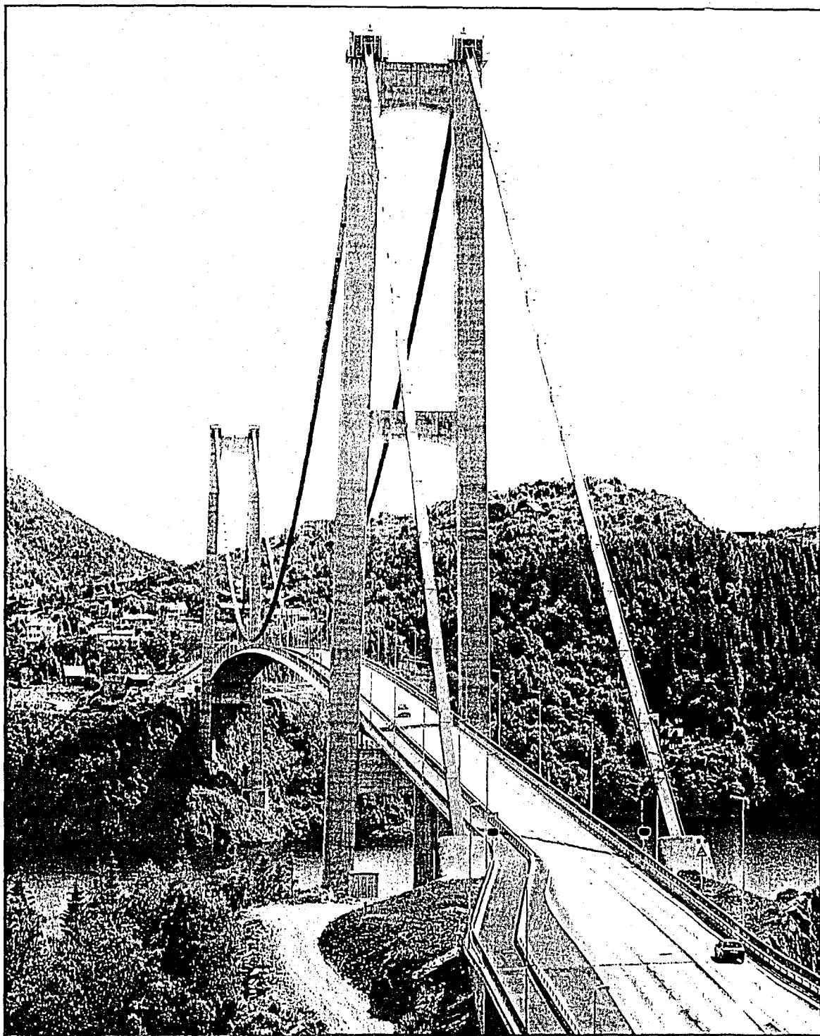
FIGURE 12.2. ASKOY BRIDGE, NORWAY (Courtesy of Monberg and Thorsen A/S, 1994)
