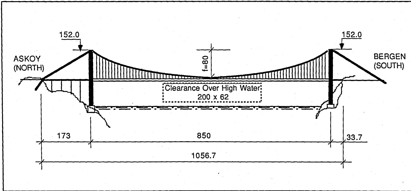
FIGURE 12.1. ELEVATION (in meters)
