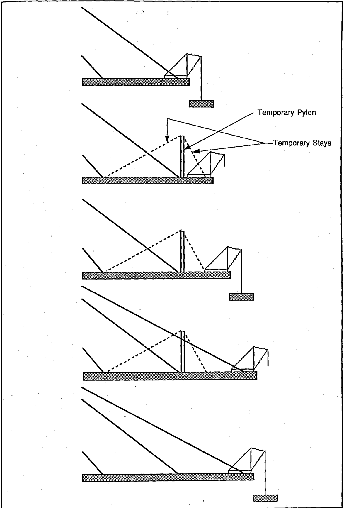
FIGURE 5.17. TEMPORARY CABLE SYSTEM
