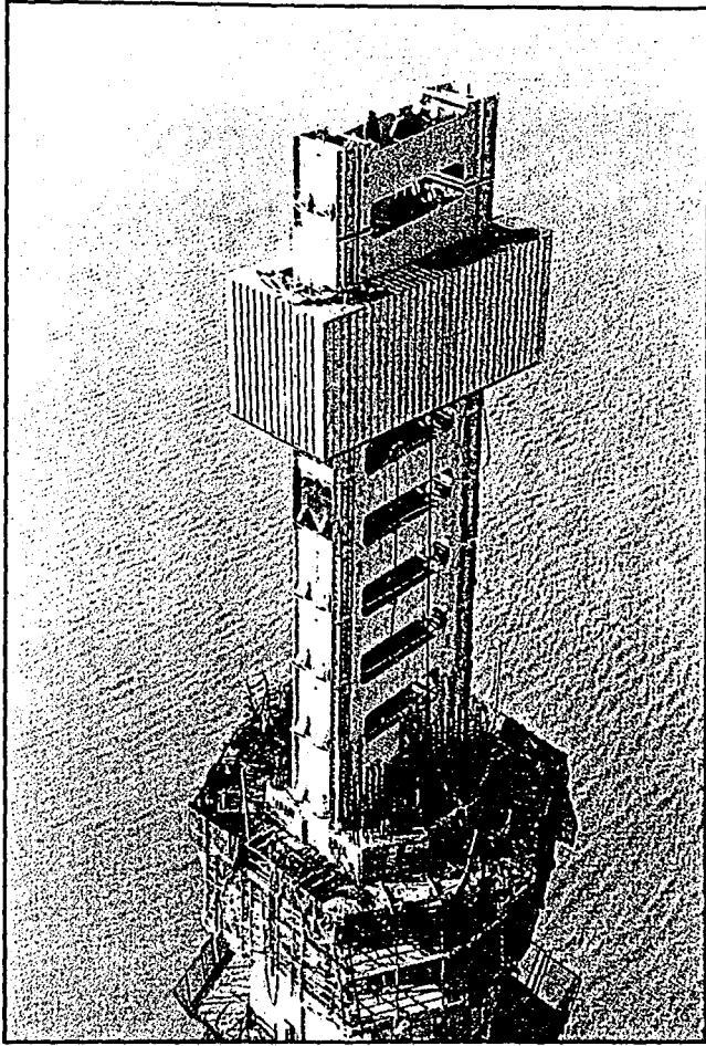
FIGURE 13.5. ANCHORAGE BOXES, SOUTH PYLON (Courtesy of AFPC, 1994)
