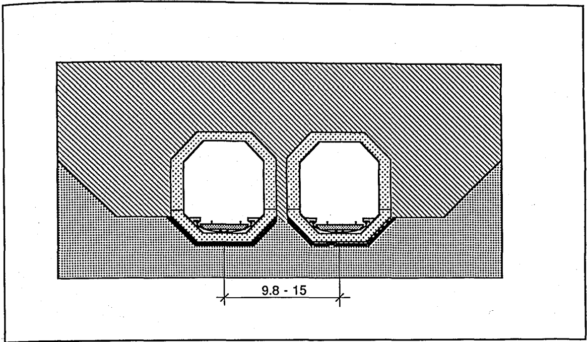
FIGURE 21.6. CUT AND COVER TUNNELS (In meters)
