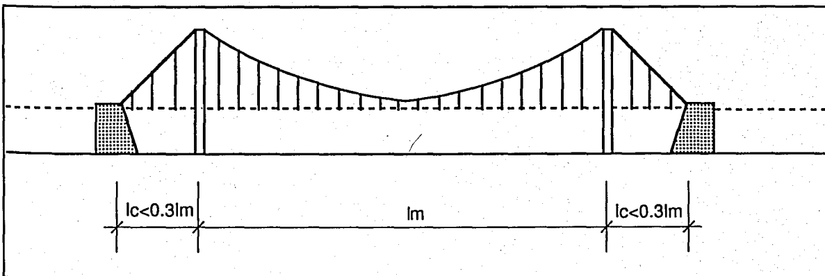
FIGURE 3.4. THREE-SPAN SUSPENSION BRIDGE WITH SHORT SIDE SPANS
