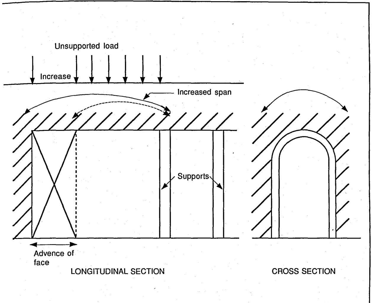
FIGURE 18.3. INCREASE OF LOAD AS FACE IS ADVANCED
