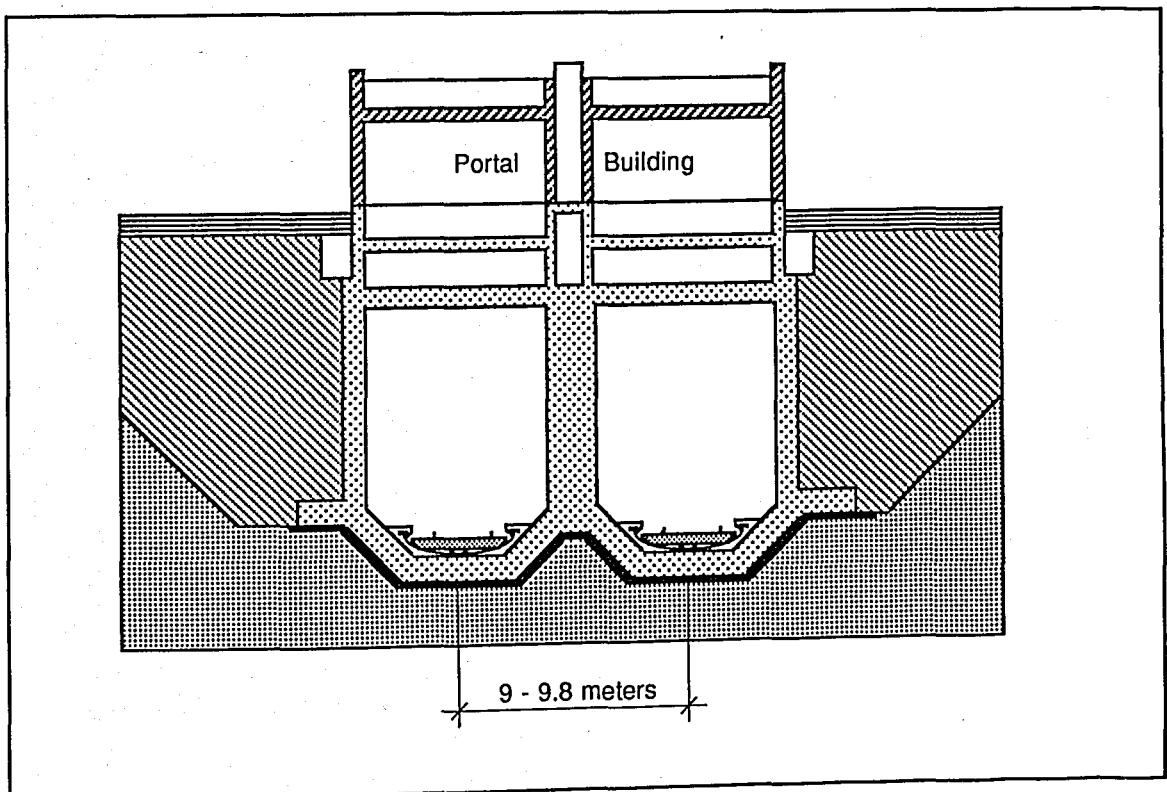
FIGURE 21.7. TUNNELS AT PORTAL (In meters)
