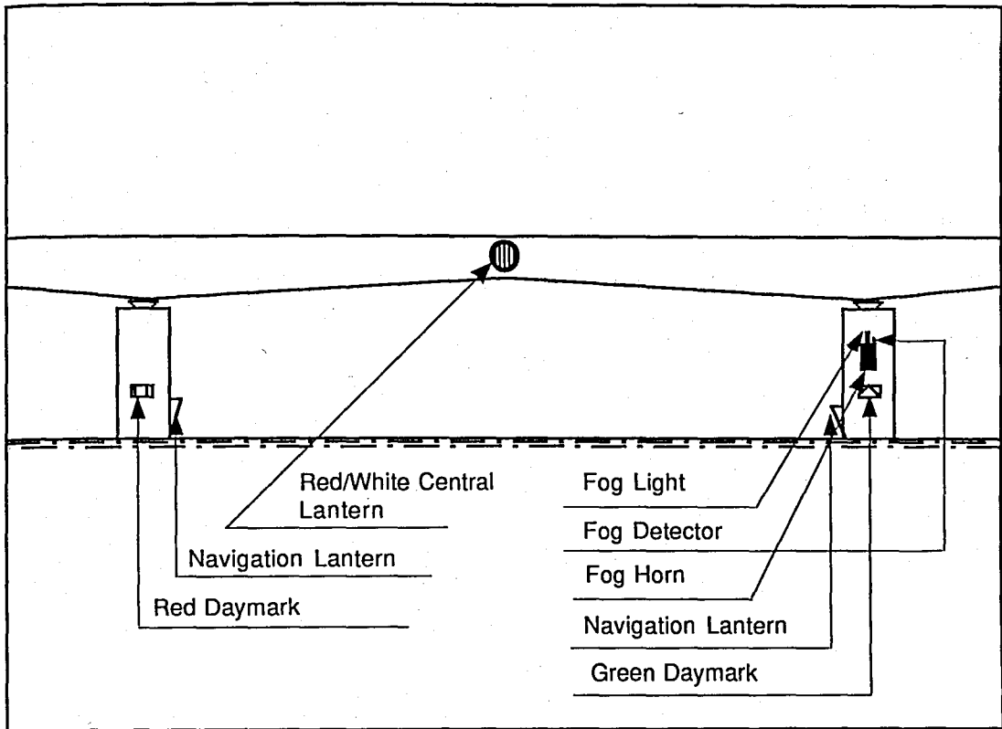
FIGURE 9.11. NAVIGATION EQUIPMENT MOUNTED ON THE NAVIGATION SPAN OF THE GREAT BELT WESTERN BRIDGE
