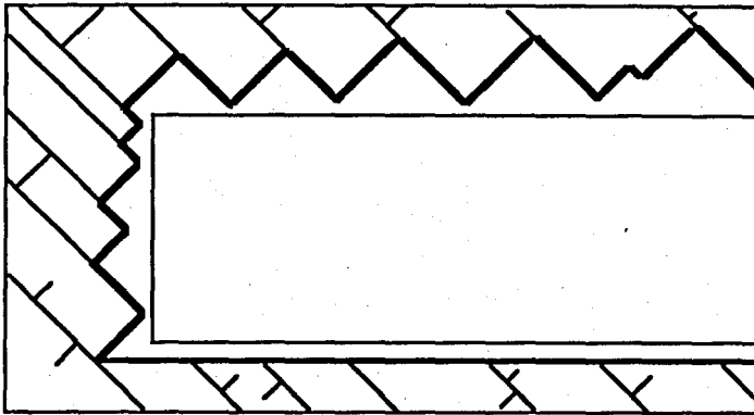
(b) Tunnel following in direction of dip
