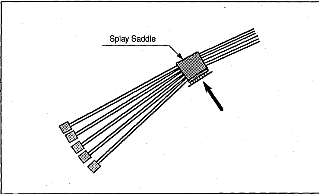
FIGURE 4.8. ONE-SIDED FLARING OF STRANDS FROM SPLAY SADDLE
