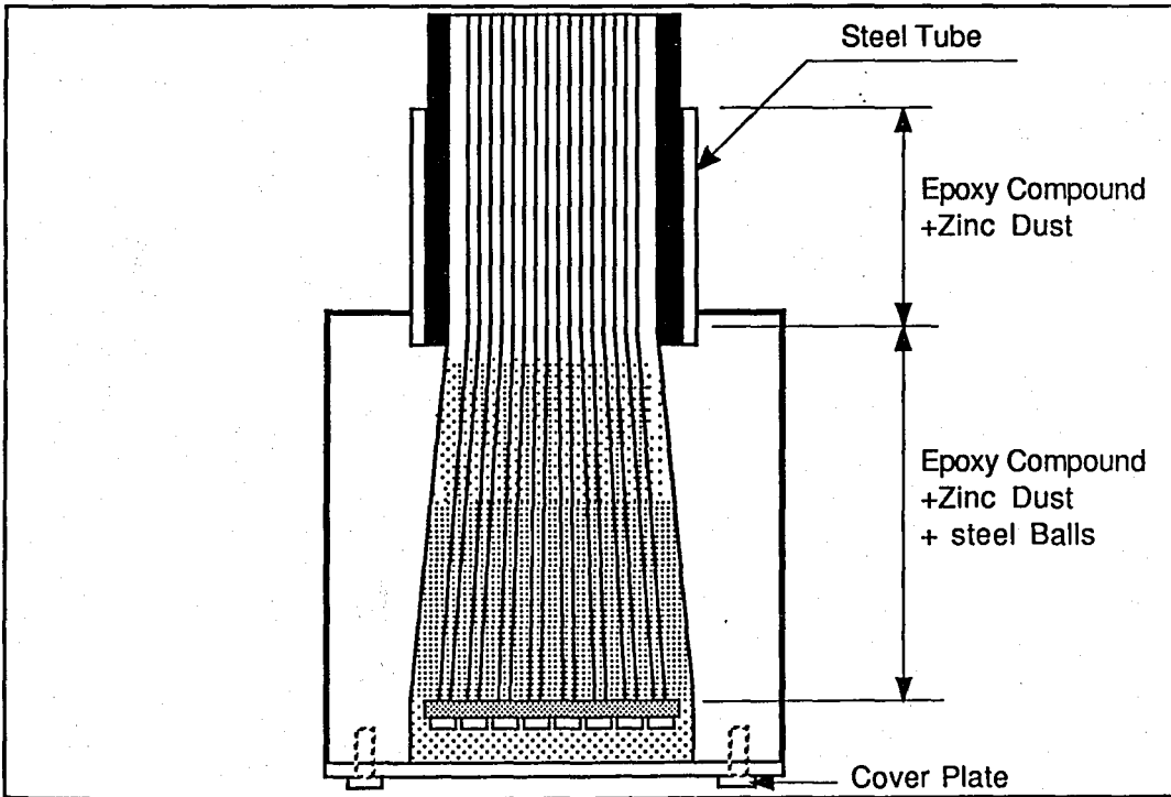
FIGURE 4.4. HIAM SOCKET
