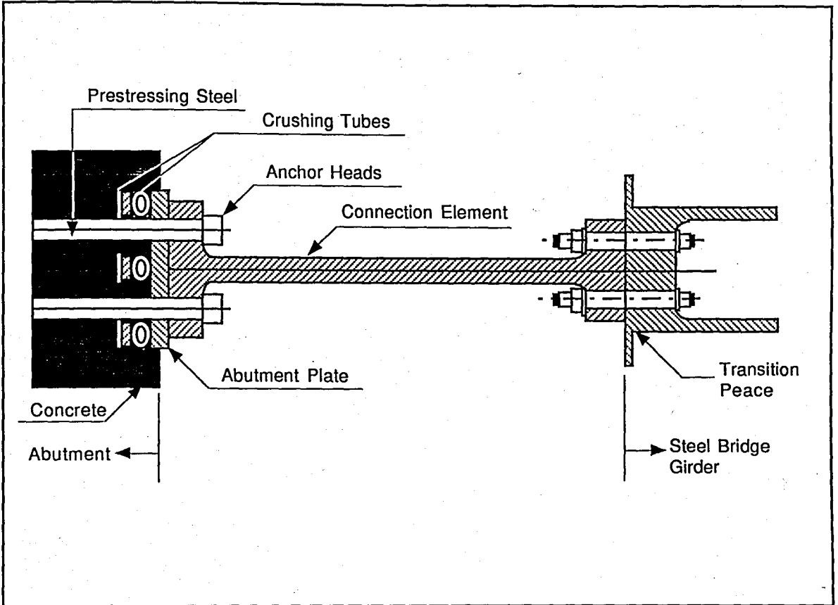
FIGURE 15.13. DETAIL OF FLEXIBLE PLATE CONNECTION
