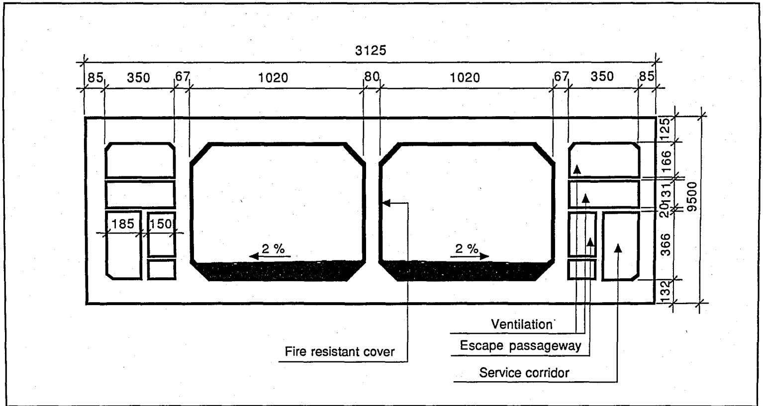
FIGURE 20.3. CROSS SECTION (in mm)
