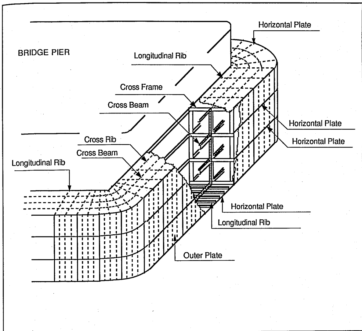
FIGURE 9.14. FRAMED STEEL FENDER SYSTEM USED FOR PROTECTION OF THE BISAN-SETO BRIDGES, JAPAN
