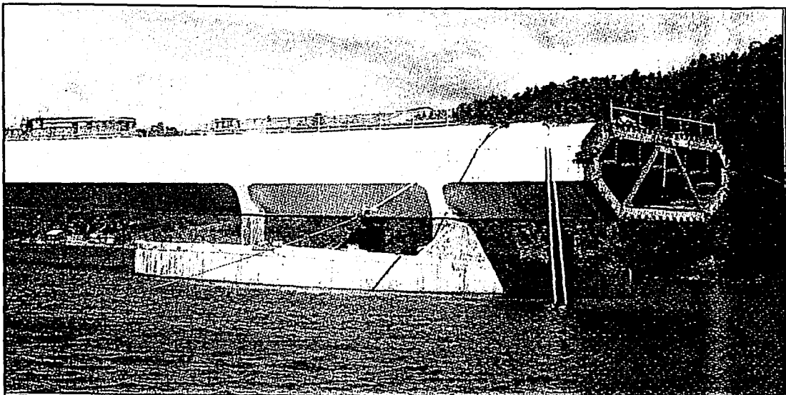
FIGURE 15.9. THE STEEL BOX GIRDERS (Courtesy of McGraw-Hill, 1994)
