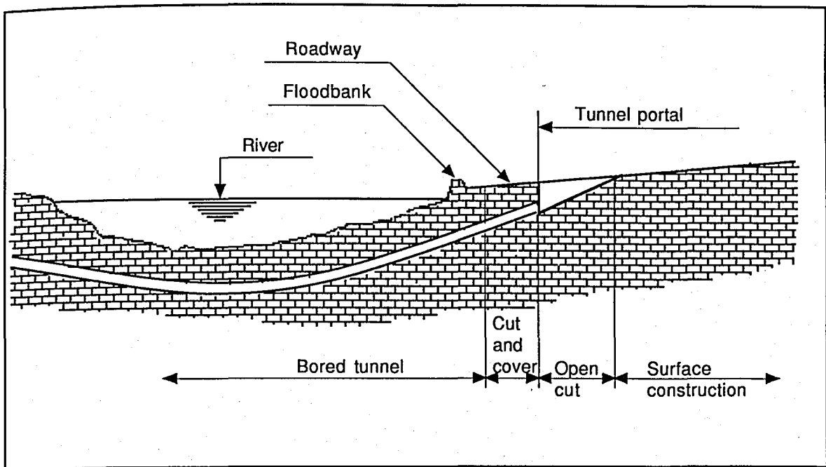
FIGURE 19.1. SUBAQUEOUS TUNNEL
