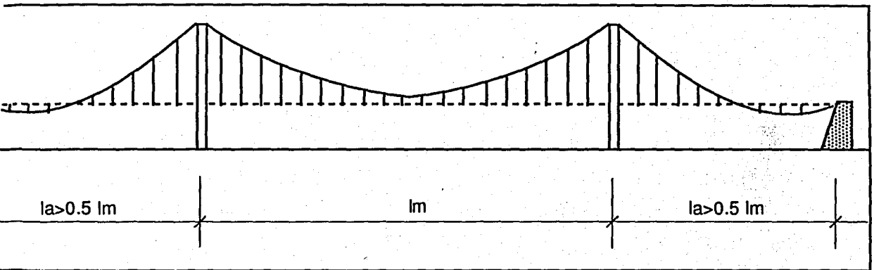
FIGURE 3.6. THREE-SPAN SUSPENSION BRIDGE WITH EXTREME SIDE SPANS
