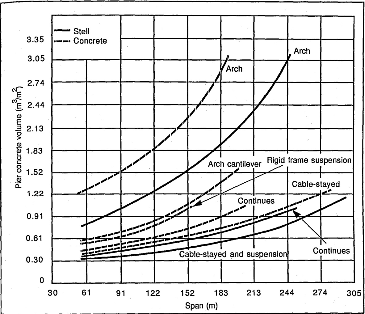
FIGURE 6.8. PIER CONCRETE VOLUME VERSUS SPAN OF BRIDGE
