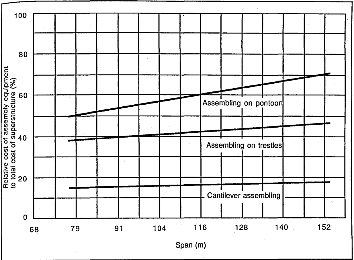
FIGURE 6.5. RELATION OF ASSEMBLY EQUIPMENT AND TOTAL COST TO SPAN OF BRIDGE
