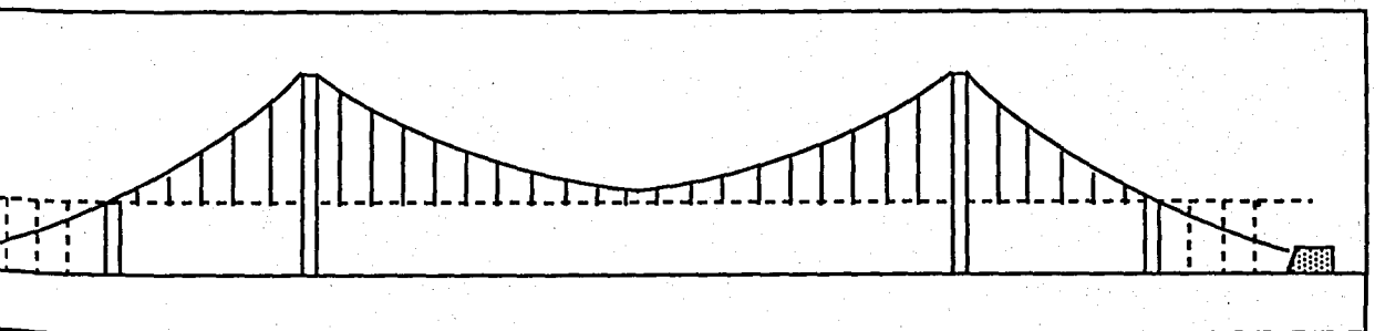
FIGURE 3.7. SUSPENSION BRIDGE WITH SECONDARY PYLONS AND THE MAIN CABLE CONTINUED TO LOW ANCHOR BLOCKS
