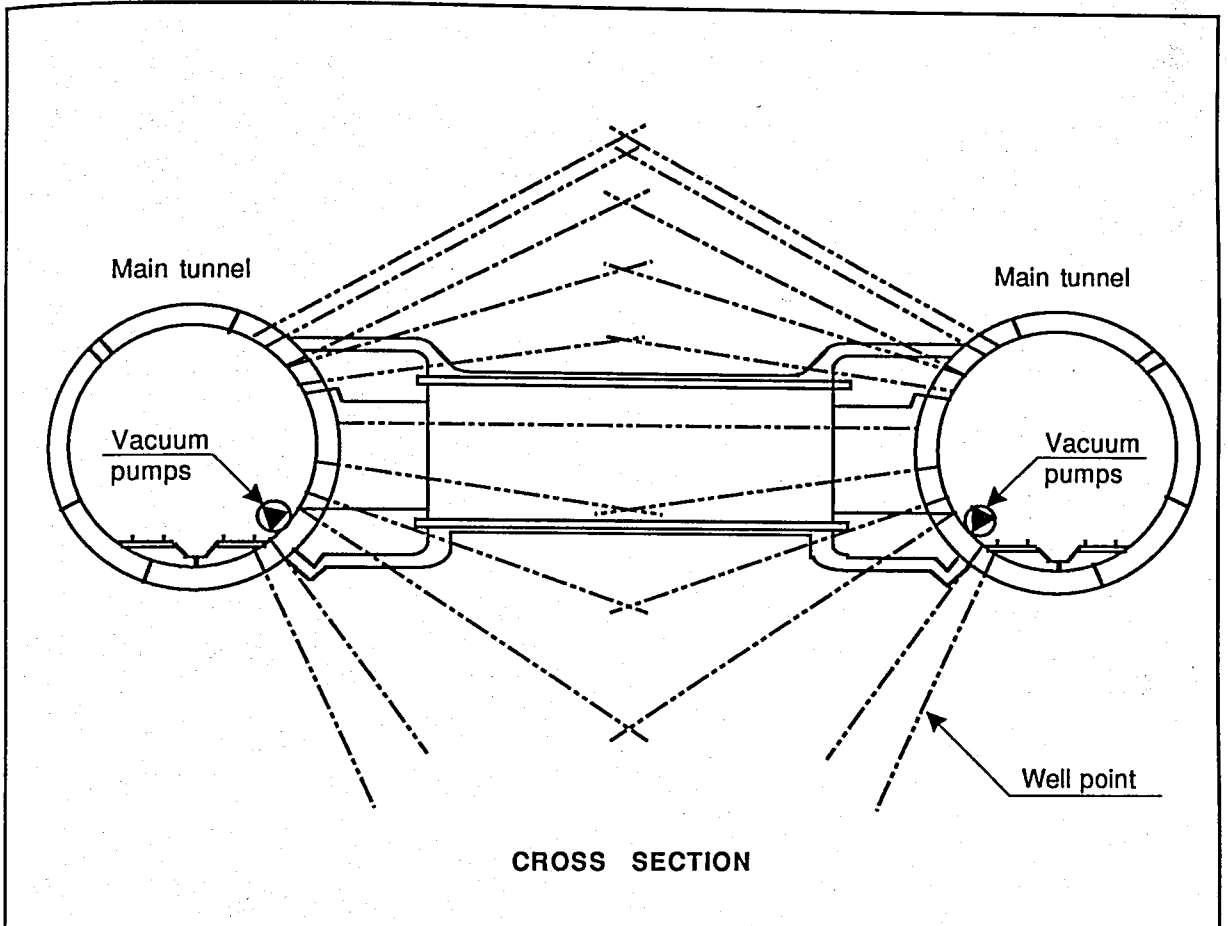
FIGURE 21.3. WELLPOINT ARRAY AT CROSS PASSAGE
