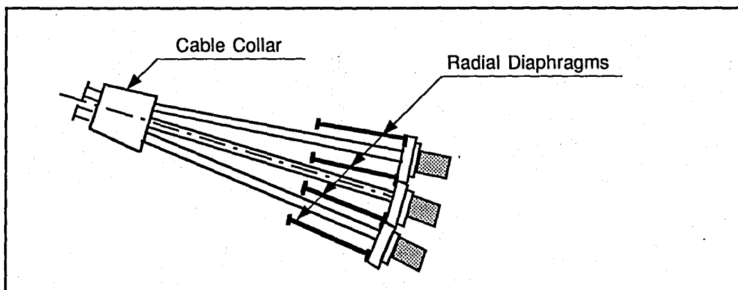
FIGURE 4.7. ANCHORAGE OF A MULTI-STRAND CABLE
