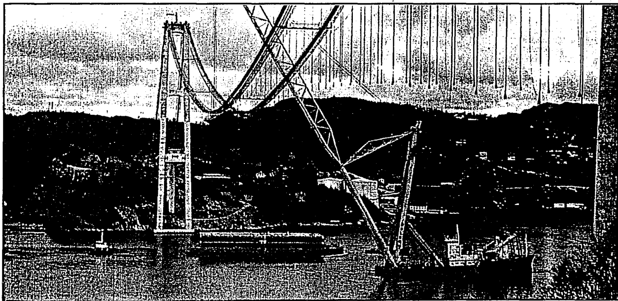
FIGURE 12.10. LIFTING OF THE GIRDER SEGMENTS (Courtesy of Monberg and Thorsen A/S, 1994)
