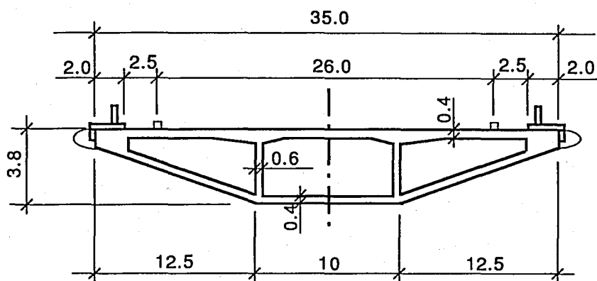
FIGURE 25.13. CROSS SECTION OF THE ACCESS SPAN DECK (In meters)
