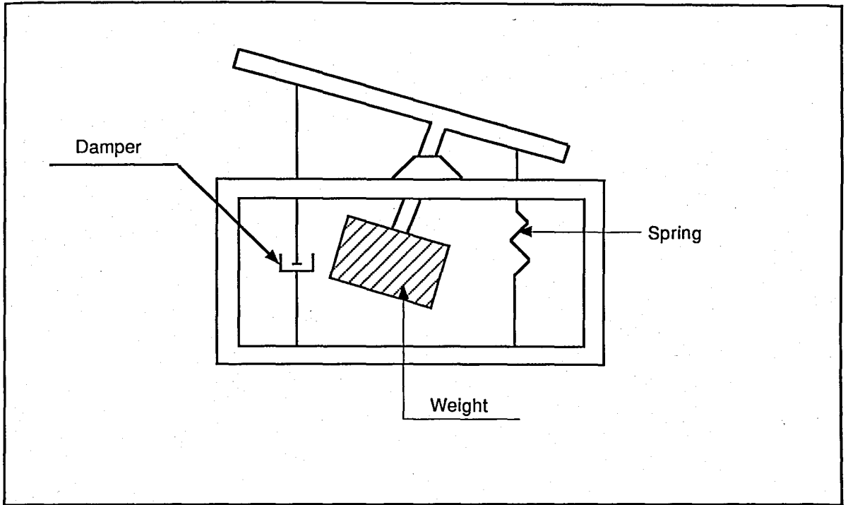
FIGURE 11.6. TUNED-MASS DAMPER
