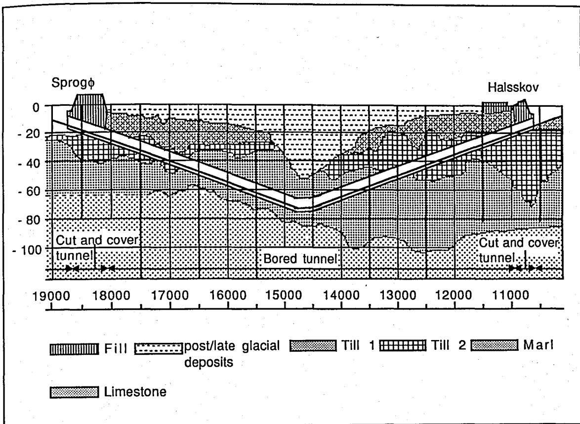
FIGURE 21.2. LONGITUDINAL SECTION (In meters)
