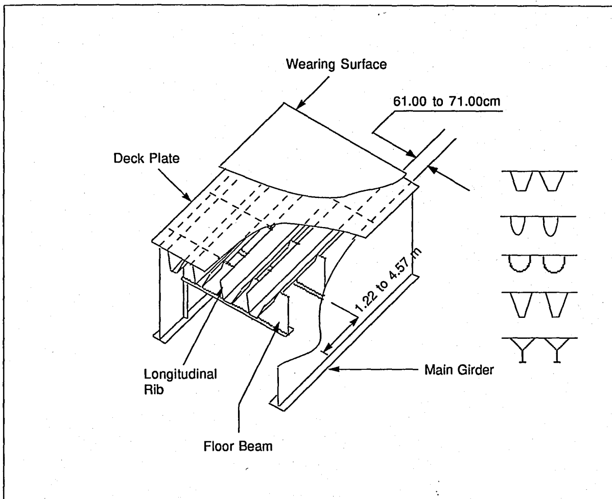
FIGURE 2.7. ORTHOTROPIC DECK BRIDGES; CLOSED RIBS
