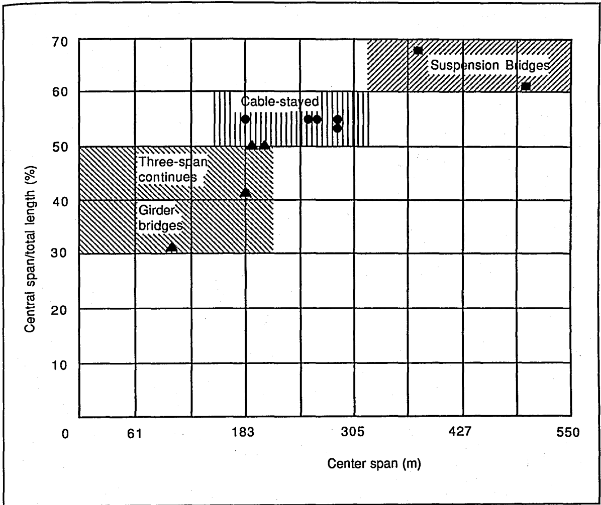
FIGURE 6.1. BRIDGE TYPE SPAN COMPARISON
