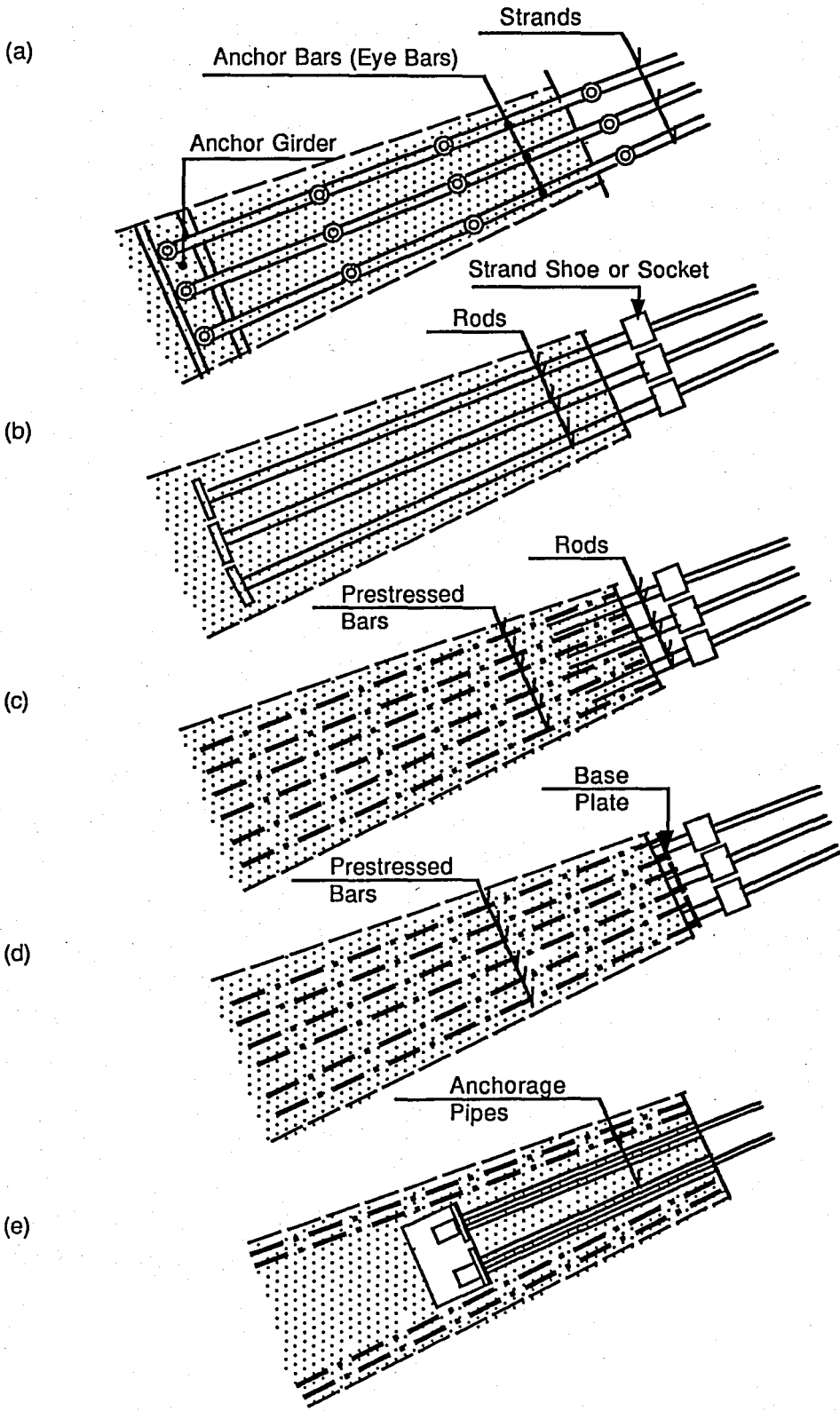
FIGURE 4.28. FIVE SOLUTIONS FOR THE TRANSMISSION OF STRAND FORCES.
