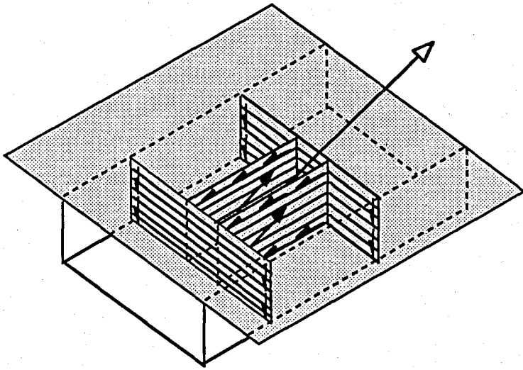
FIGURE 4.11. CONNECTION BETWEEN A LARGE MULTI-STRAND STAY CABLE AND A WIDE MONO-CELLULAR STIFFENING GIRDER
