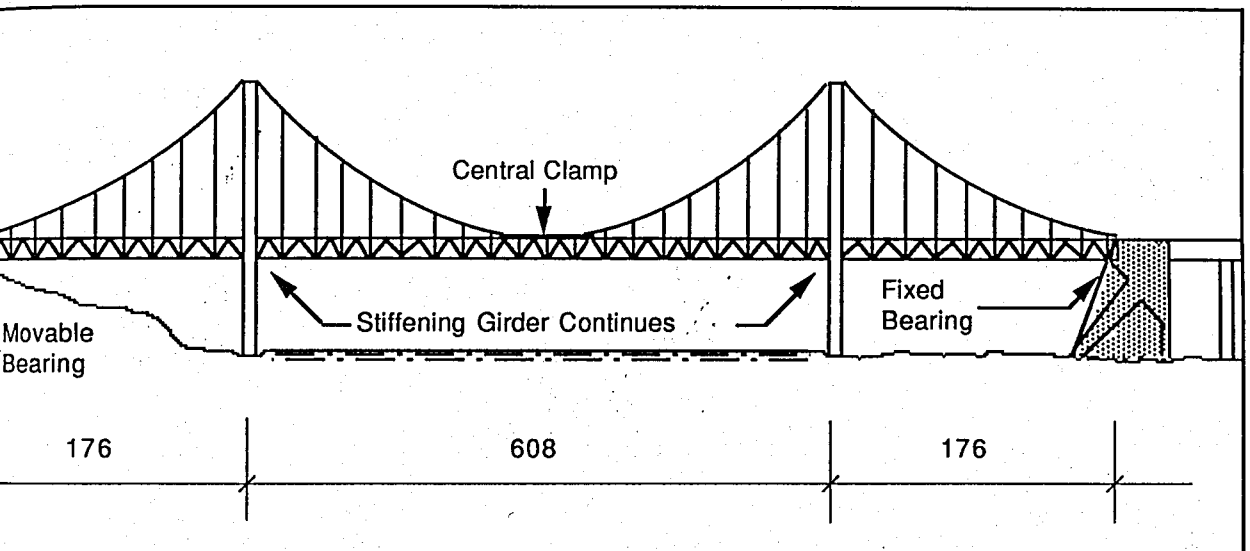
FIGURE 3.9. TANCARVILLE BRIDGE (In meters)
