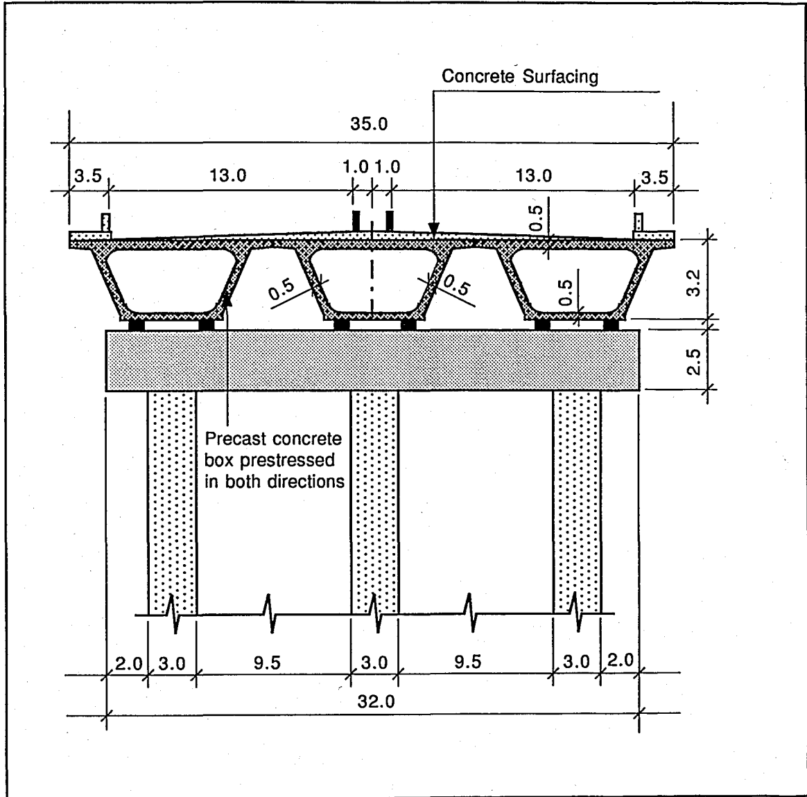
FIGURE 25.11. CROSS SECTION, APPROACH SPANS (in meters)
