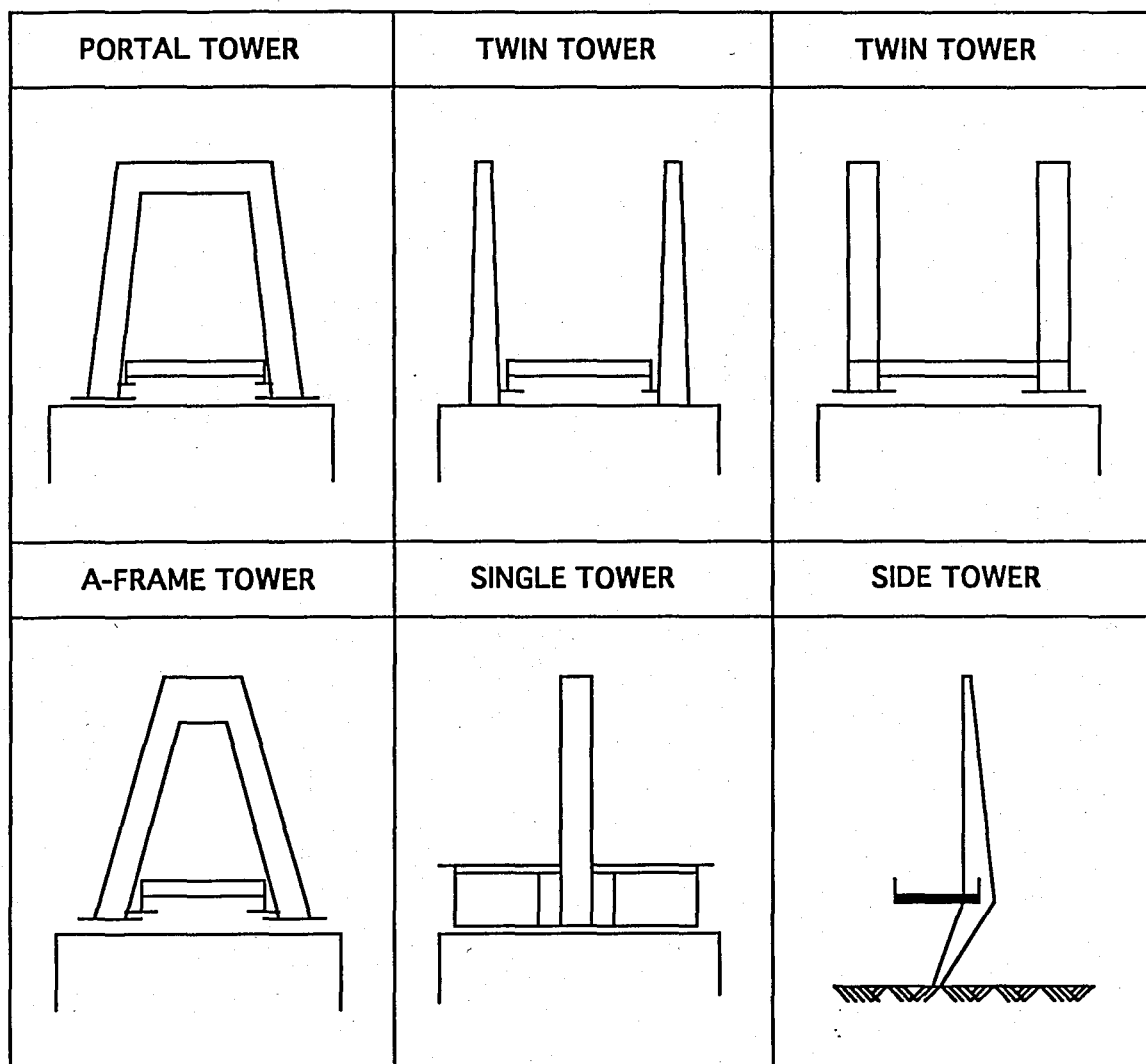
FIGURE 2.4. TOWER TYPES
