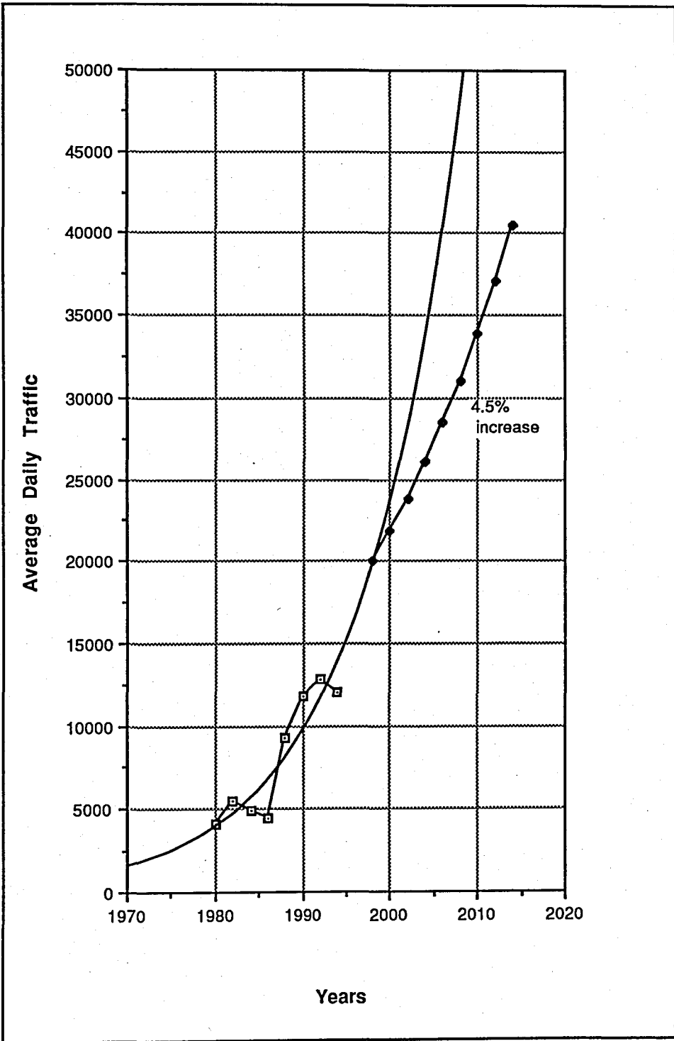
FIGURE 26.1. TRAFFIC FORECAST
