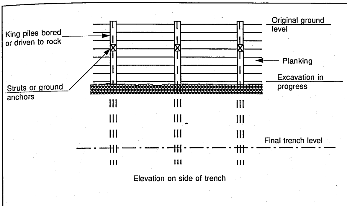
FIGURE 19.3. KING PILES
