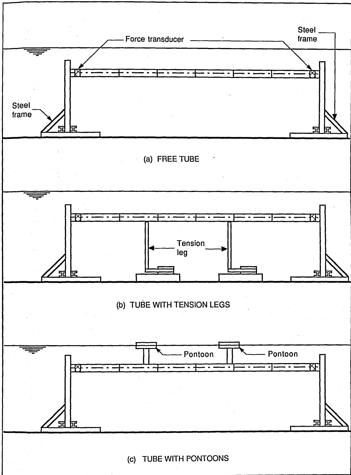
FIGURE 8.5. SUBMERGED FLOATING TUBE BRIDGE MODELS
