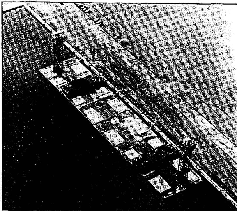
FIGURE 20.5. THE TUNNEL UNIT AT THE FINISHING JETTY (Courtesy of J. Krokeborg, 1990)
