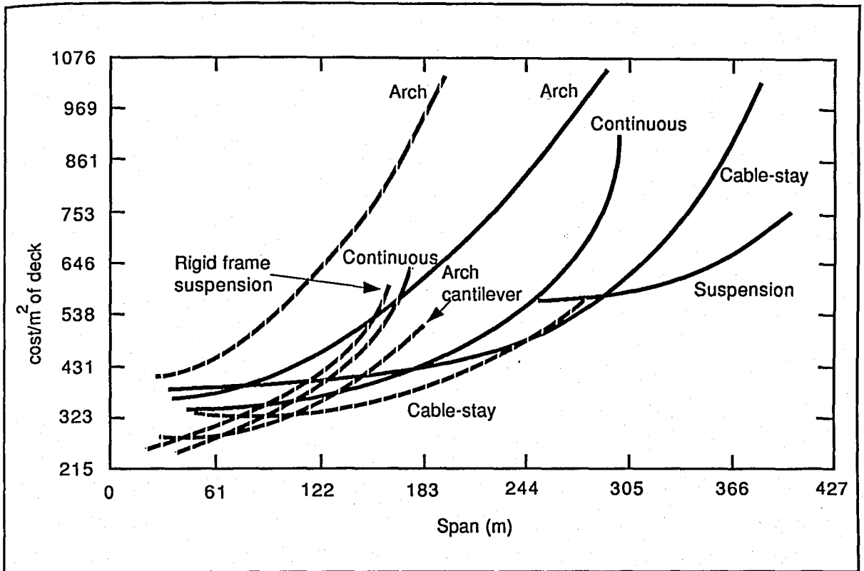
FIGURE 6.9. COST PER \text{m}^2 DECK VERSUS SPAN
