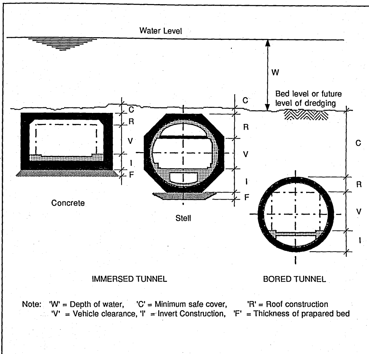
FIGURE 16.1. COMPARATIVE DEPTHS REQUIRED FOR TUNNELS
