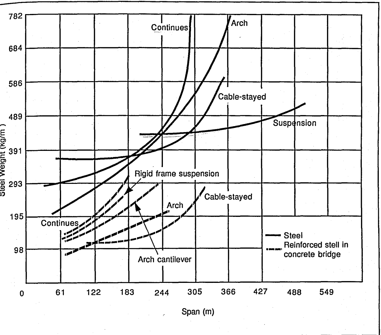
FIGURE 6.7. STEEL SUPERSTRUCTURE WEIGHT VERSUS SPAN OF BRIDGE
