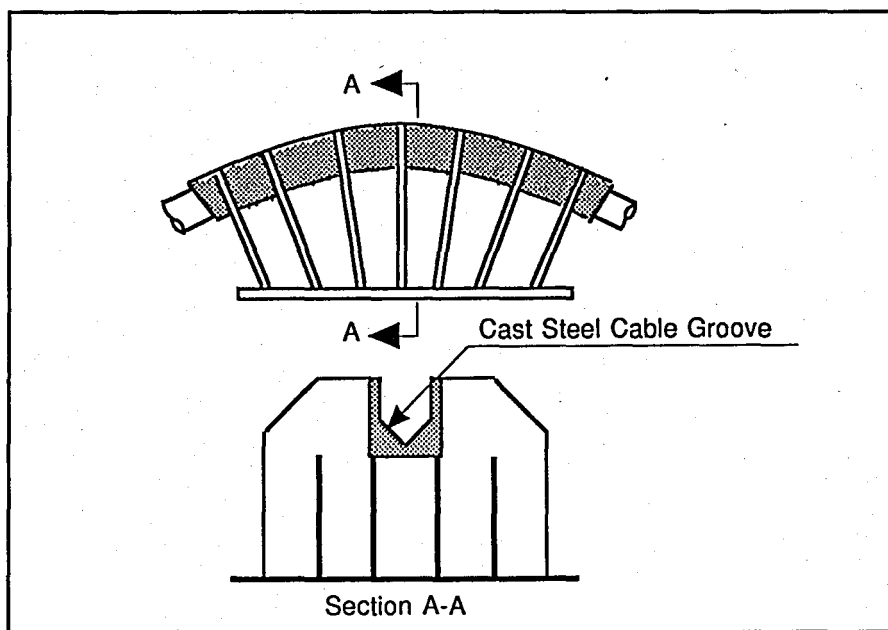
FIGURE 4.26. CABLE SADDLE
