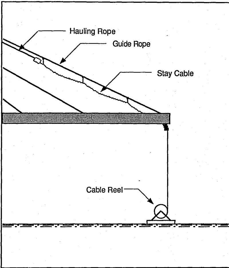
FIGURE 5.12. PARALLEL-WIRE CABLE SUPPORTED BY TROLLEYS
