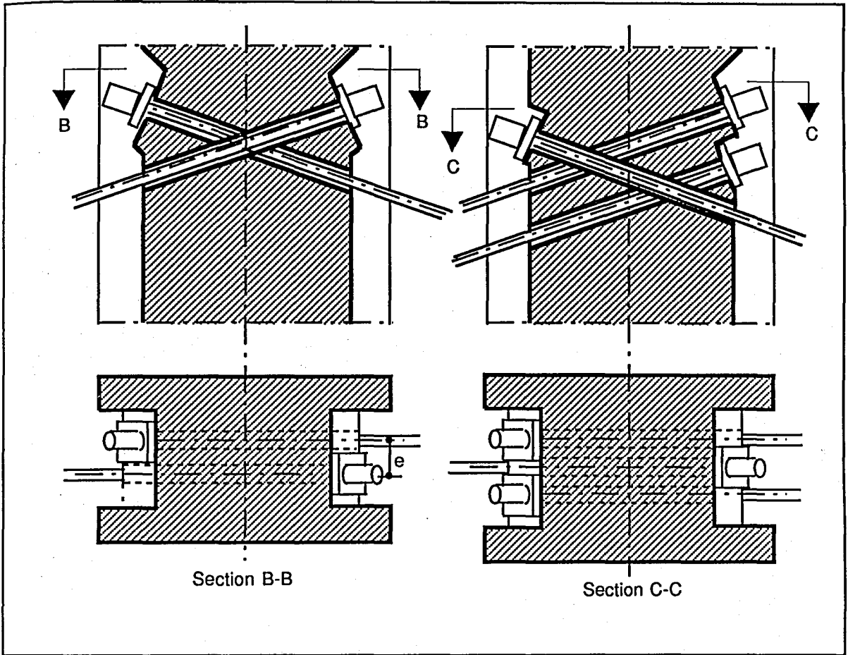
FIGURE 4.23. OVERLAPING OF STAY CABLE ANCHORAGES IN A CONCRETE PYLON
