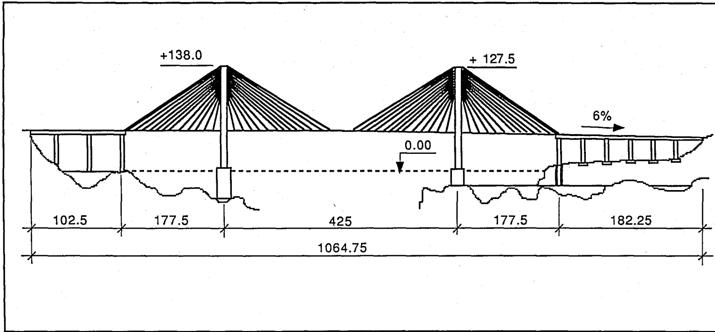
FIGURE 10.7. ELEVATION (in meters)
