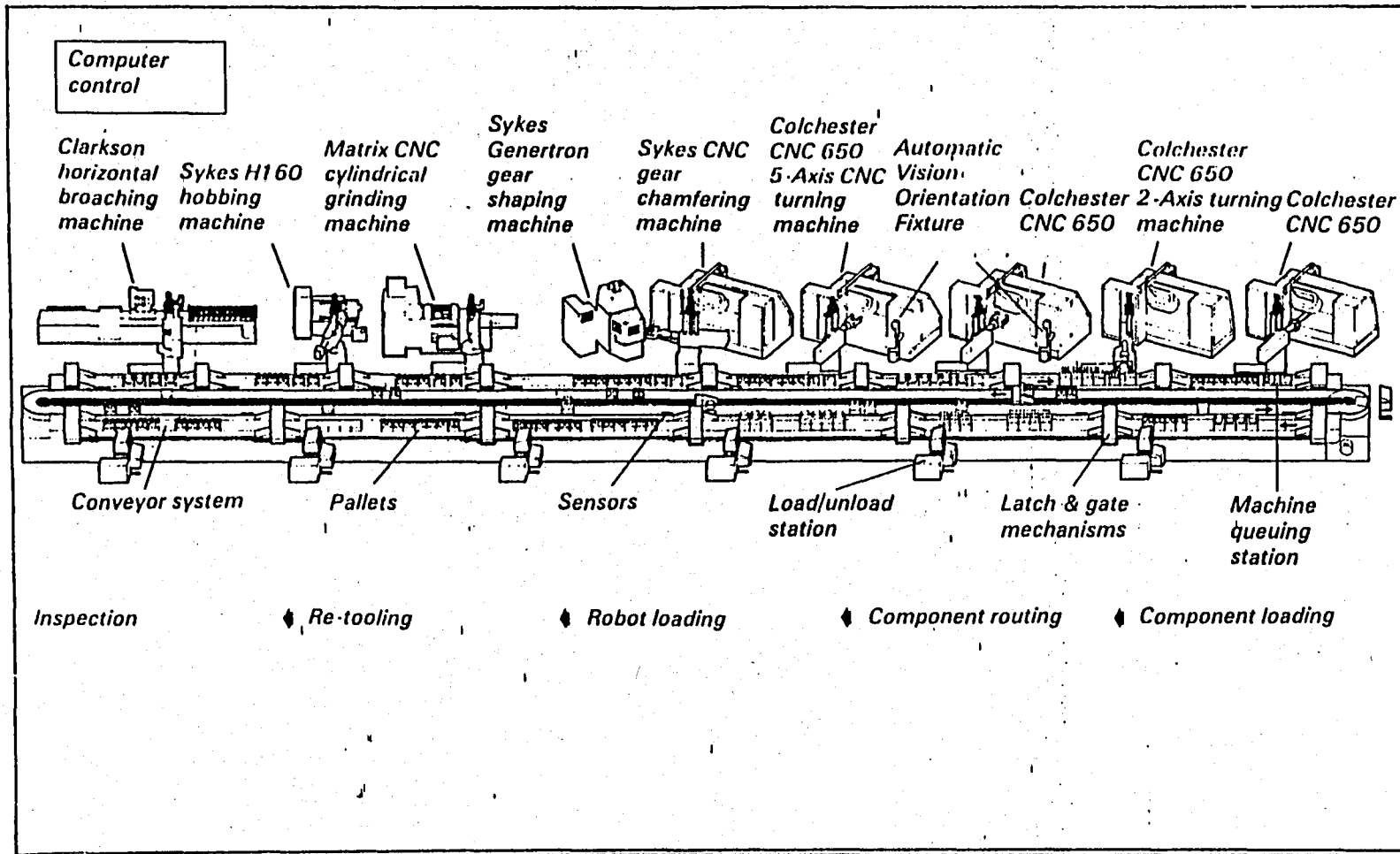
Figure 2.7 The SCAMP FMS [4]
