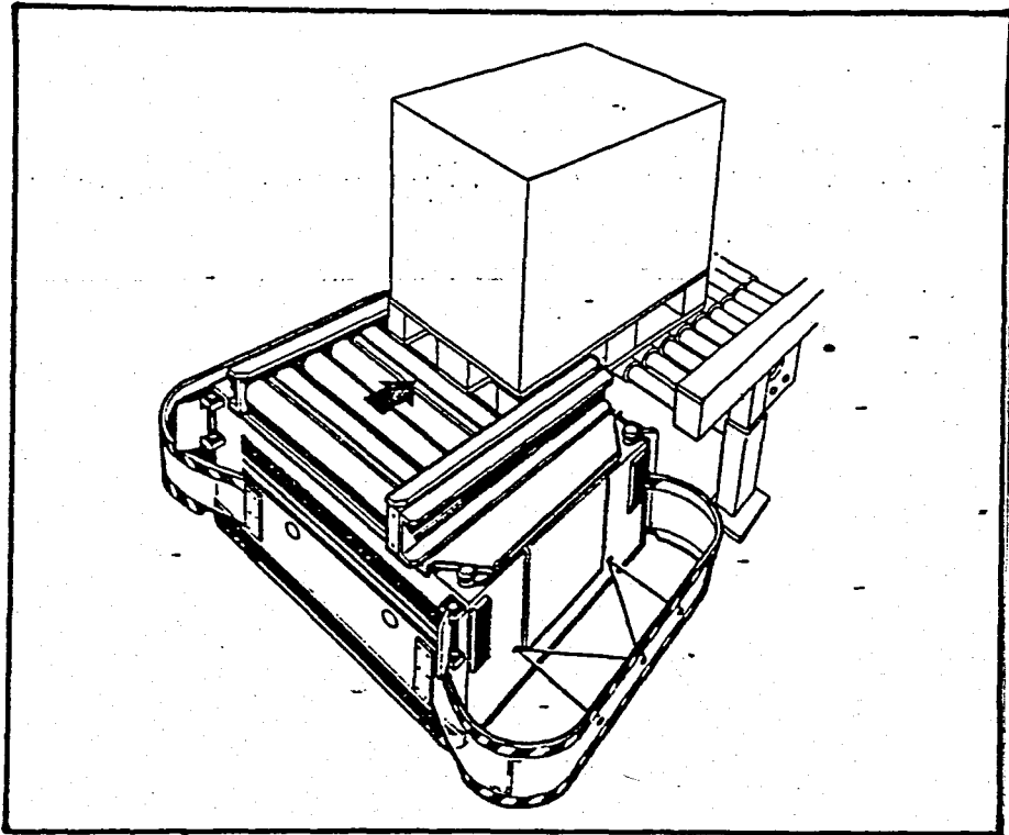
Figure 2.5 Unit load carrier [6]
