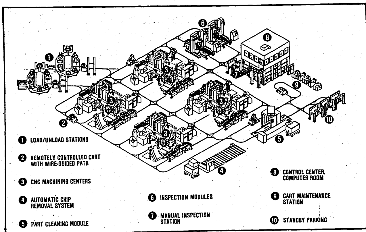
Figure 2.9 The FMS of VOUGHT Aero Products Division [2]
