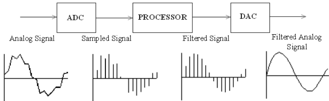
Figure 4.17. Analog to Digital Conversion process to get the desired analog signal at the output
