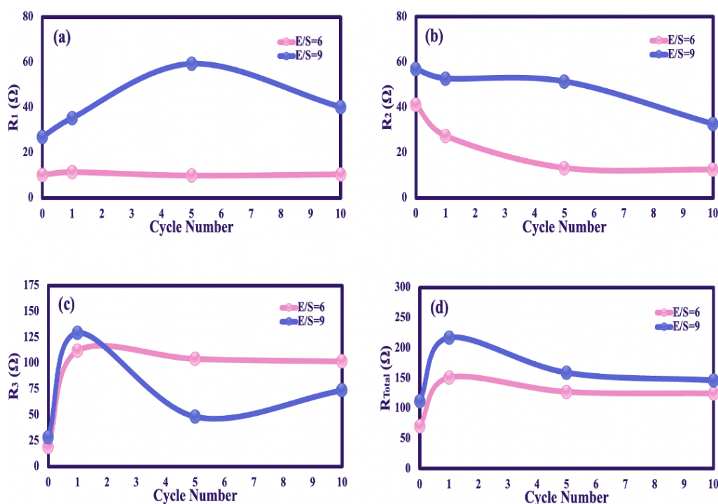
Figure 5.18. Change in (a) R_1 , electrolyte resistance, (b) R_2 , charge transfer resistance, (c) R_3 , \text{Li}_2\text{S} film resistance, and (d) R_{\text{Total}} , total resistance of cells with \text{LiClO}_4 in sulfolane (SL) at E/S ratio of 6 \mu\text{L}/\text{mg} and 9 \mu\text{L}/\text{mg} .
