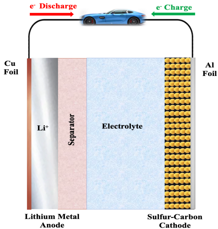
Figure 1.1. Schematic description of lithium-sulfur (Li-S) batteries.
