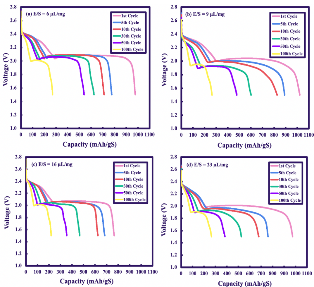
Figure 5.8. Discharge profiles of the Li-S cells with E/S ratios of (a) 6 \mu\text{L}/\text{mg} , (b) 9 \mu\text{L}/\text{mg} , (c) 16 \mu\text{L}/\text{mg} , and (d) 23 \mu\text{L}/\text{mg} for 1M LiTFSI in Sulfolane electrolyte.
