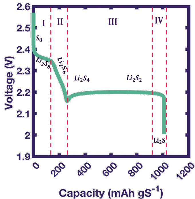
Figure 1.2. Illustration of the discharge profile of Li-S batteries.
