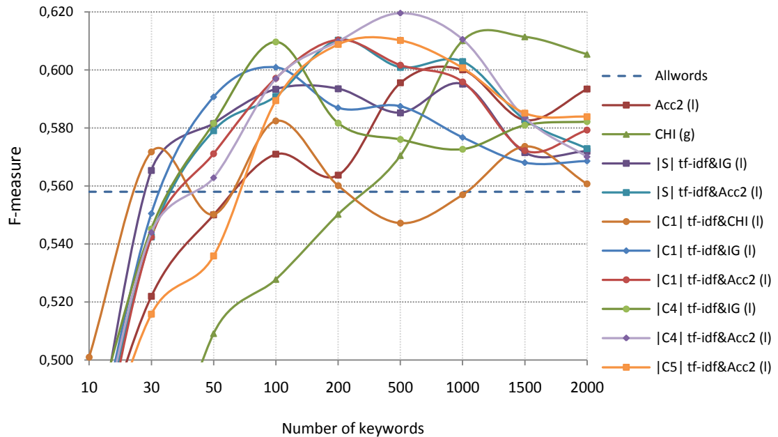
Figure A.4. Performance of the combinations with high macro-averaged F-measures in local policy for Hitech dataset.
