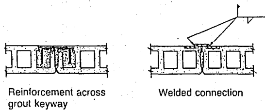
Fig. 16 Alternate longitudinal shear connections
