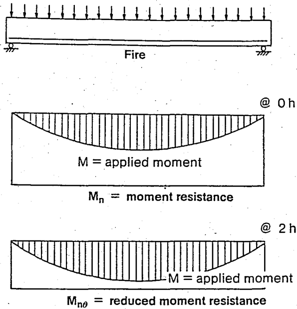
Fig. 6 Moment diagrams for simply-supported beam or slab
