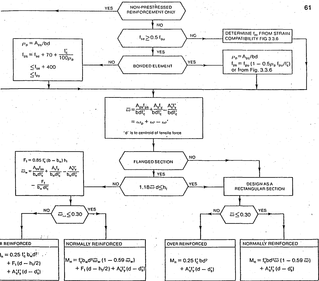
Fig. 27 Flow chart for flexural resistance calculations
