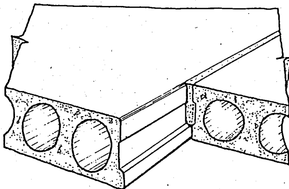
Fig. 15 Typical slab to slab connection
