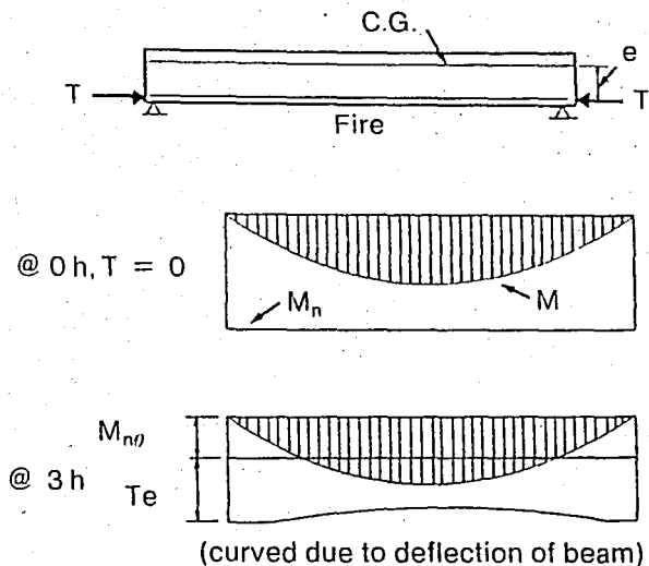
Fig. 10 Axially restrained beam during fire exposure
