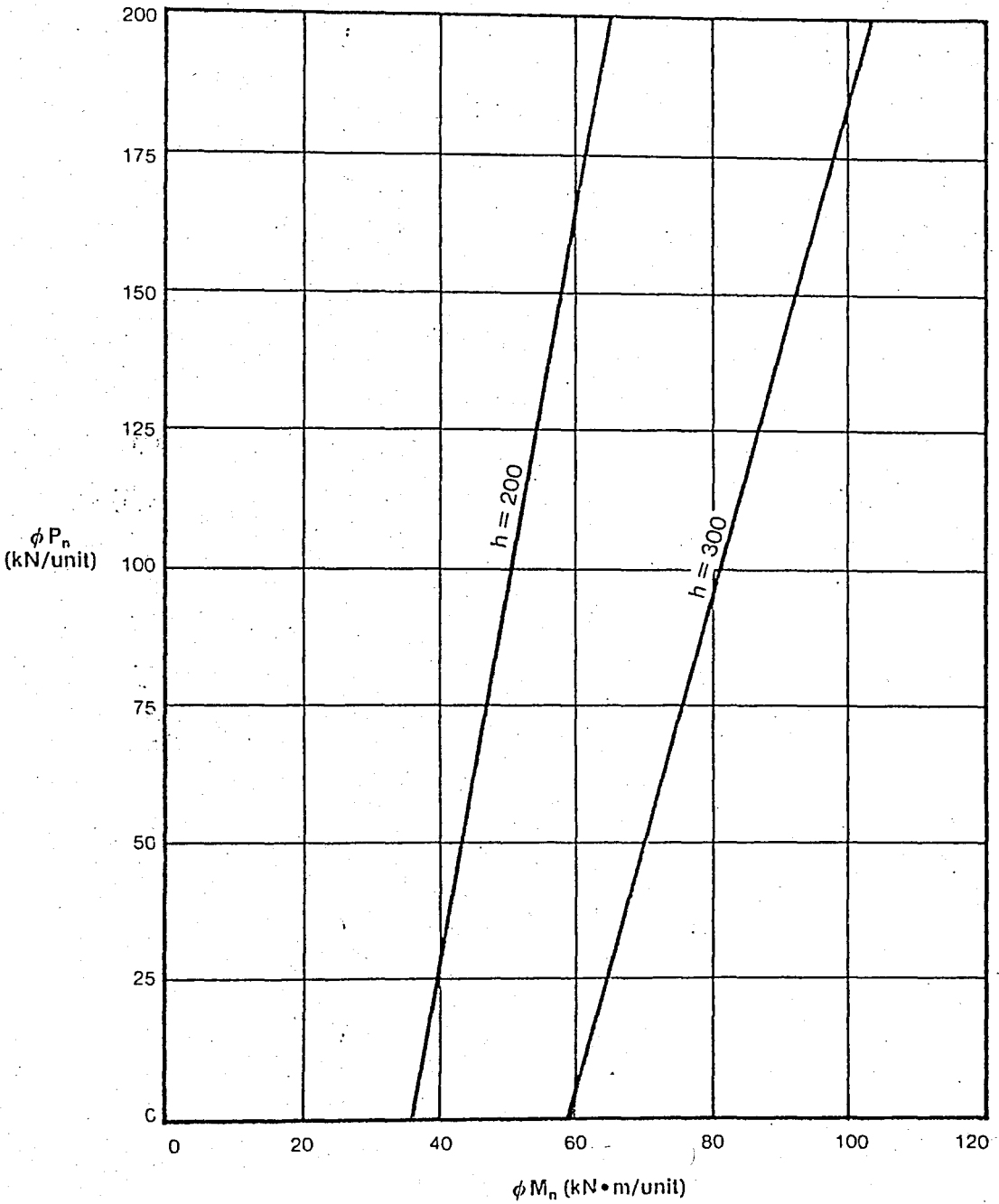
Fig. 14 Partial interaction curve for prestressed hollow-core wall panels
