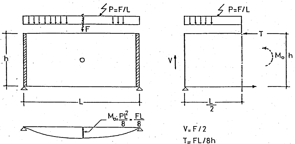
Fig. 23 Simple Beam Action Type 1
