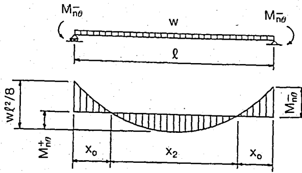
Fig. 9 Symmetrical uniformly loaded element continuous at both supports
