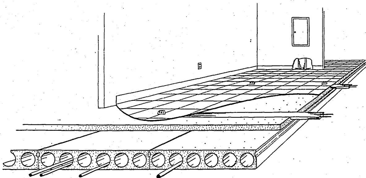
Fig. 13 Use of electrical ducts with slabs within concrete topping
