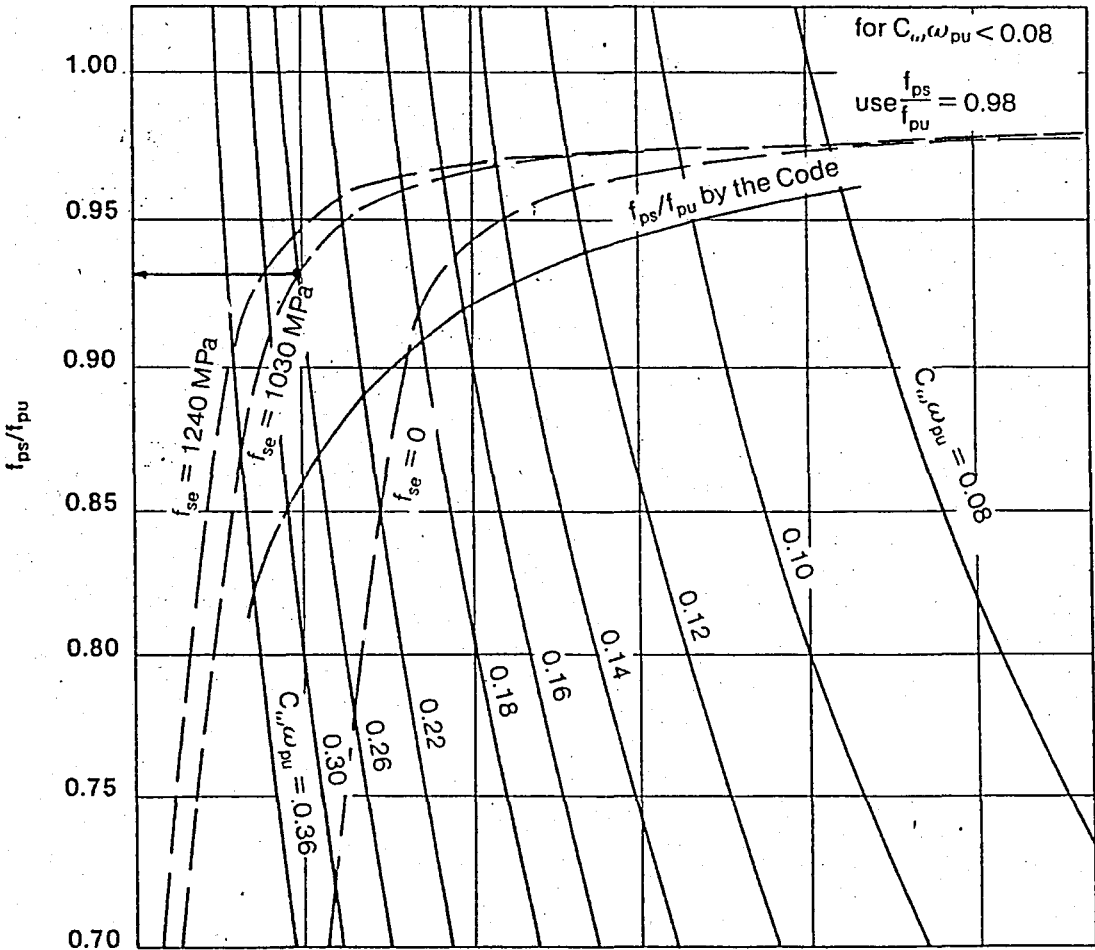
Fig. 26 Values of f_{ps} by stress-strain relationship-bonded strand
