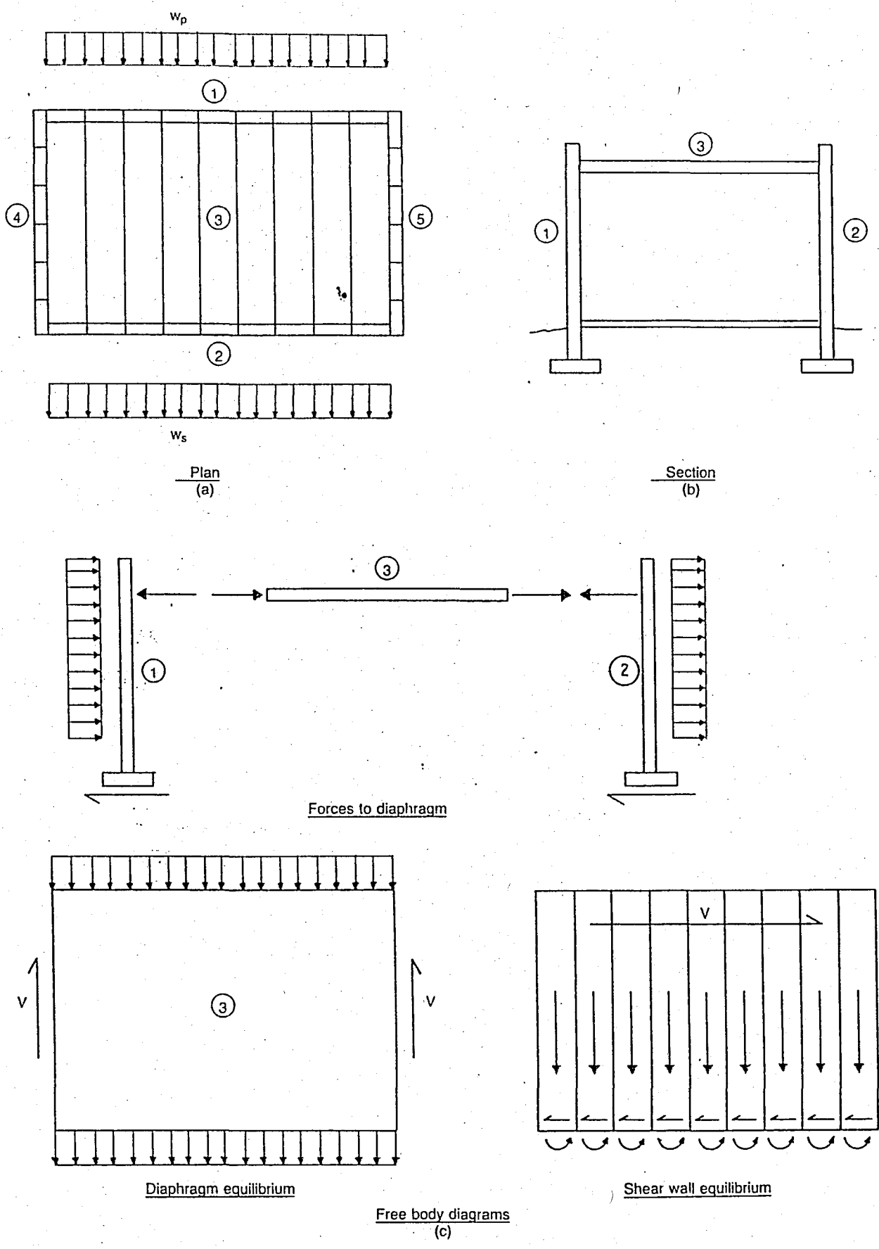
Fig. 22 Elements of a lateral load resisting system
