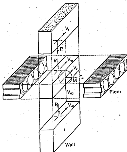
Fig. 19 An interior floor to wall connection
