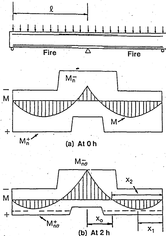
Fig. 7 Moment diagram for two-span continuous beam
