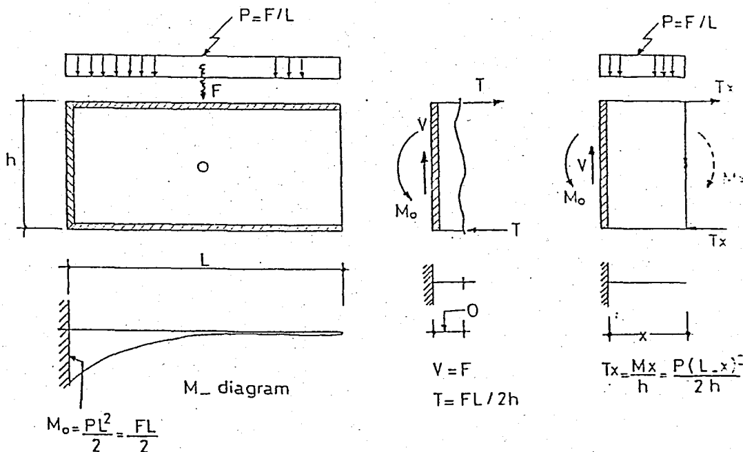
Fig. 24 Cantilever Beam Action Type 2
