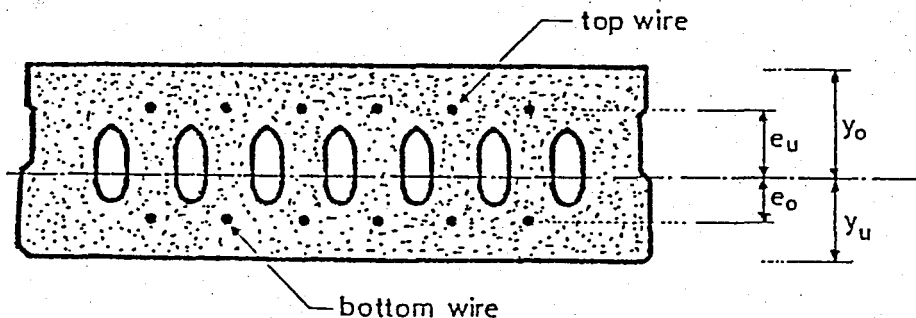
Fig. 37 Cross-section of a cantilever hollow core slab
