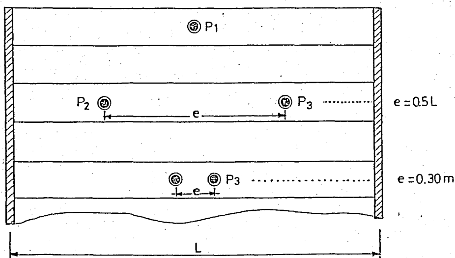
Fig. 31 Locations of maximum point loads
