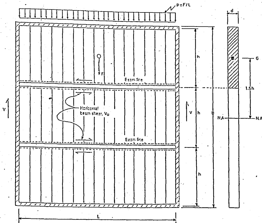
Fig. 17 Multi-bay slab arrangement
