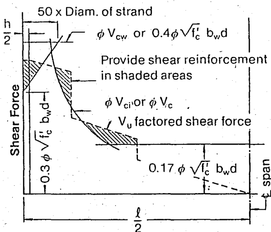
Fig. 29 Shear Diagram
