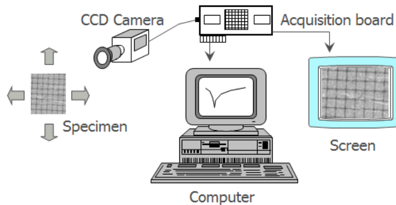
Figure 6.1. DIC setup.
