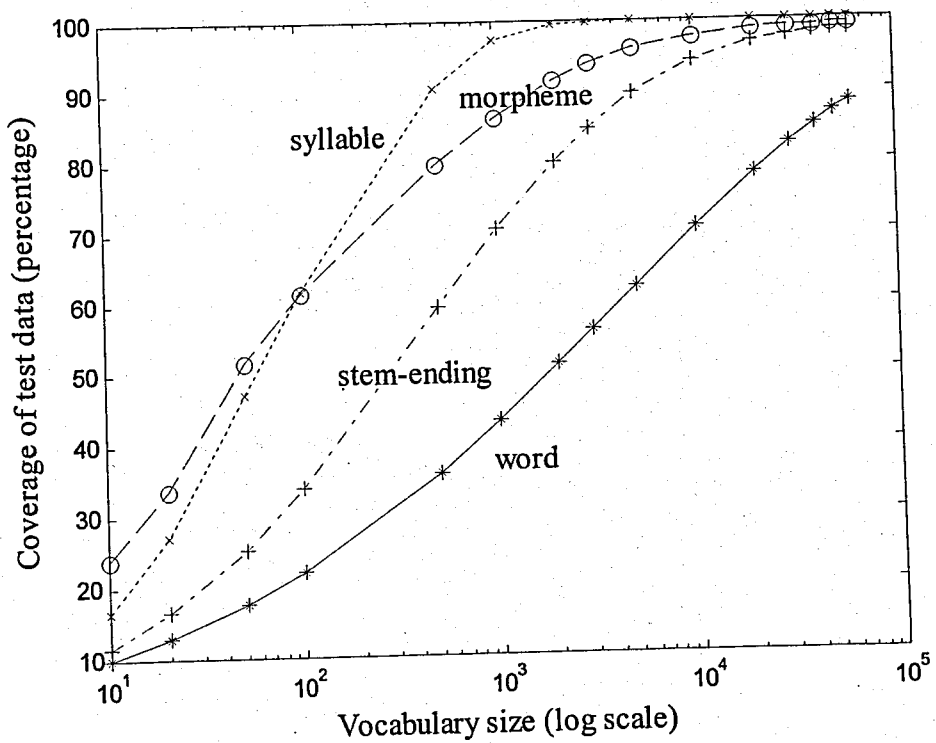
Figure 5.9. Coverage of test data in percentage with respect to vocabulary size
