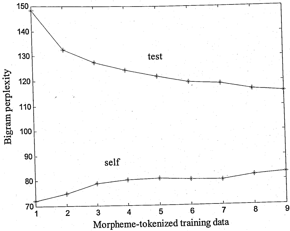
Figure 5.11. Perplexities of bigram language models obtained from morpheme-tokenized training data set with respect to self and test data
