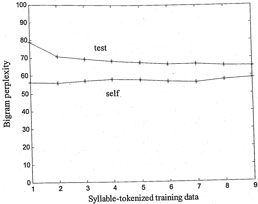
Figure 5.13. Perplexities of bigram language models obtained from syllable-tokenized training data set with respect to self and test data
