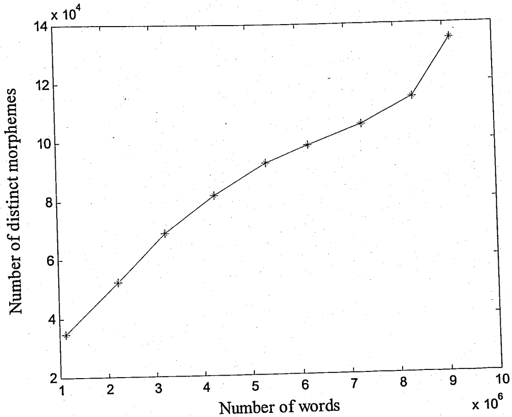
Figure 5.3. Number of distinct tokens (morphemes) versus number of words in the morpheme-tokenized training data set
