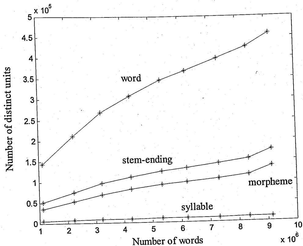
Figure 5.7. Number of distinct tokens versus number of words for training data set
