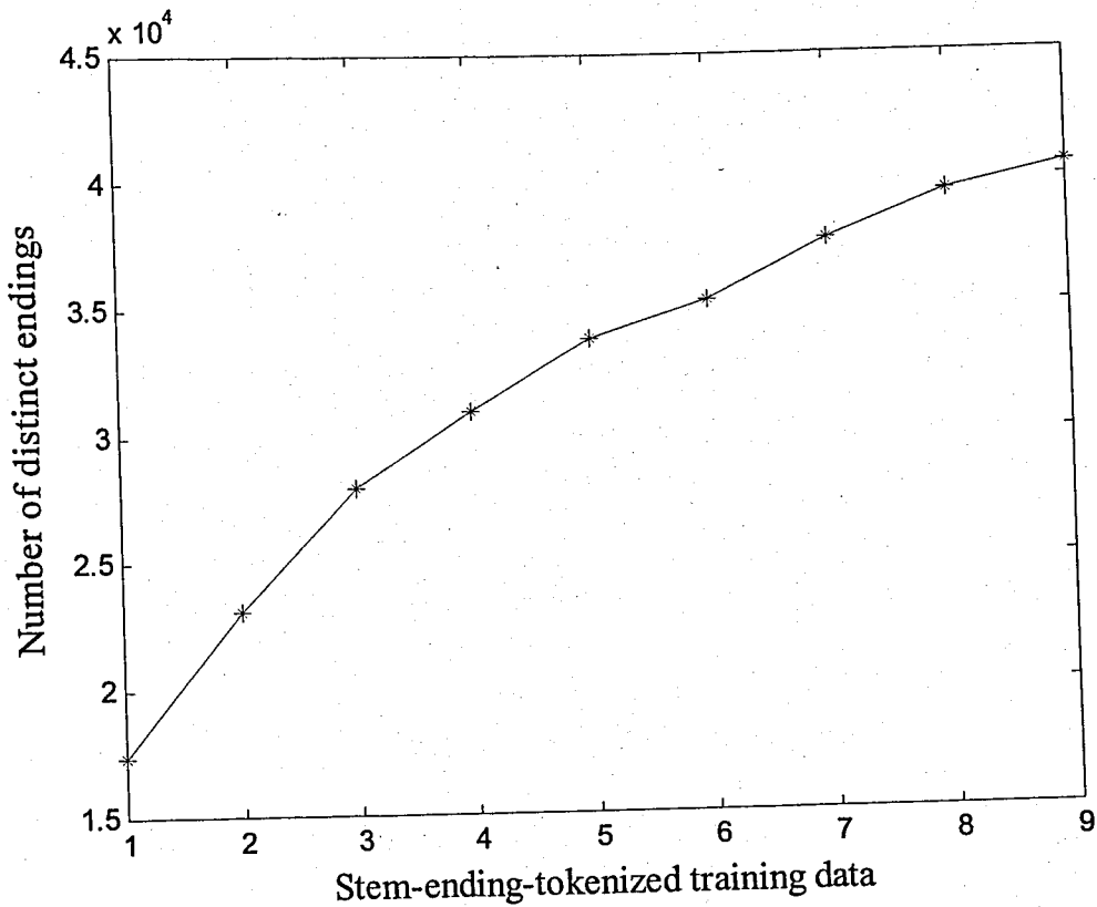
Figure 5.5. Number of distinct endings in the stem-ending-tokenized training texts
