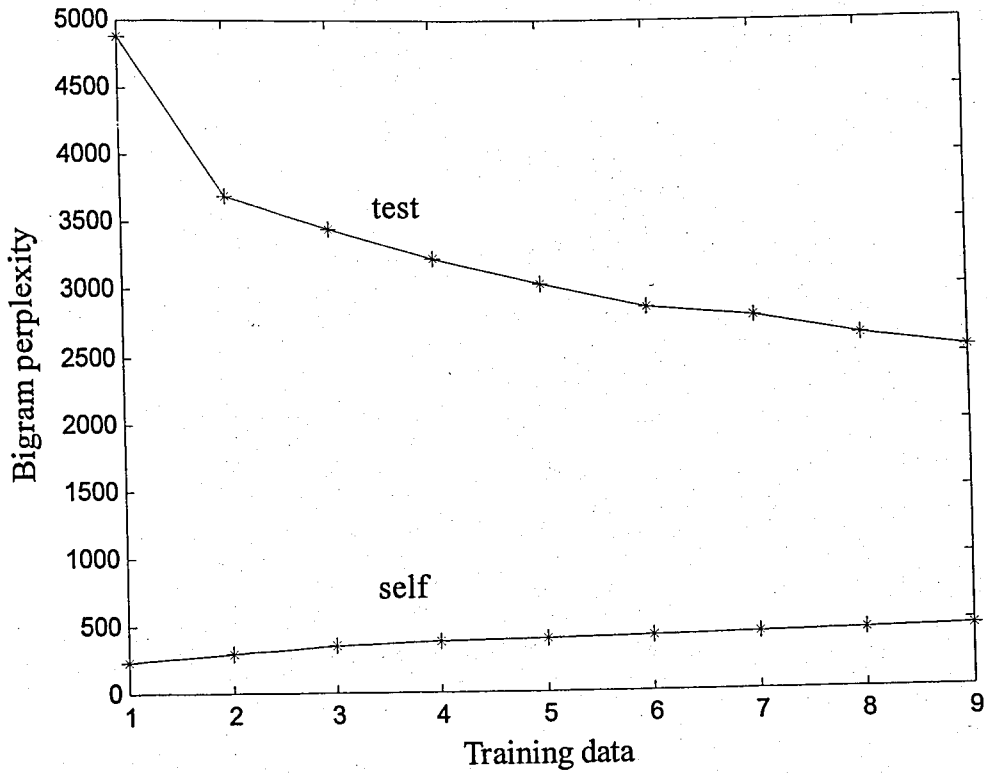
Figure 5.10. Perplexities of bigram language models obtained from word-tokenized training data set with respect to self and test data
