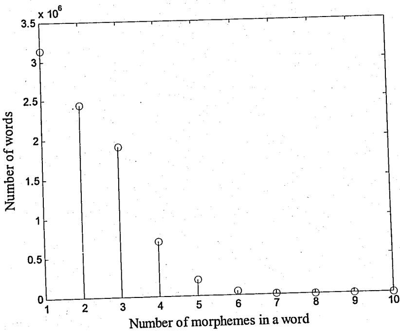
Figure 5.2. Histogram of number of morphemes per word
