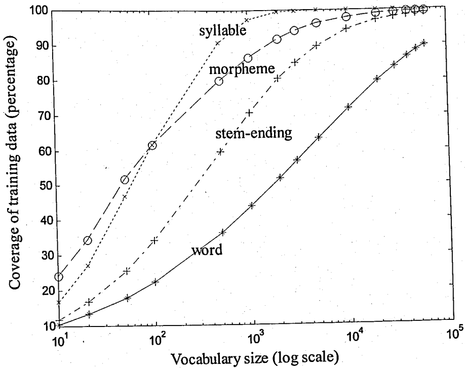
Figure 5.8. Coverage of training data in percentage with respect to vocabulary size
