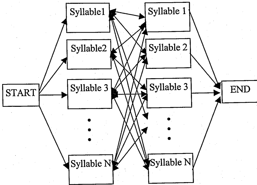
Figure 4.5. Syllable-based word model
