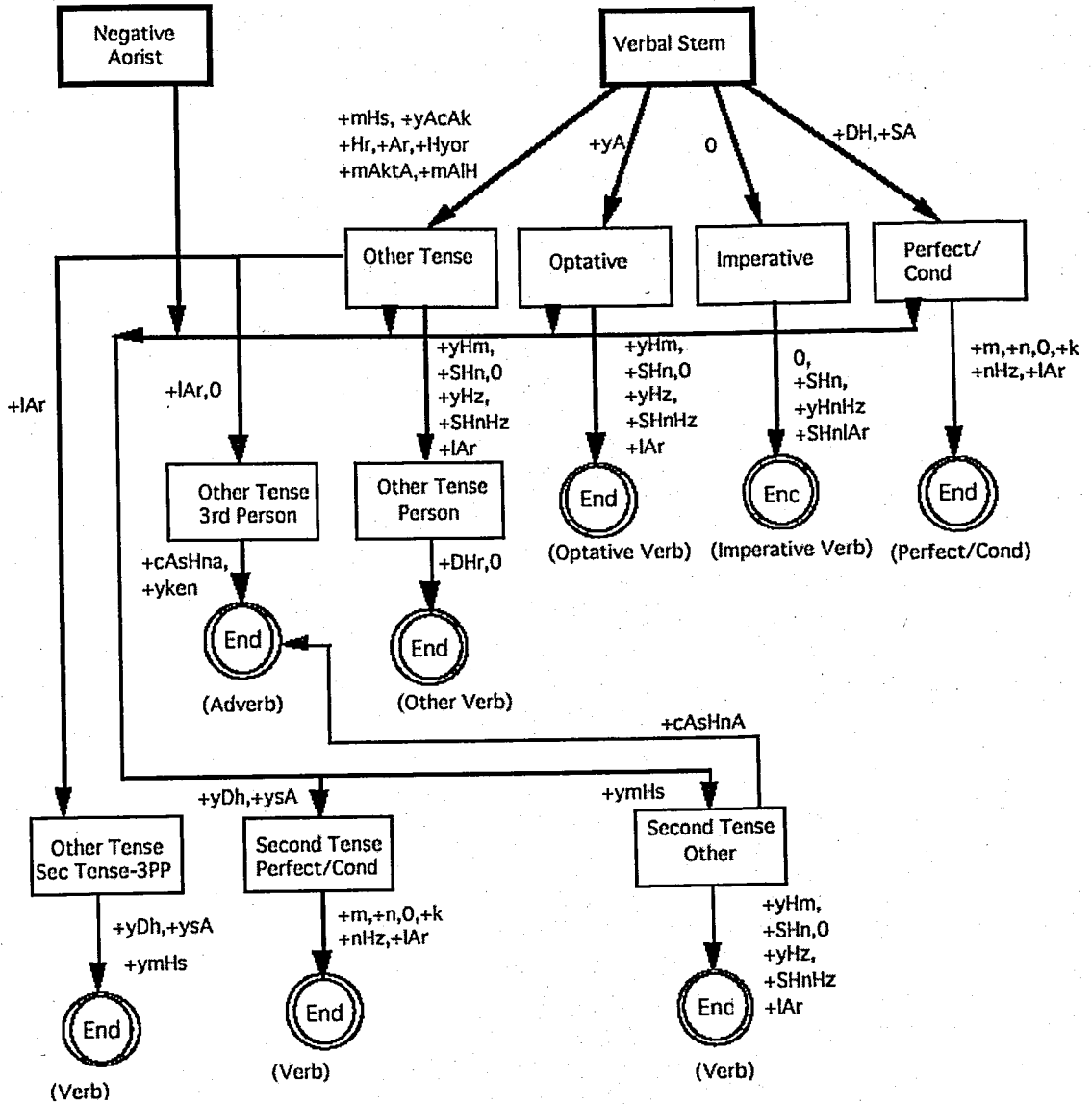
Figure 3.2. Finite state machine for verbs (continued) (Ofizer, 1994)
