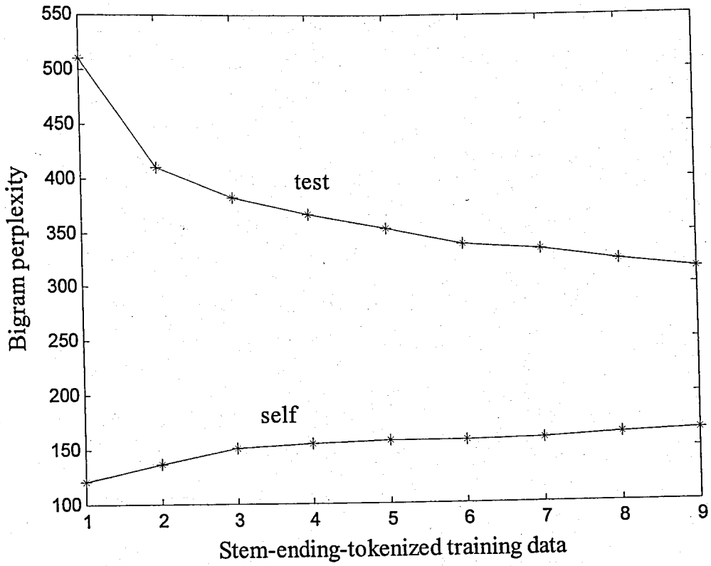
Figure 5.12. Perplexities of bigram language models obtained from stem-ending-tokenized training data set with respect to self and test data
