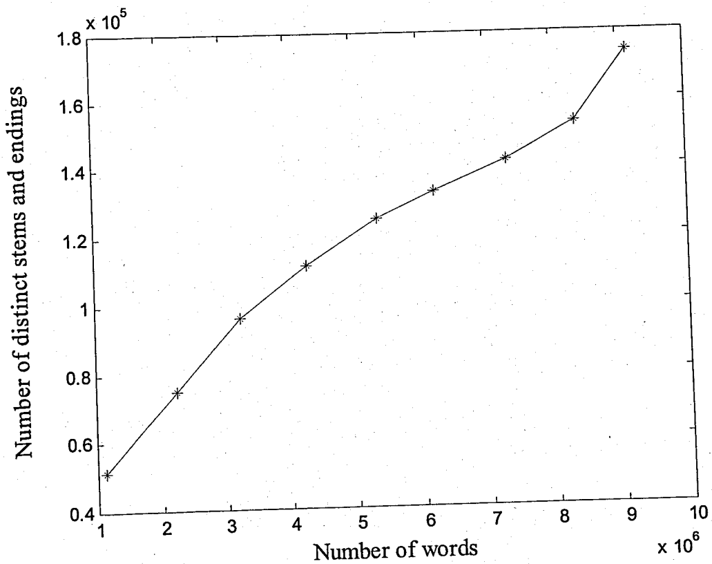
Figure 5.4. Number of distinct tokens (stems and endings) versus number of words in the stem-ending-tokenized training data set
