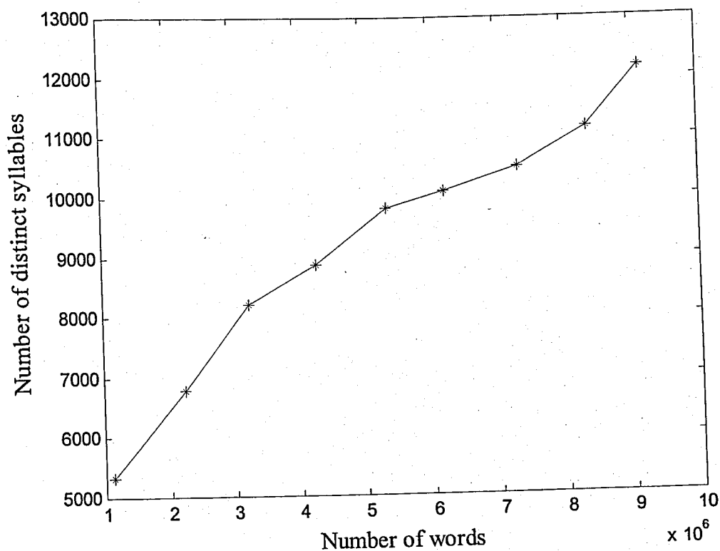
Figure 5.6. Number of distinct tokens (syllables) versus number of words in the syllable-tokenized training data set
