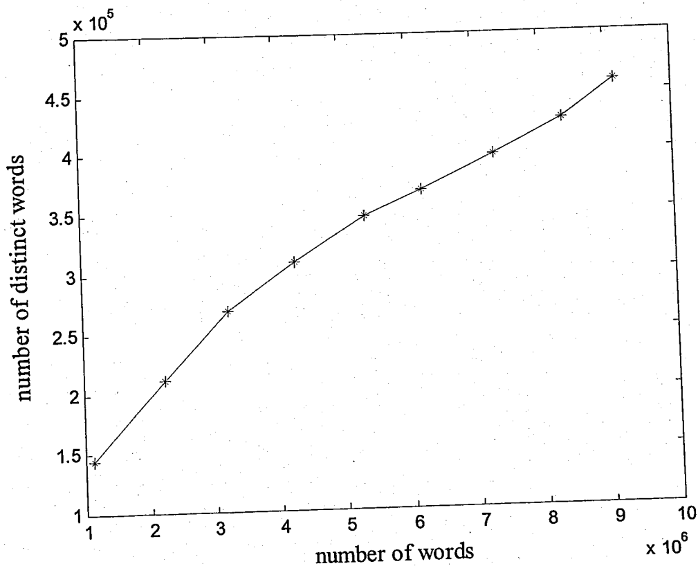
Figure 5.1. Number of distinct tokens (words) versus number of words in the word-tokenized training data set
