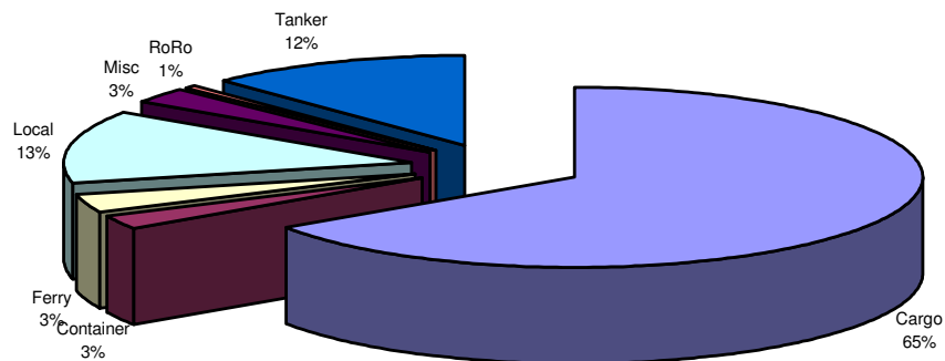
Figure 6.8. The percentage distributions of vessel types involved in accidents in the Istanbul Strait in the 1995-2004 period
